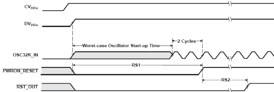
Figure 6-8 Reset Sequence
