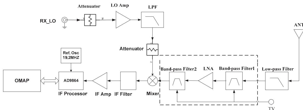
Figure 11-2 Block Diagram of Receiver Circuit
