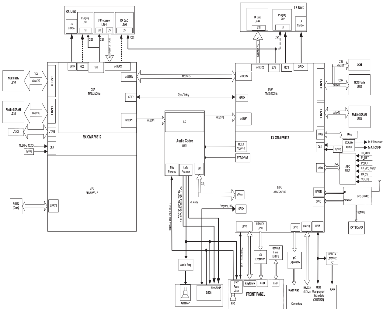
Figure 6-5 Baseband Block Diagram
