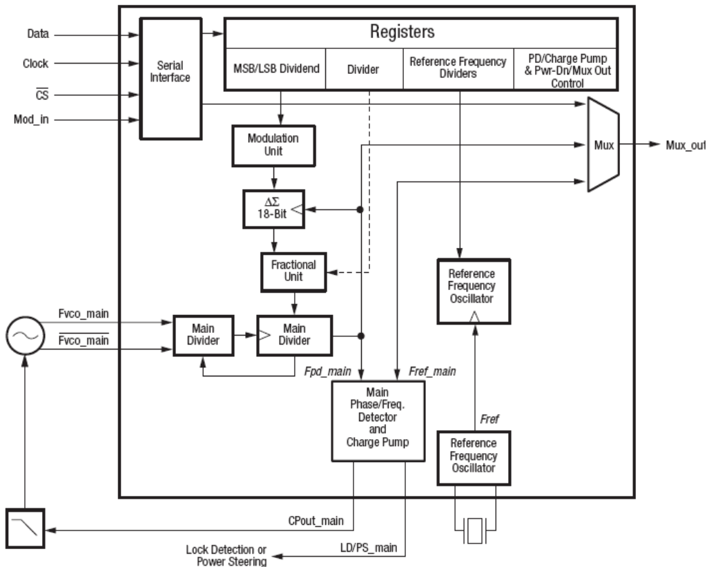
Figure 9-6 Block Diagram of PLL IC
