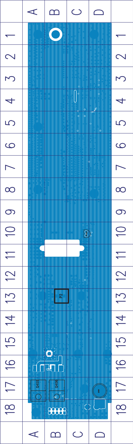
RD98X PCB View (PA Board) Bottom Layer
