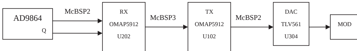
Figure 6-21 Relay Audio Path
