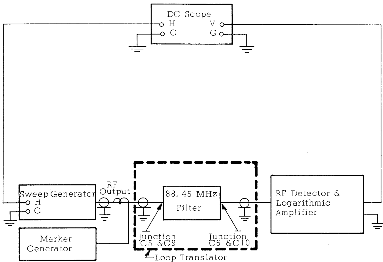
Figure 6. 1 Test set-up: 88.45-MHz filter alignment.
