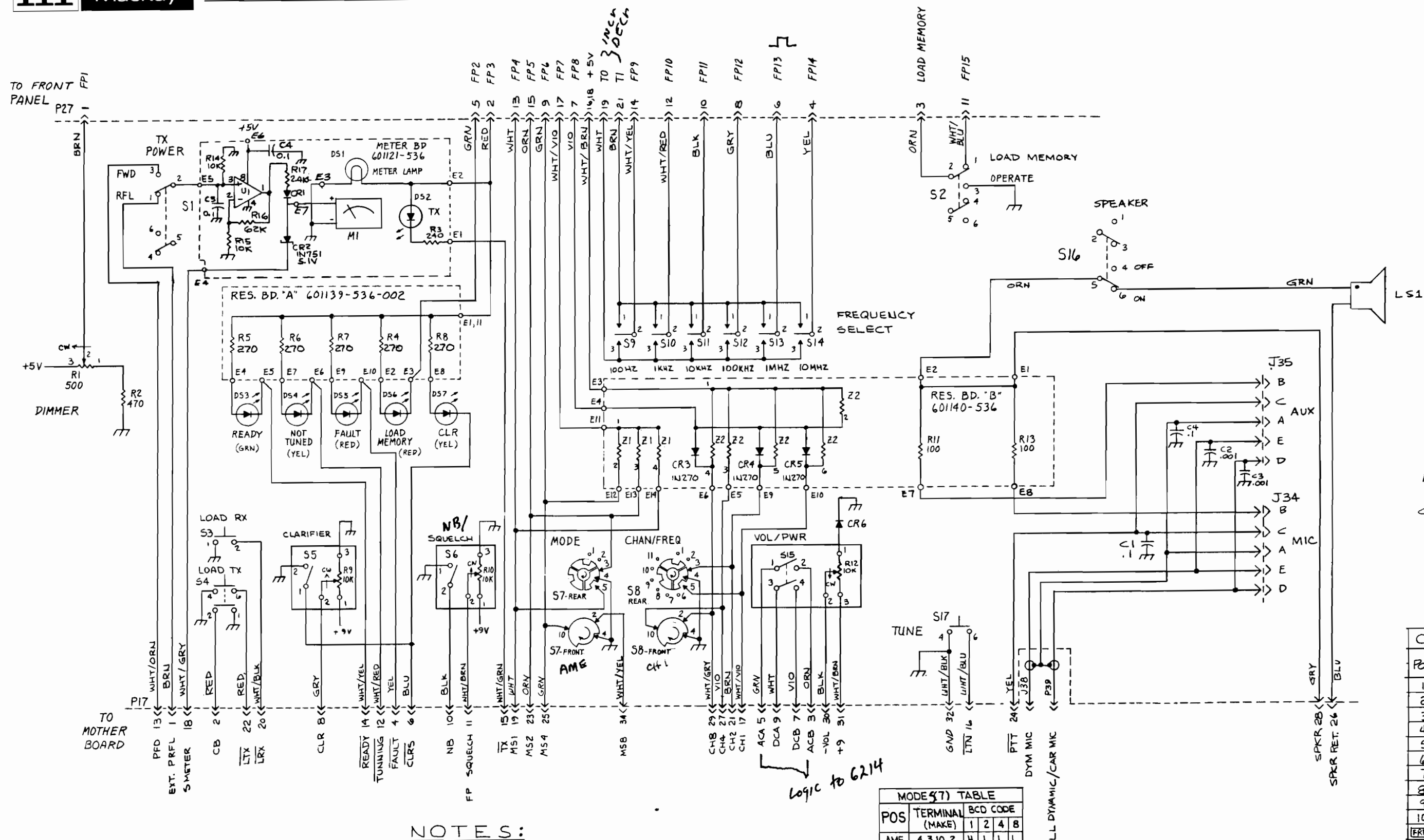
Figure 5.48 Front Panel Schematic
