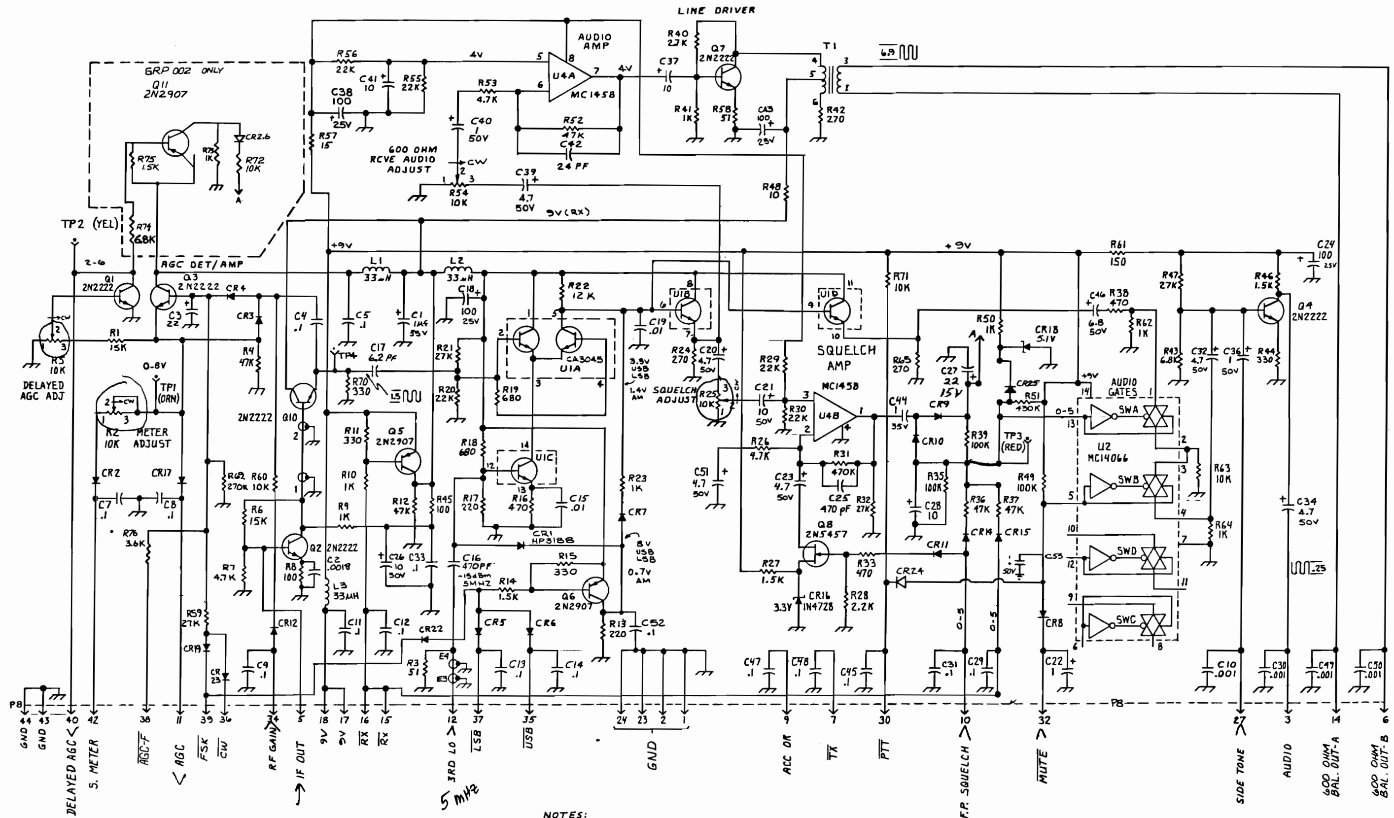
Figure 5.27 Audio/Squelch Schematic
