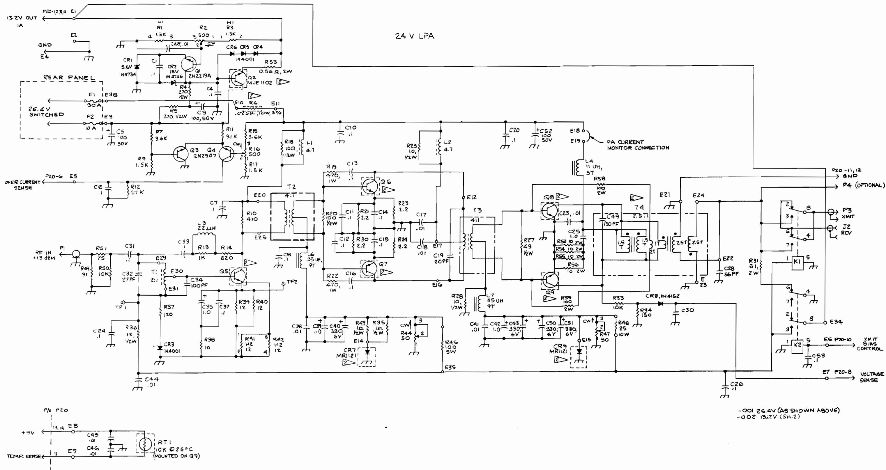
Figure 5.58 24 Volt Broadband Power Amplifier Schematic
