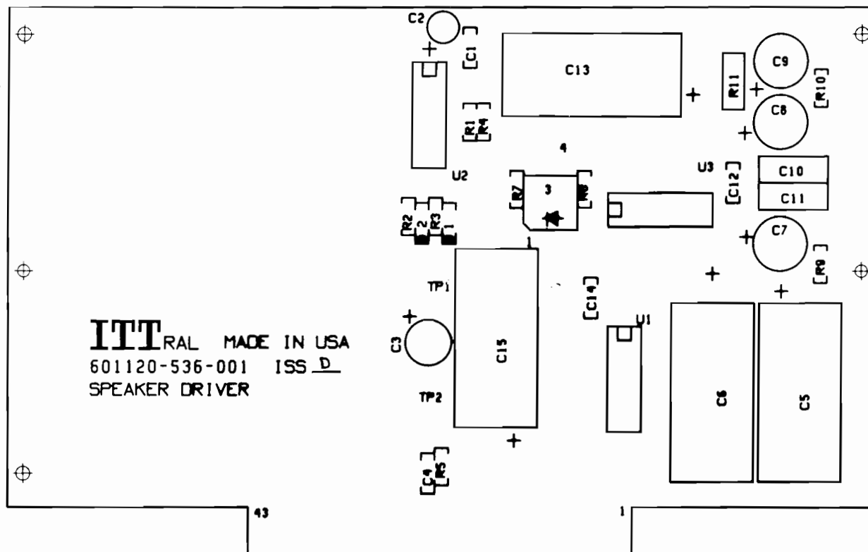
SPEAKER/DRIVER (601120-536)
