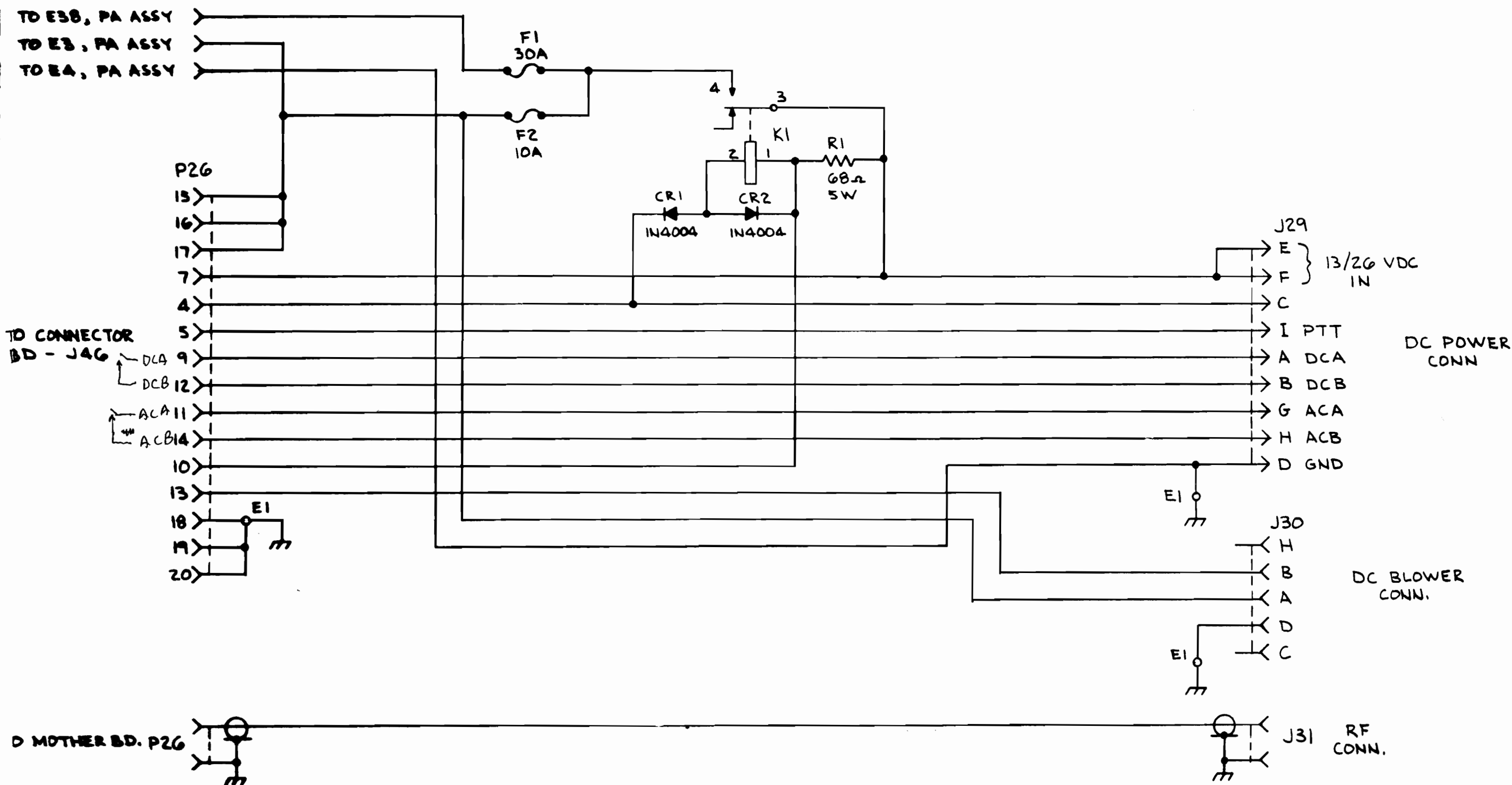
Figure 5.53 Rear Panel Schematic
