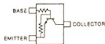
DTC114EU (Symbol: 24)
