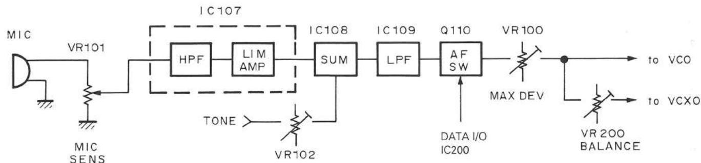
Fig. 4 Microphone amplification
