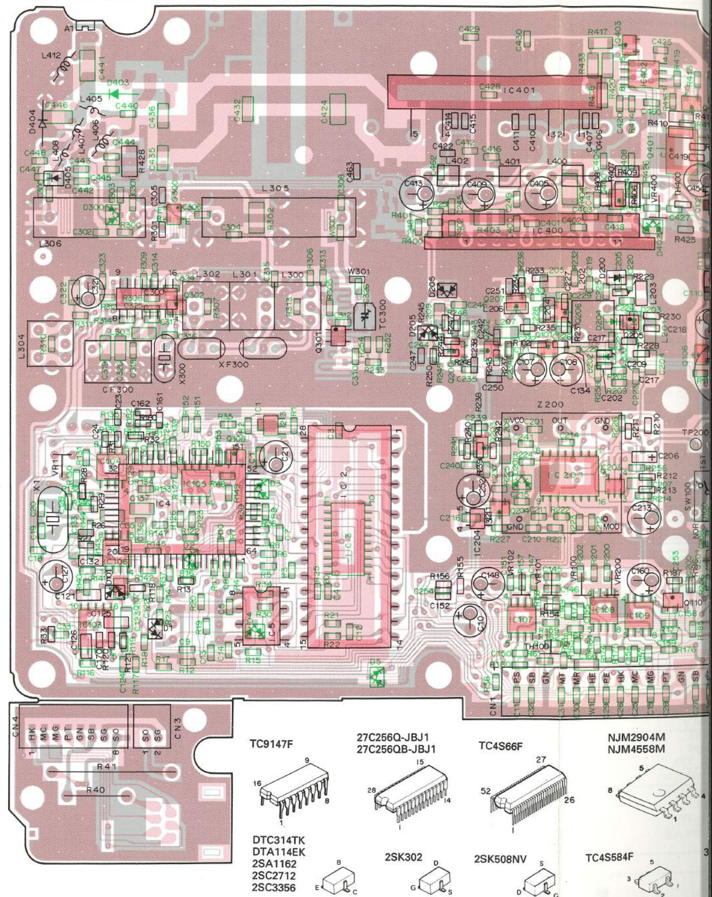
TX-RX UNIT (X57-3570-11) Foil side view
