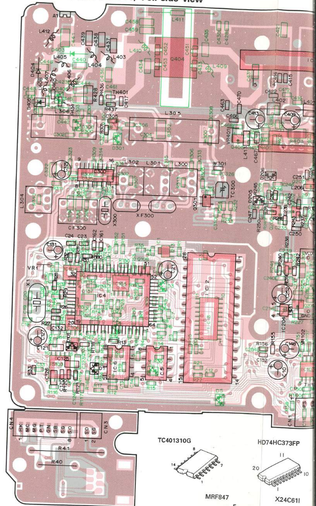
TX-RX UNIT (X57-3560-11) Foil side view
