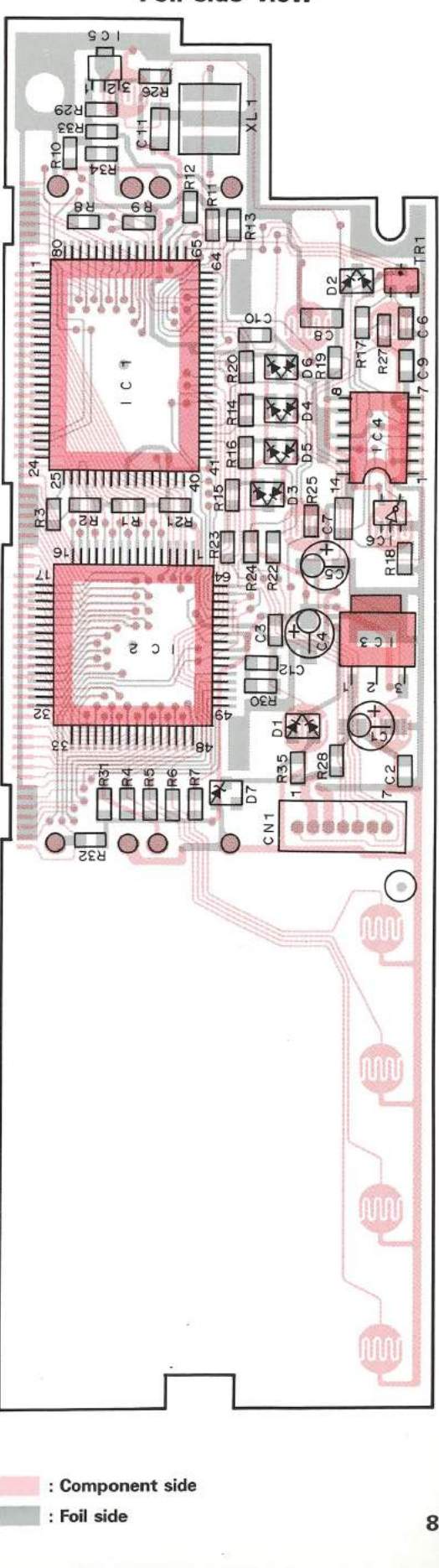
LCD ASS'Y (B38-0332-05) Foil side view
