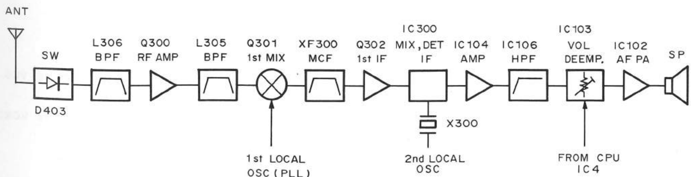
Fig. 2 Receiving system
