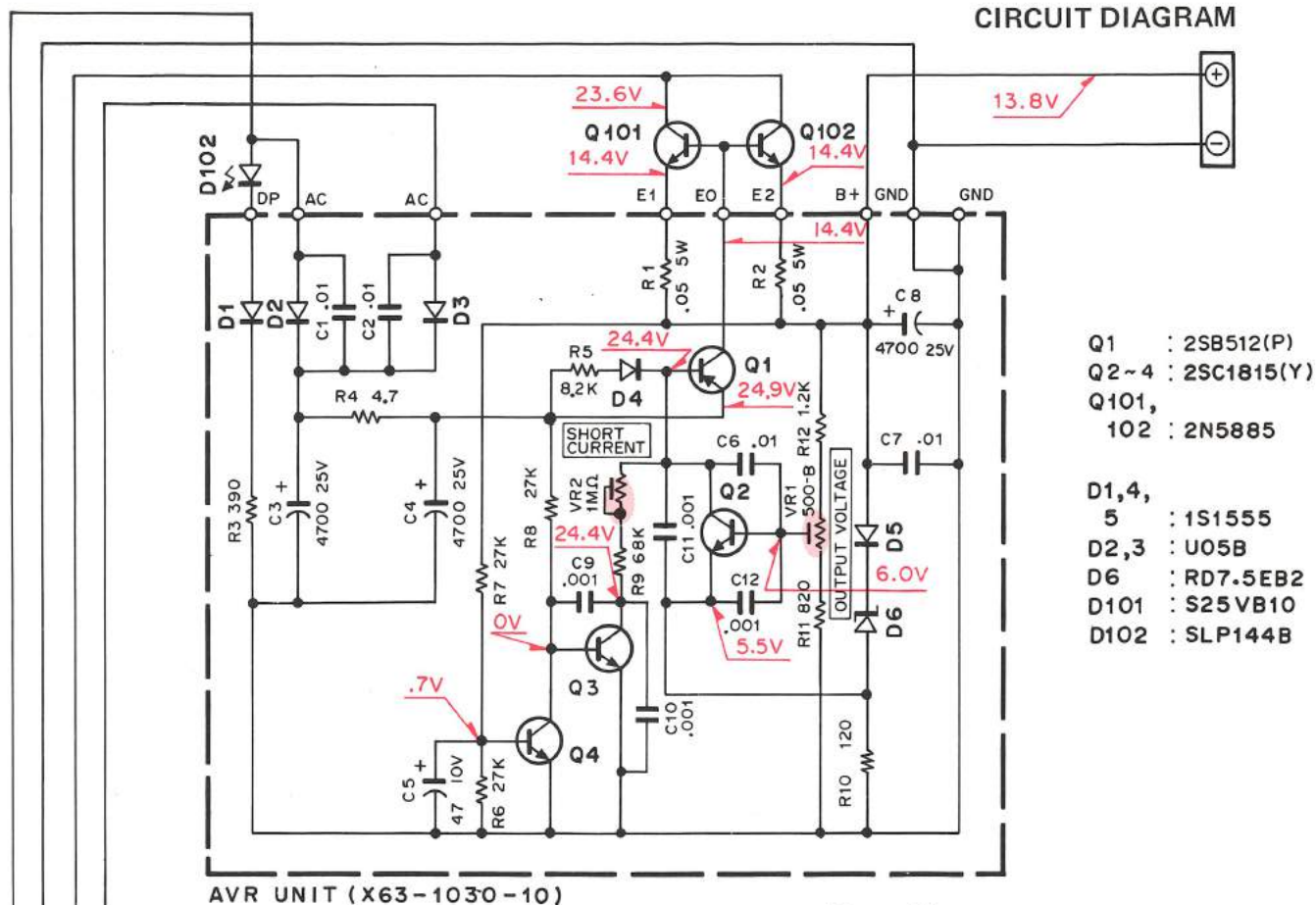
CIRCUIT DIAGRAM
