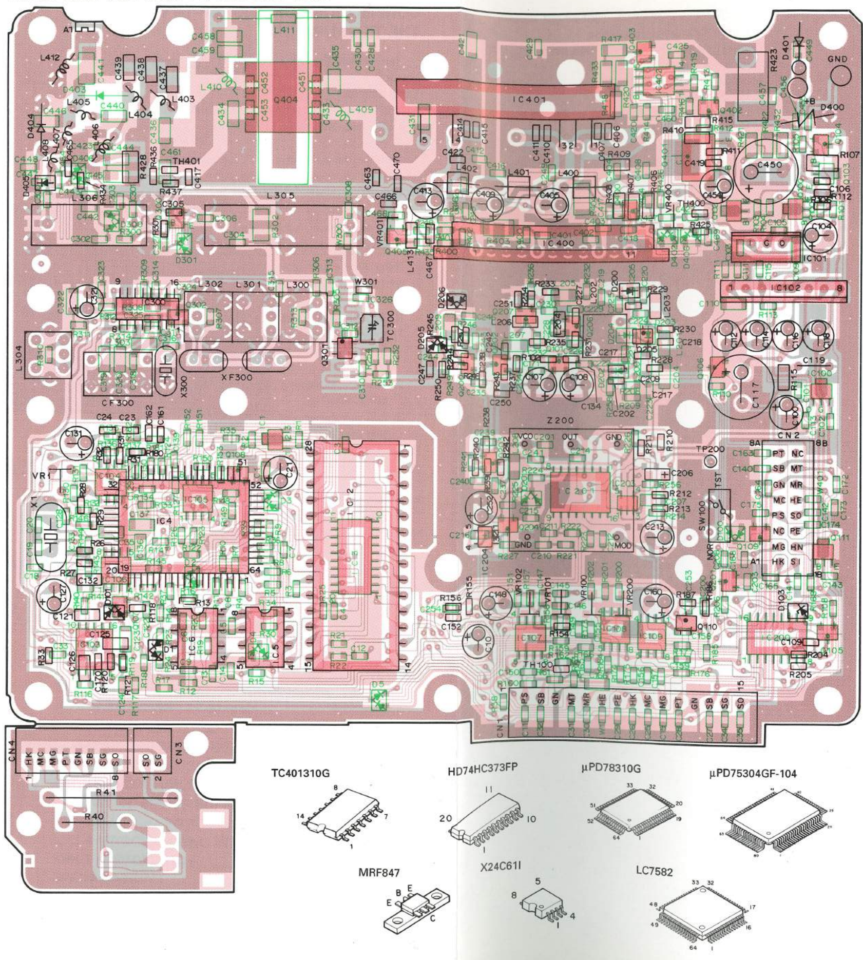
TX-RX UNIT (X57-3560-11) Foil side view
