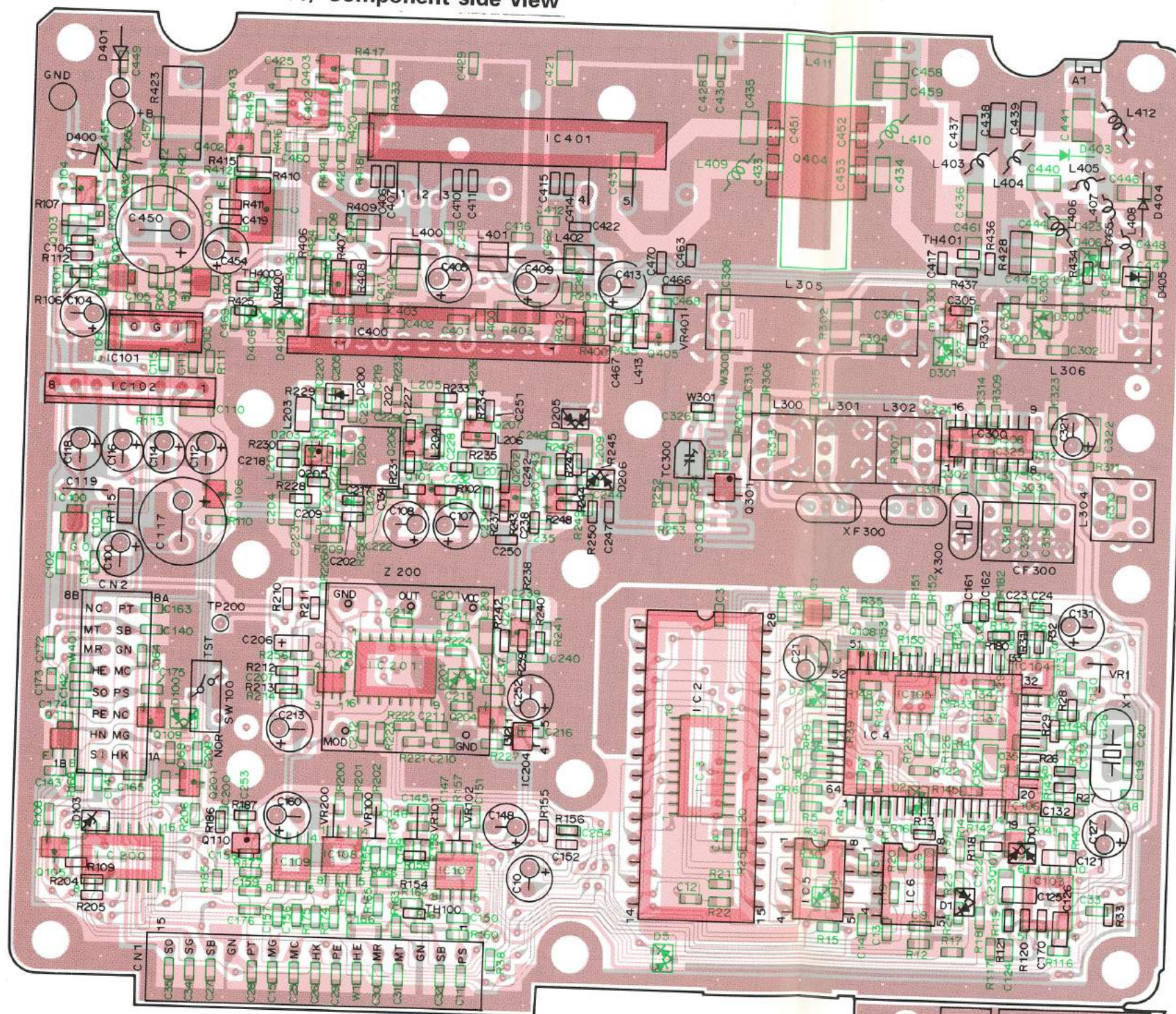
TX-RX UNIT (X57-3560-11) Component side view
