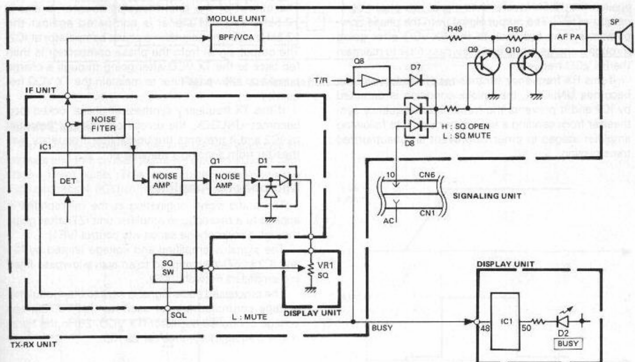
Fig. 3 Squelch circuit
