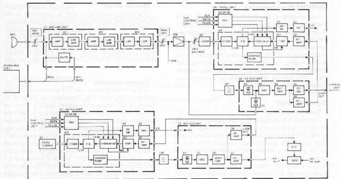
Fig. 4 PLL &amp; Modulation circuit block diagram
