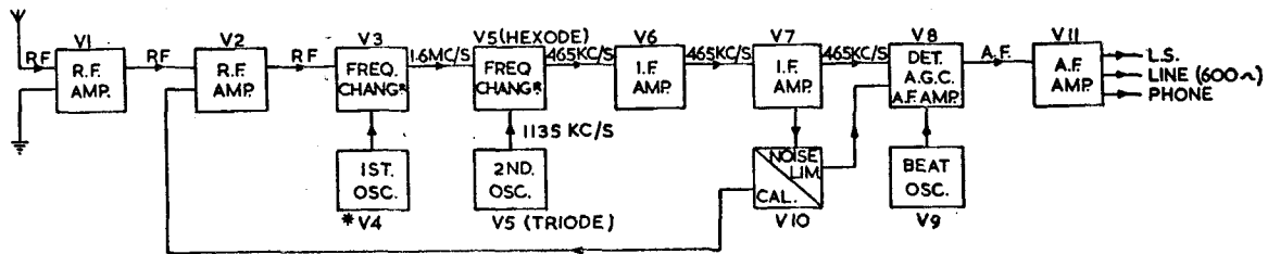
FIG. 2. BLOCK DIAGRAM.
