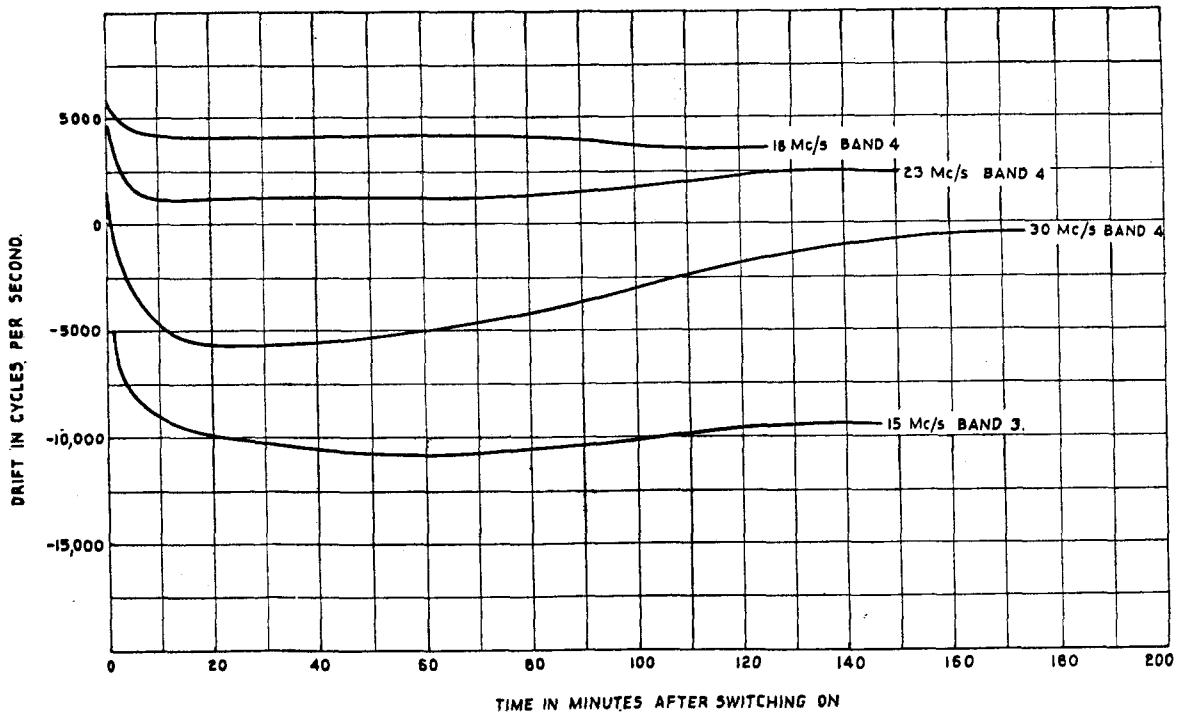
FIG. 16. FREQUENCY DRIFT.
