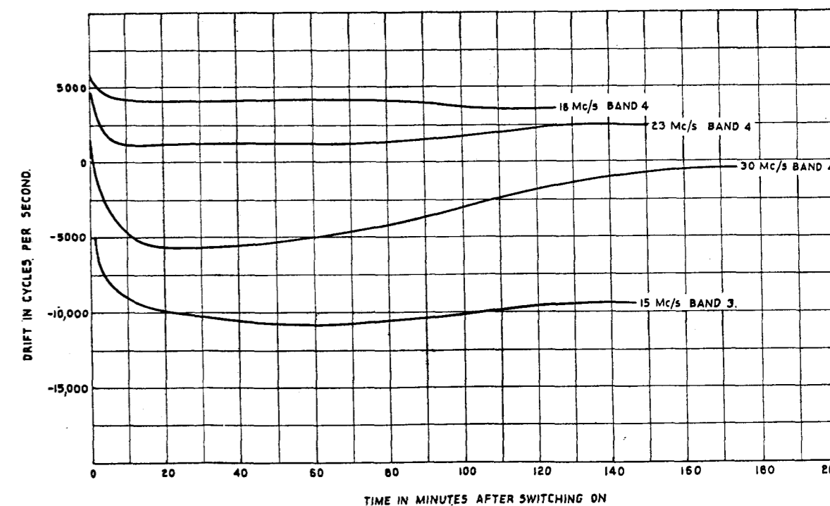
FIG. 16. FREQUENCY DRIFT.
