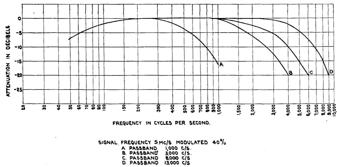
FIG. 14. OVERALL FREQUENCY RESPONSE.
