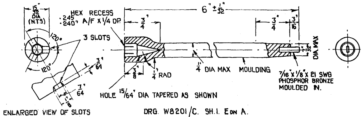
FIG. 6. GANGING TOOL
