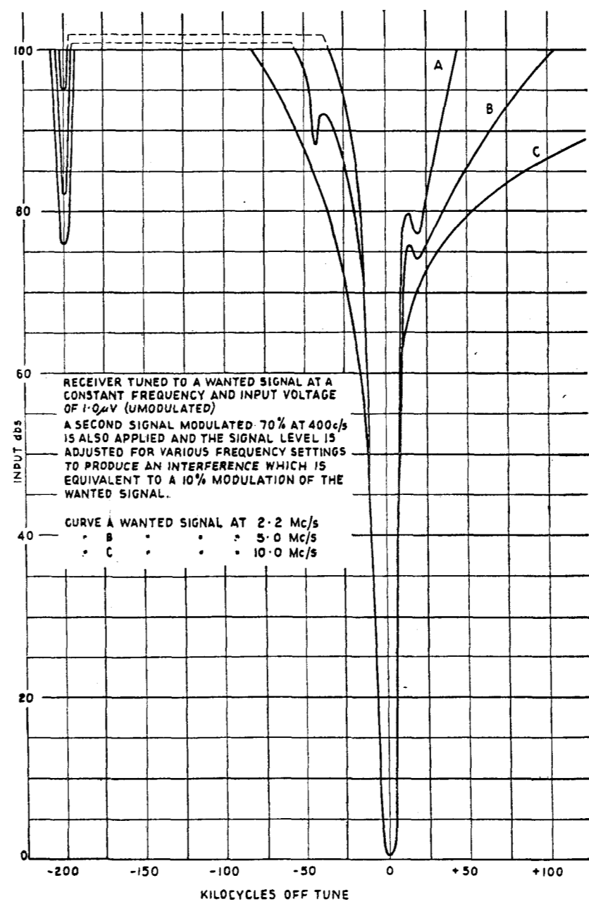
FIG. 13. SELECTIVITY CURVES.
