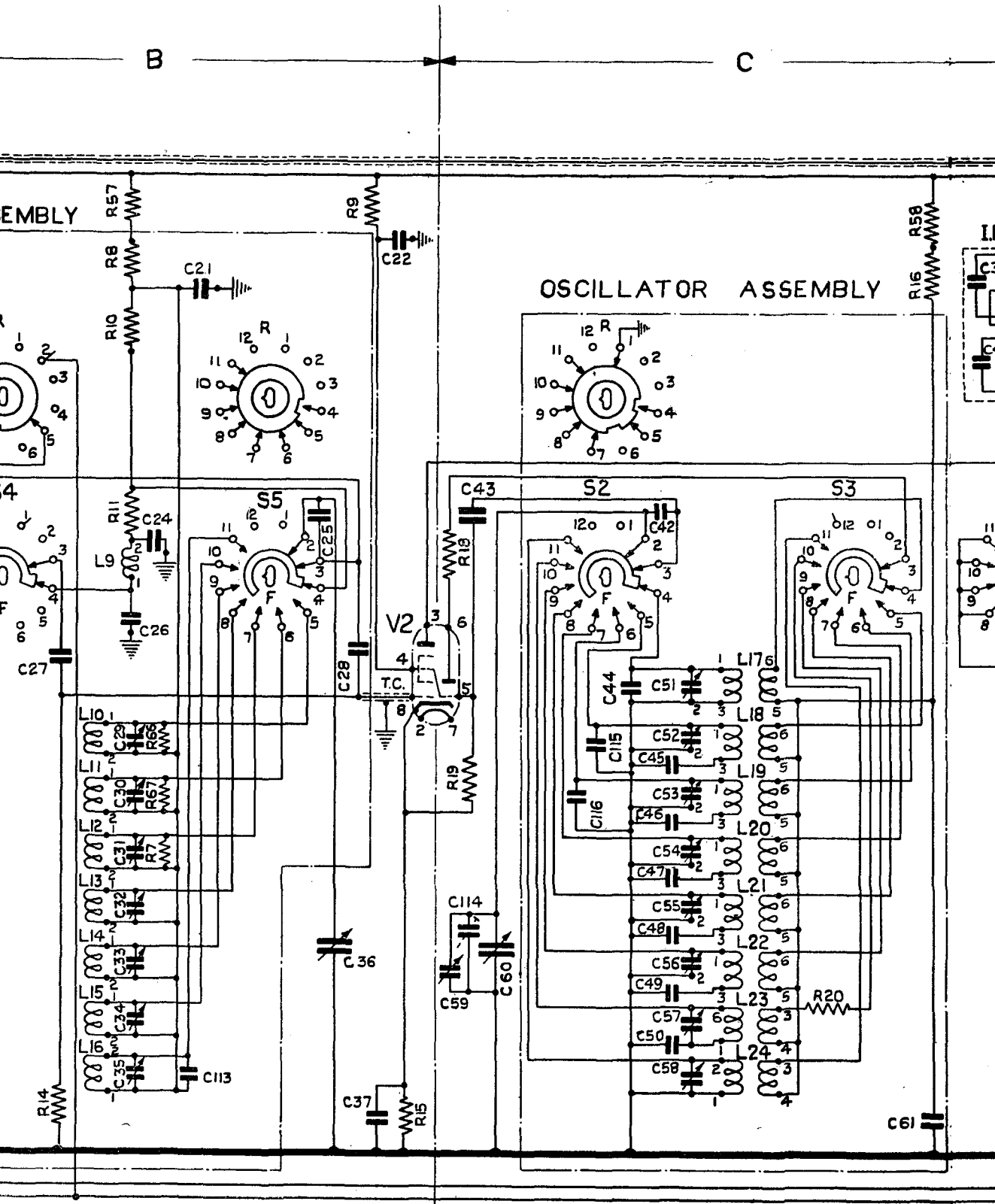
CIRCUIT DIAGRAM OF TYPE CR
