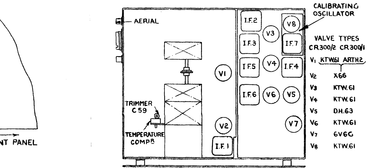
Fig. 6. Position of Valves in Receiver.
