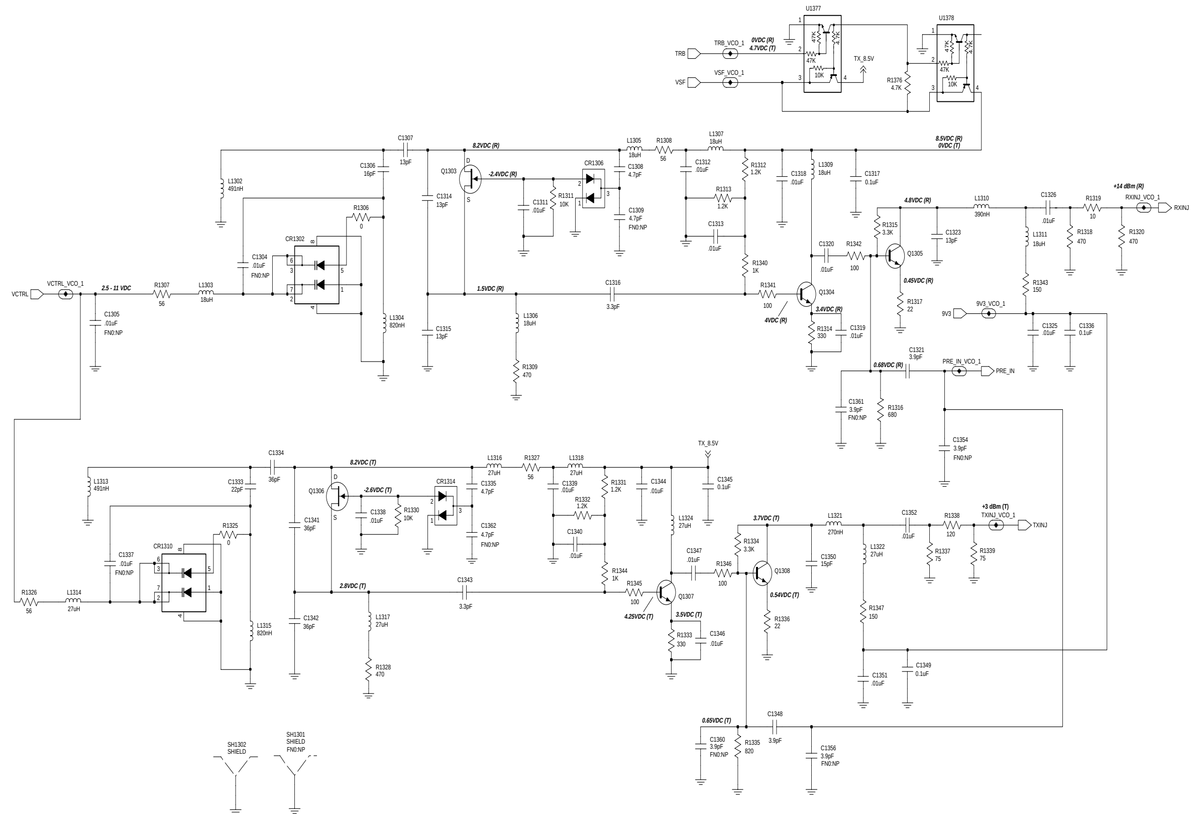
Low Band Range 3 (42-50 MHz) Voltage Controlled Oscillator
