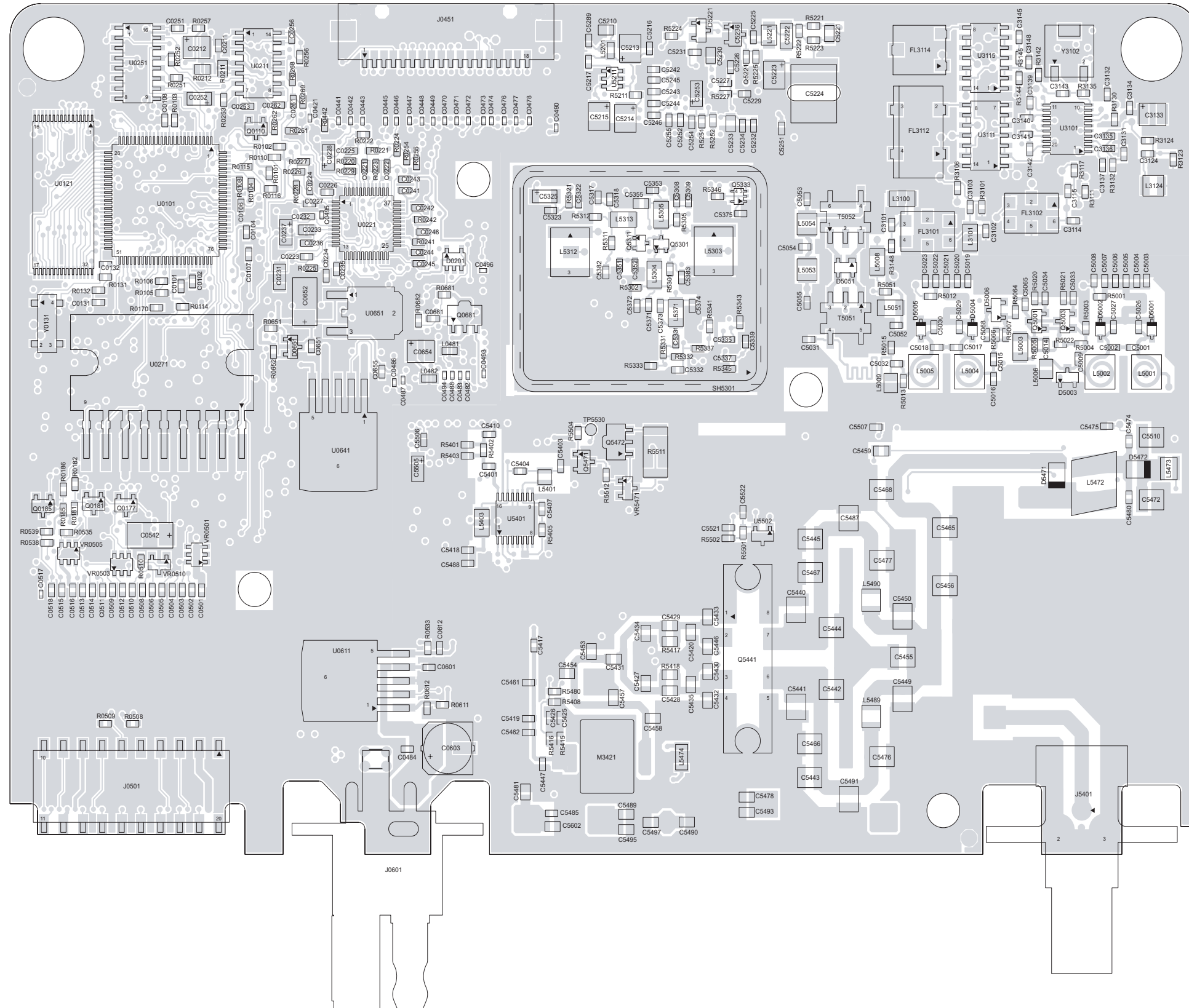
UHF Band 2 (450-512/520 MHz) 25-40W LDMOS PCB 8486250Z02 Top Side
