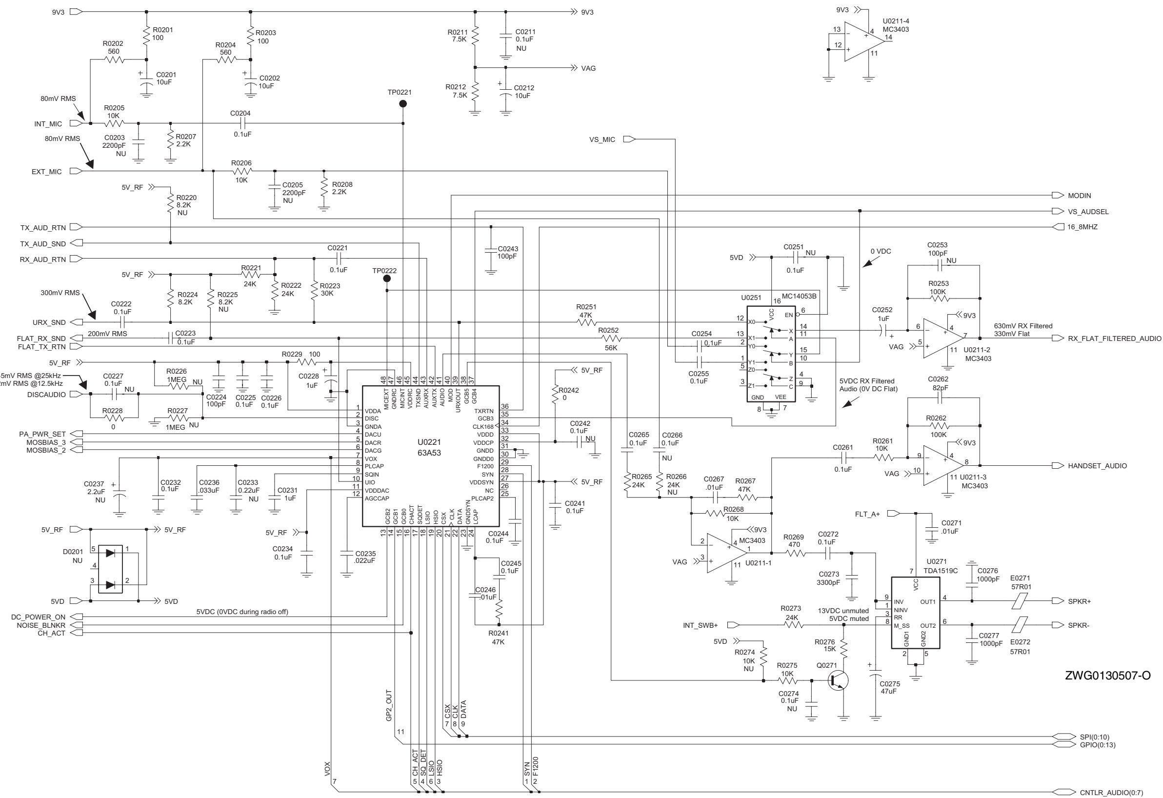
Controller T5 Schematic Diagram - Audio
