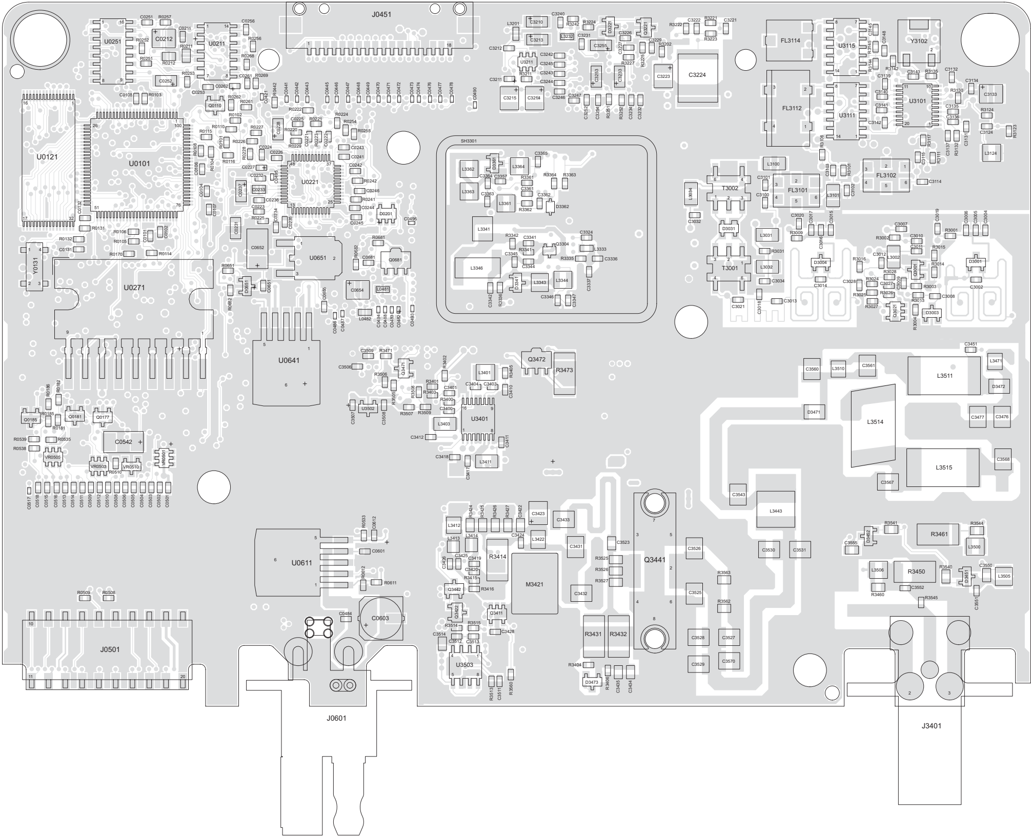
VHF (136-174 MHz) 25-45W LDMOS PCB 8486140B15 Top Side
