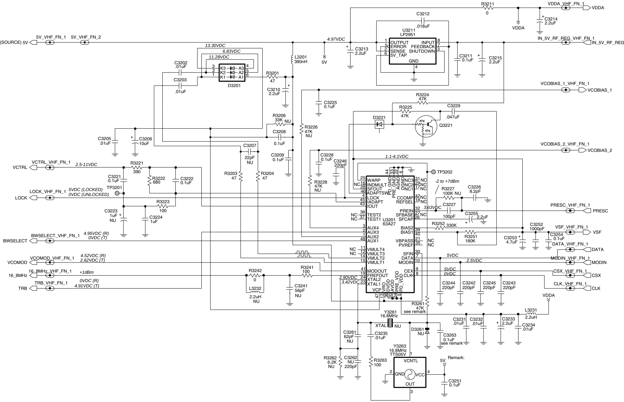
VHF (136-174 MHz) 1-25W FRACN Synthesizer
