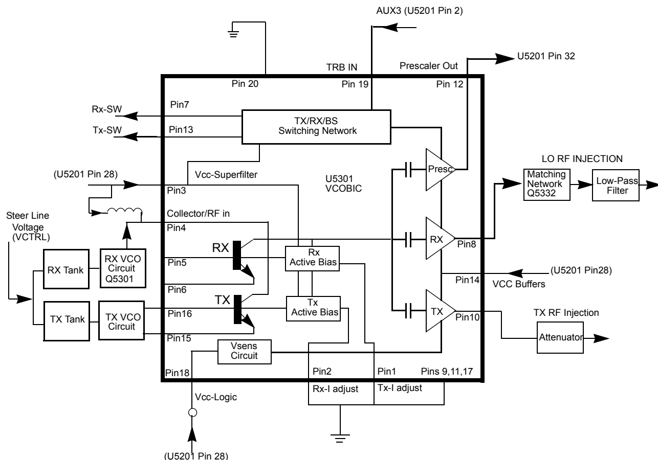
Figure 6-4 UHF VCO Block Diagram
