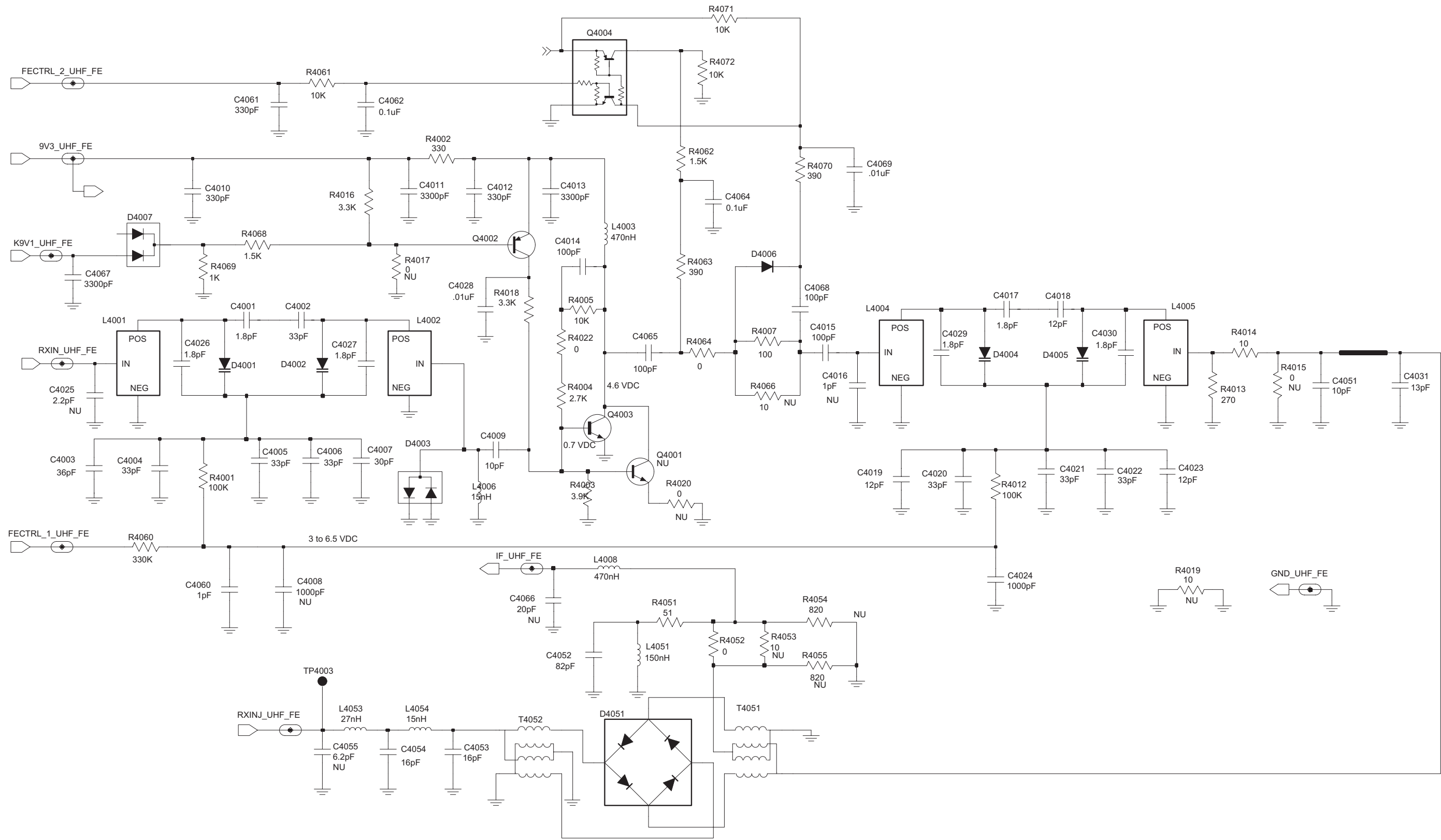
UHF Band 1 (403-470 MHz) 25-40W LDMOS Receiver Front-End
