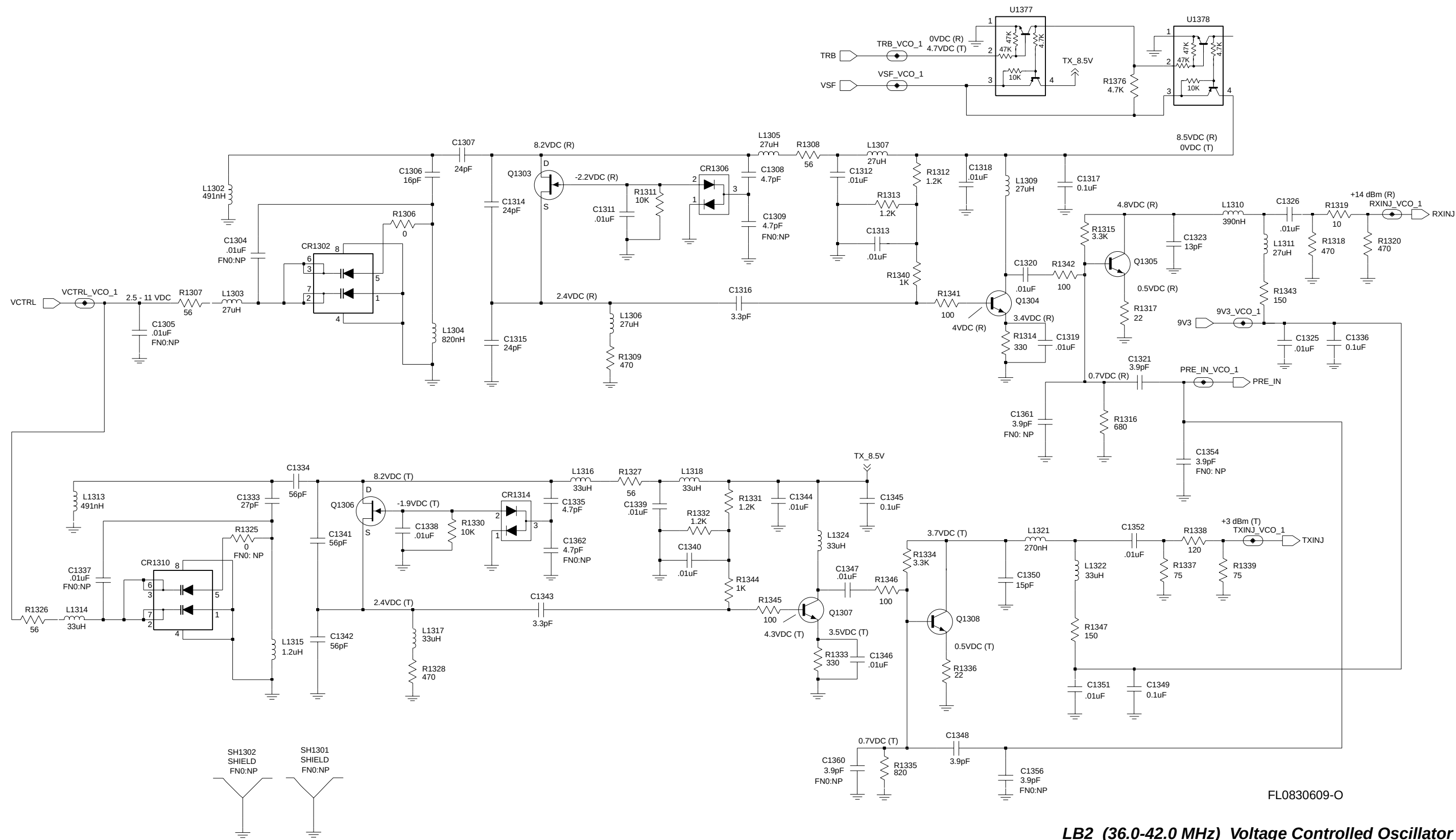
LB2 (36.0-42.0 MHz) Voltage Controlled Oscillator
