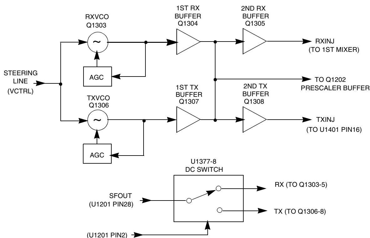
Figure 2-4 LowBand VCO/Buffer Block Diagram
