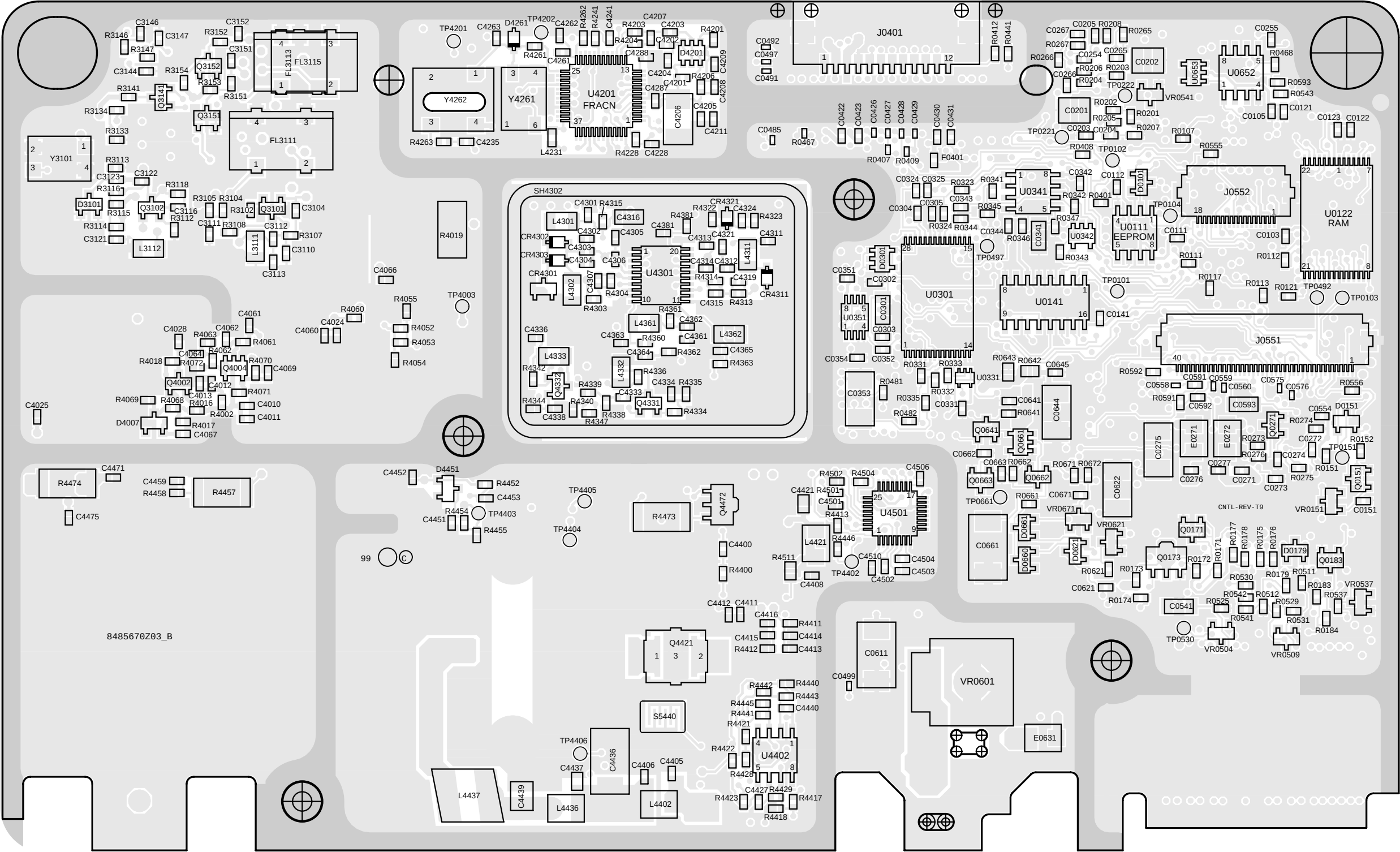
UHF (403-470MHz) 1-25W 8485670z03 Bot Side
