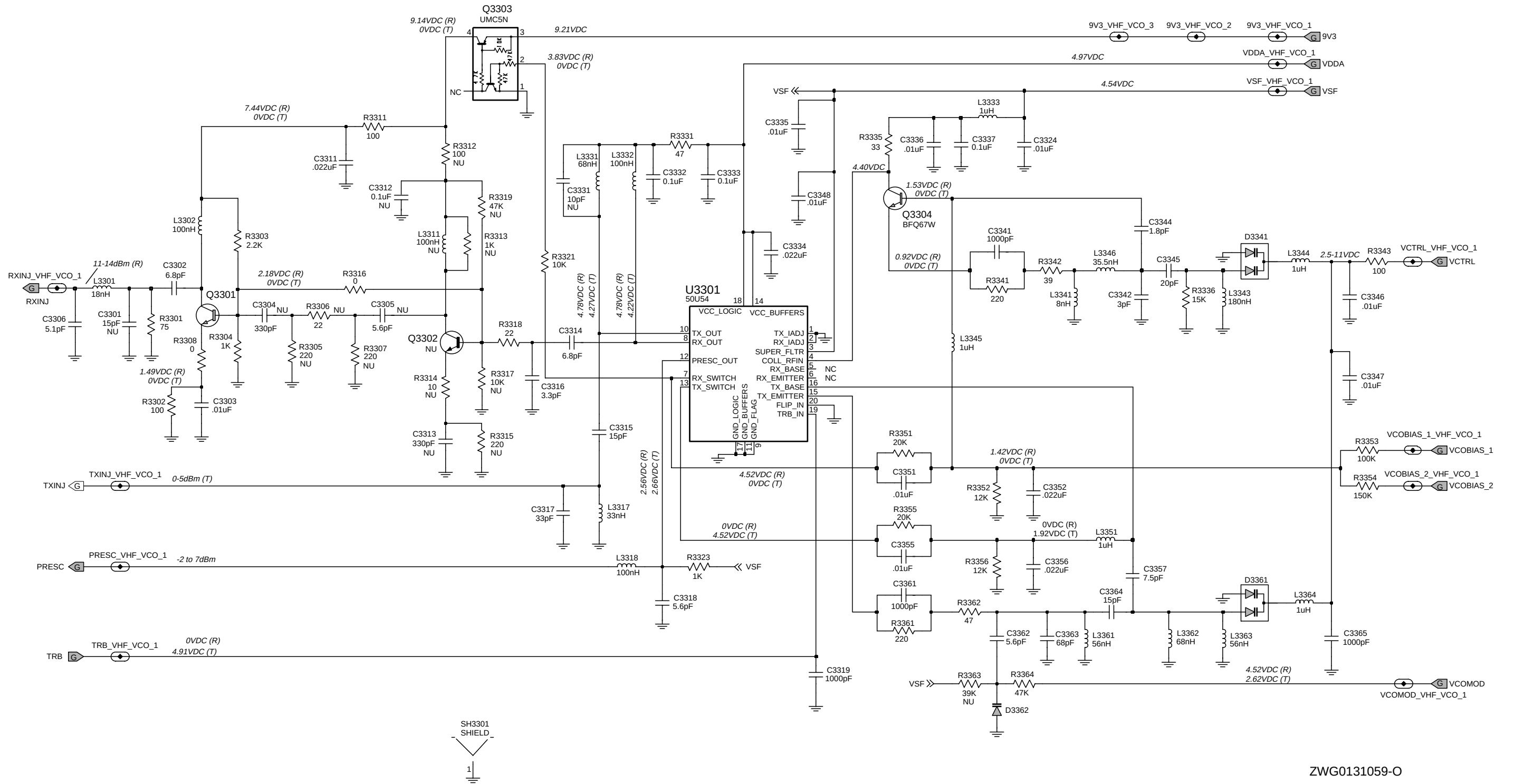
VHF (136-174 MHz) Voltage Controlled Oscillator
