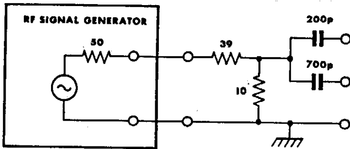
Fig. 8.1 Dummy Aerial Network
