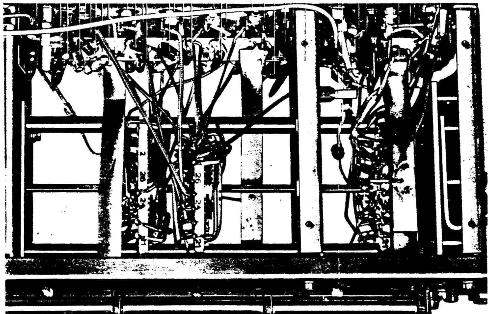
... im HF-Verstärker Rel 455 V 311a (von links gesehen) ... in the RF amplifier Type Rel 455 V 311a (viewed from the left)
