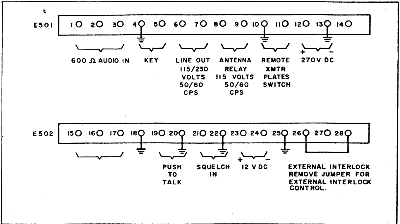
Figure 2-3. Cabinet Frame Assembly, CAB-7, Terminal Board Connections
