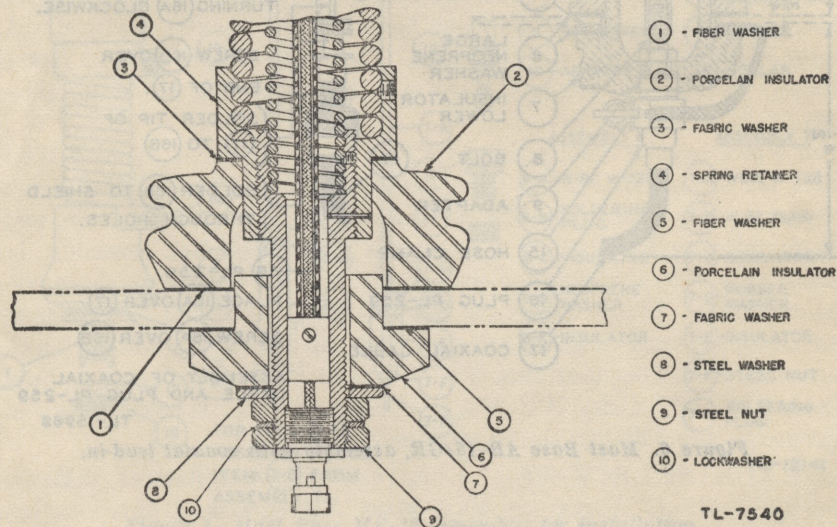
Figure 8. Mast Base MP-57, assembly for installation.
