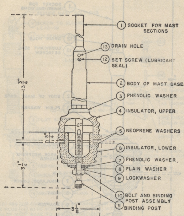
Figure 4. Mast Base MP-65-A, assembly for installation.
