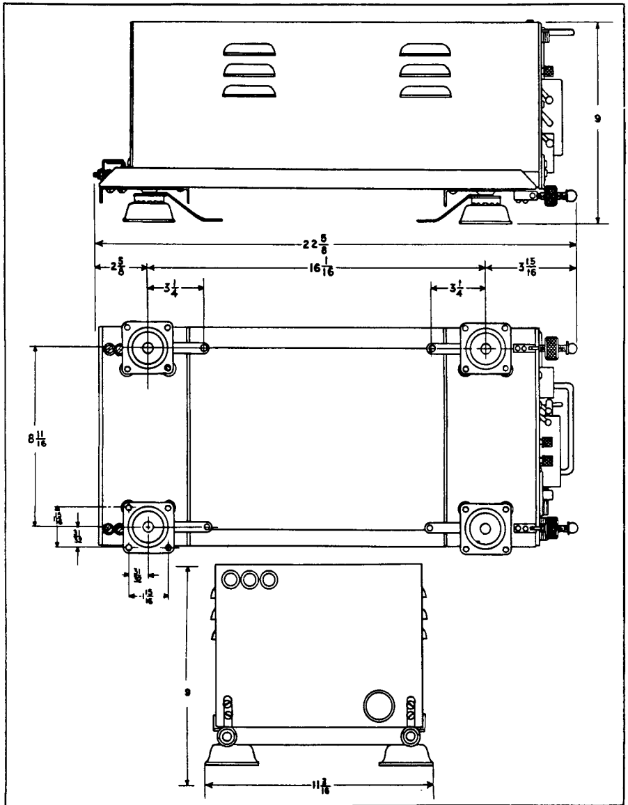
Figure 7-3. Radio Receivers R-45/ARR-7 and R-595/ARR-7AX — Outline Dimensions
