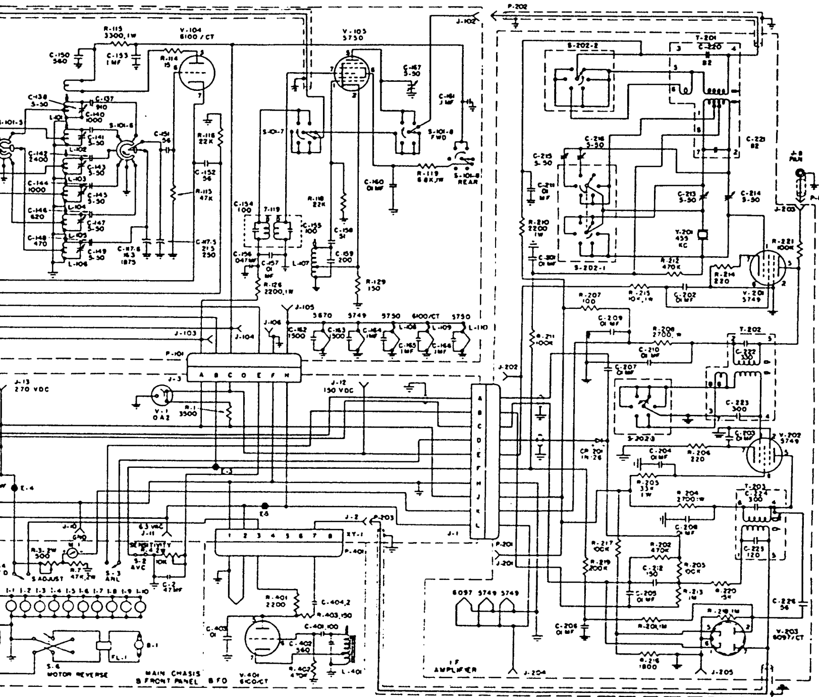
Figure 7-7. Radio Receiver R-595 ARR-7AX — Schematic Circuit Diagram
