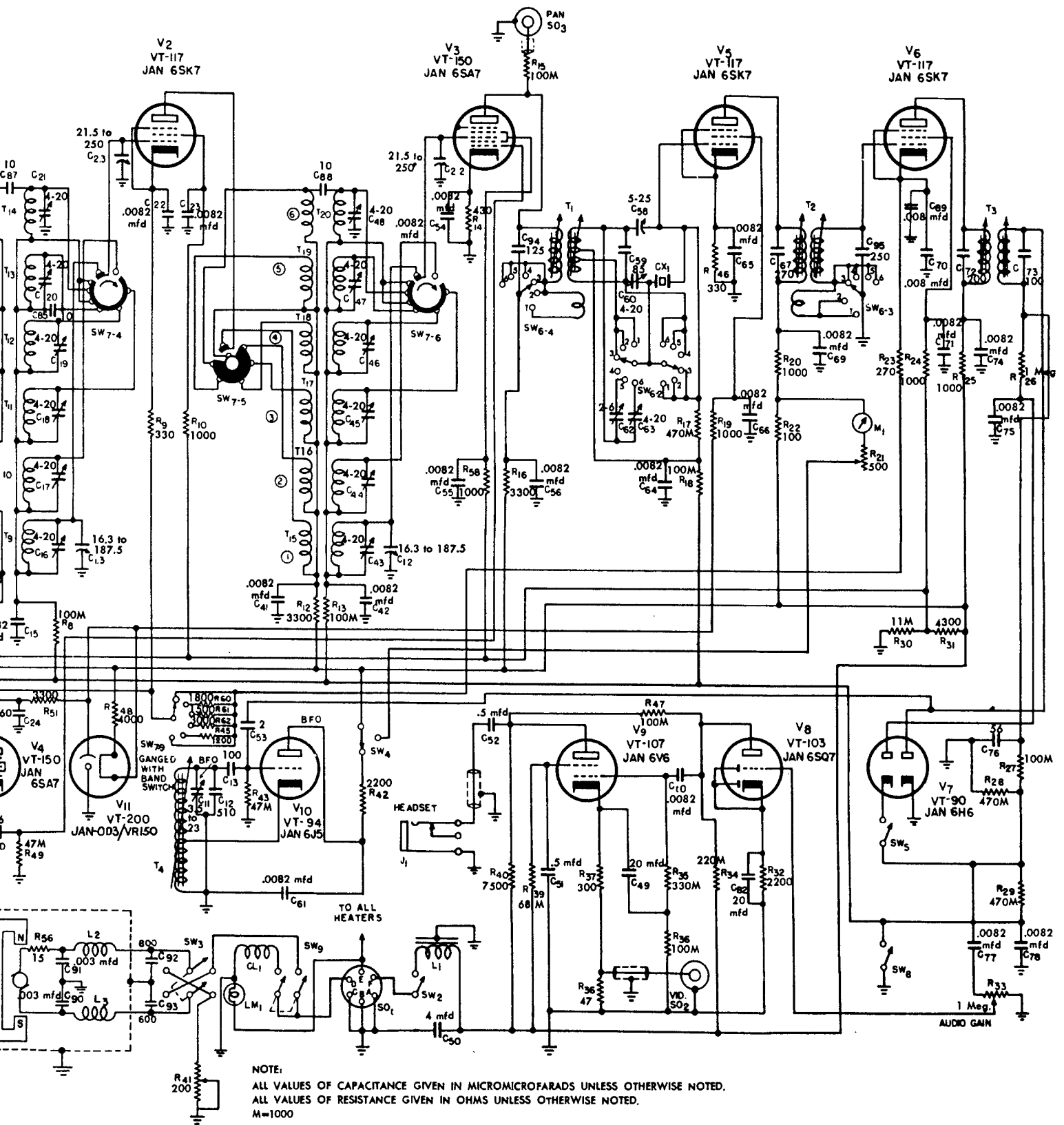
Figure 7-5. Radio Receiver R-45/ARR-7 — Schematic Circuit Diagram
