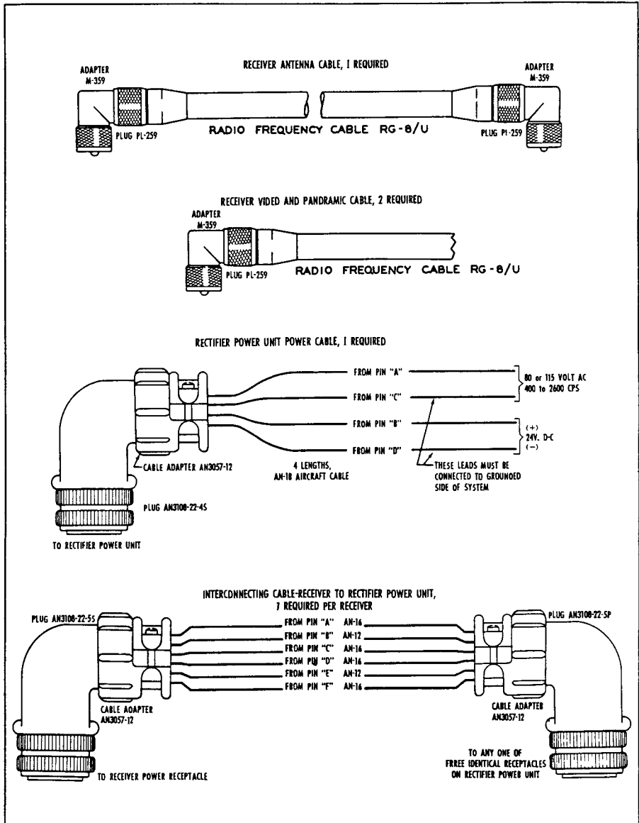
Figure 7-2. Radio Receiving Sets AN/ARR-7 and AN/ARR-TAX—Cable Assembly Diagram
