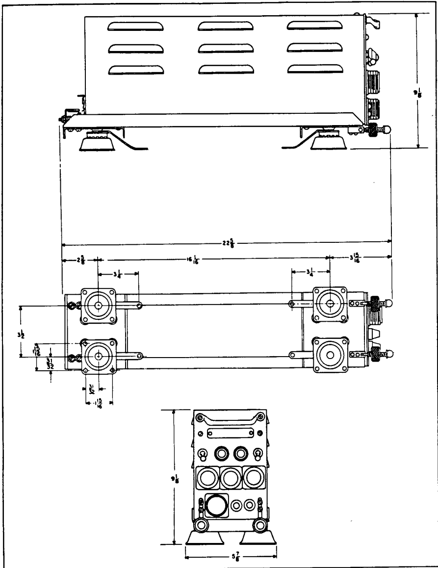
Figure 7-4. Rectifier Power Unit PP-32/AR — Outline Dimensions
