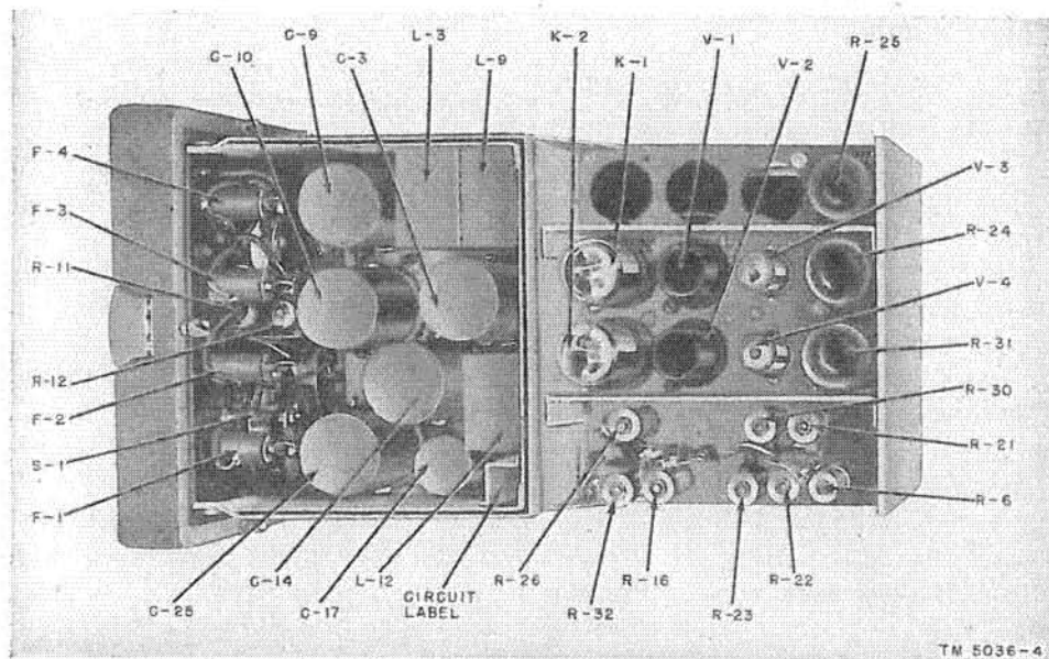
Figure 66. Power supply PP-109/GR, top view of chassis.
