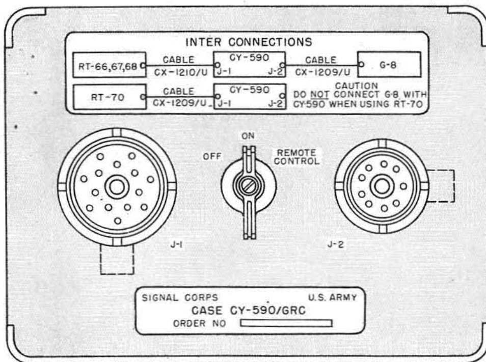
Figure 78. Case CY-590/GRC, front panel.
