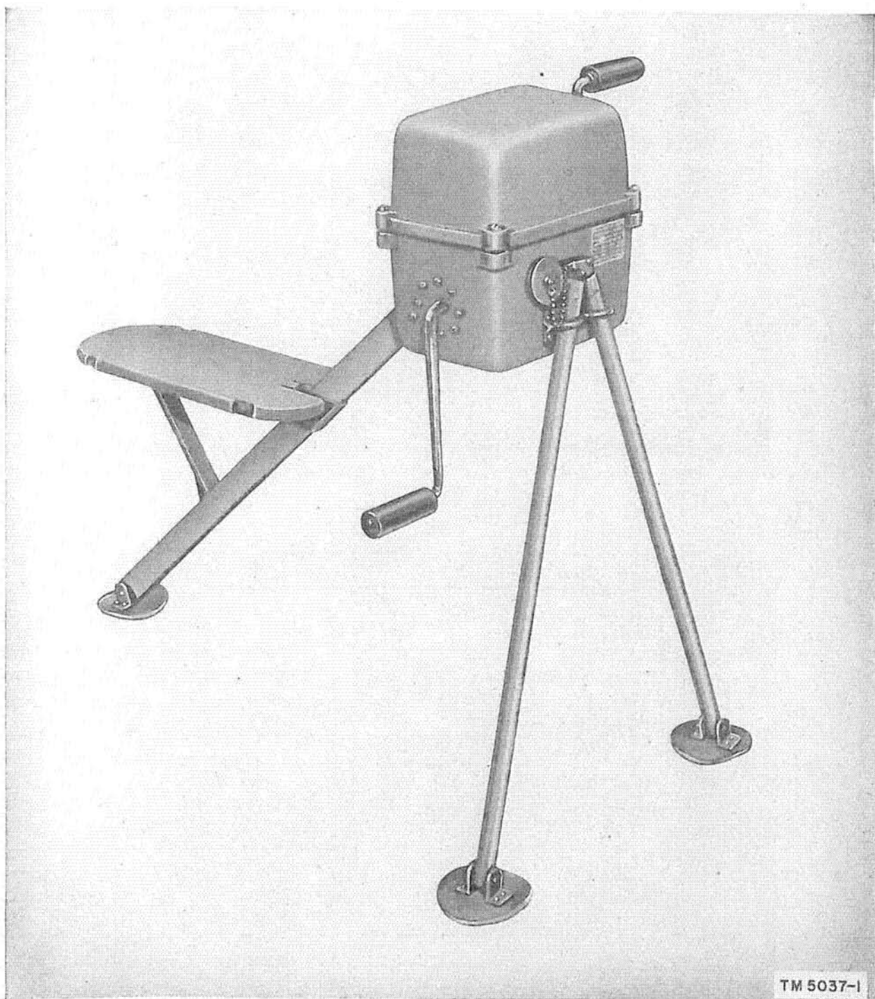
Figure 76. Generator G-8/GRC.
