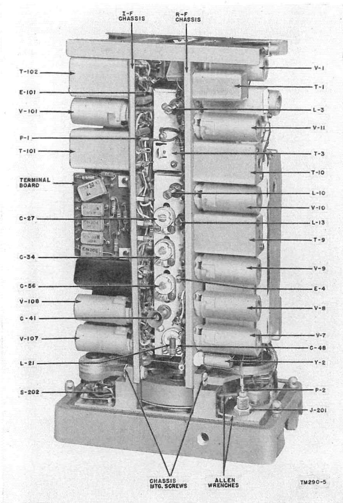
Figure 62. Set 2, top view of panel-chassis assembly.
