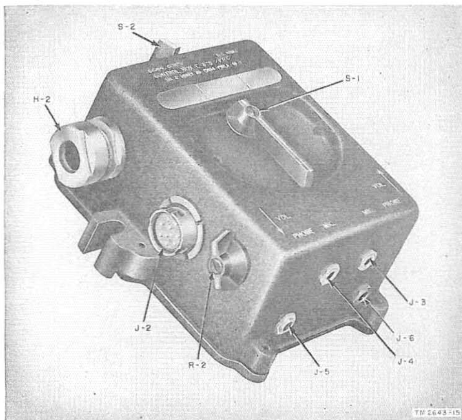
Figure 73. Control box C-375/VRC, left oblique view.
