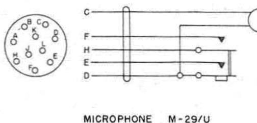
Figure 95. Audio accessories, schematic diagram.
