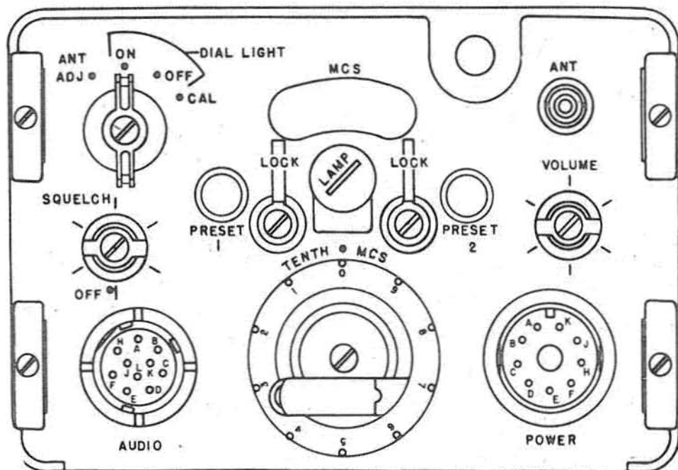
Figure 34. Set 2 panel.
