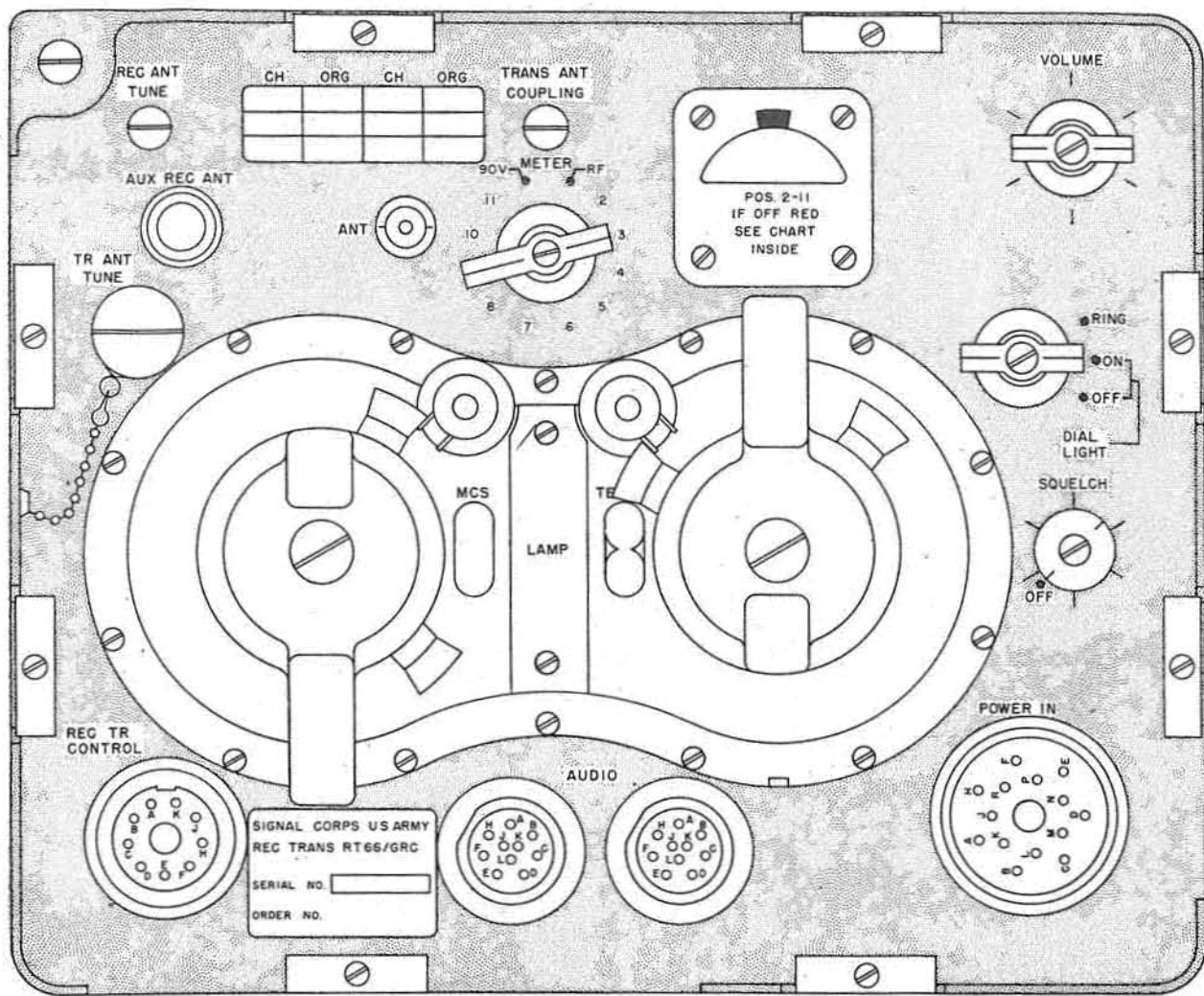
Figure 36. Set 1 panel.
