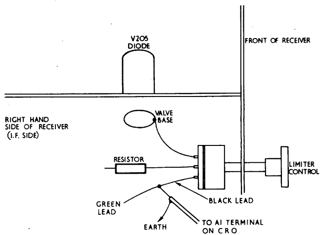
CONNECTION TO RECEIVER FROM CRO FIG. 9
