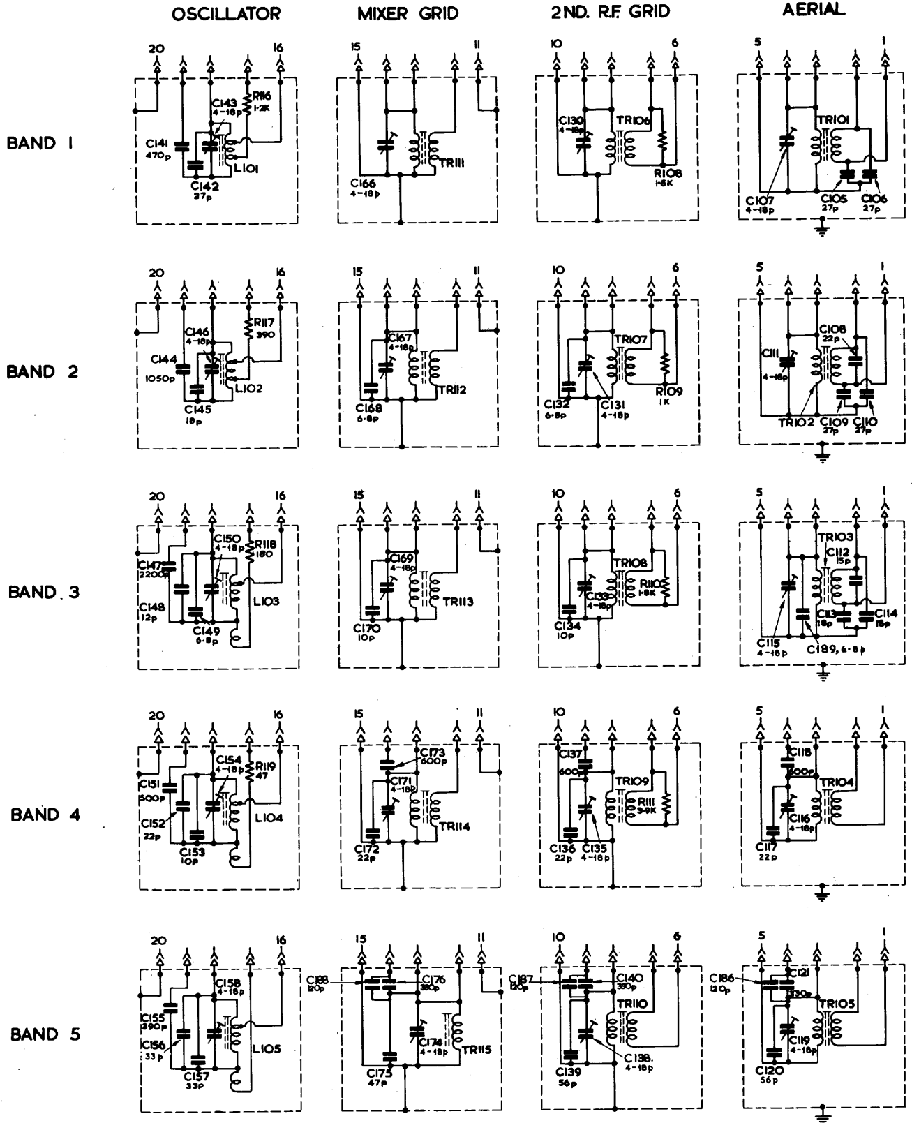
RECEIVER B40 A.P. 57140 D. TURRET SWITCH COMPONENTS. CIRCUIT DIAGRAM.
