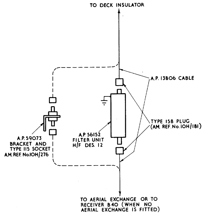
FILTER UNIT DES.12 AP.56152. INSTALLATION DIAGRAM. FIG. 10
