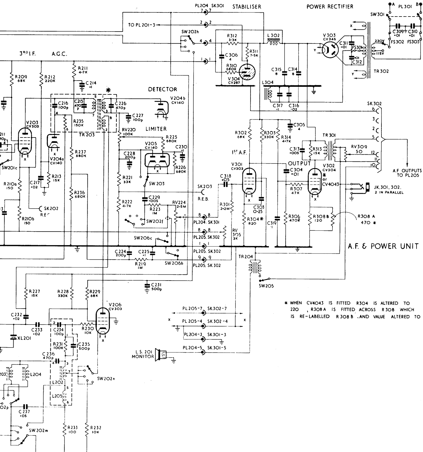
RECEIVER 62B. A.P. 67757 CIRCUIT DIAGRAM.
