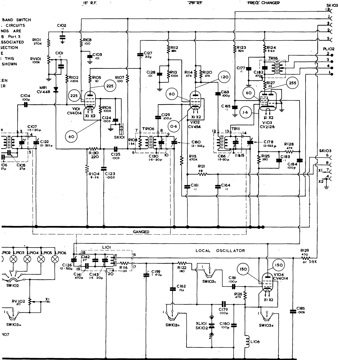
RECEIVER B40 A.P. 57140D R.F. UNIT CIRCUIT DIAGRAM
