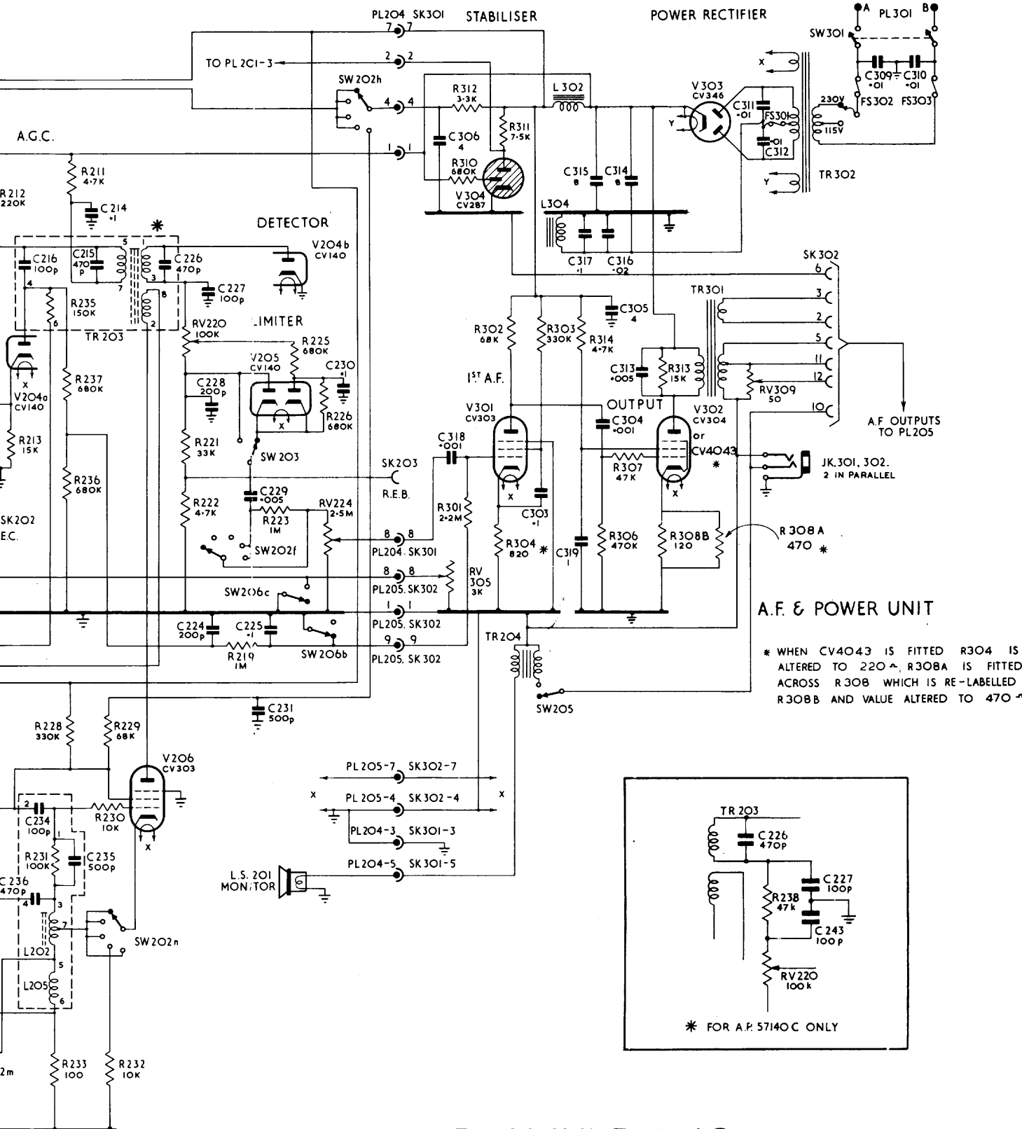
RECEIVER B40. A.P. 57140B/C. CIRCUIT DIAGRAM.
