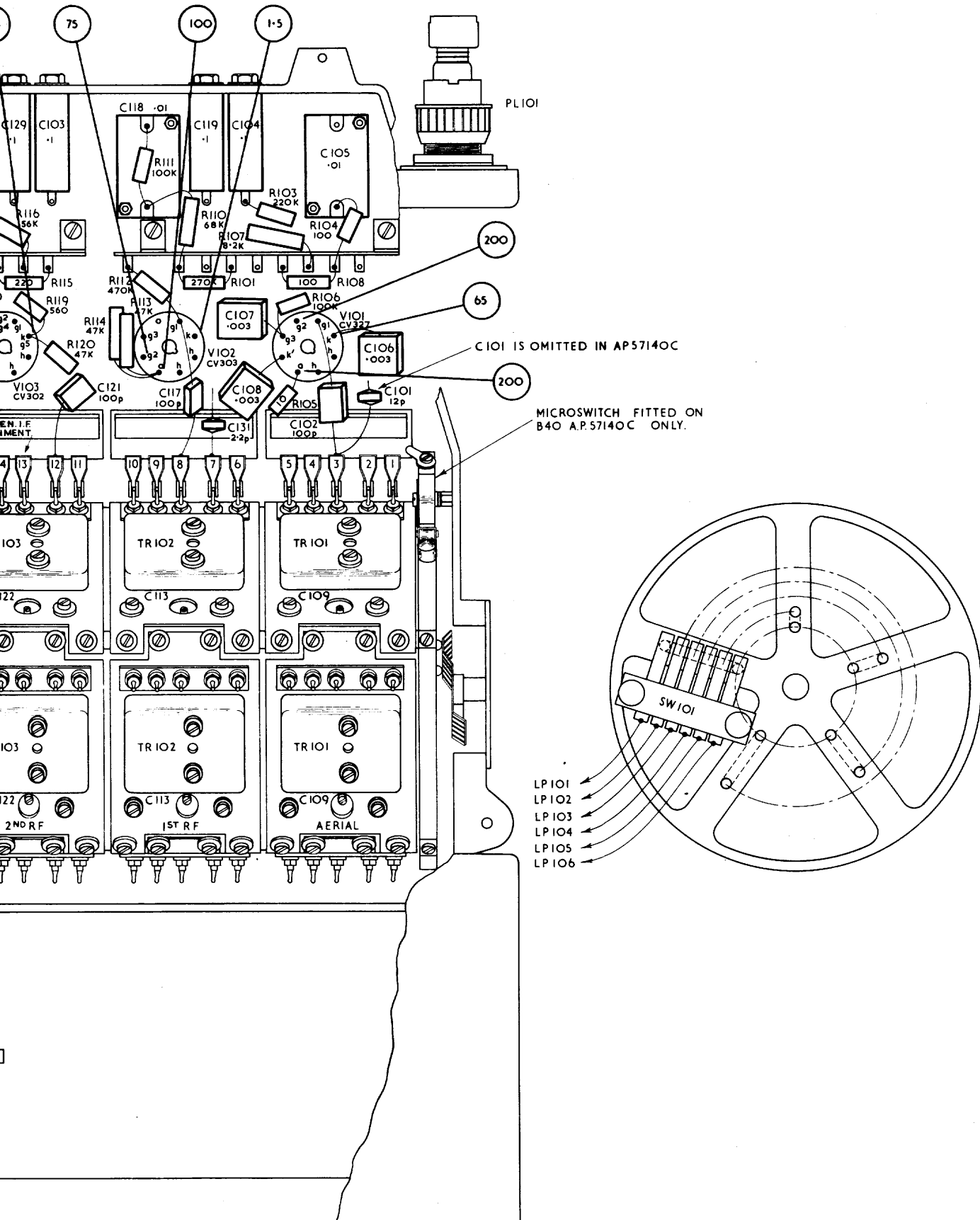
RECEIVER B40 A.P.57140/A/B/C R.F. UNIT. RIGHT HAND LAYOUT.
