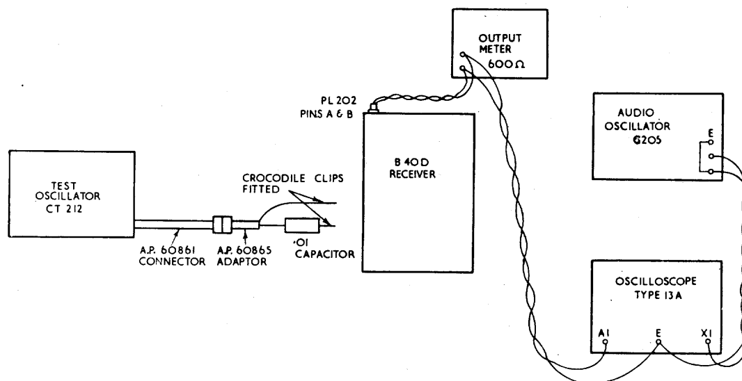
B.F.O. ALIGNMENT (B 4OD) TEST EQUIPMENT CONNECTION DIAGRAM
