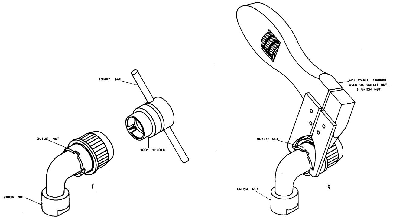
ASSEMBLY DETAILS OF MK. 4 SOCKET
