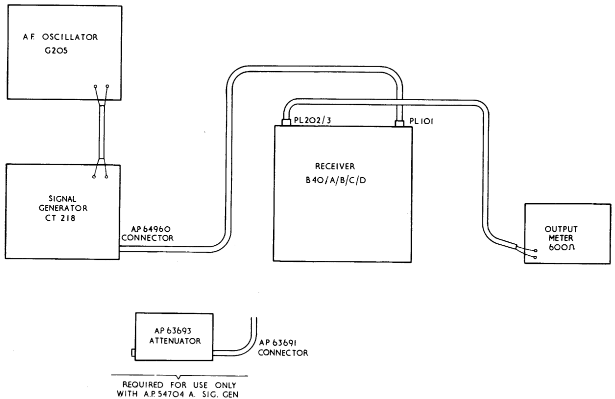
TEST EQUIPMENT CONNECTION DIAGRAM FIG 4
