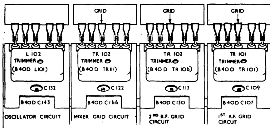
DETAILS OF R.F. COIL ASSEMBLY
