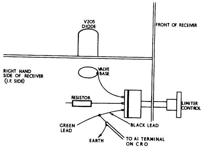
CONNECTION TO RECEIVER FROM CRO FIG. 14(b)
