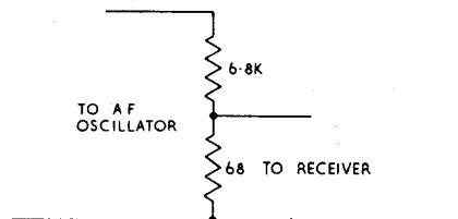
100/1 VOLTAGE DIVIDER
