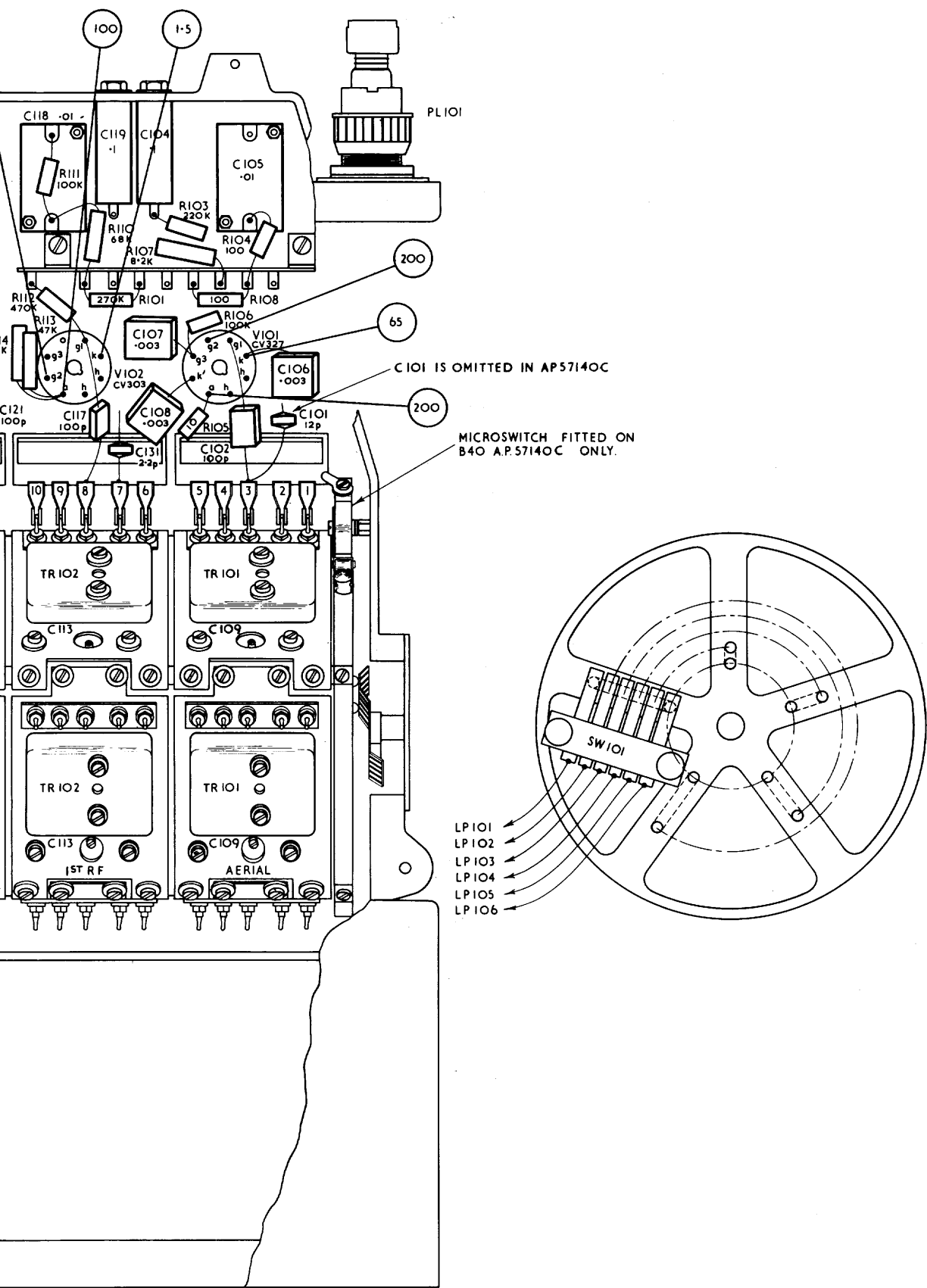
RECEIVER B40 A.P.57140/A/B/C R.F. UNIT. RIGHT HAND LAYOUT.
