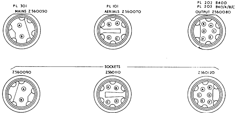
FIG.1 RECEIVER B40 AP 57140/A/B/C MK 4 PLUGS & SOCKETS PIN IDENTIFICATIONS
