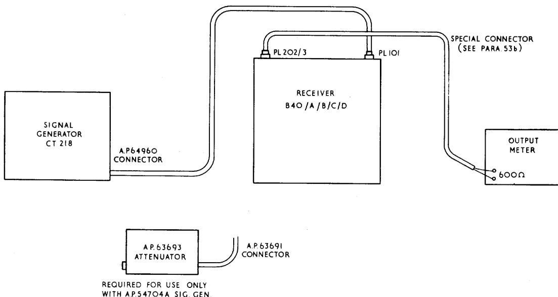
TEST EQUIPMENT CONNECTION DIAGRAM
