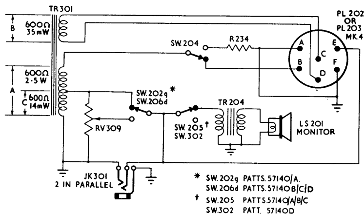
OUTPUT LINES
