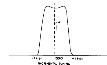
RESPONSE - CRYSTAL FILTER FIG. 7
