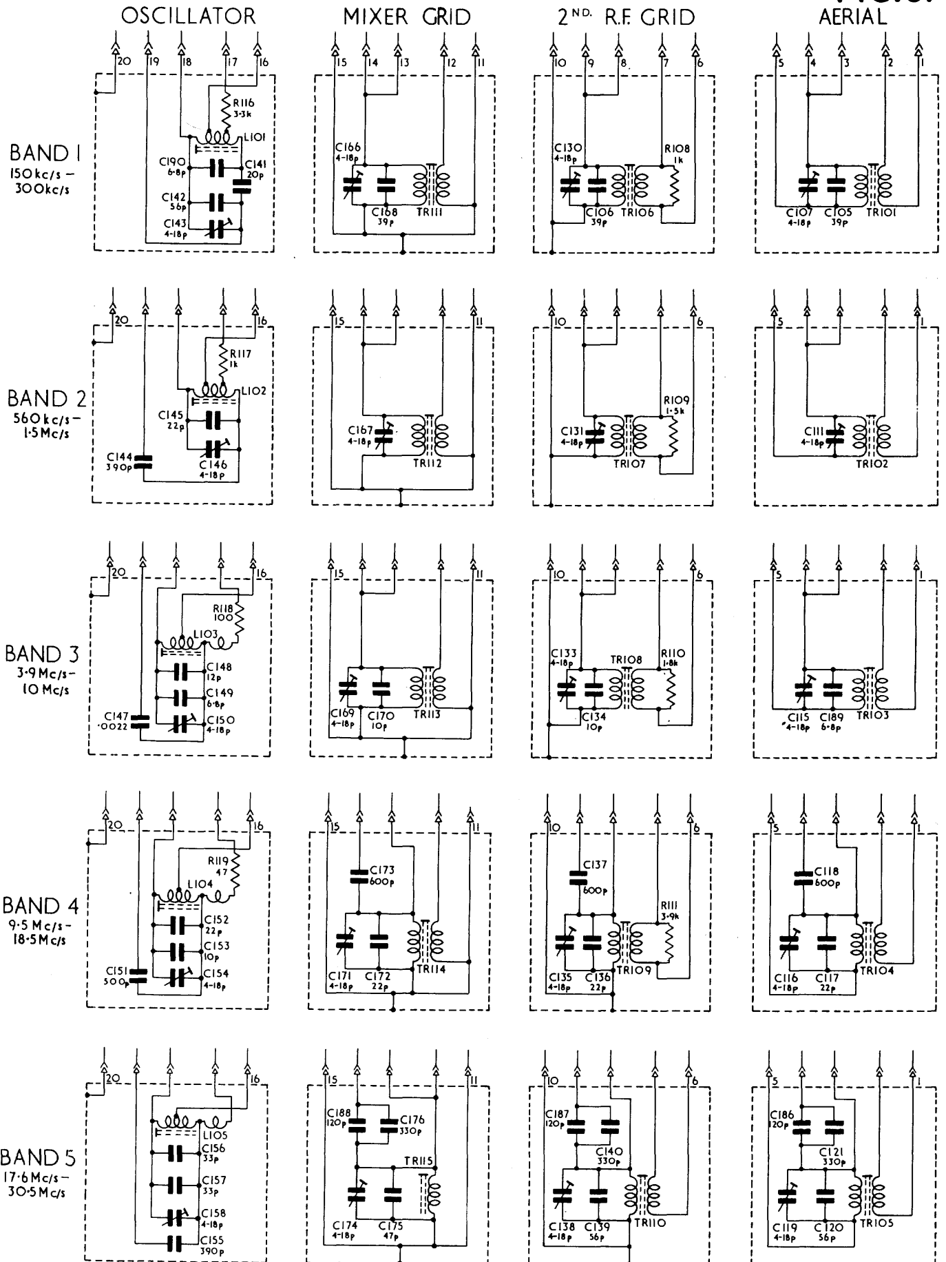
RECEIVER 62B AP. 67757 A. TURRET SWITCH COMPONENTS. CIRCUIT DIAGRAM
