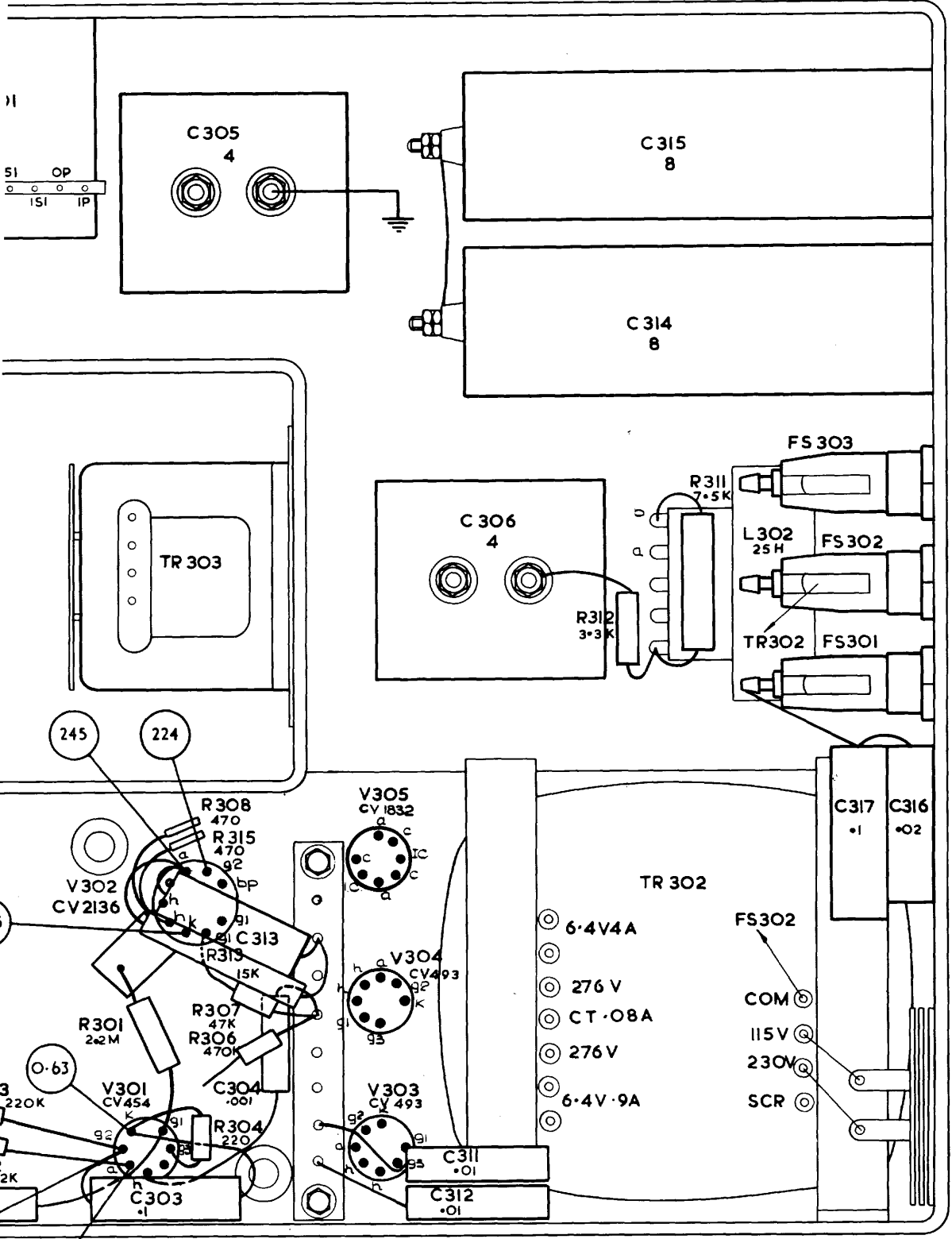
RECEIVER B40 A.P. 57140 D. A.F. & POWER UNIT. BOTTOM LAYOUT.
