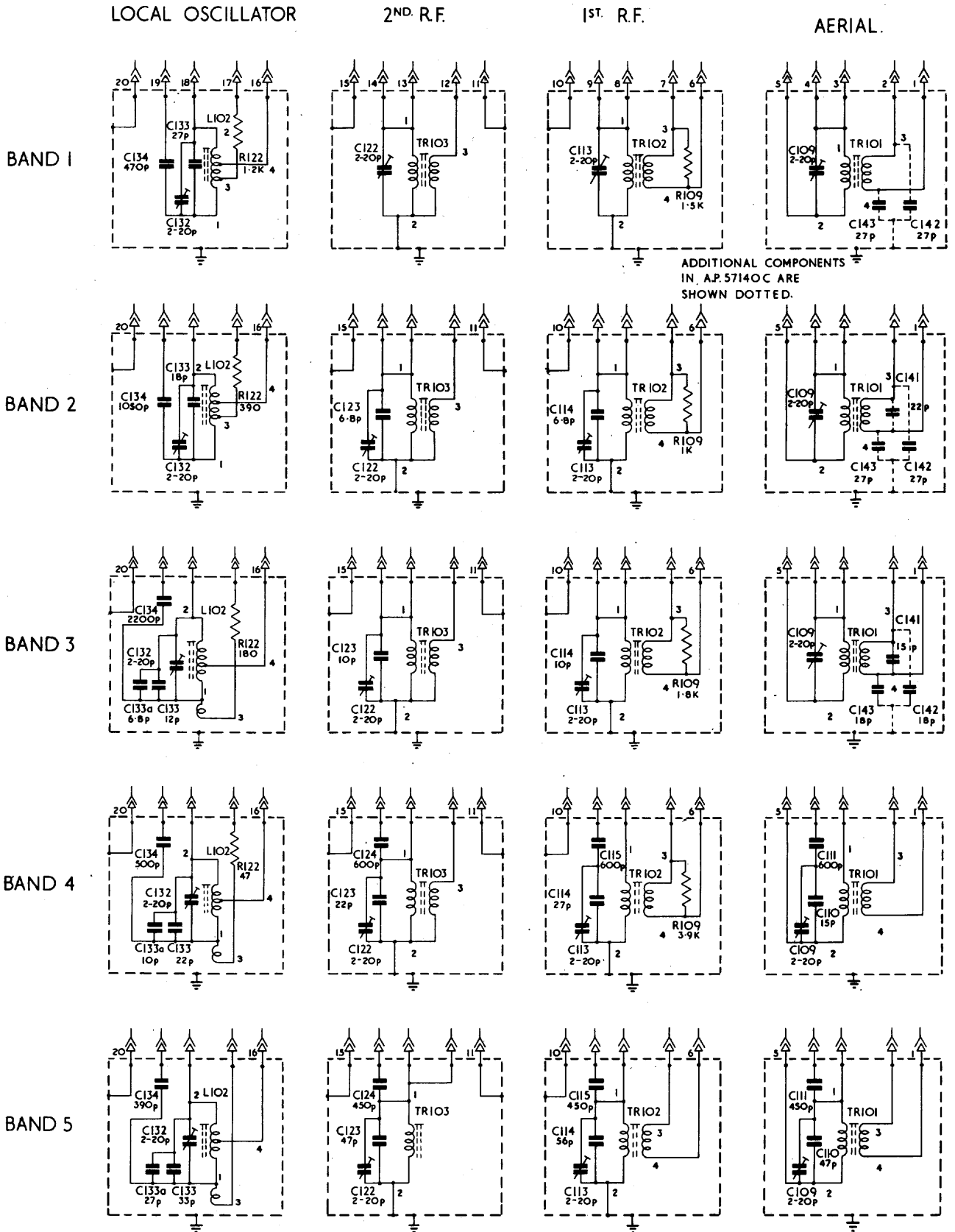
RECEIVER B 40. A.P. 57140/A/B/C. TURRET SWITCH COMPONENTS. CIRCUIT DIAGRAM.
