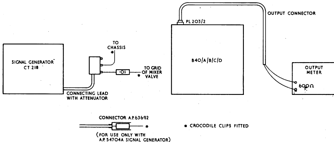
FIG. 16 TEST EQUIPMENT CONNECTION DIAGRAM
