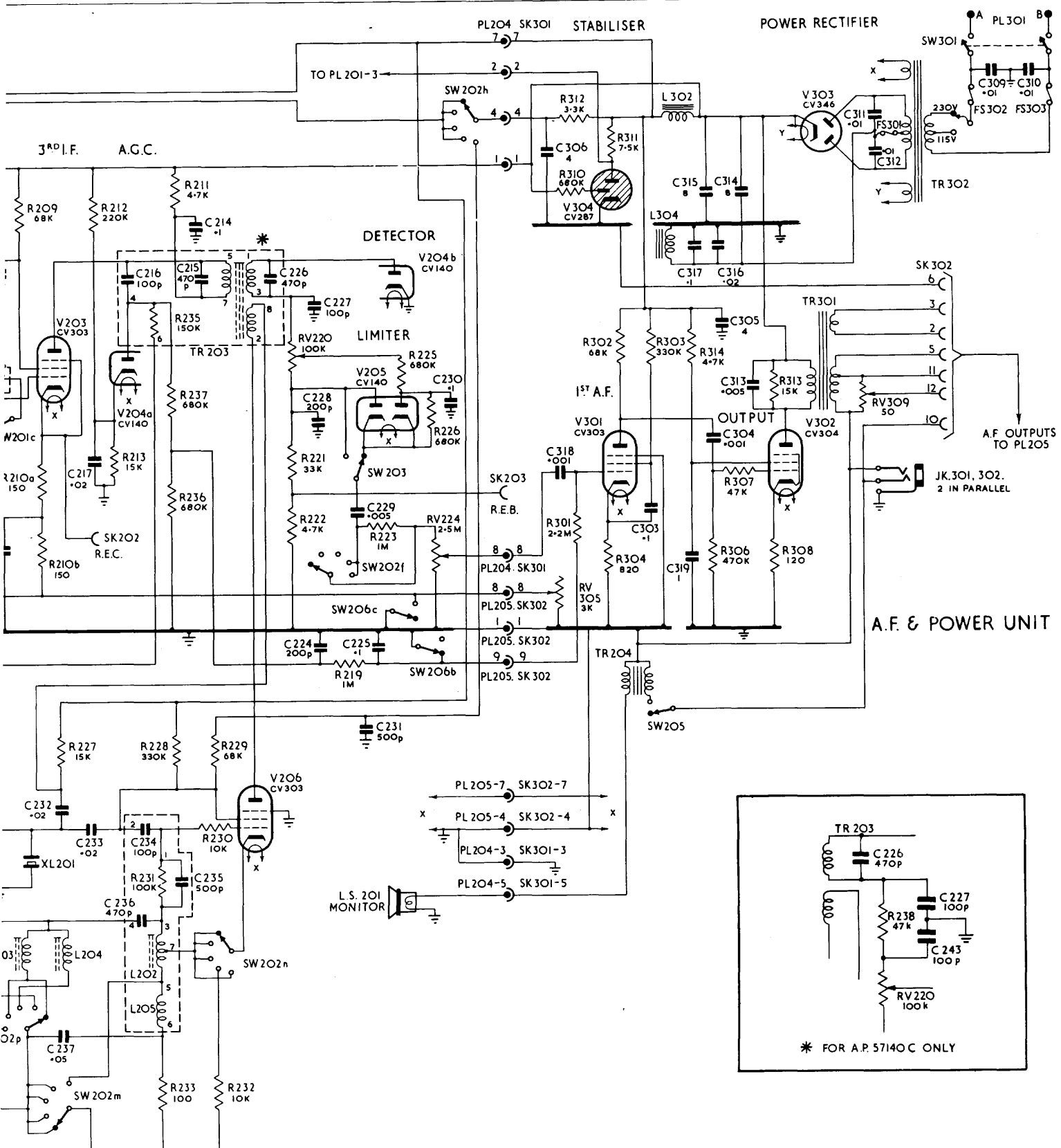
RECEIVER B40. A.P. 57140B/C. CIRCUIT DIAGRAM.
