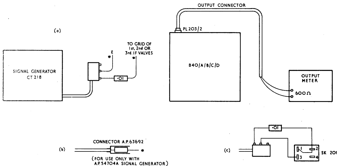
FIG. 17 TEST EQUIPMENT CONNECTION DIAGRAM
