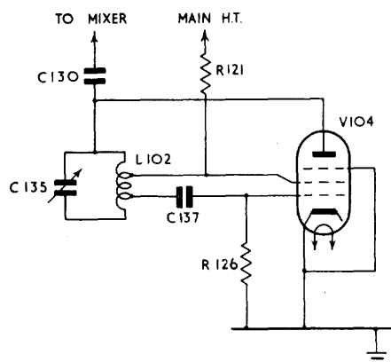
SIMPLIFIED VARIABLE FREQUENCY OSCILLATOR CIRCUIT FIG. 1
