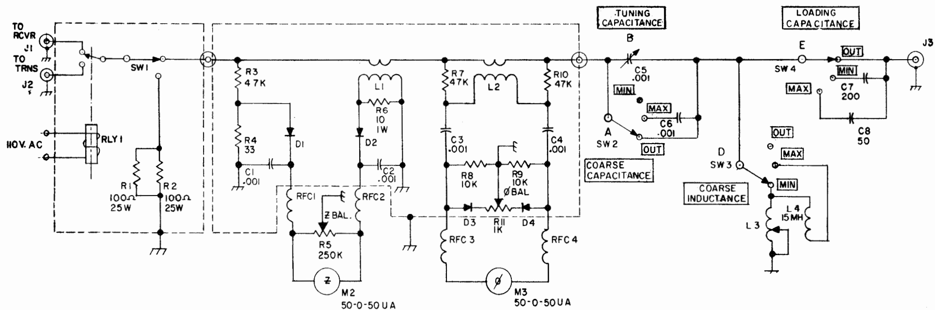
M-100 CIRCUIT DIAGRAM
