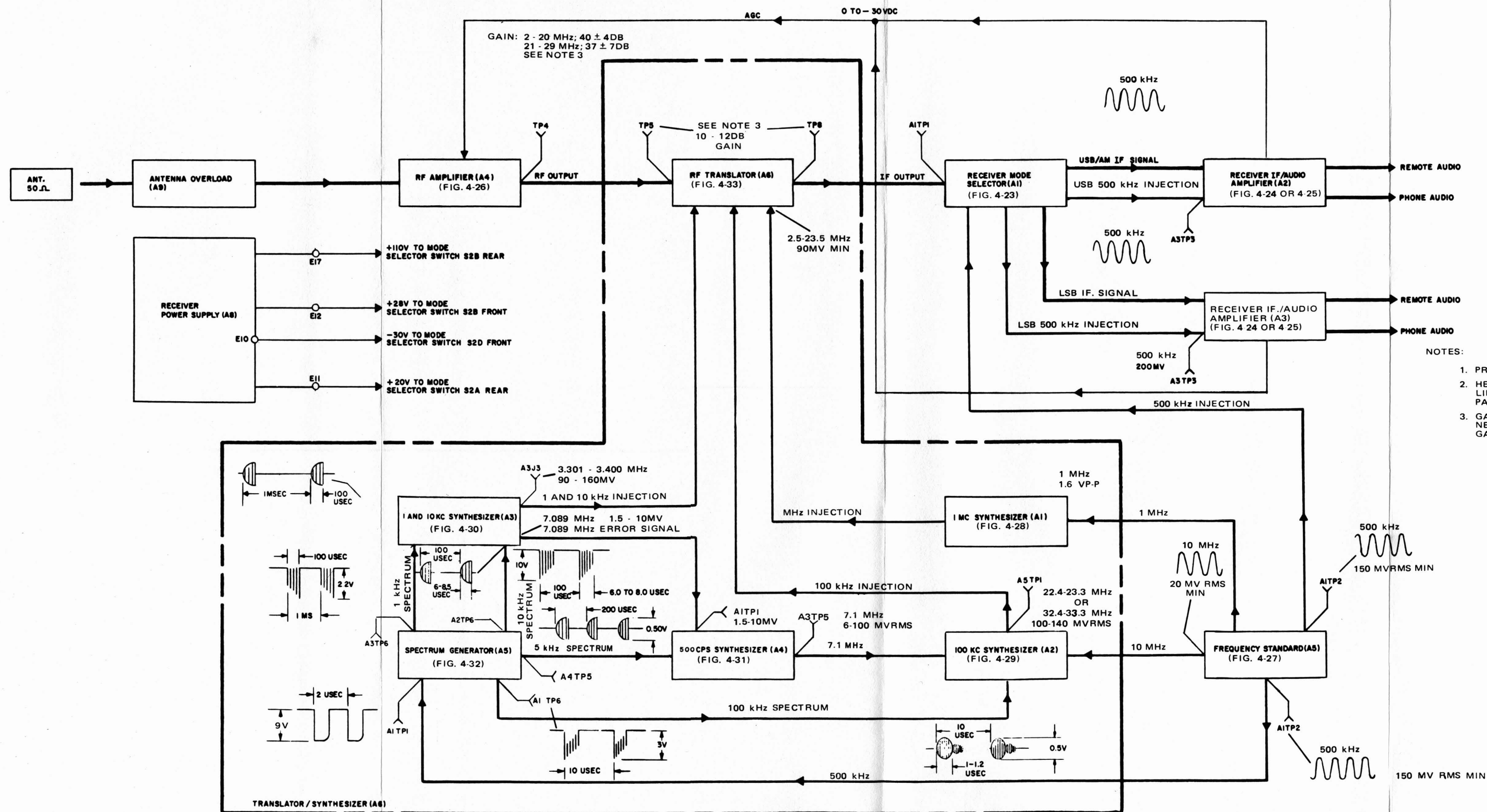
Figure 4-22. Radio Receiver R-1051/URR, Overall Servicing Diagram
