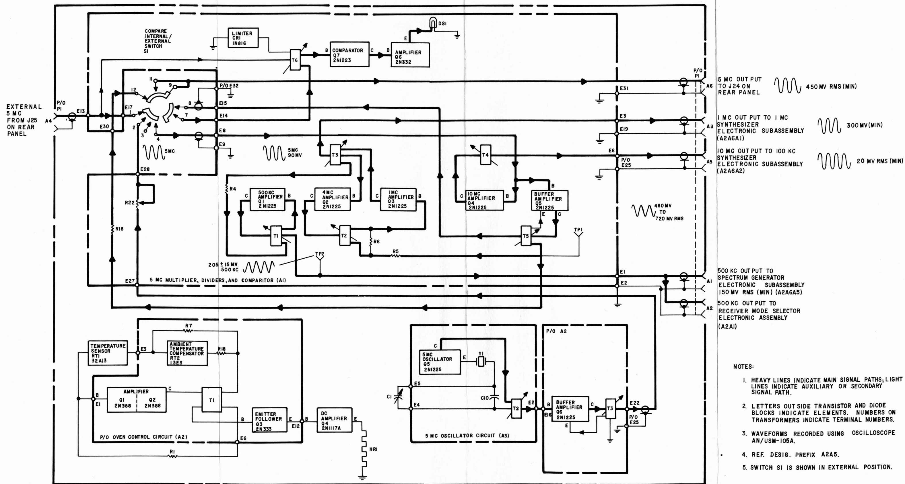
Figure 4-27. Frequency Standard Assembly A2A5, Servicing Block Diagram
