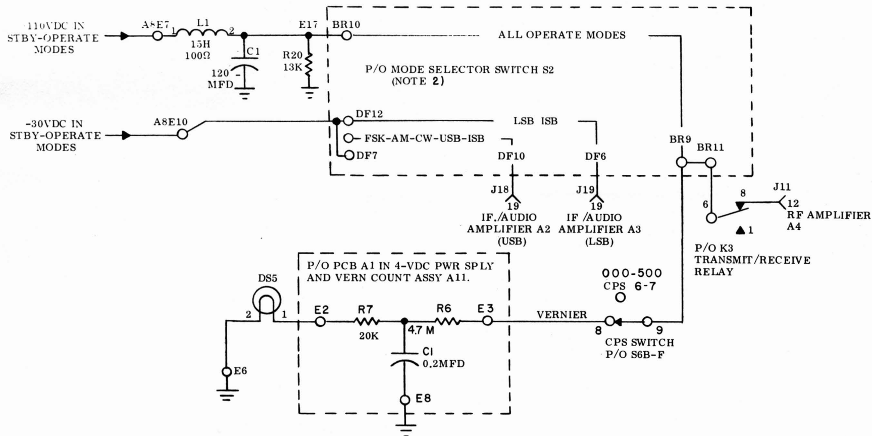
Figure 4-11. 30- and 110-VDC Distribution Diagram
