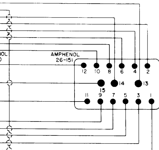
CABLE NO.3
