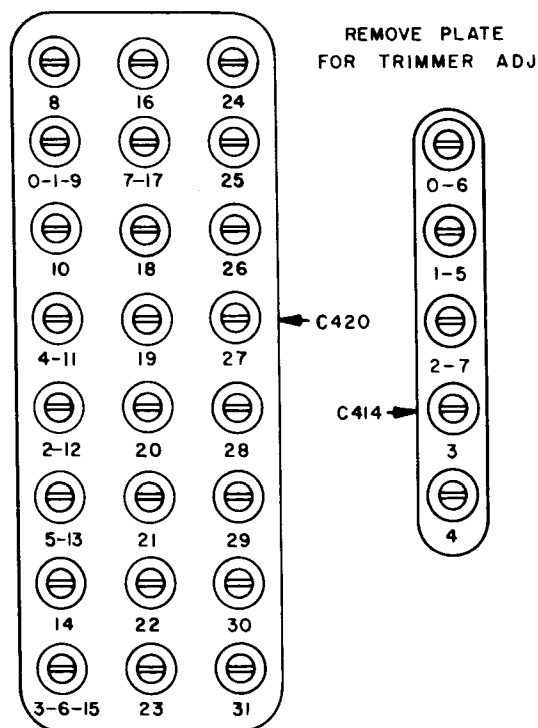
Figure 105. Crystal-oscillator trimmers.
