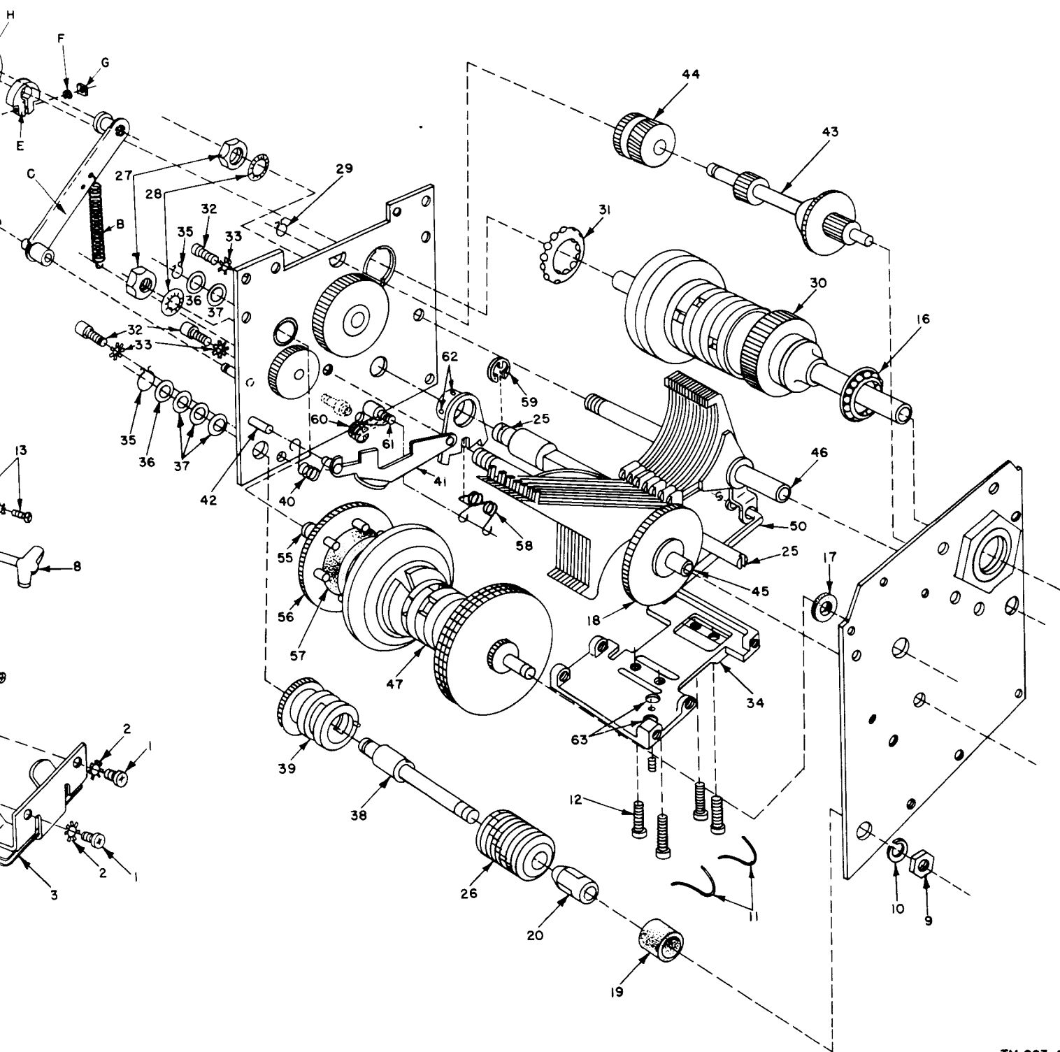
Autotune multiturn positioning head.
