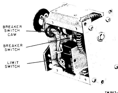
Figure 61. Autotune system, control head, right dust cover removed.
