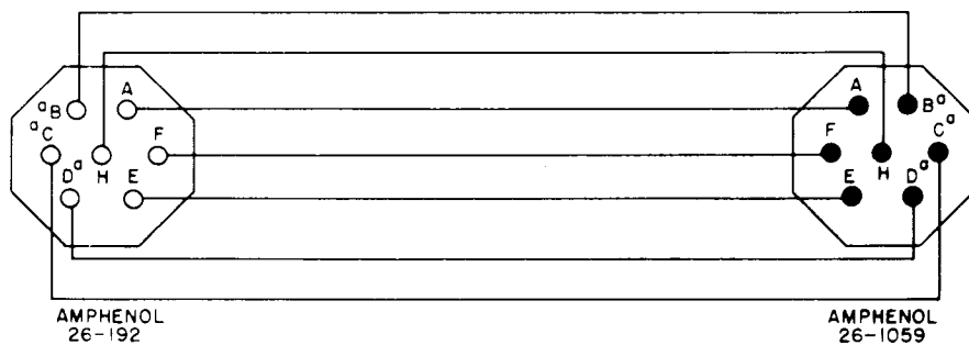
CABLE NO.6
