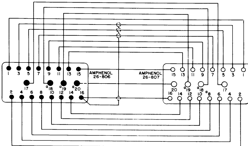
CABLE NO.8
