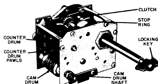
Figure 63. Autotune system, multiturn positioning head, rear view.
