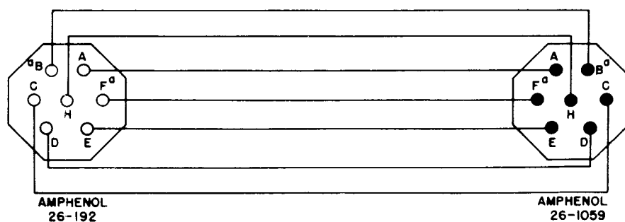
CABLE NO.2
