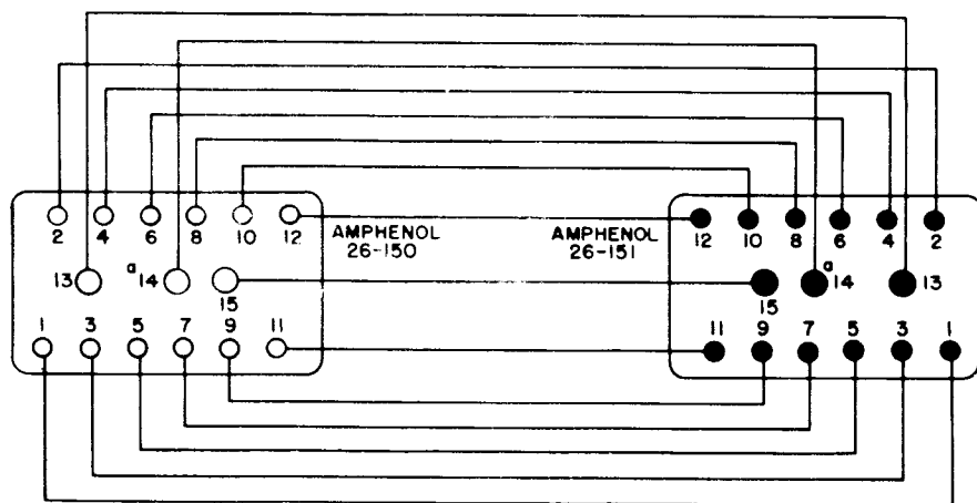
CABLE NO.5
