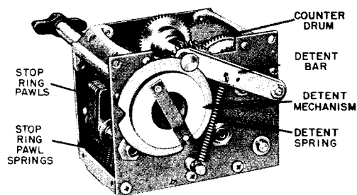
Figure 62. Autotune system, multiturn positioning head, front view.
