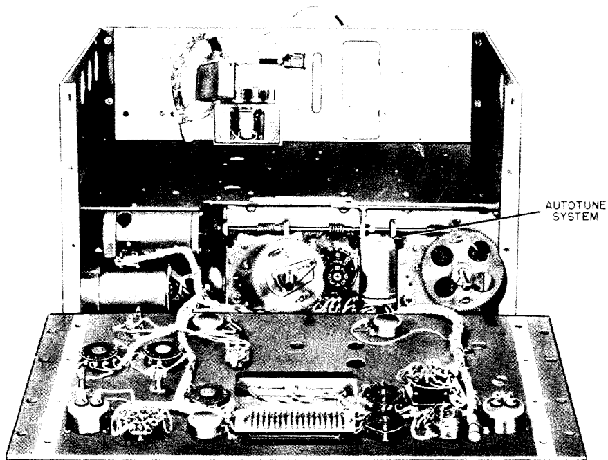
Figure 8. Radio Receiver R-391/URR, front panel and main frame.
