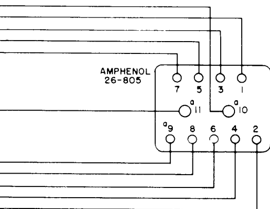
CABLE NO.4
