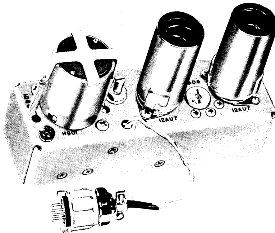
Figure 14. Calibration-oscillator subchassis.
