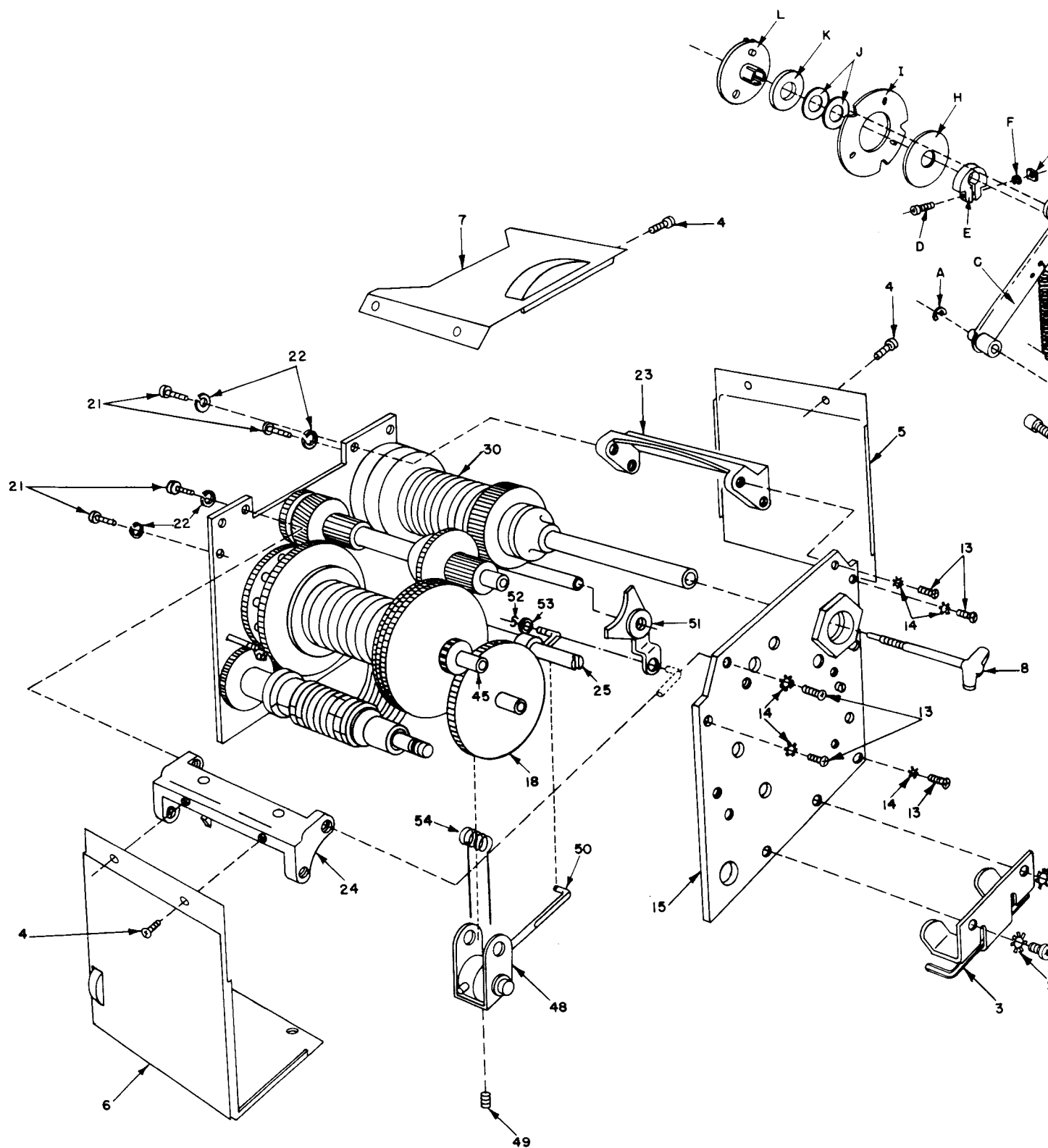
Figure 109. Disassembly of Autotune mu
