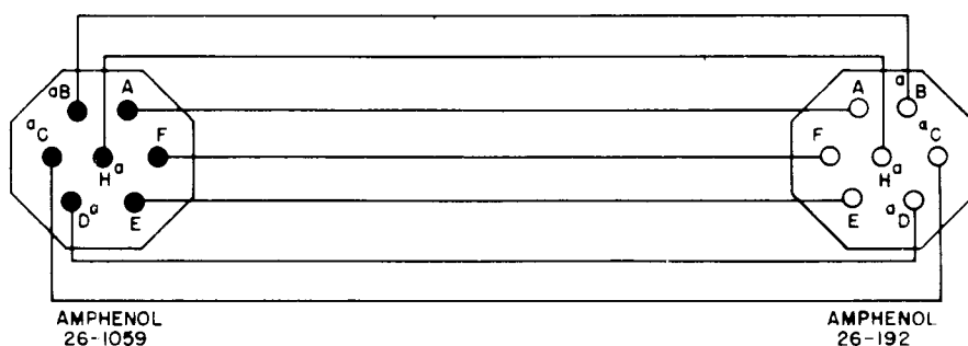
CABLE NO.7
