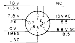
1ST MIXER V203 6C4
