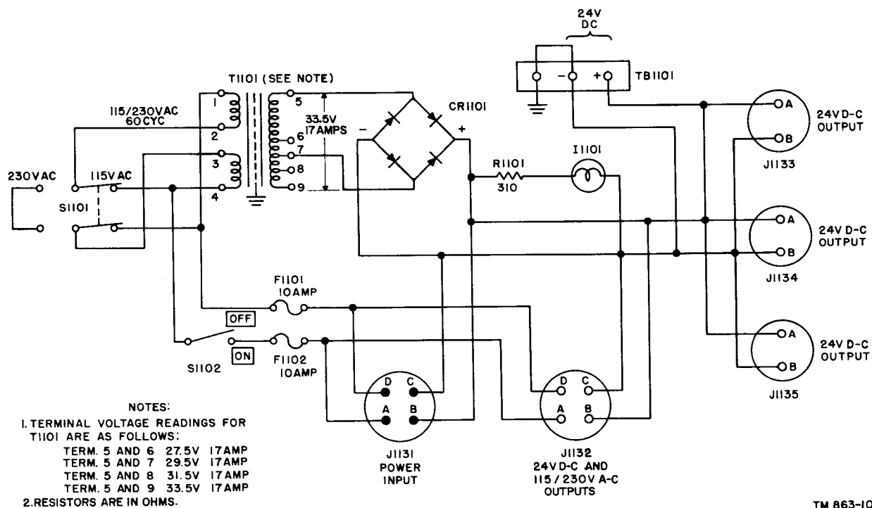
Figure 117. Power Supply PP-629/URR, schematic diagram.
