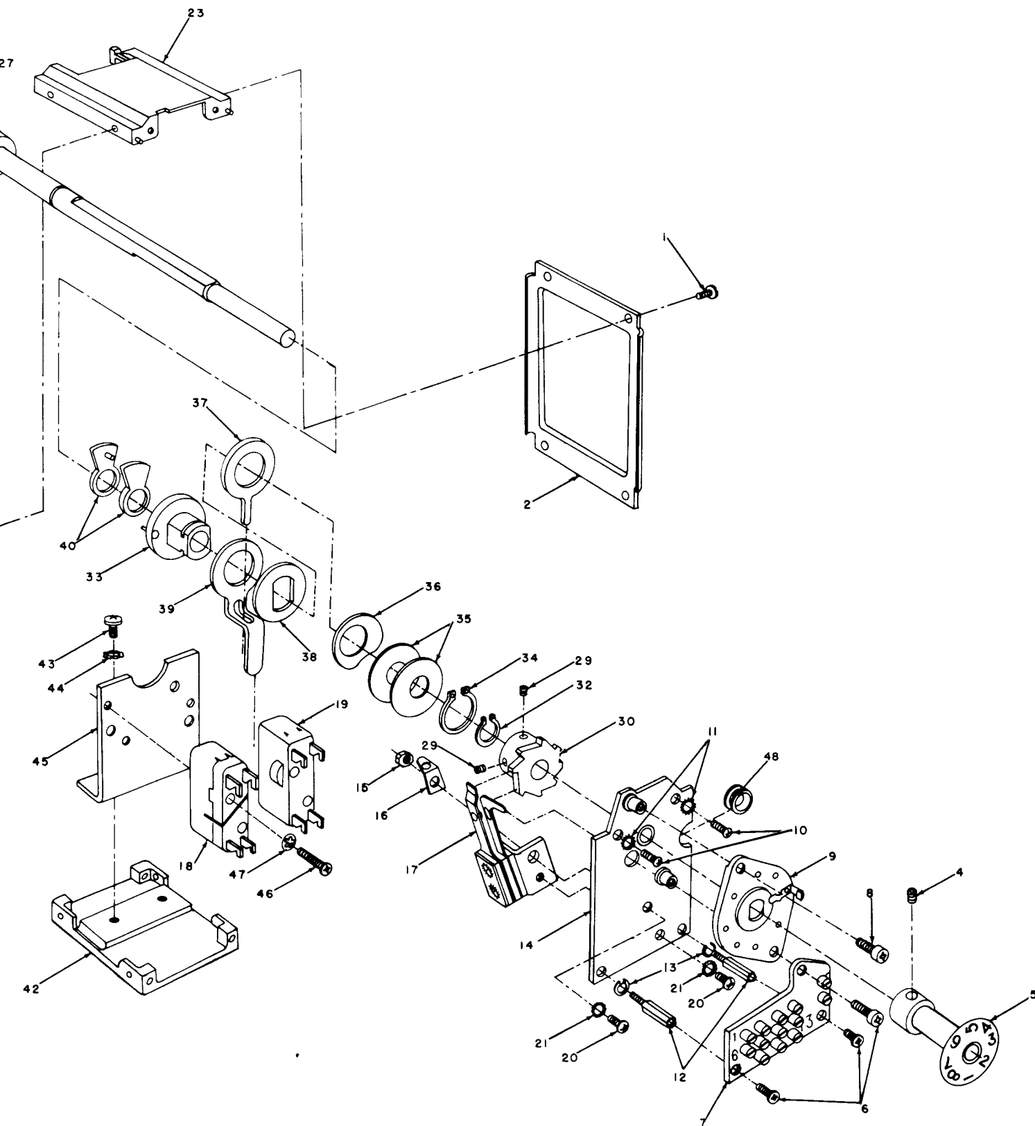
Figure 110. Dissassembly of Autotune control head.
