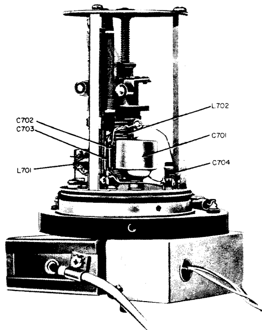
Figure 78. Vfo subchassis, bottom view.
