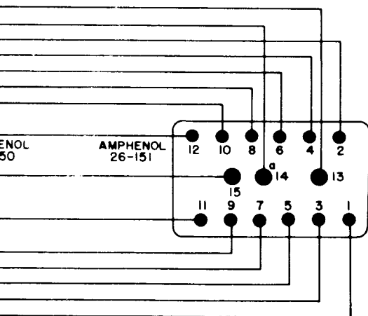
CABLE NO.5
