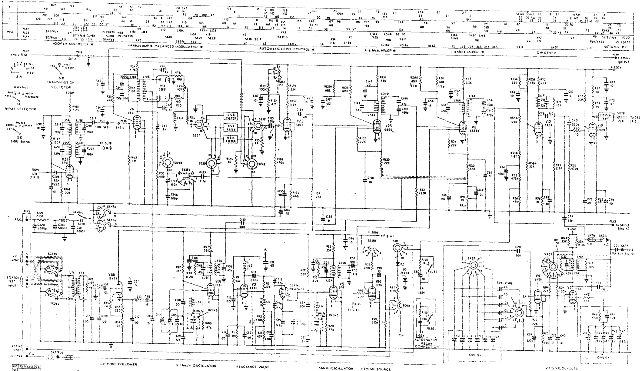
MA.79C CIRCUIT DIAGRAM-1-MODULATION AND I.F. STAGES
