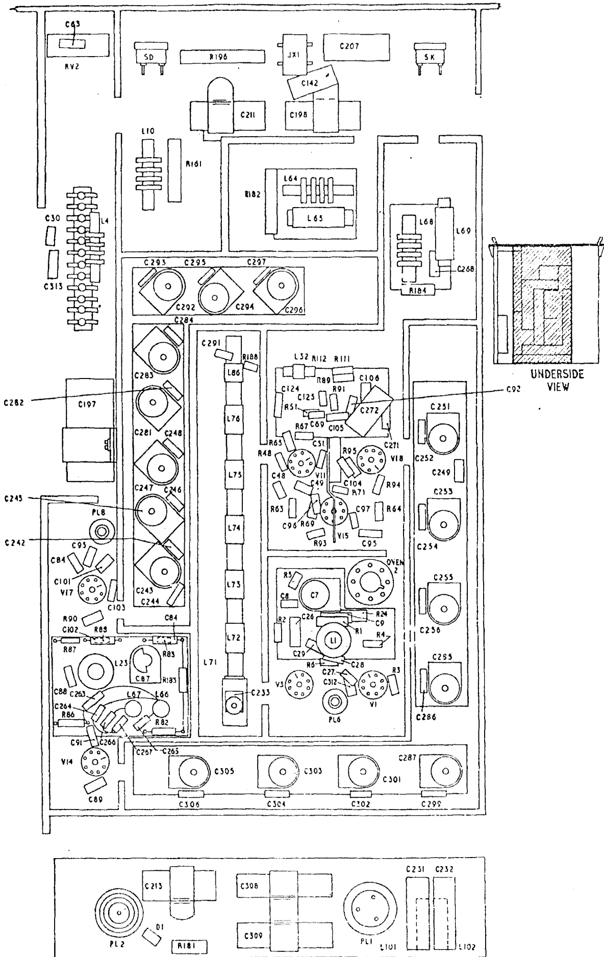
MA.79G MAIN CHASSIS COMPONENT LAYOUT-I
