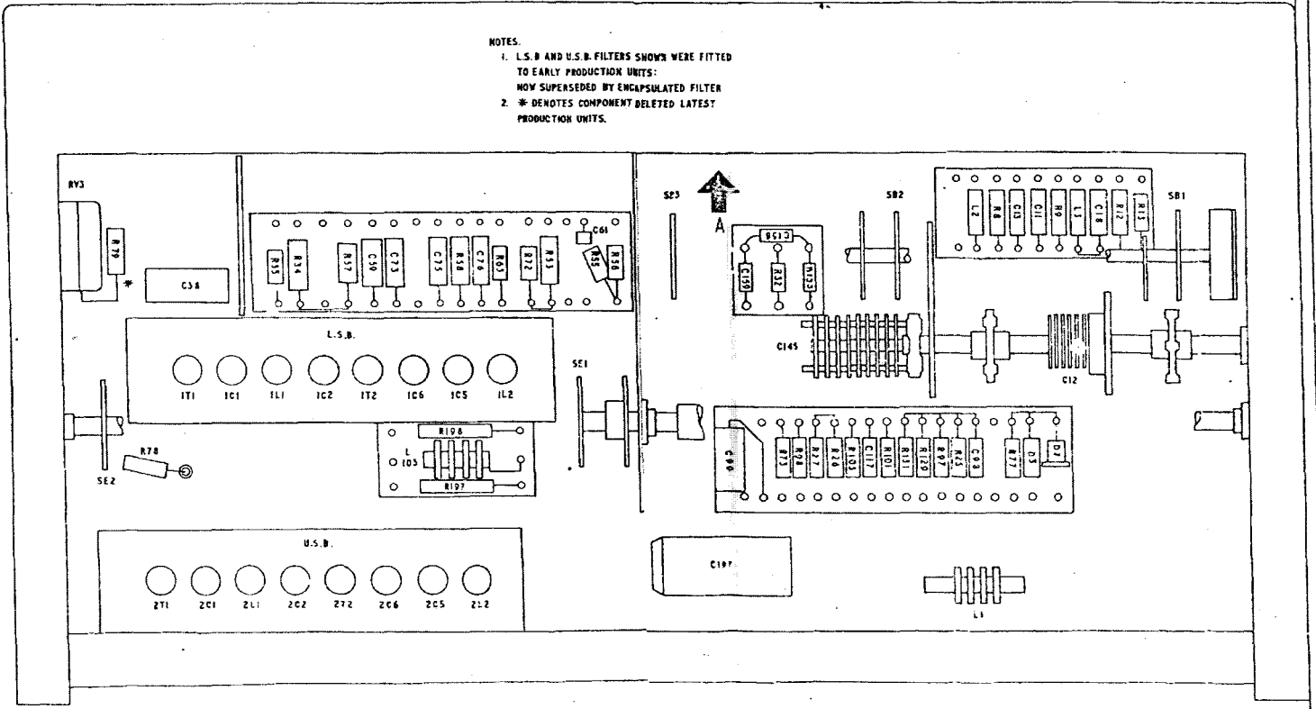
MA.79G MODULATION CHASSIS COMPONENT LAYOUT
