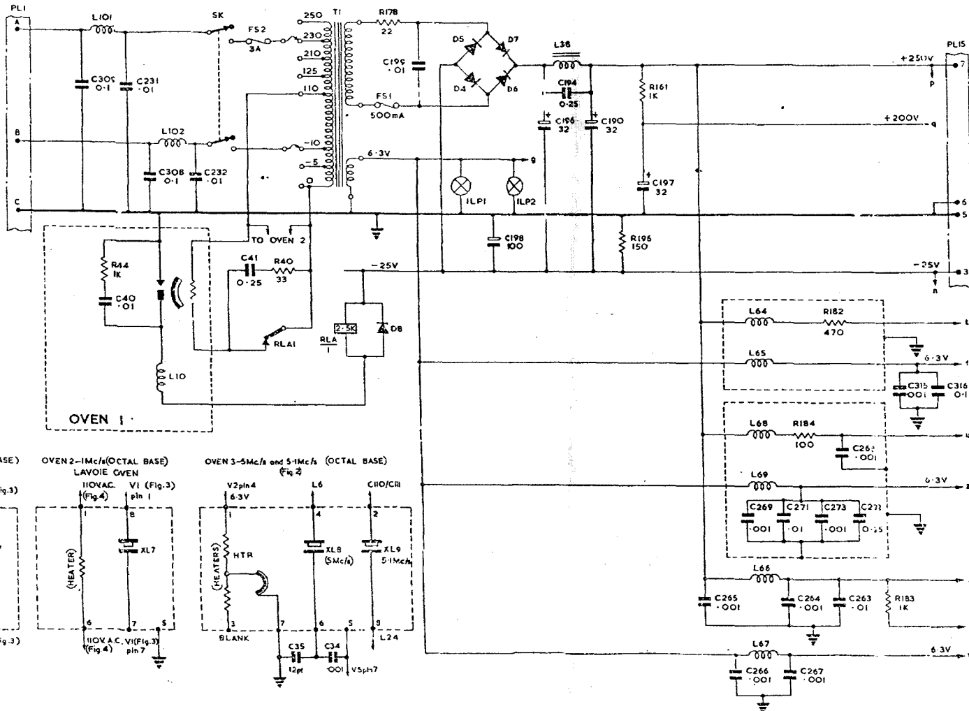
MA.79 - ANCILLARY CIRCUITS.
