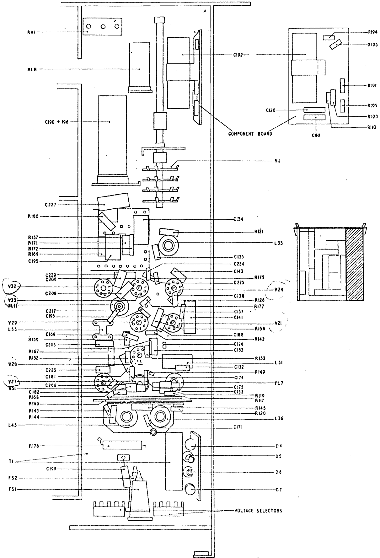
MA79G MAIN CHASSIS COMPONENT LAYOUT-2
