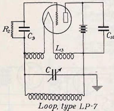
FIGURE 8.—Simplified transmitter circuit.
