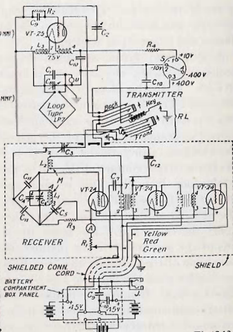
FIGURE 6.—Circuit diagram, SCR-131 (161).
