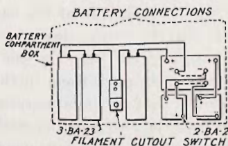
FIGURE 6.—Circuit diagram, SCR-131 (161).
