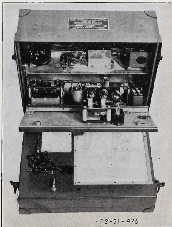
FIGURE 3.—Radio receiver and transmitter BC-148 (151), showing interior of apparatus box.
