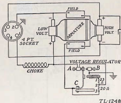
FIGURE 11.—Wiring diagram GN-35.
