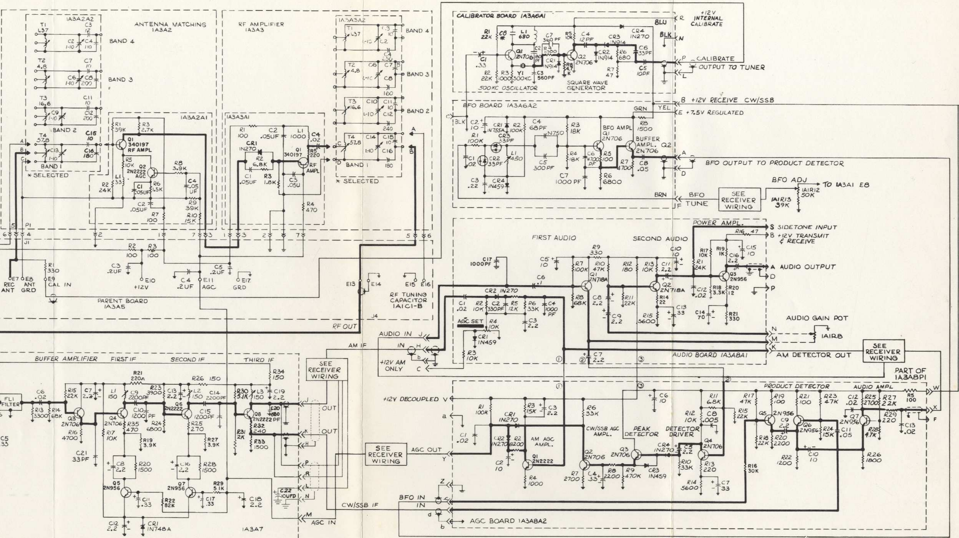
Figure 3-2. RR-224 Schematic Diagram
