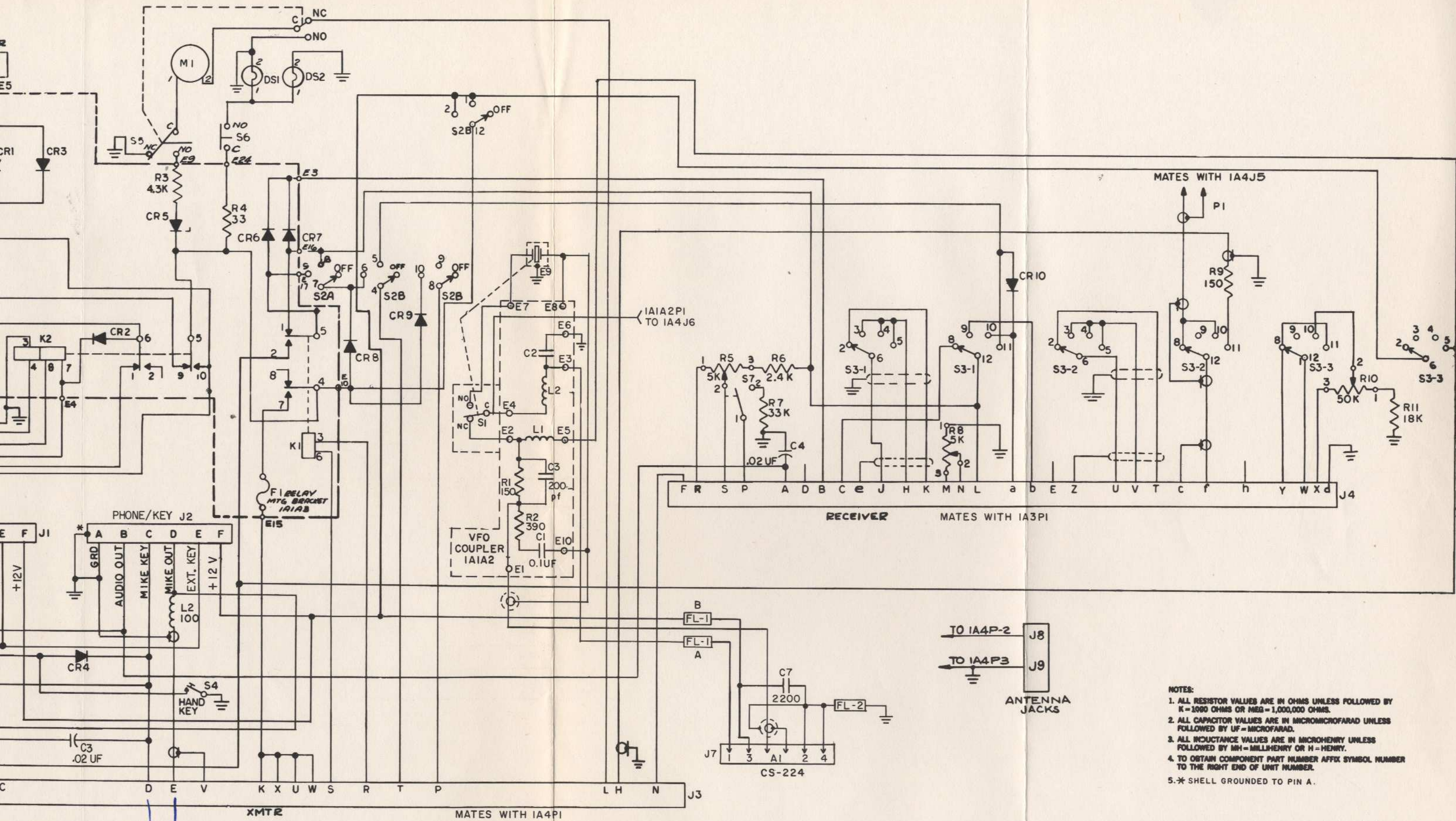
Figure 3-3. TAR-224 Front Panel Schematic Diagram
