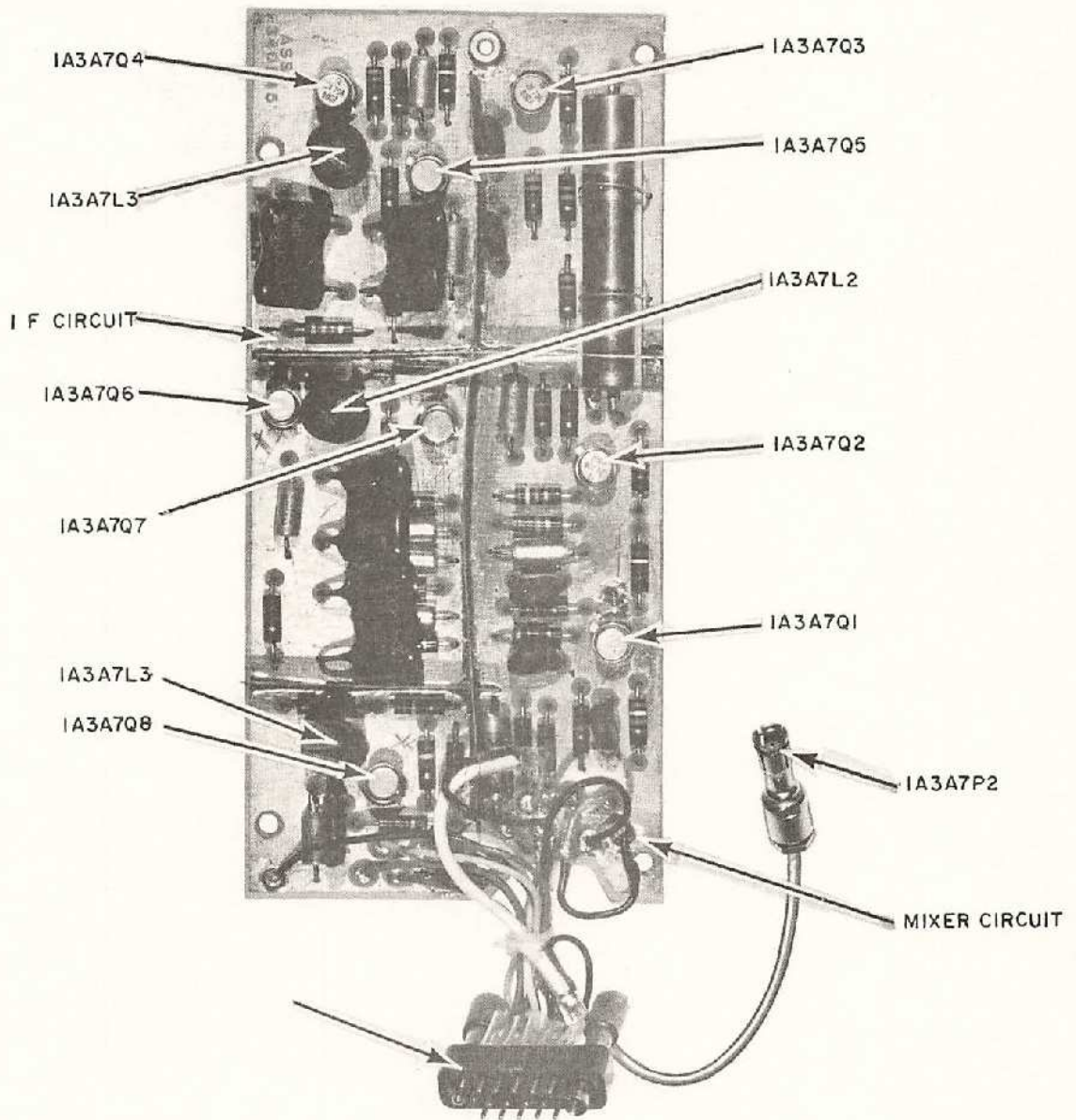
IF AND MIXER ASSEMBLY IA3A7
