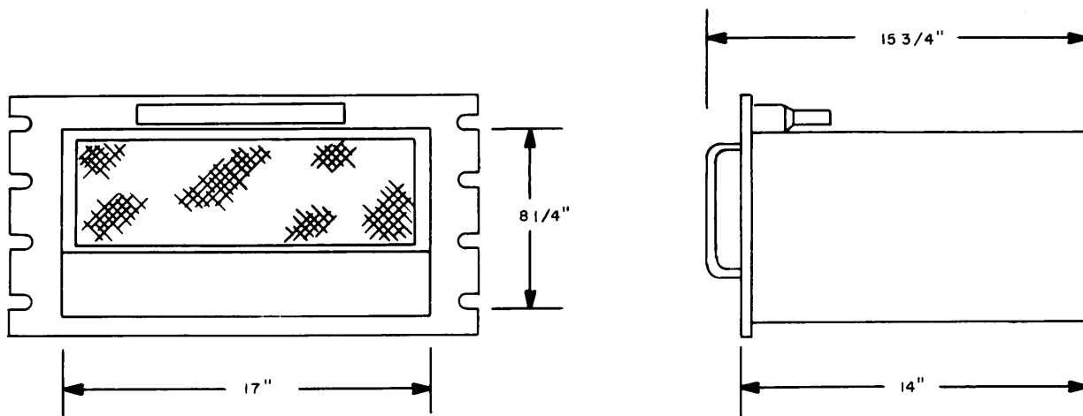
Figure 2-2. Outline Dimensional Drawing, Model GPR-90RXD
