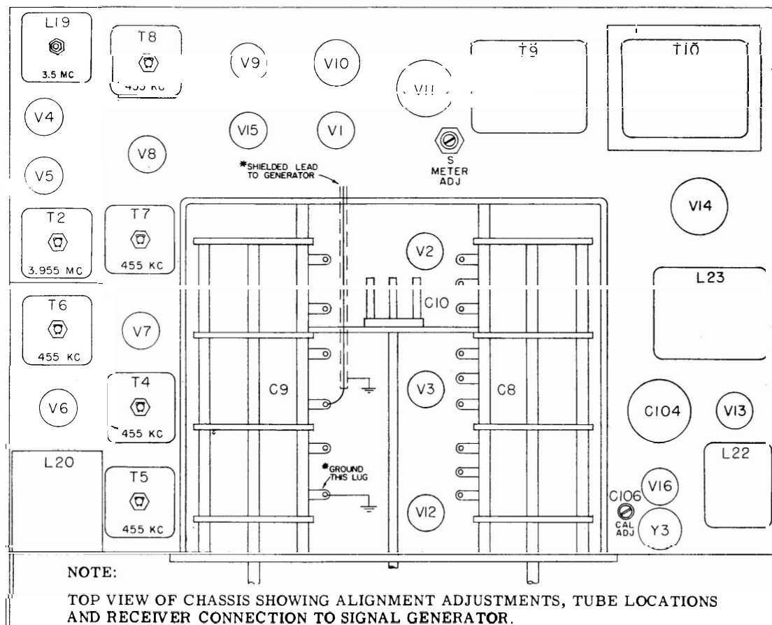
Figure 4-1. Top View of Chassis
