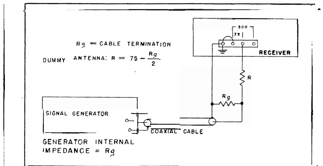
Figure 4-3. Signal Generator Connections for RF Alignment
