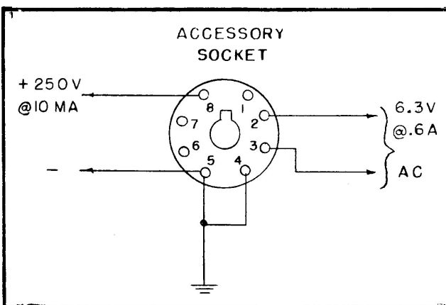
Figure 2-5. Accessory Power Socket Connections
