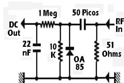
Fig.5 Dummy Load Schematic
