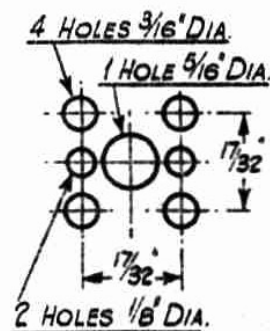
CHASSIS PIERCING
