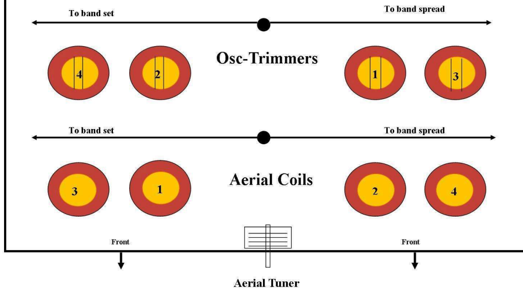
Codar CR-66 coil ass Top View
