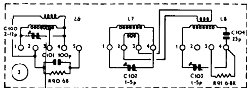
CCL TURRET WIRING (RINGED NUMBER INDICATES RANGE)
