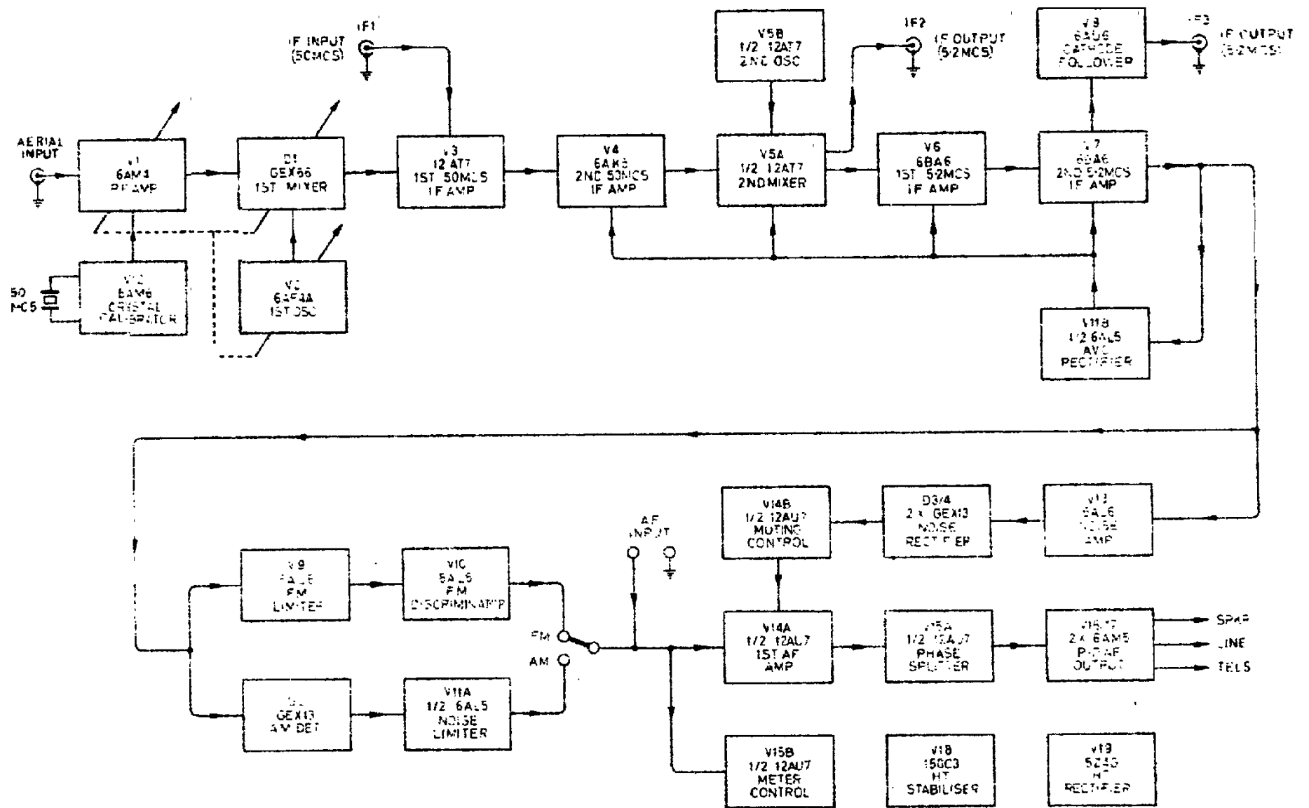
Fig. 1. Block Schematic Diagram of 770U (L3, II) Receiver.
