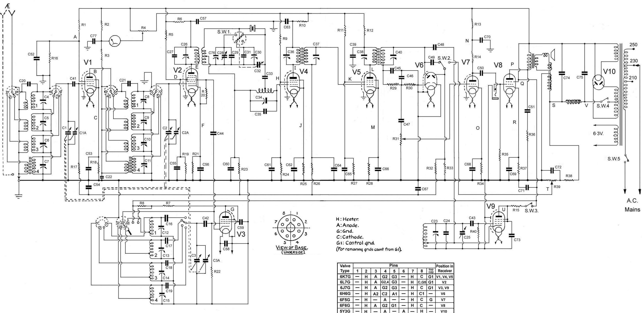
Valve Pin Connections
