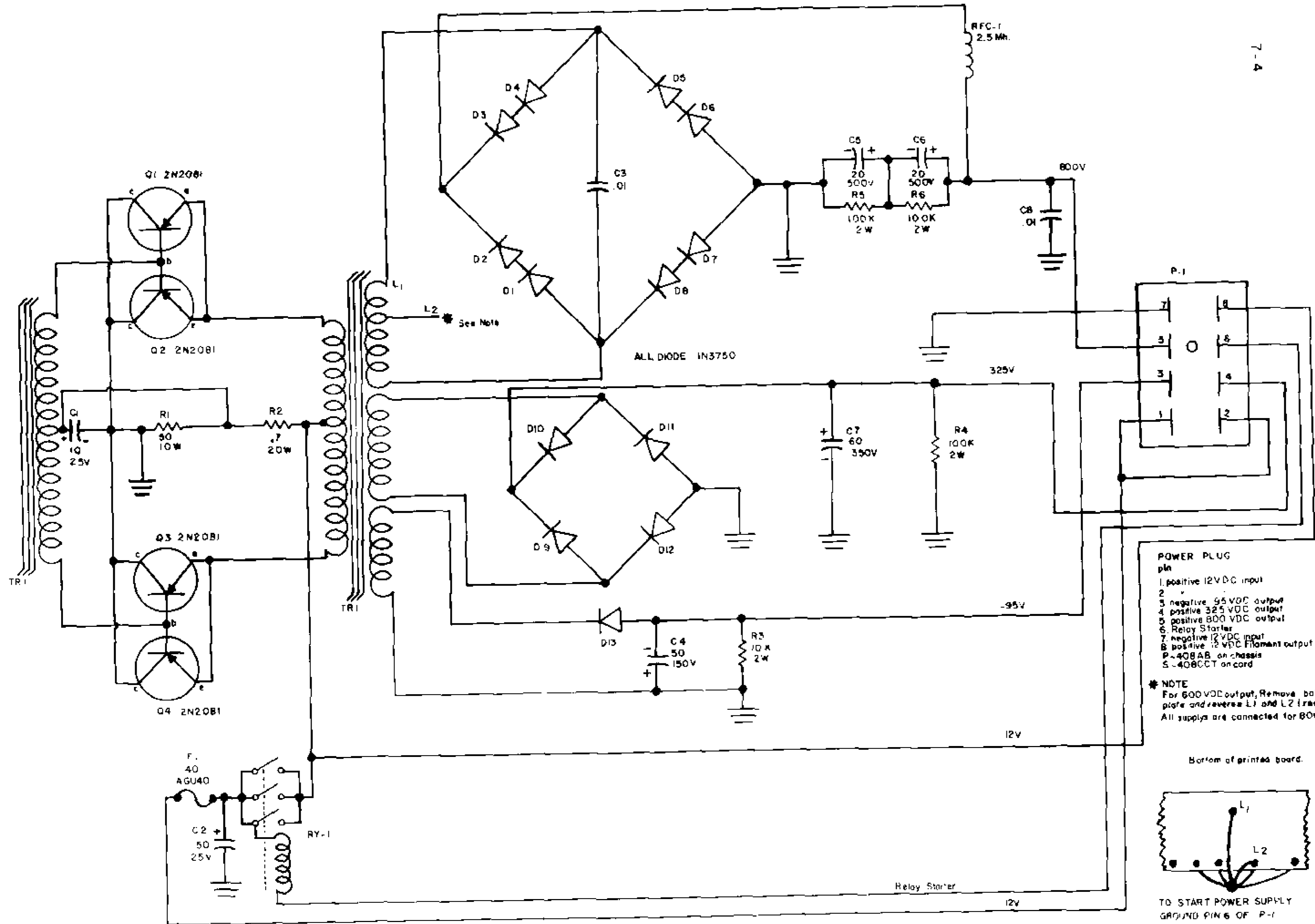
FIGURE-P G-300DC SCHEMATIC
