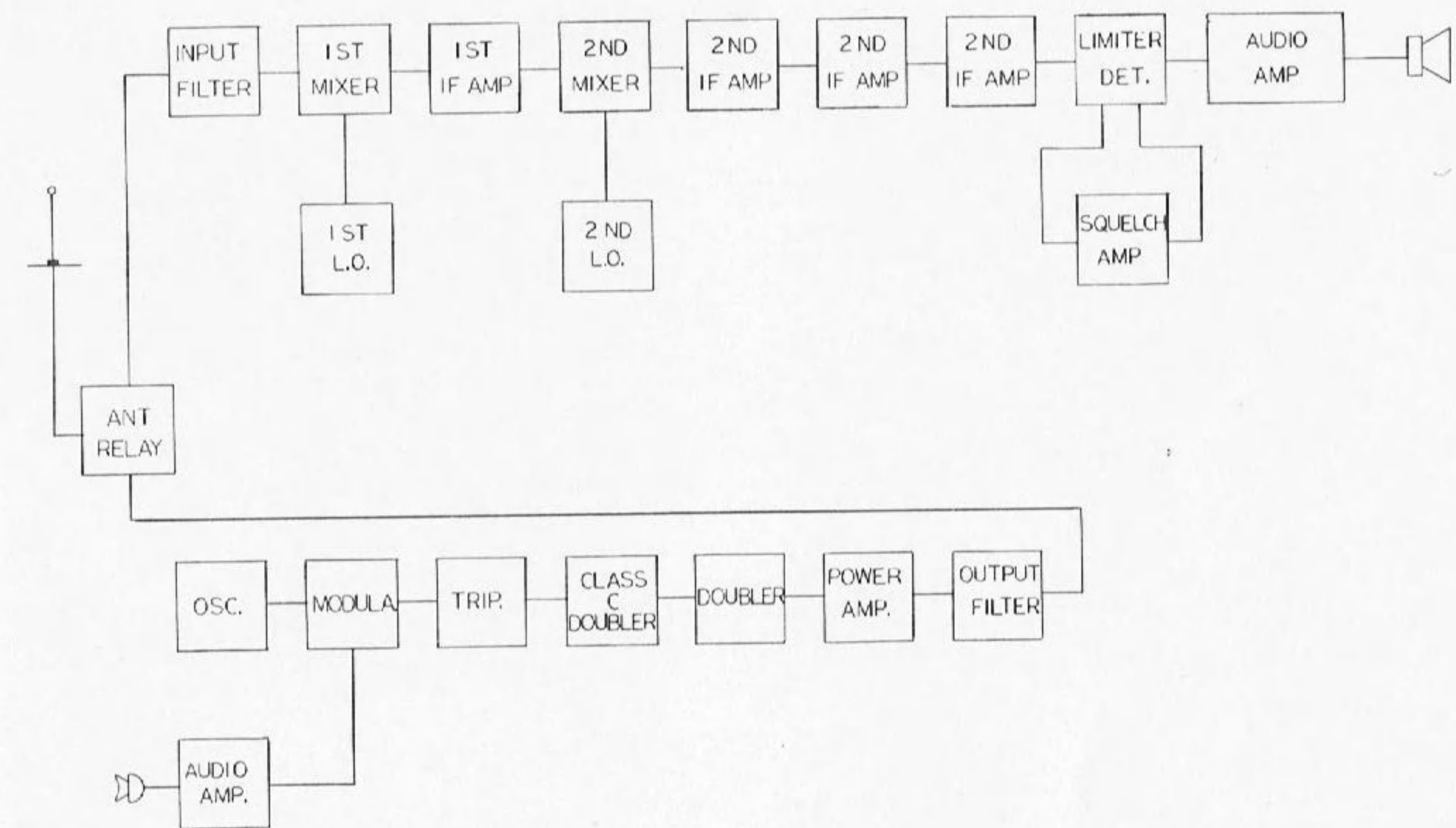
Block Diagram
