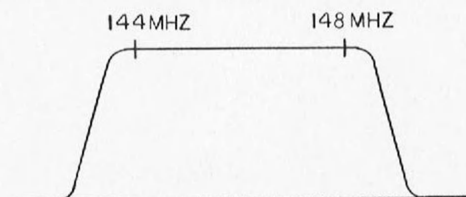
Swept Input Filter Figure 1
