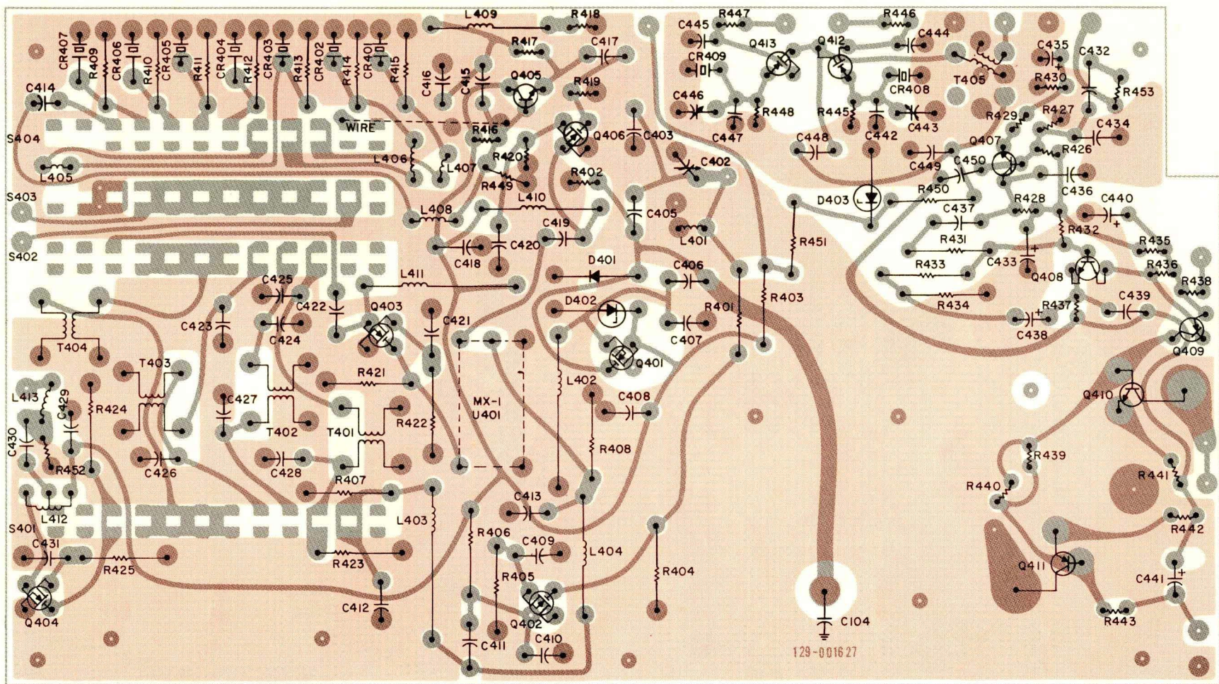
Figure 7-7. Component Layout, VFO/Pre-Mixer/Audio Amplifier Module.
