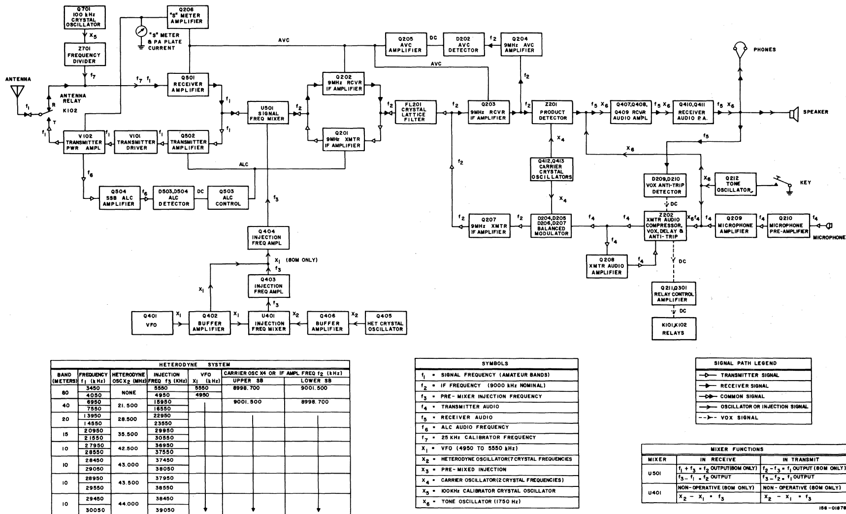
Figure 6-1. Block Diagram of Model FPM-300 MK II Transceiver.
