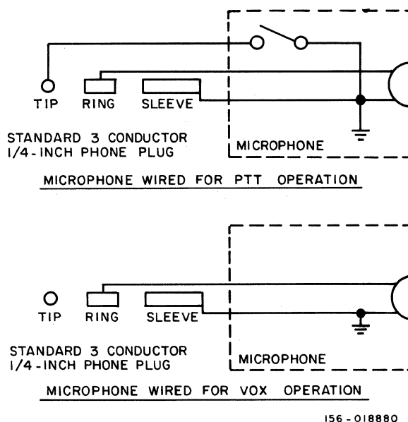
Figure 3-2. Microphone Wiring for Push-to-Talk and VOX Transmitter Control.
