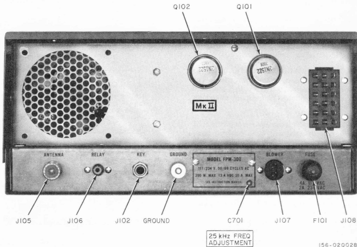
Figure 3-1. Rear View of Model FPM-300 MK II Transceiver.
