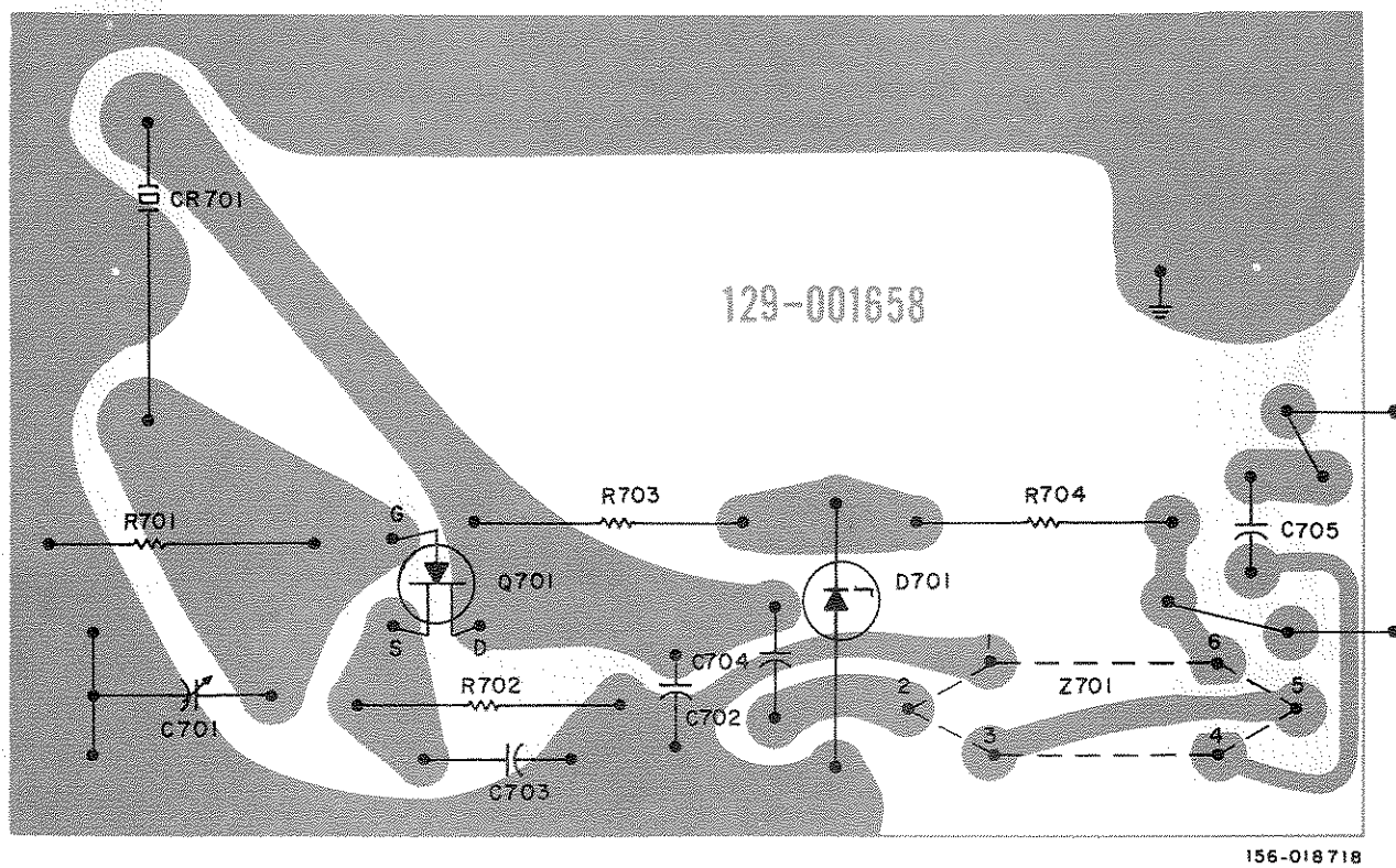
Figure 7-10. Component Layout, 25 kHz Calibrator Module.
