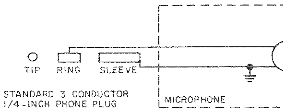
MICROPHONE WIRED FOR VOX OPERATION
