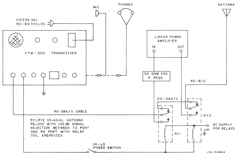
Figure 3-3. Base Station Installation with Linear Amplifier.
