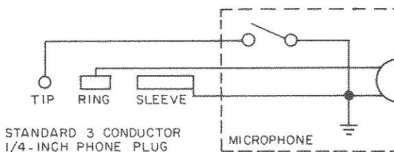
MICROPHONE WIRED FOR PTT OPERATION
