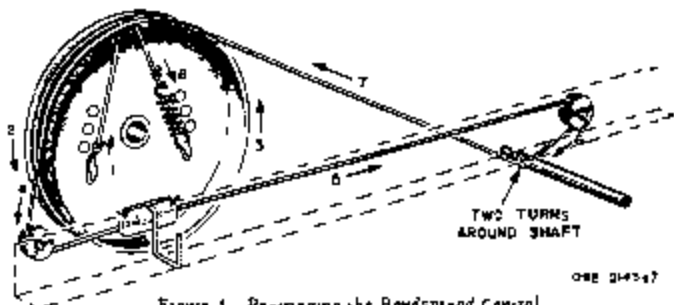
Figure 4. Restringing the Bandspread Control
