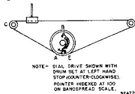
Figure 2. Dial cable stringing procedure, band spread
