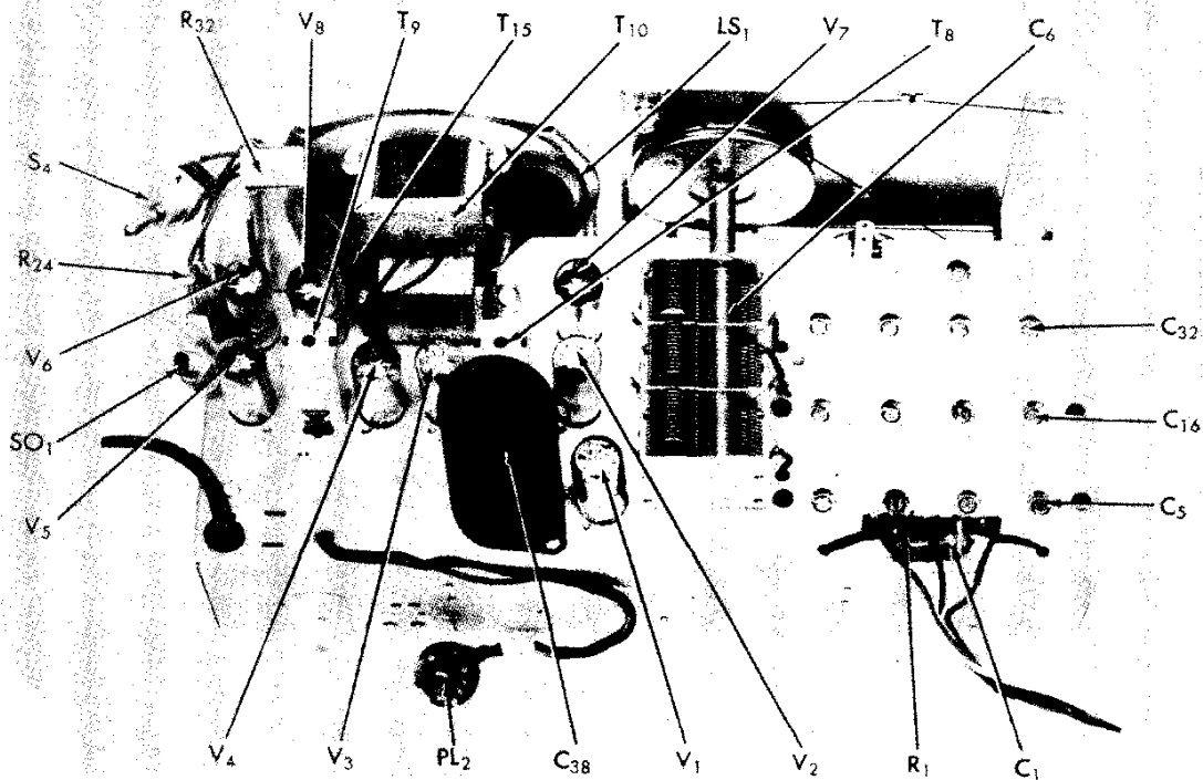
Figure 5. Top view, component location
