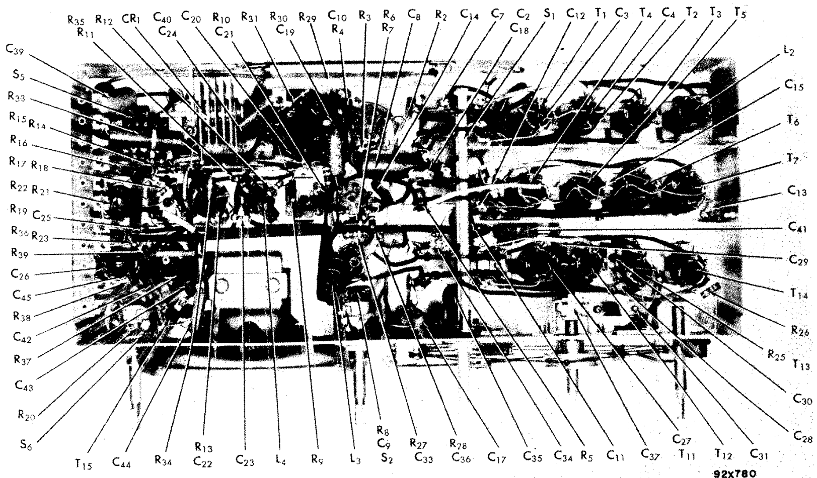
Figure 6. Bottom view, component location
