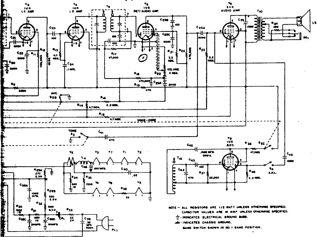
Fig. 8. Schematic diagram
