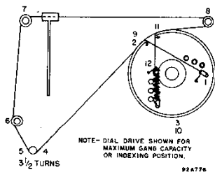
Figure 1. Dial cable stringing procedure, general coverage
