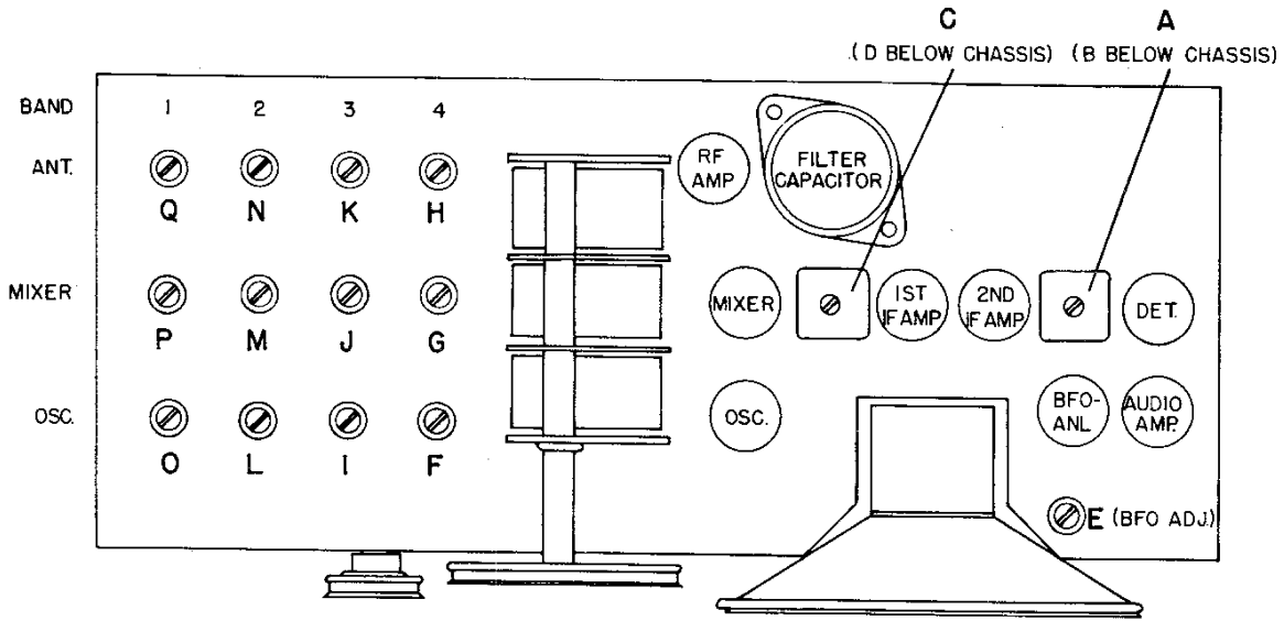
Figure 4. Alignment points
