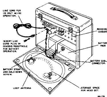
Figure 3. Battery compartment
