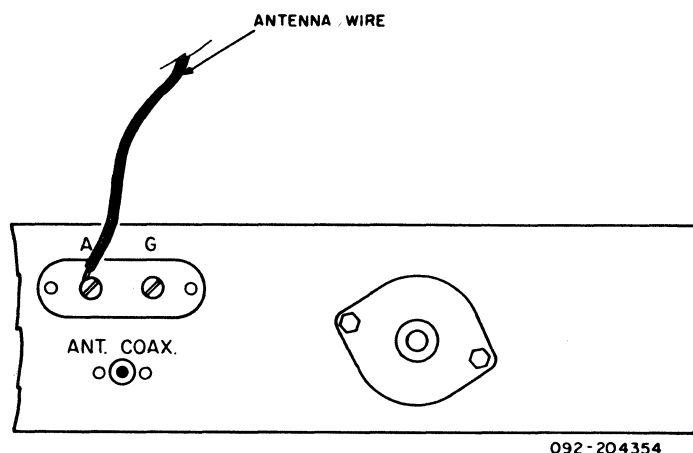
Figure 2. Single Wire Antenna
