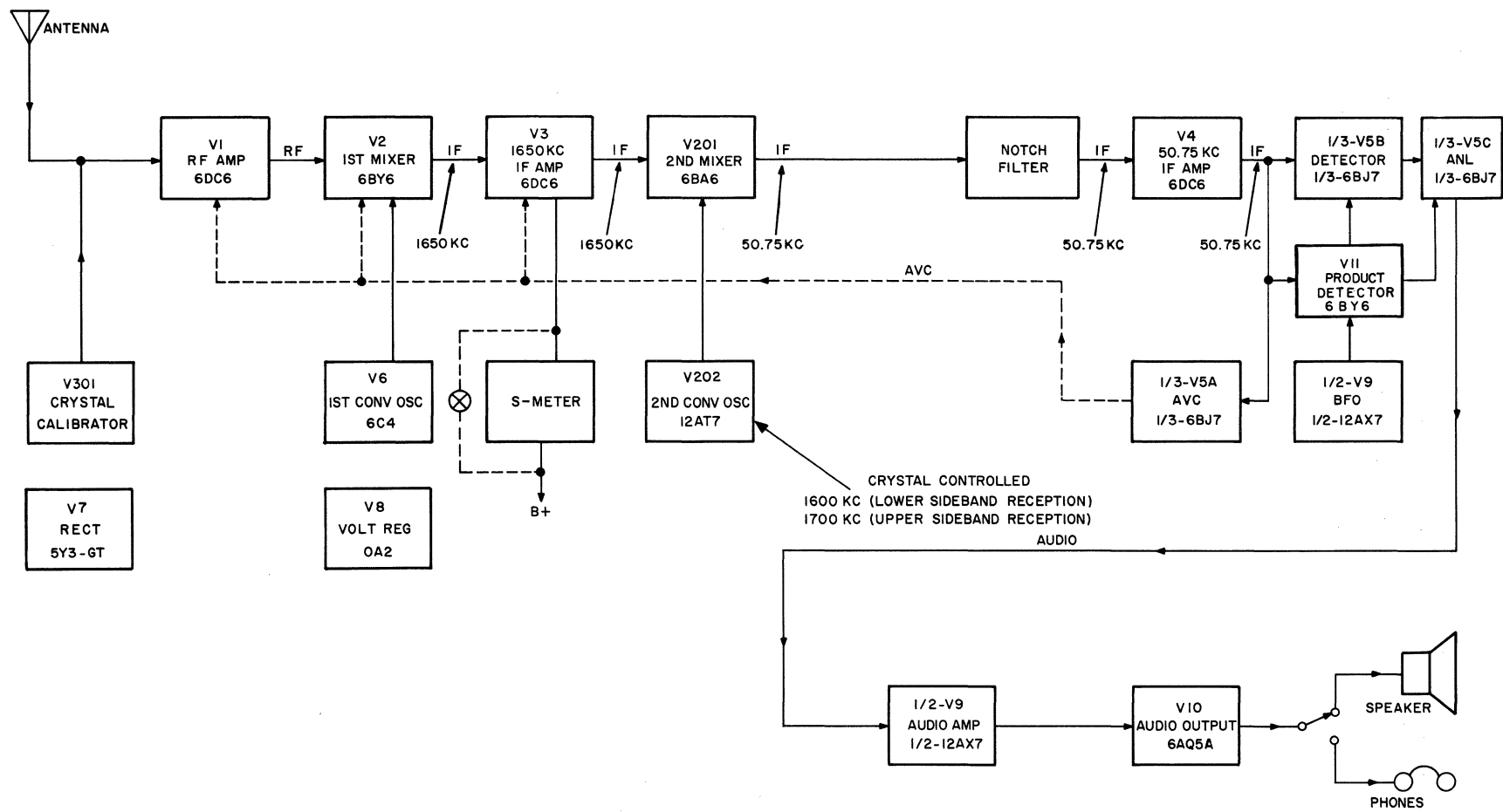
Figure 14. Block Diagram of SX-111 Receiver
