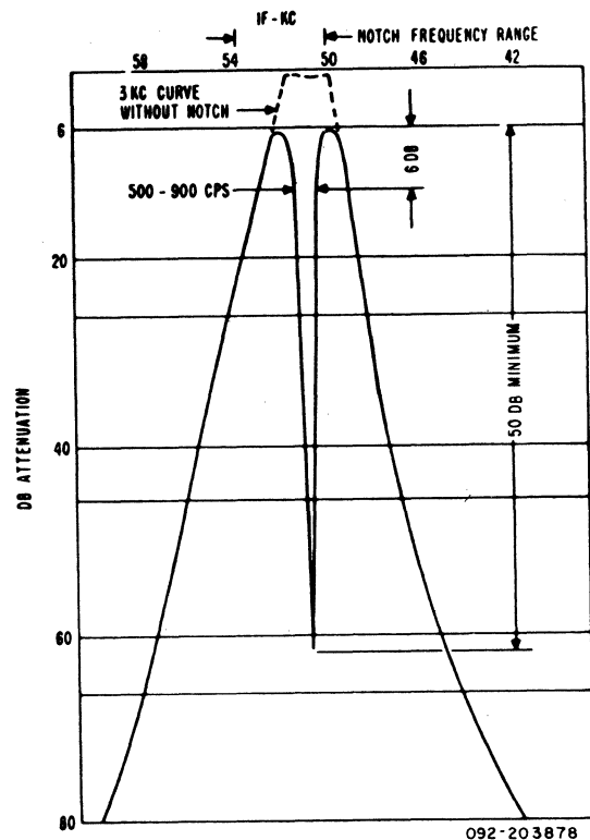
Figure 8. IF Selectivity Curve With Notch
