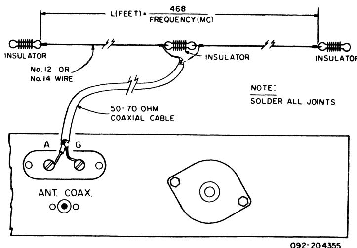
Figure 3. Doublet Antenna Using Twin-Lead Transmission Line
