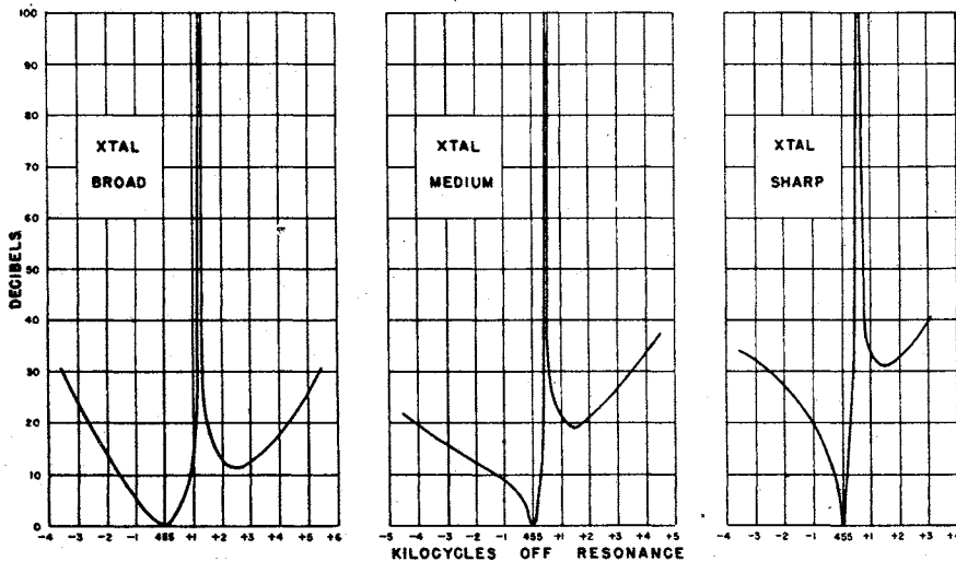
FIG. 4—CRYSTAL SELECTIVITY
