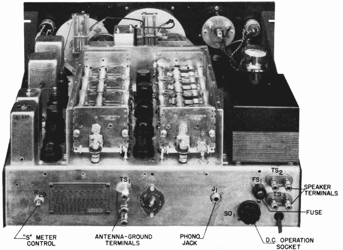
FIG. 9—SX28-A—REAR VIEW
