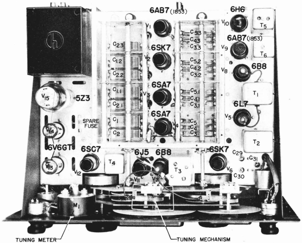
FIG. 9—SX28-A—REAR VIEW
