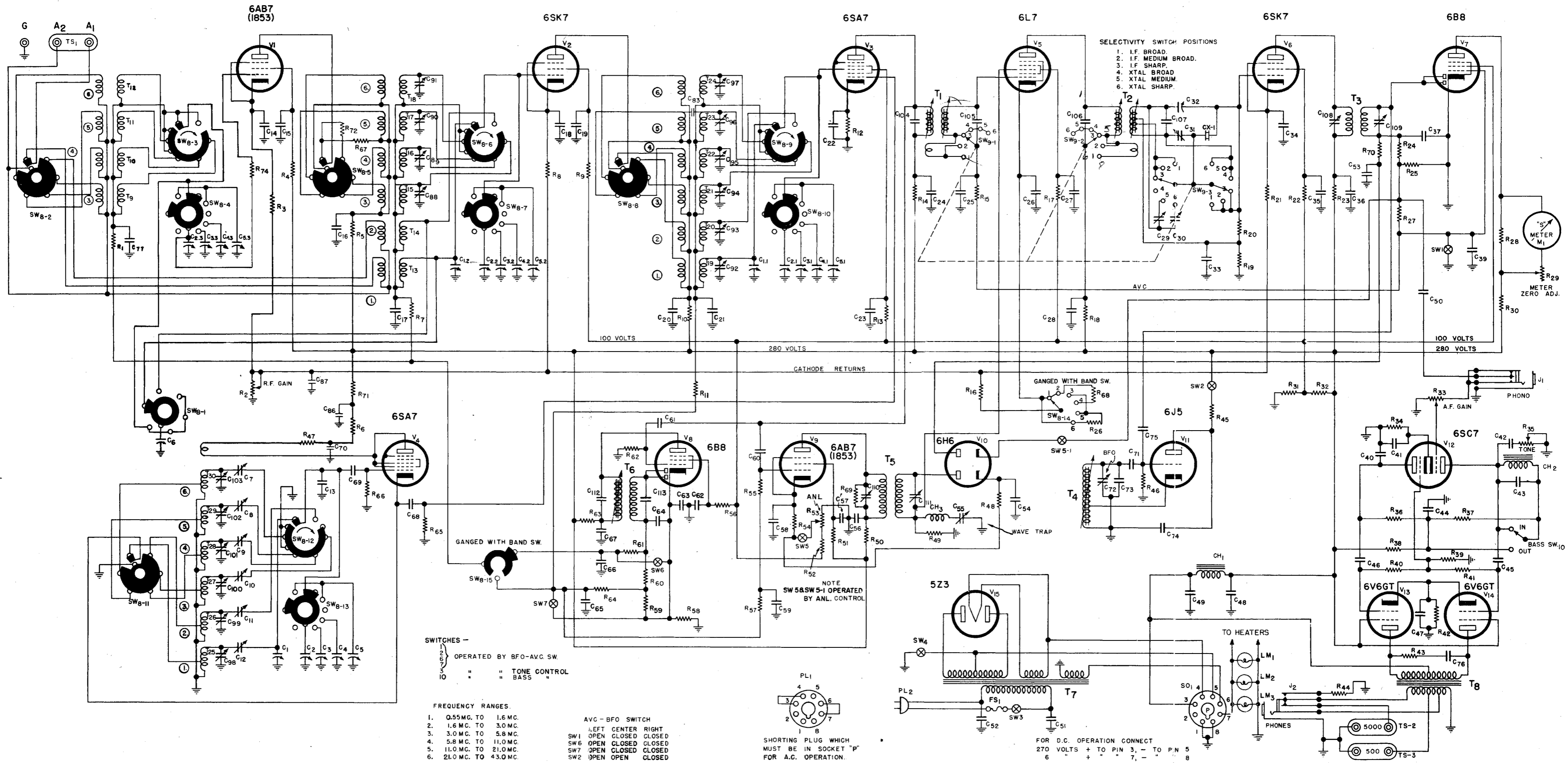
FIG. 13-SX28-A-SCHEMATIC
