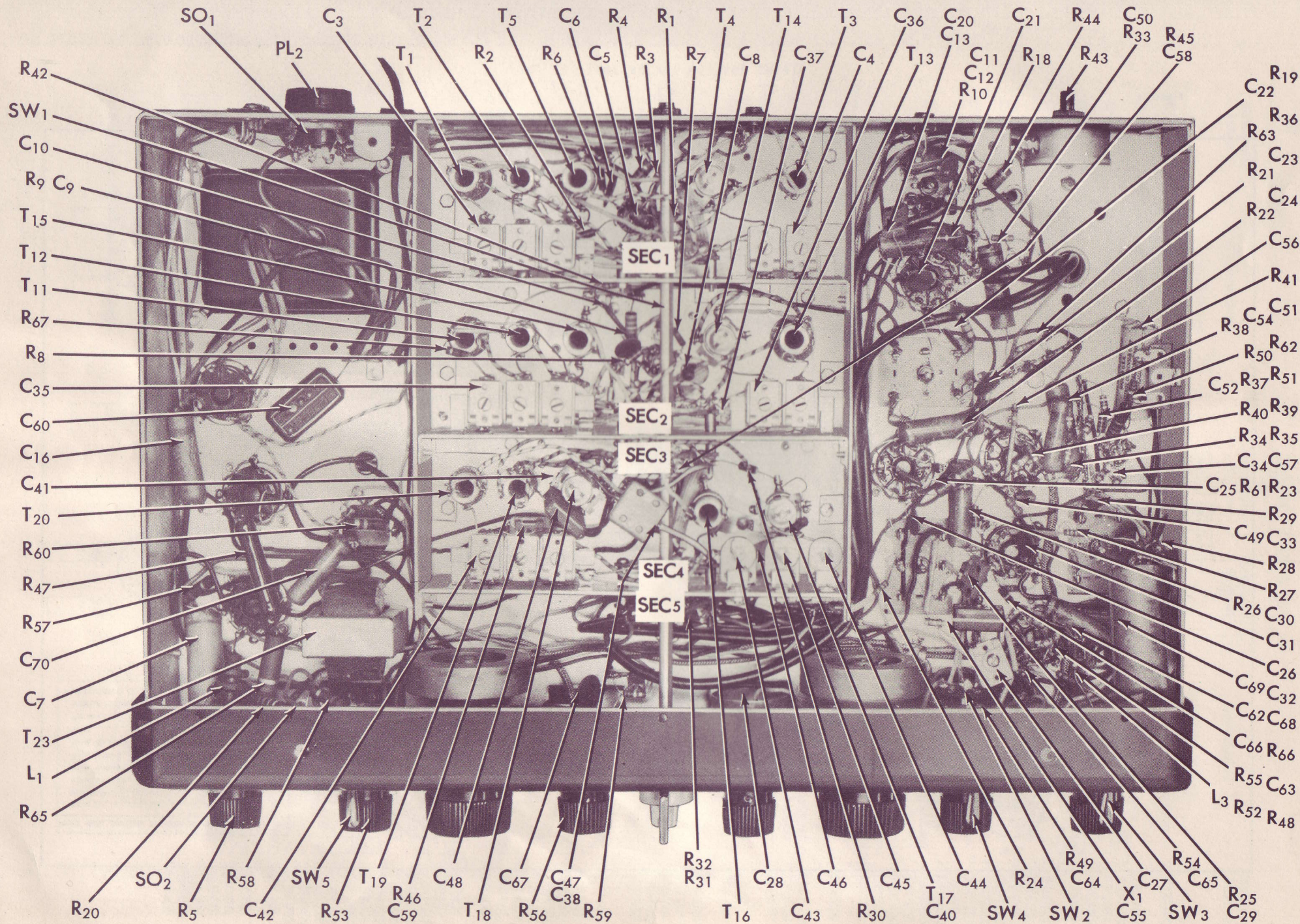
FIG. 15. BOTTOM VIEW - COMPONENT LOCATION
