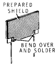
Detail 3-11C
