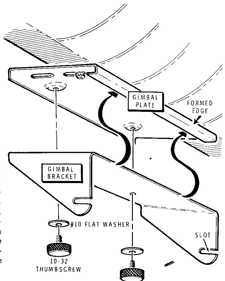
PICTORIAL 11-9
