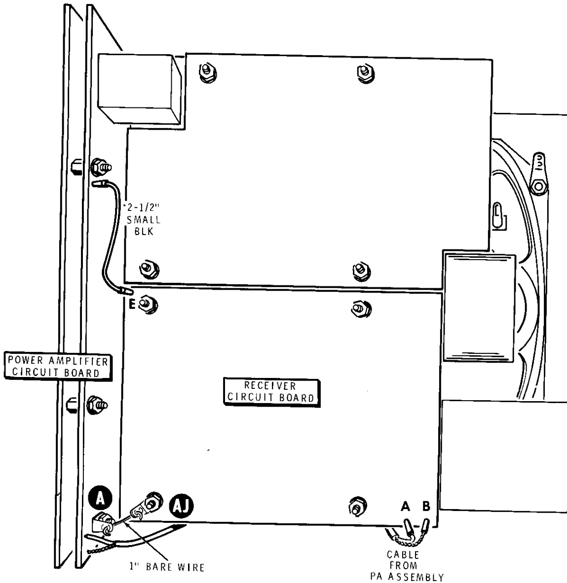
PICTORIAL 6-15
