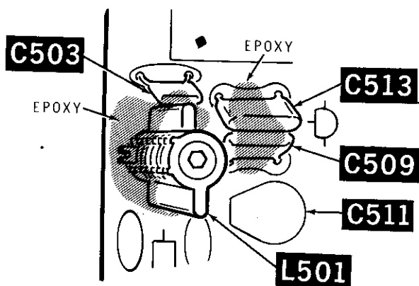
PICTORIAL 2-6
