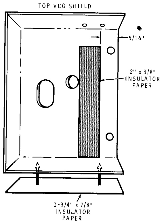
Detail 2-9B
