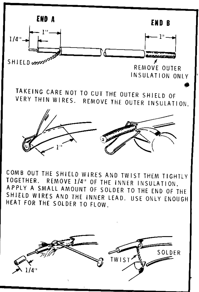
Detail 2-7H
