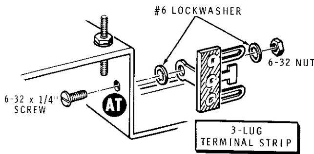
Detail 1-3G
