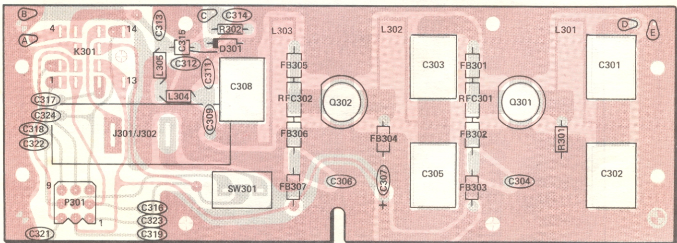
POWER AMPLIFIER CIRCUIT BOARD (Shown from component side.) Foil on component side is shown in red.)
