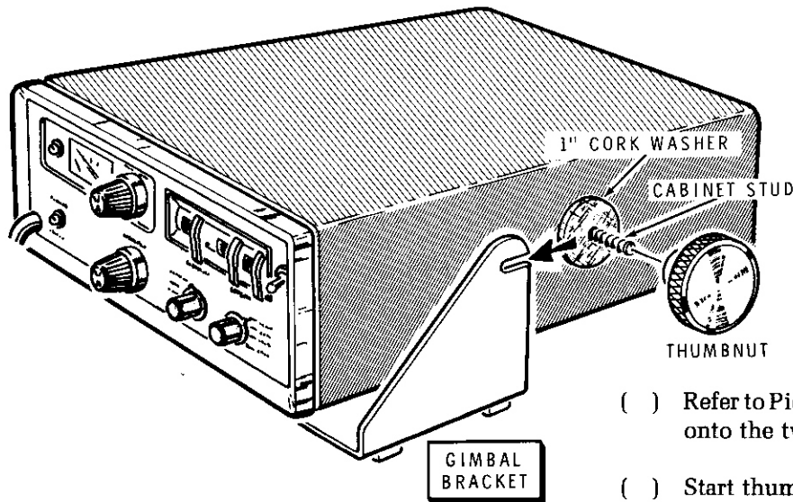
PICTORIAL 11-3
