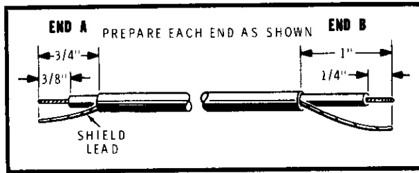
Detail 6-10D
