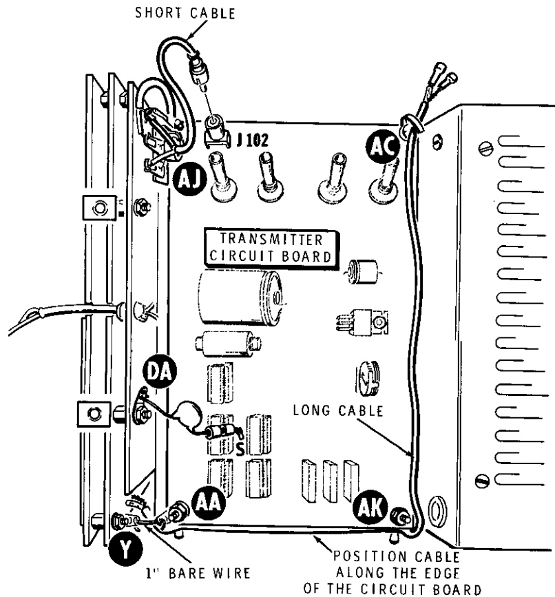
PICTORIAL 6-14
