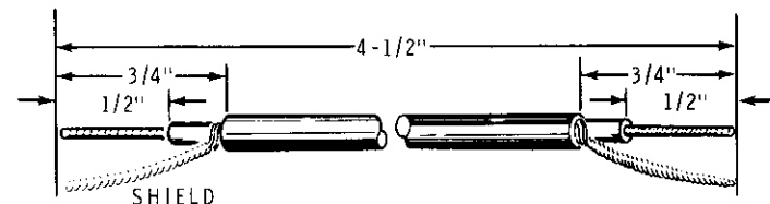
Detail 4-10B
