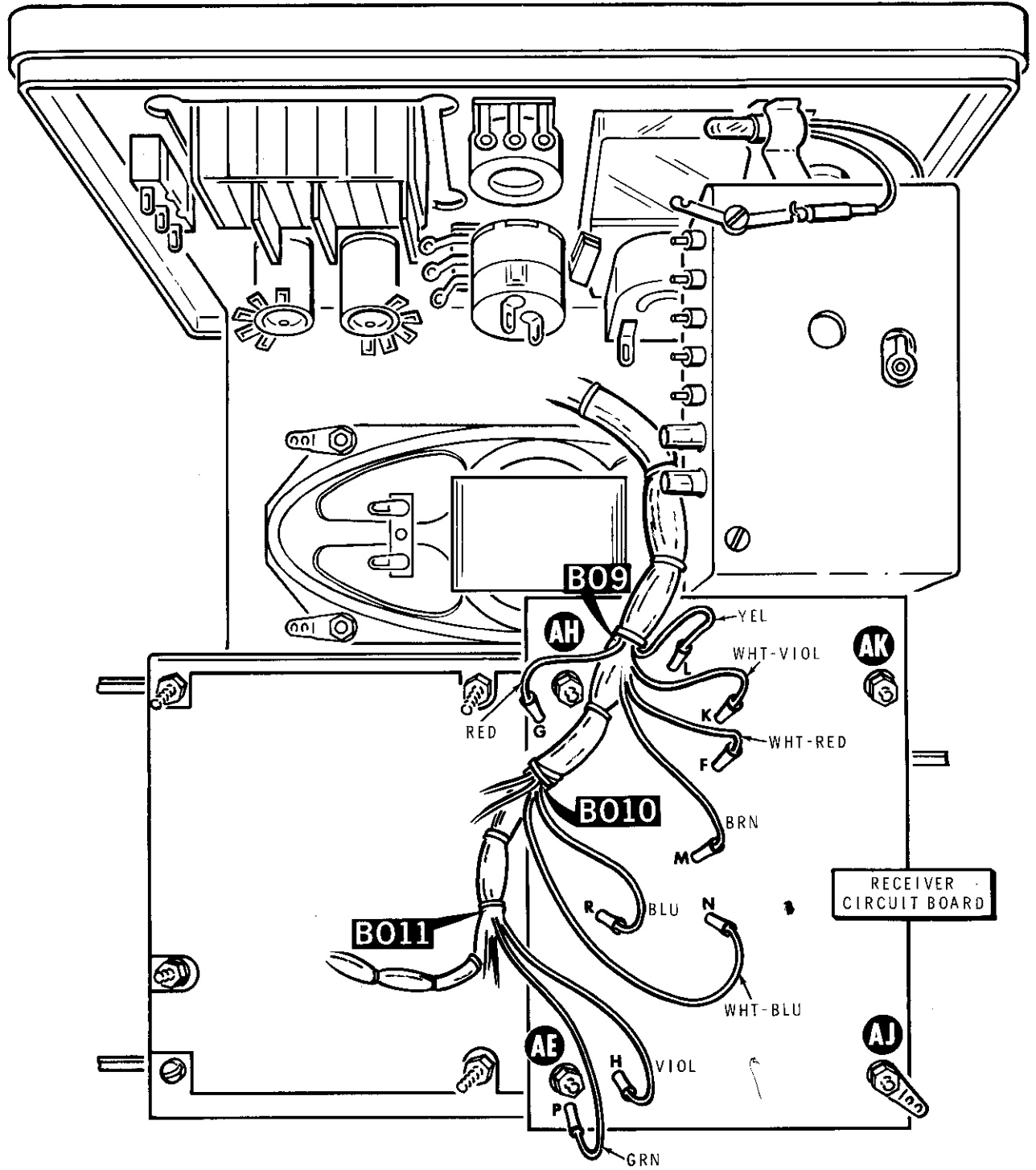
PICTORIAL 3-12
