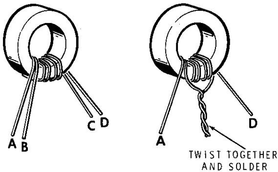
Detail 6-10A
