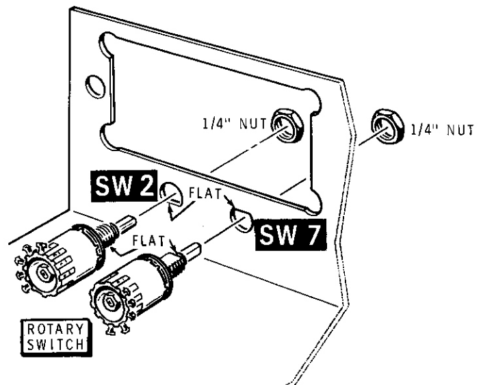
Detail 1-3J
