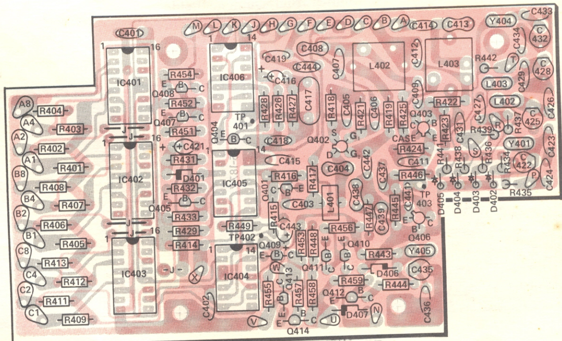
SYNTHESIZER CIRCUIT BOARD (Shown from component side. Foil on component side is shown in red.)
