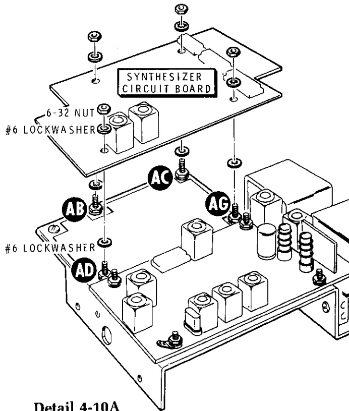
Detail 4-10A
