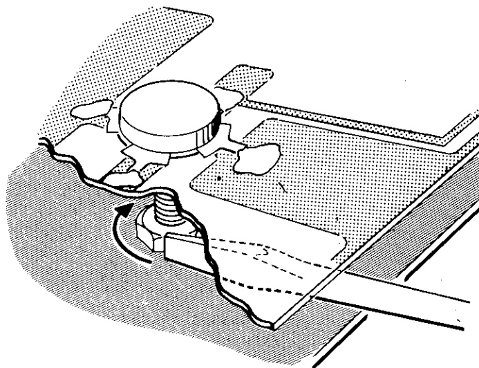
Detail 6-12C
