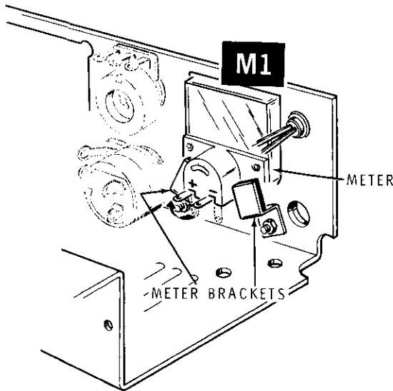
Detail 1-3F
