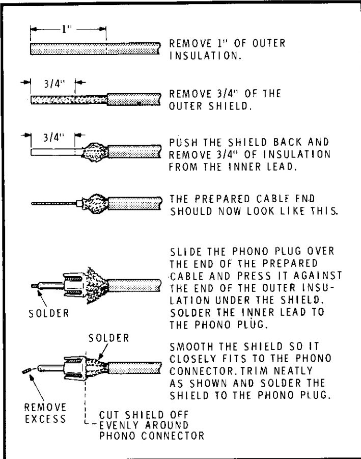
PICTORIAL 11-5
