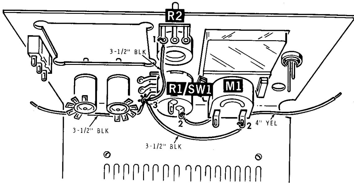
PICTORIAL1-4
