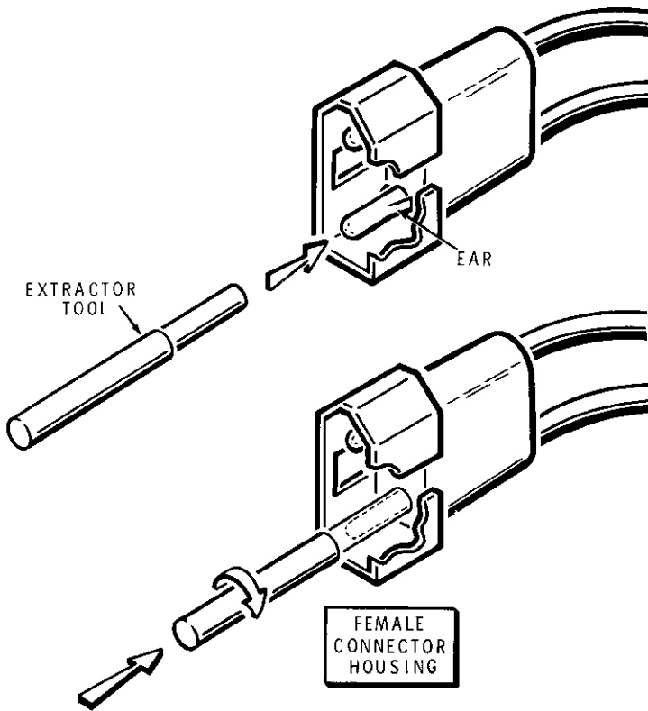
Detail 5-12B
