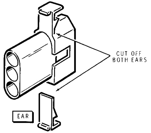
Detail 5-12A
