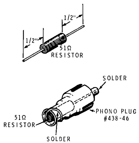
PICTORIAL 9-4
