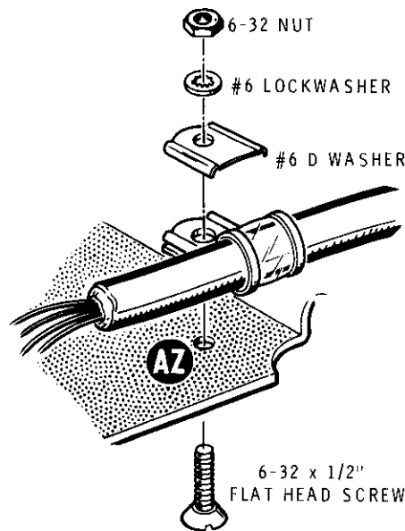
Detail 7-1A
