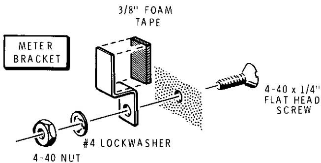
Detail 1-3C
