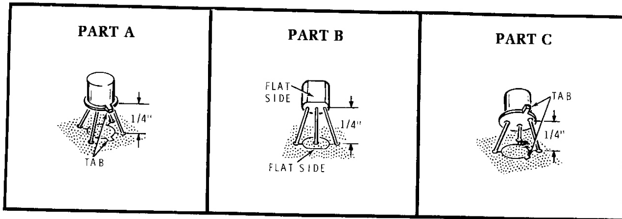
Detail 4-5A
