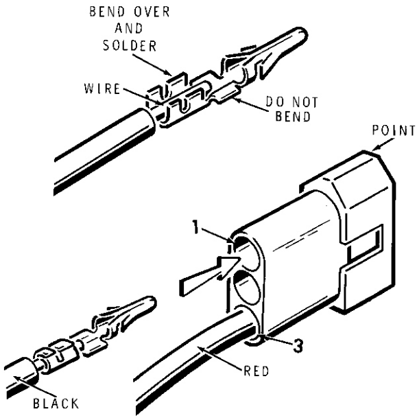
PICTORIAL 5-12
