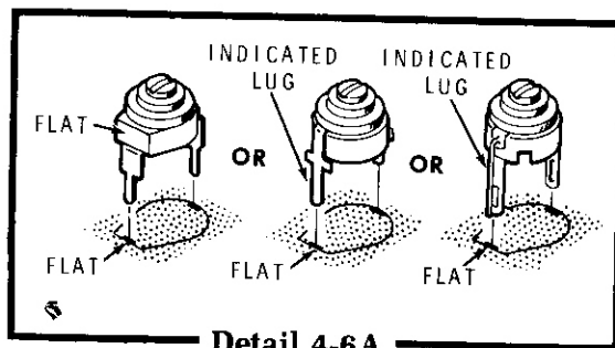
Detail 4-6A
