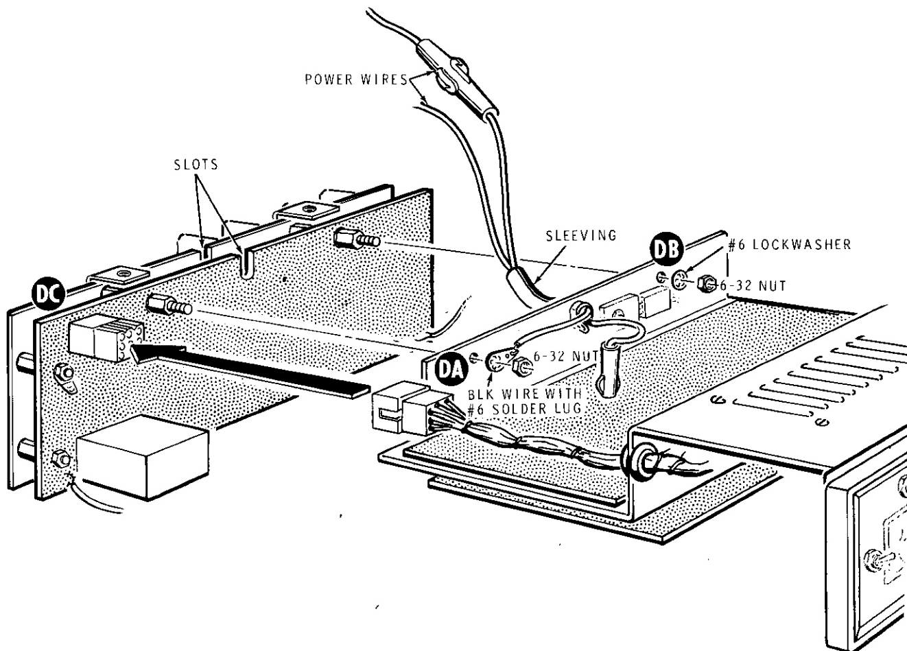
PICTORIAL 6-13
