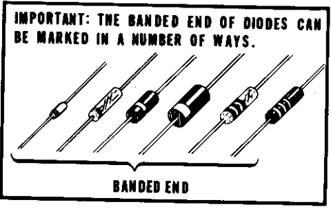
Detail 5-2A
