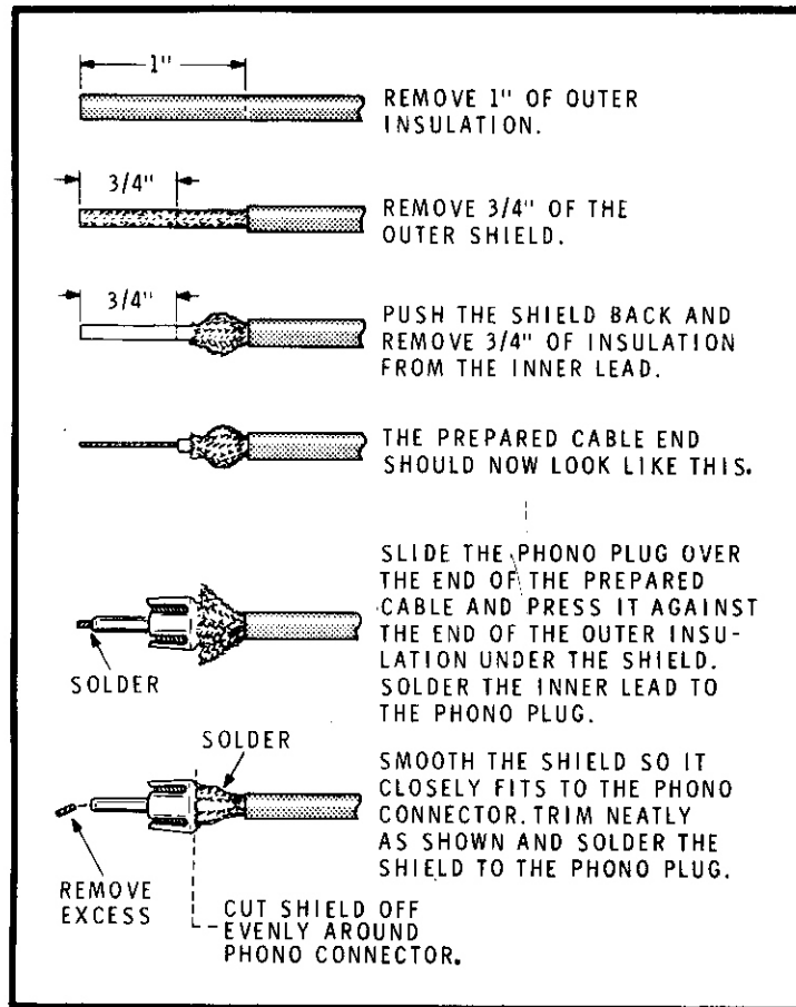
PICTORIAL 11-12
