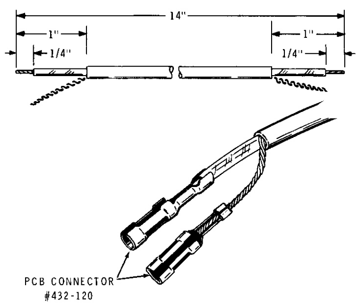
PICTORIAL 9-3
