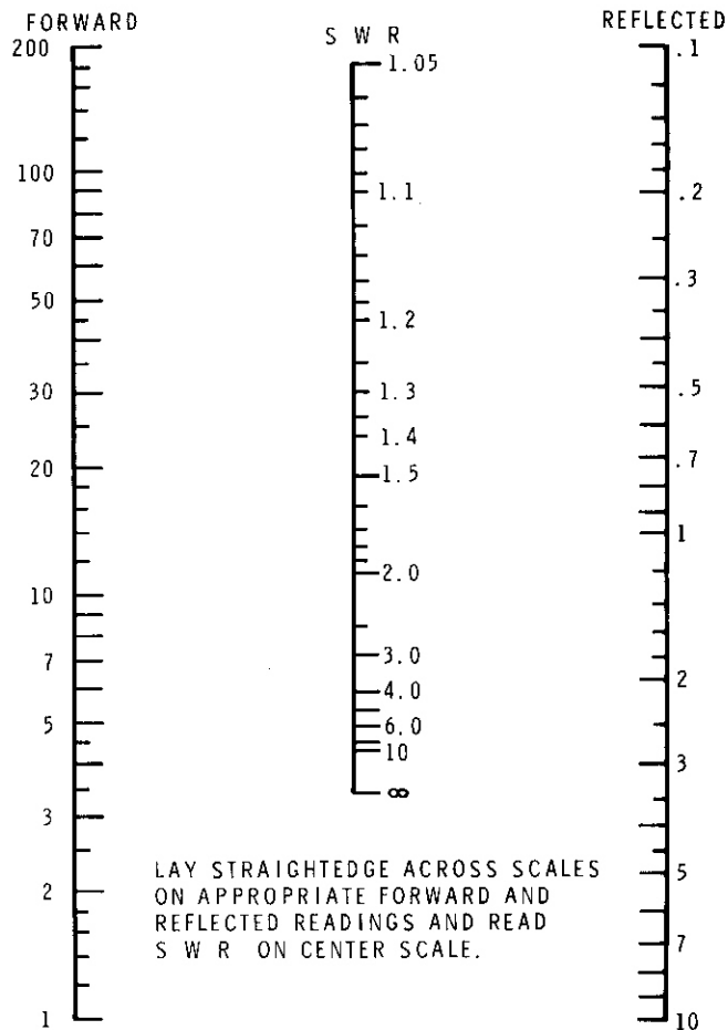
SWR CALCULATOR
