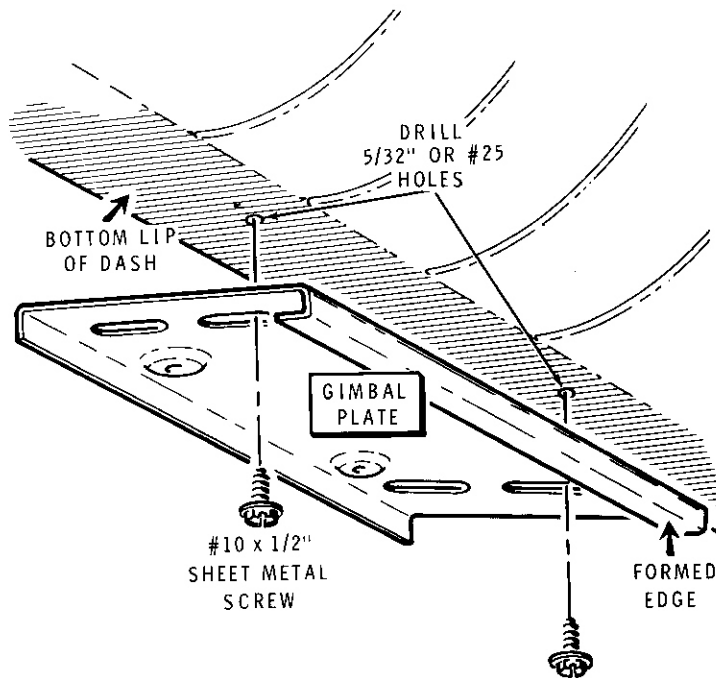
PICTORIAL 11-8
