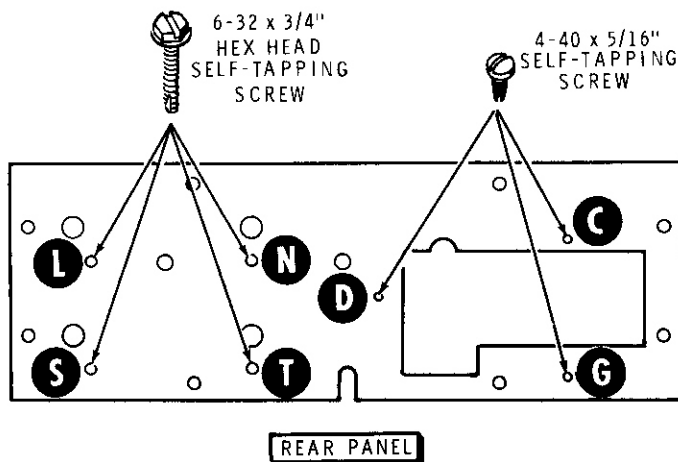
Detail 6-11A
