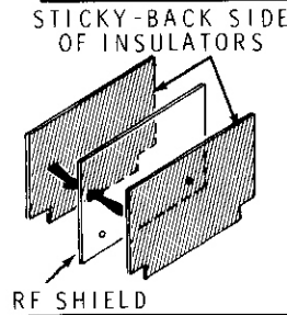
Detail 3-11B
