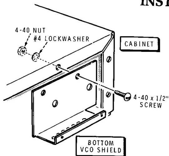
Detail 2-7A
