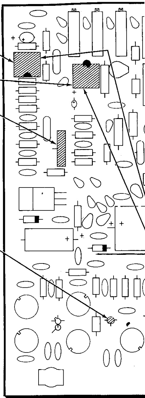
PICTORIAL 5-7
