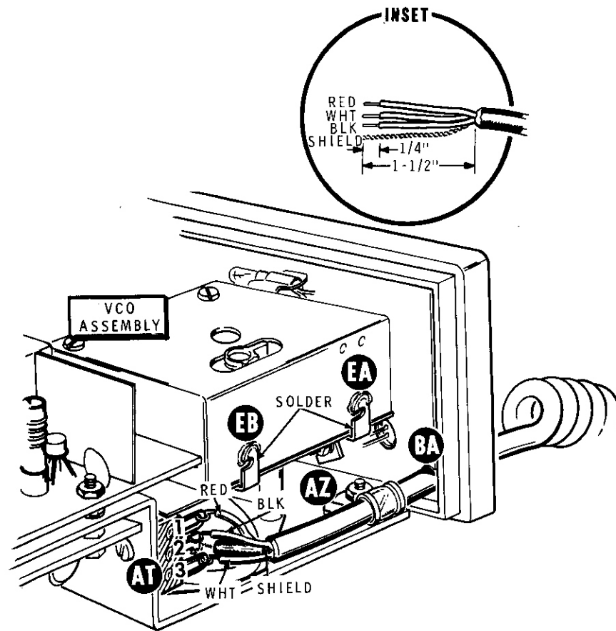
PICTORIAL 7-1
