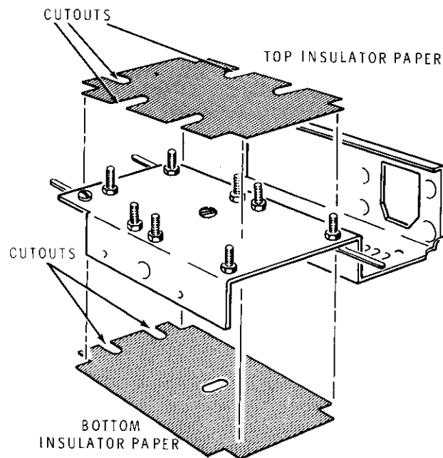
Detail 1-3B
