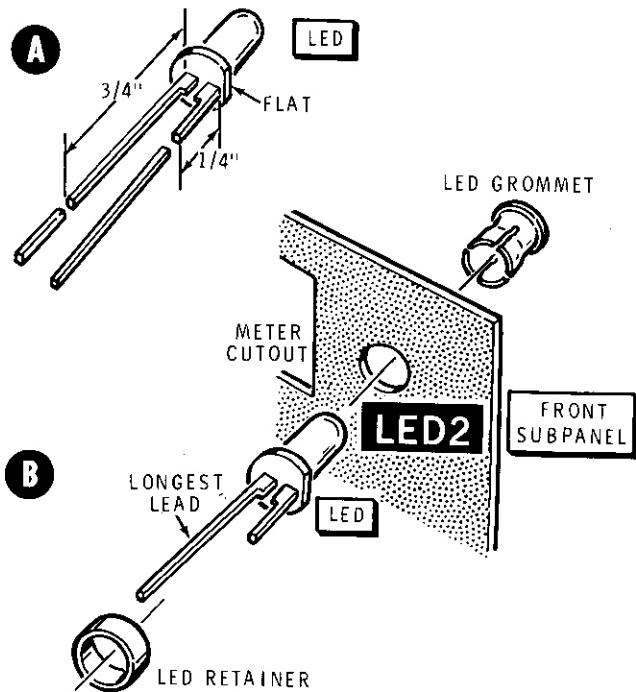
Detail 1-3D
