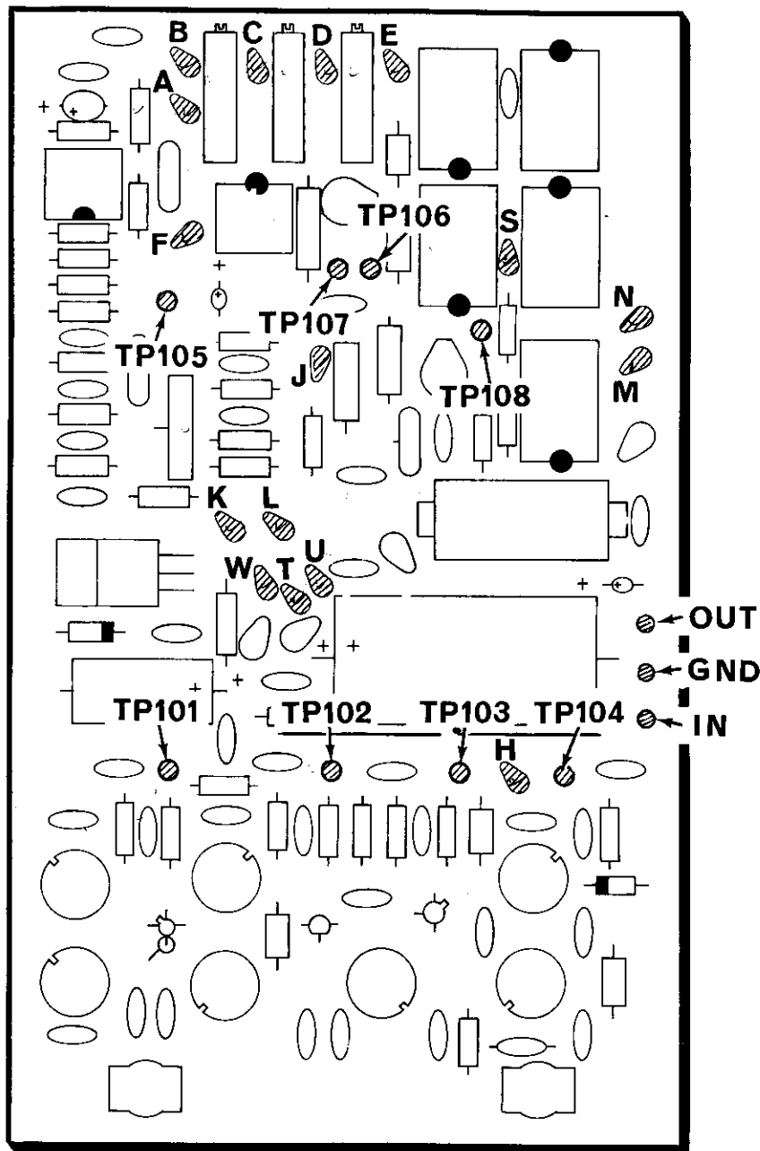
PICTORIAL 5-1
