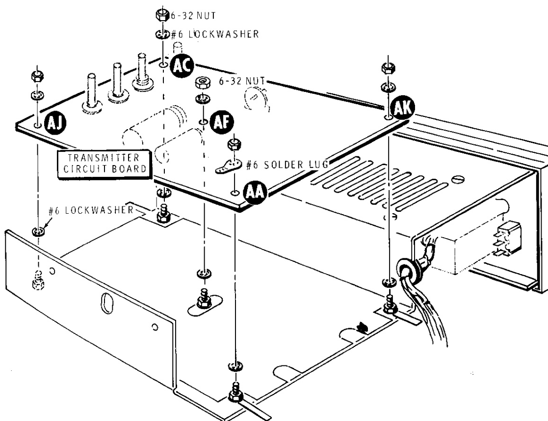
Detail 5-11A
