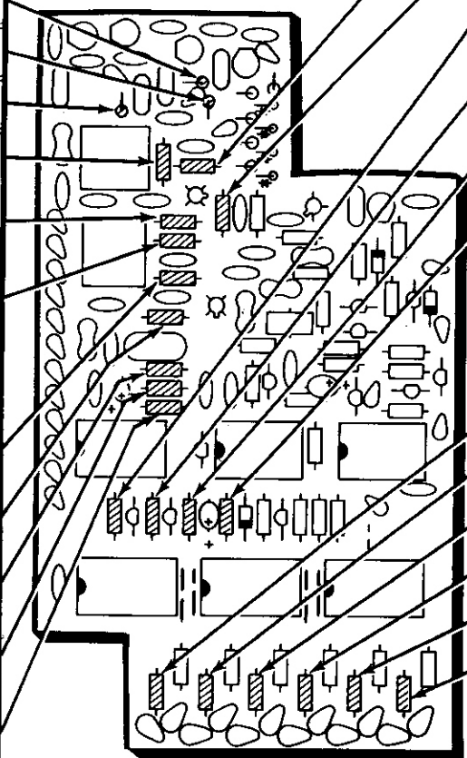
PICTORIAL 4-3
