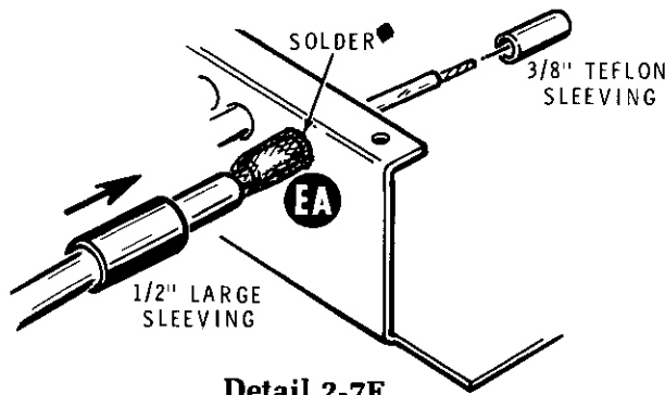
Detail 2-7F
