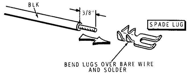
PICTORIAL 11-11
