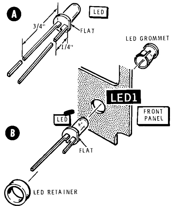
Detail 1-7C
