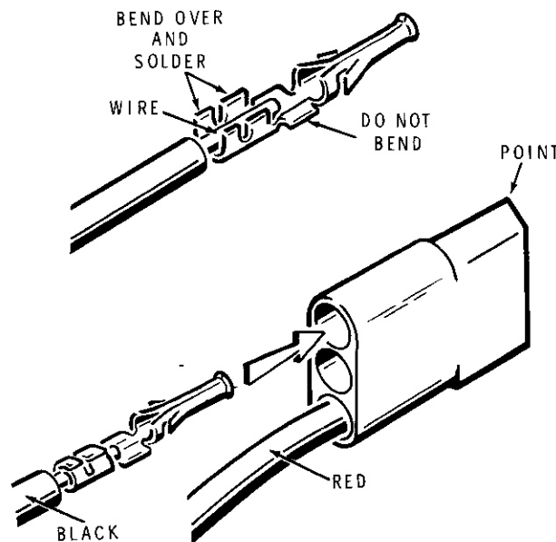
PICTORIAL 11-4
