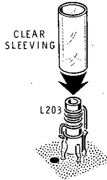
Detail 3-10A
