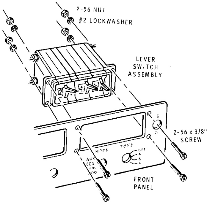
Detail 1-7B
