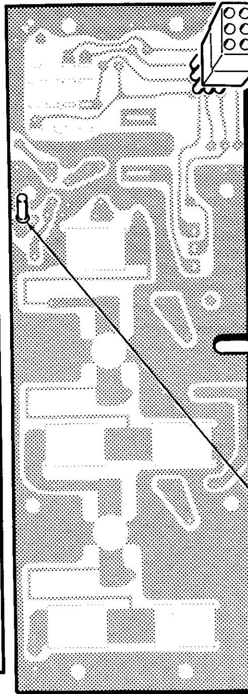
PICTORIAL 6-5
