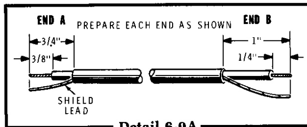
Detail 6-9A
