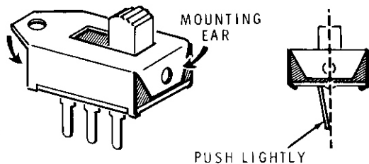
Detail 6-12A
