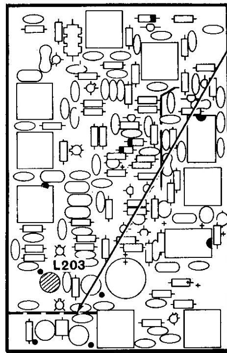
Detail 3-11B
