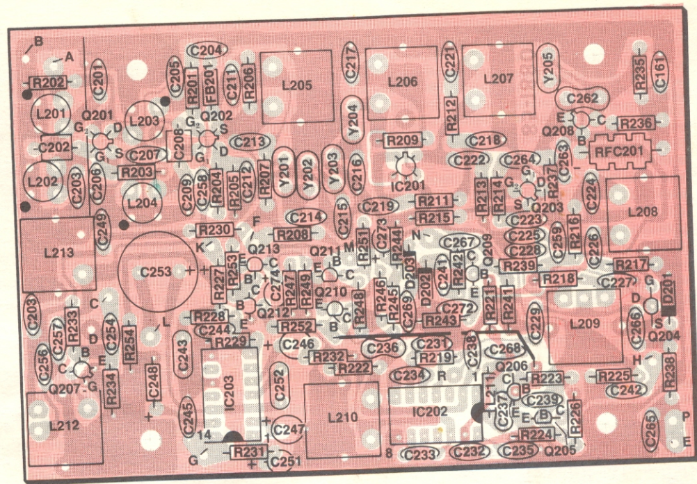
RECEIVER CIRCUIT BOARD (Shown from component side. Foil on component side is shown in red.)
