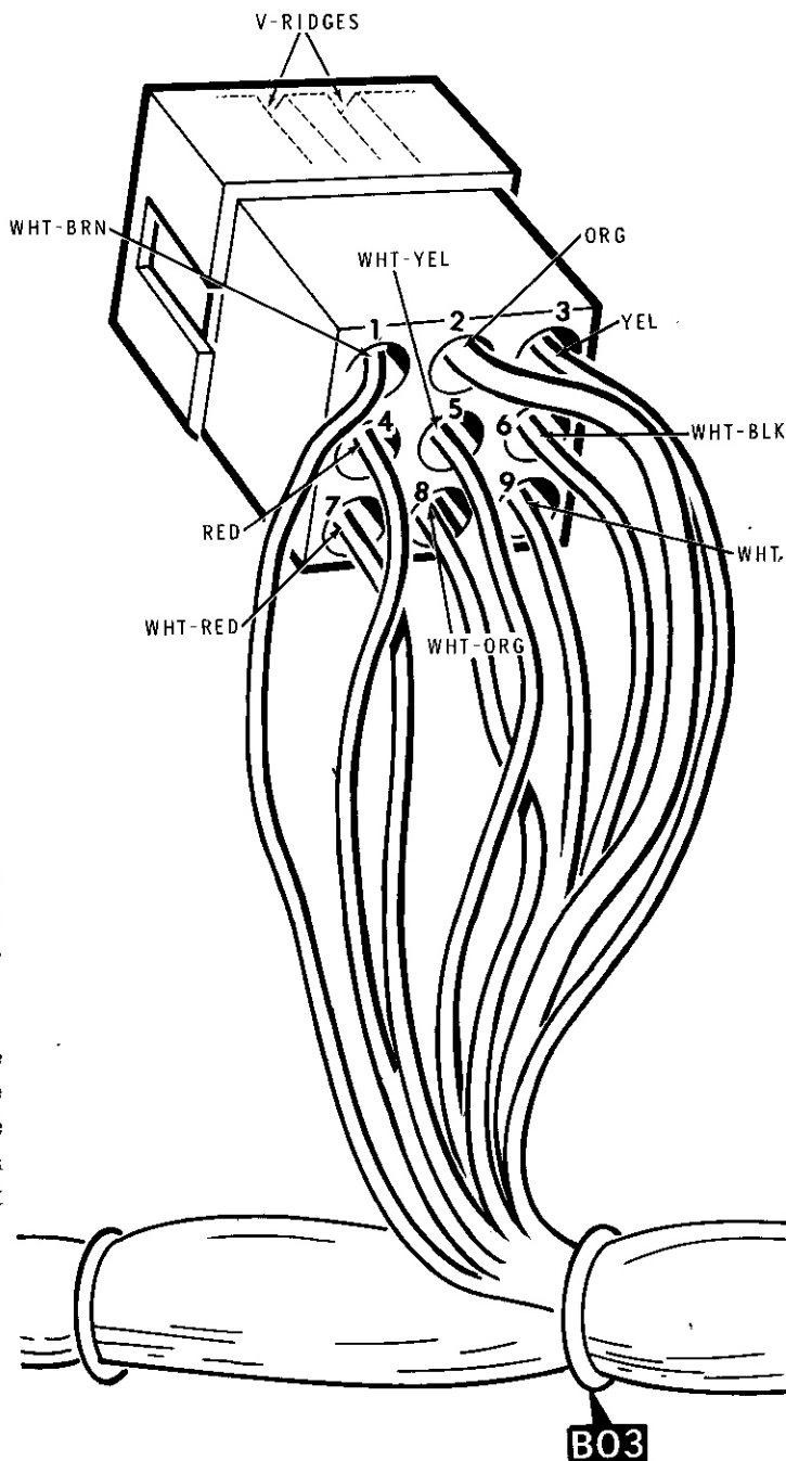
PICTORIAL 1-2
