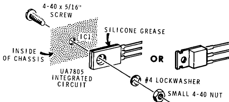
Detail 5-11B
