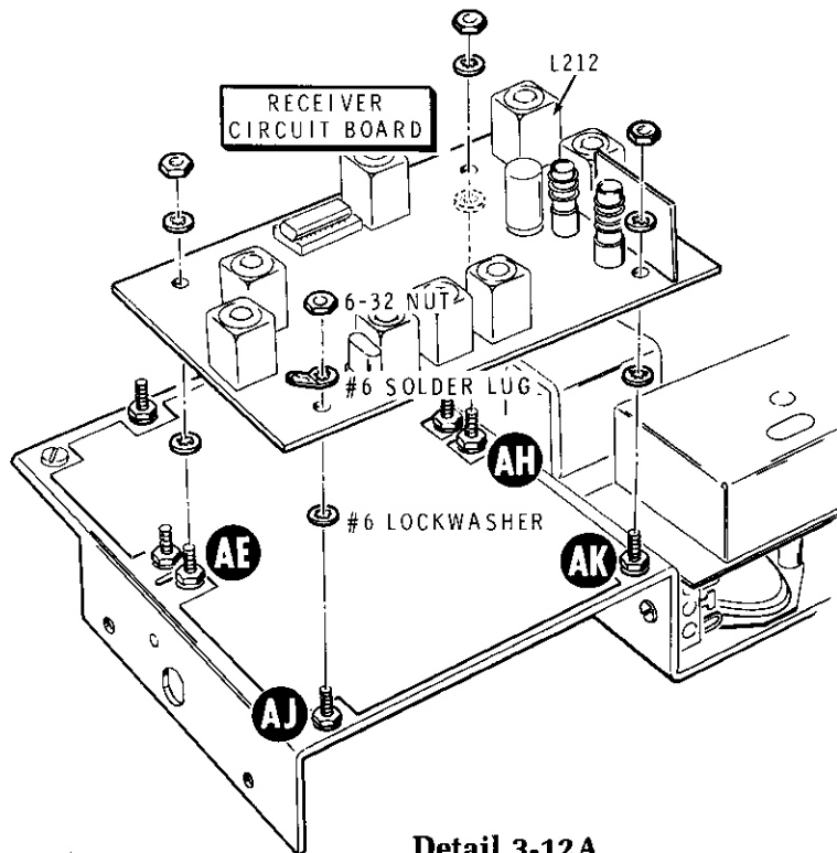
Detail 3-12A
