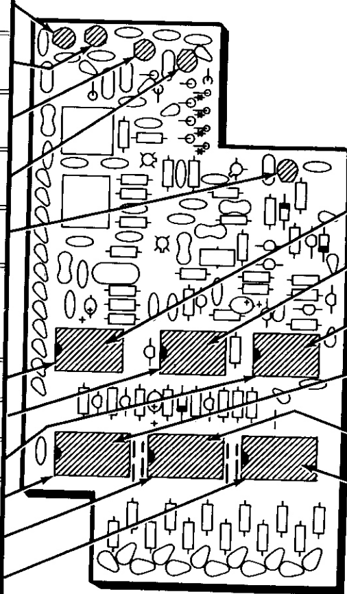
PICTORIAL 4-6
