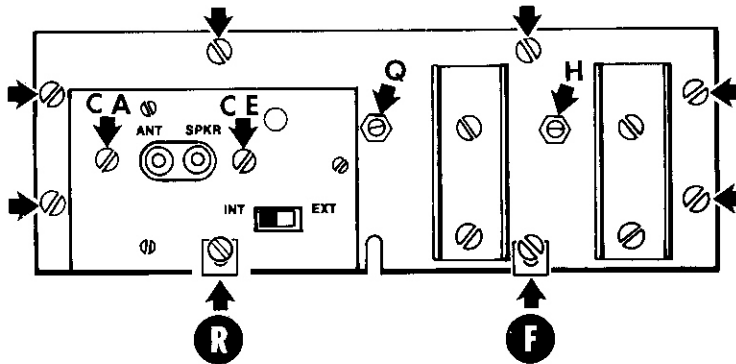
PICTORIAL 13-1
