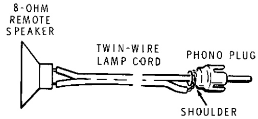
PICTORIAL 11-6
