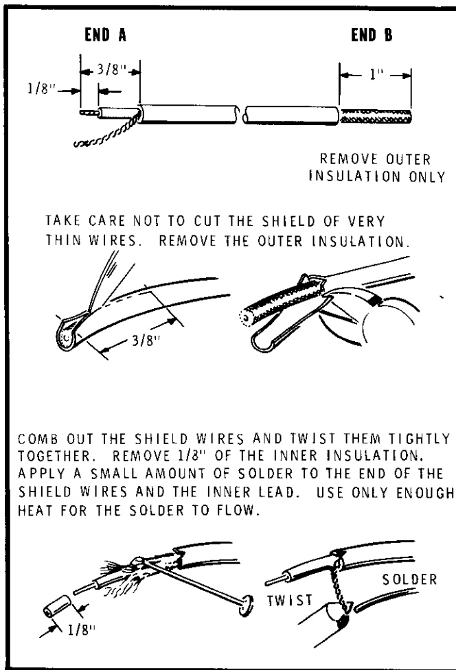
Detail 2-7D
