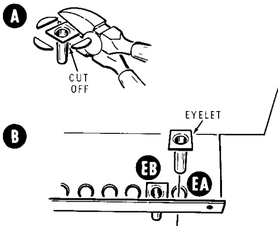
Detail 2-7B
