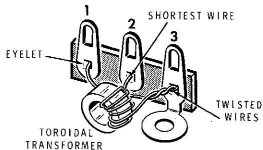
Detail 6-10C
