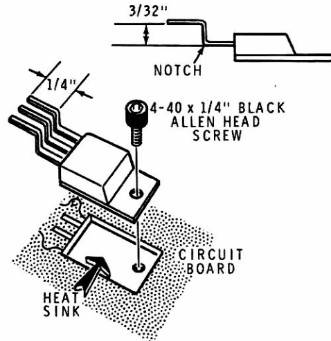
Detail 14-6C
