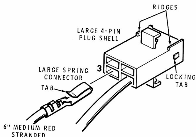
Detail 15-10G
