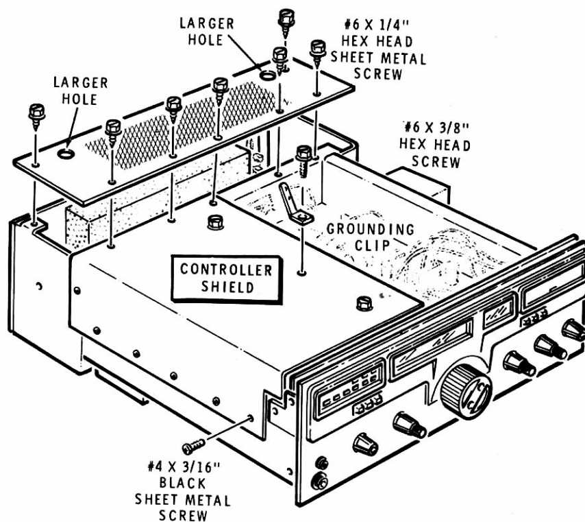
PICTORIAL 17-1
