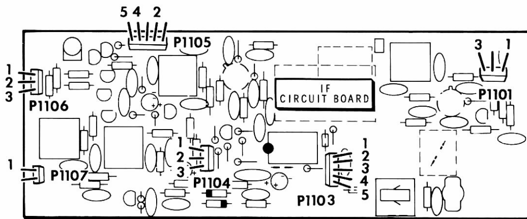
PICTORIAL 8-8
