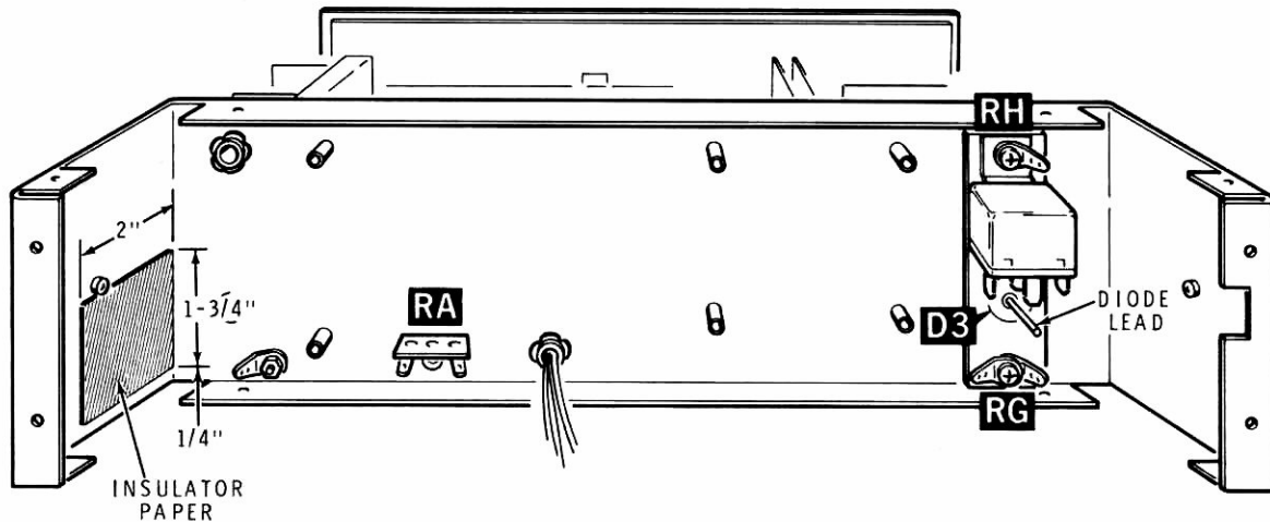
PICTORIAL 15-9
