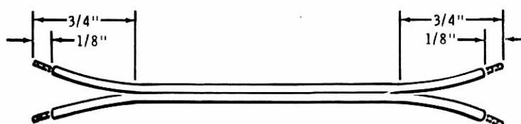
Detail 3-8B
