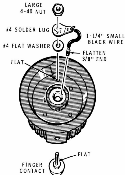
Detail 15-12C
