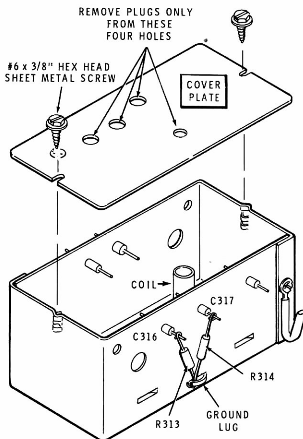
PICTORIAL 6-8
