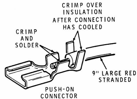
Detail 15-10A
