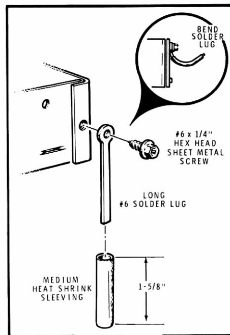
Detail 6-5A
