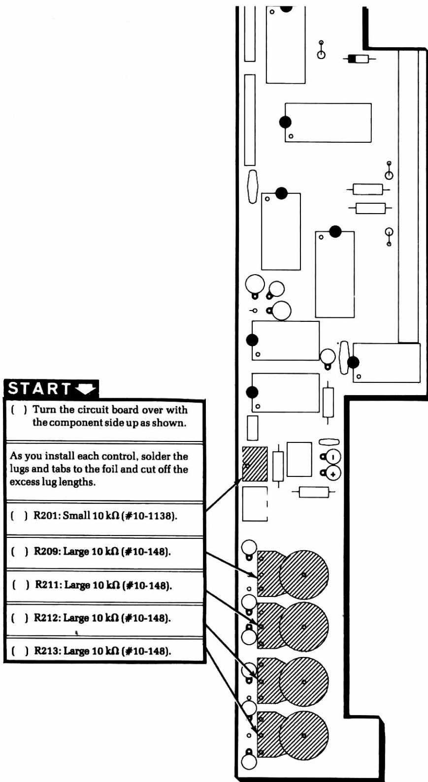
PICTORIAL 3-6
