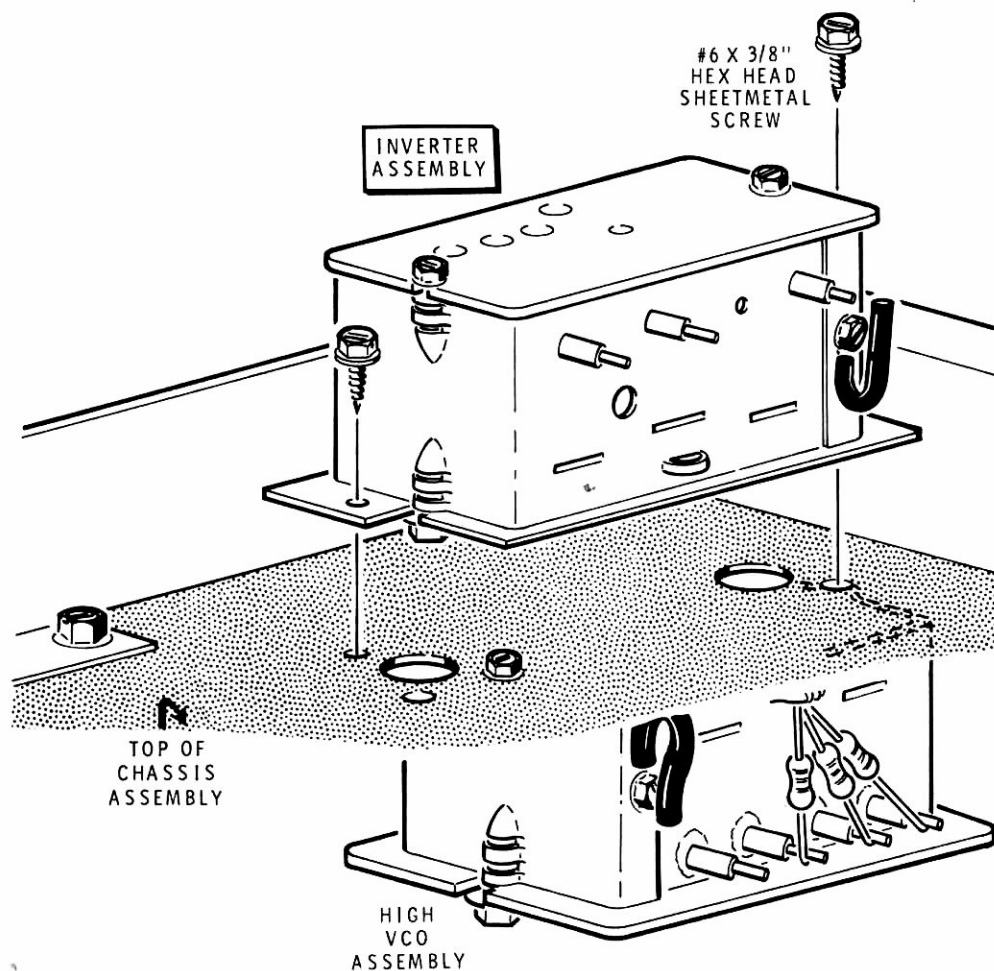
Detail 15-5B
