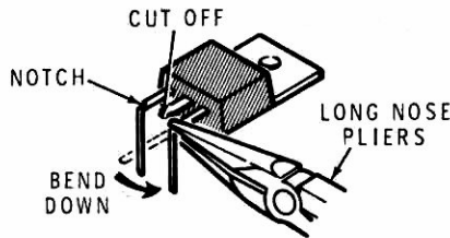
Detail 14-5A
