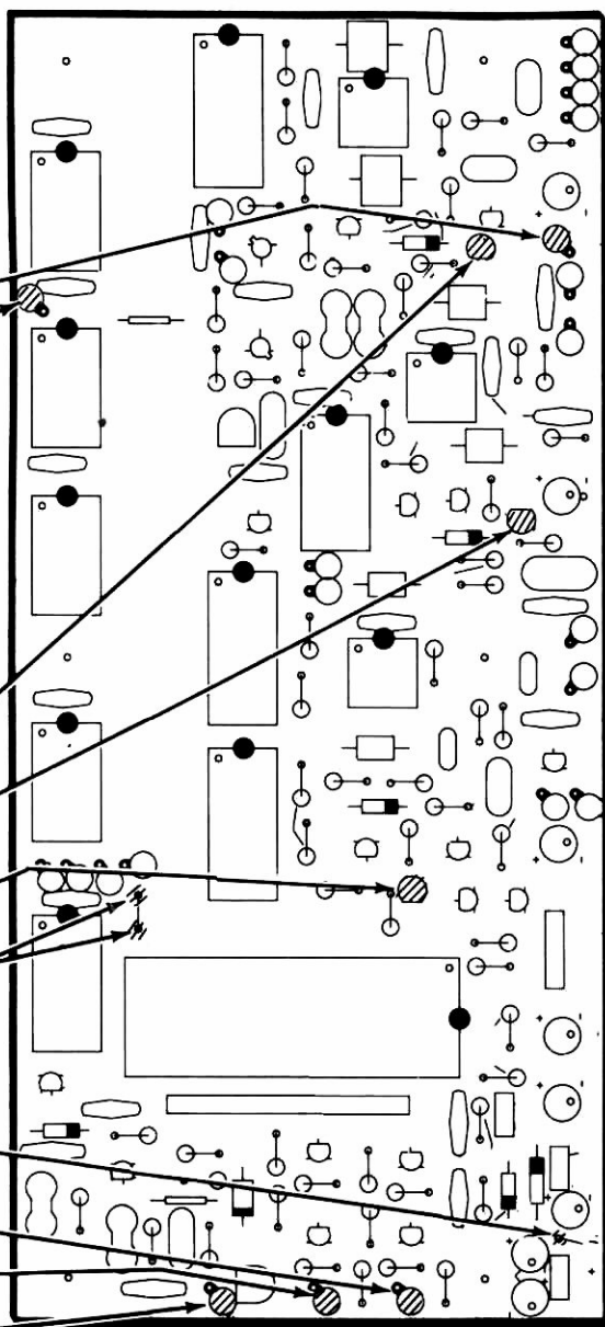
PICTORIAL 10-4
