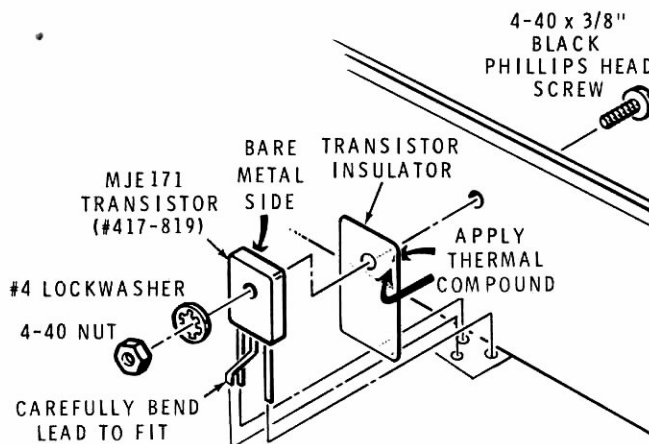
Detail 7-5B
