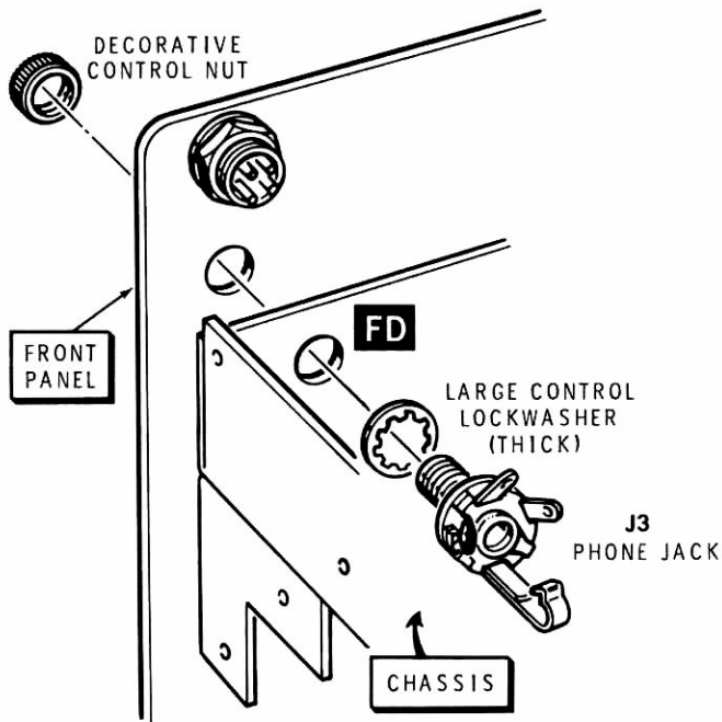
Detail 15-4A
