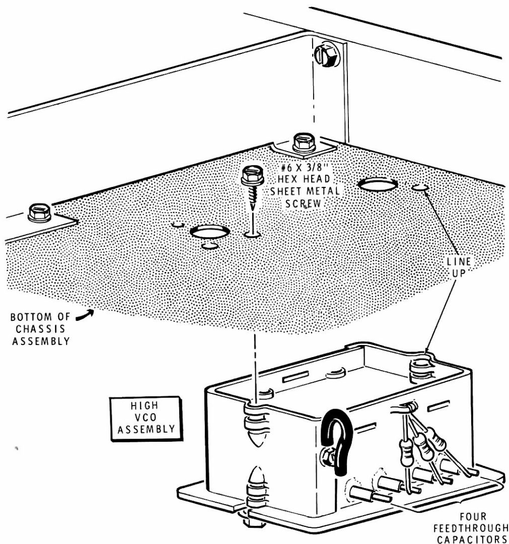
Detail 15-5A
