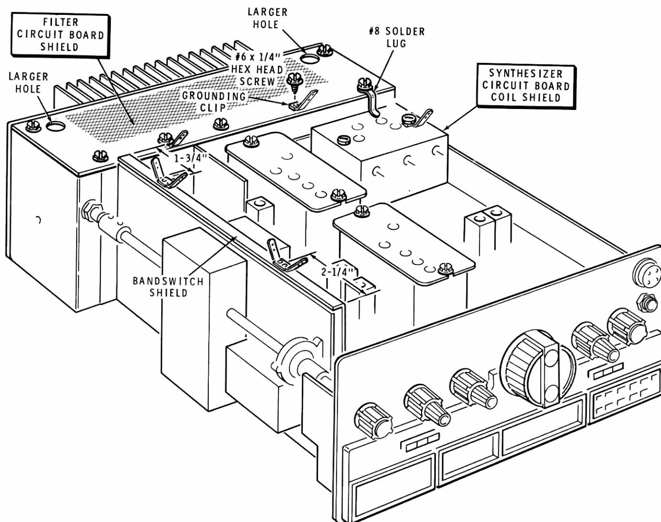
PICTORIAL 17-2
