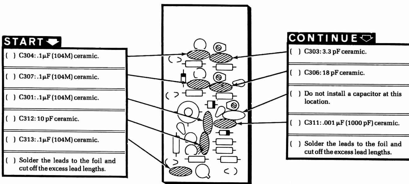
PICTORIAL 6-3
