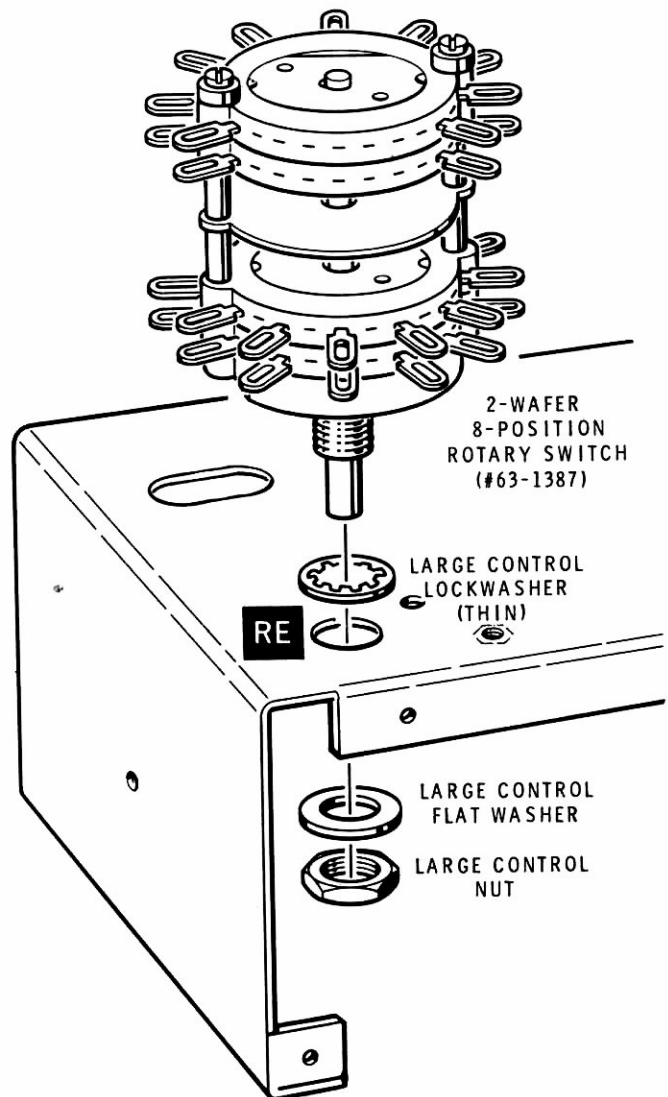
Detail 15-1A
