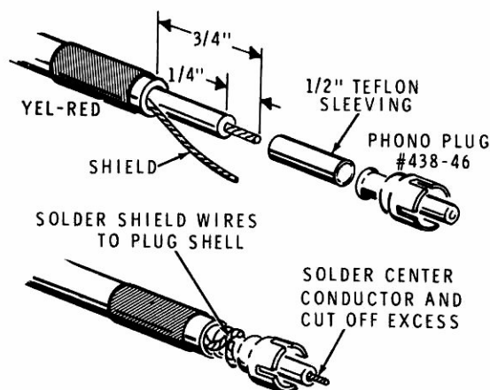
Detail 16-2A
