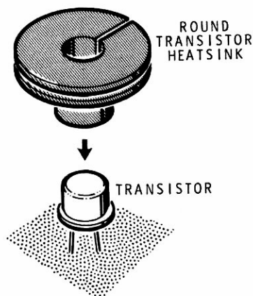
Detail 12-11D
