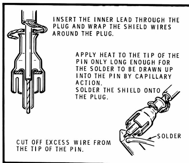
Detail 15-10K
