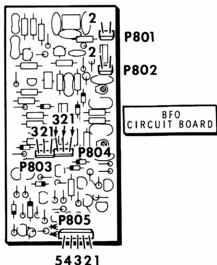
PICTORIAL 9-8
