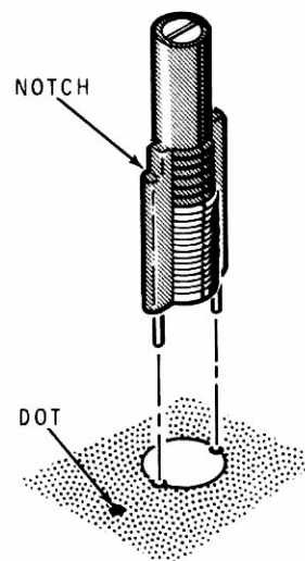
Detail 12-11C
