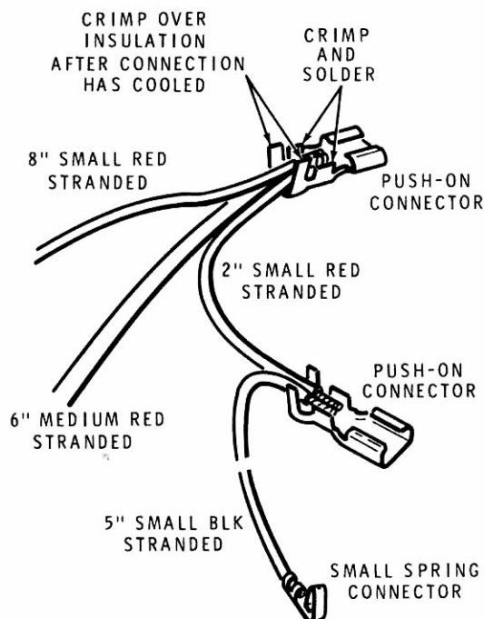
Detail 15-10F
