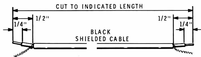
Detail 10-11A
