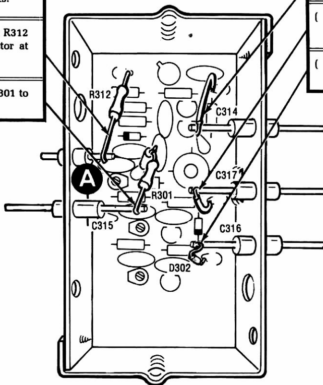
PICTORIAL 6-7
