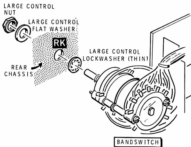
Detail 15-11A
