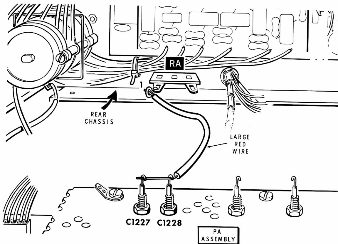
Detail 16-18A
