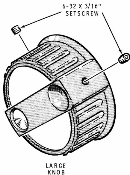
Detail 15-12B
