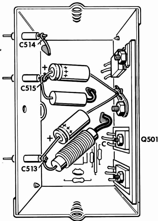
PICTORIAL 7-7
