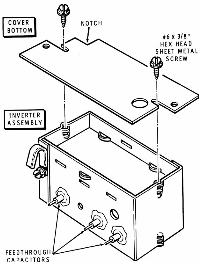
PICTORIAL 7-6
