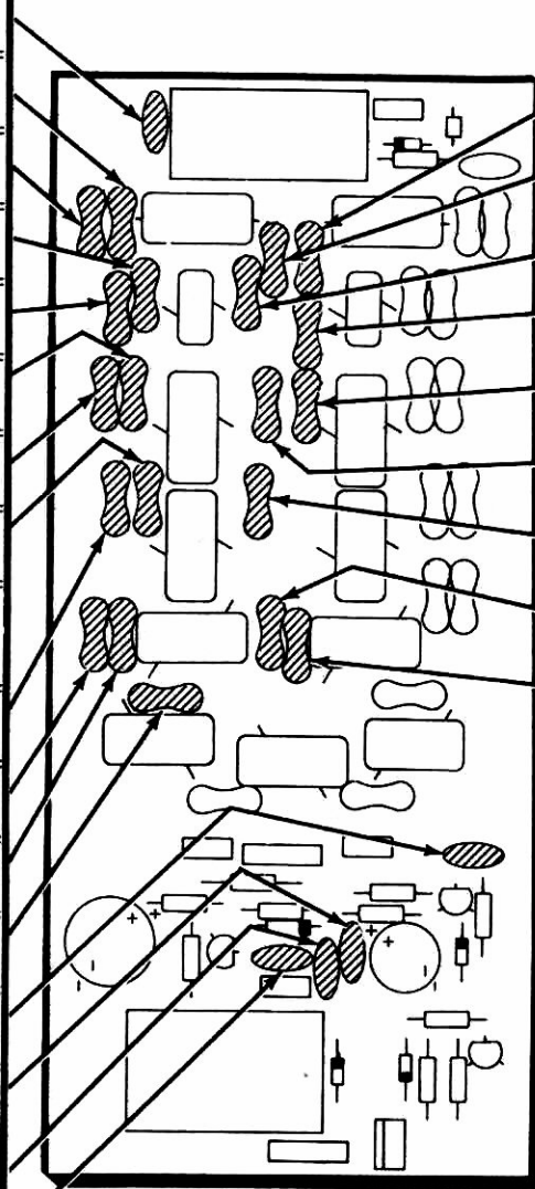
PICTORIAL 2-3
