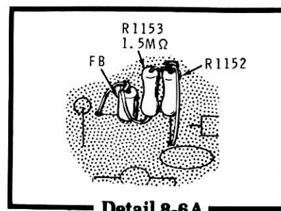
Detail 8-6A
