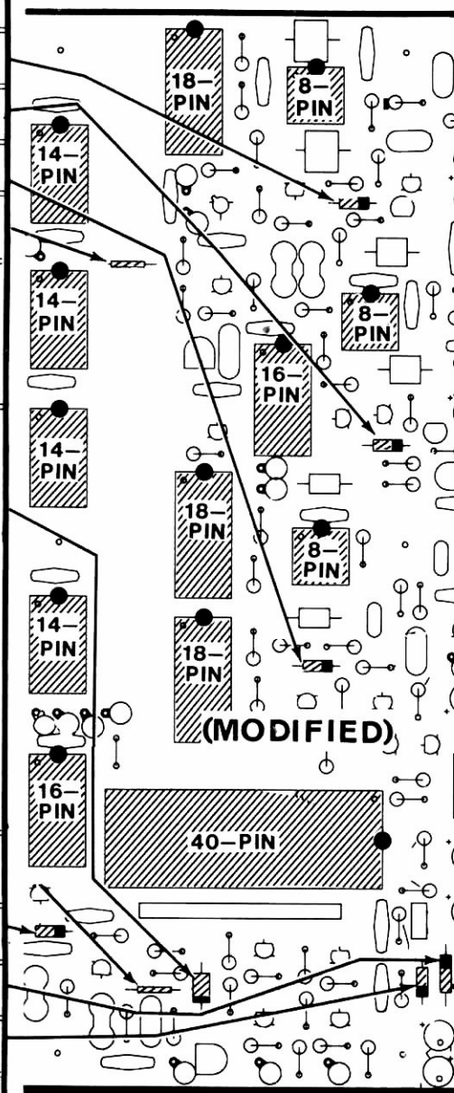
PICTORIAL 10-1
