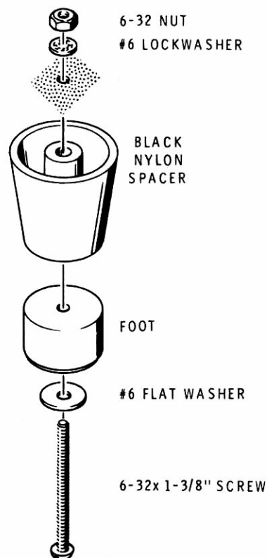
Detail 17-3A
