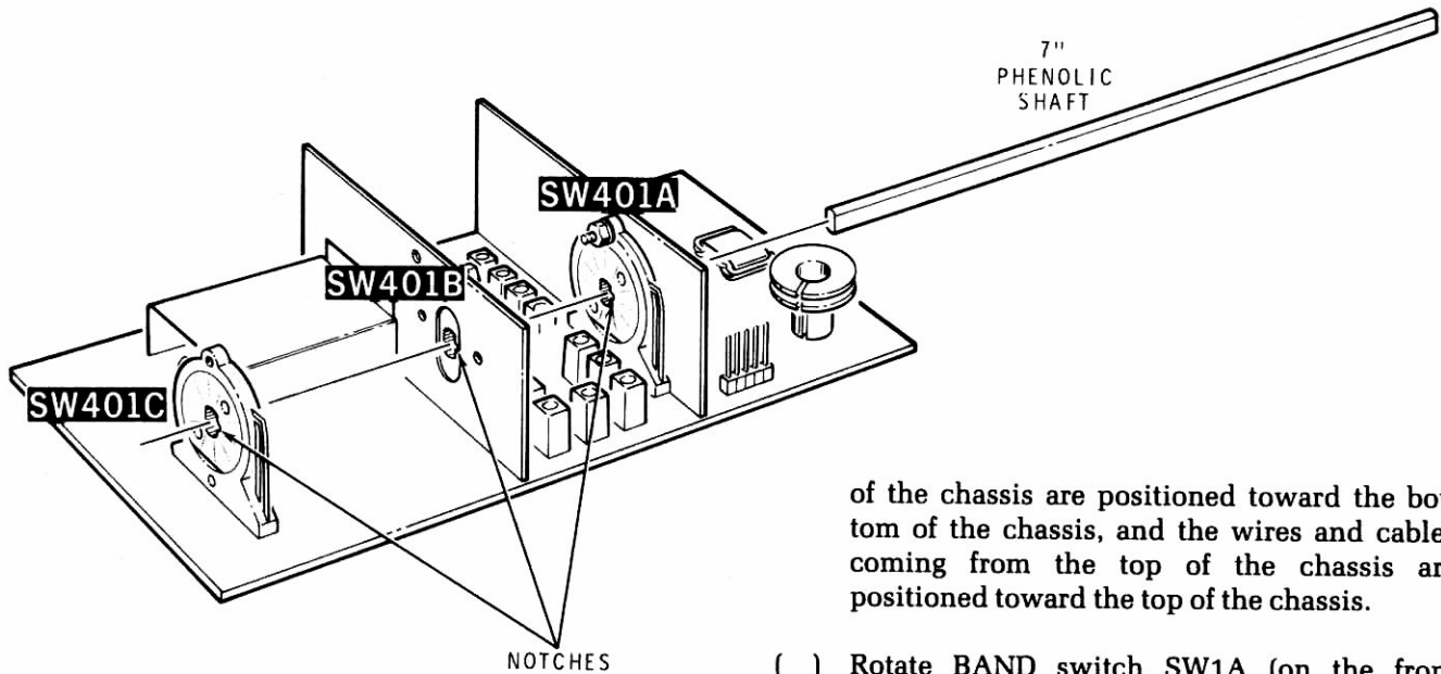
Detail 16-13A
