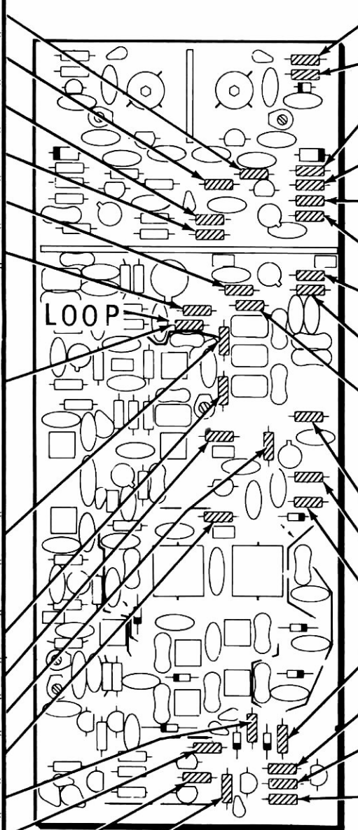
PICTORIAL 11-3
