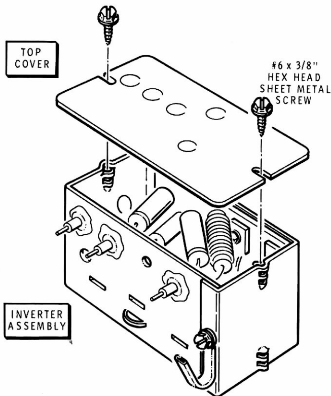
PICTORIAL 7-8
