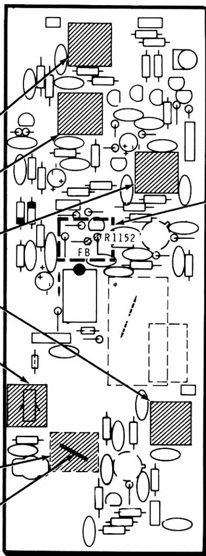
PICTORIAL 8-6
