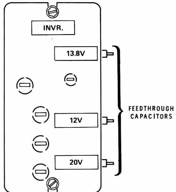
Detail 7-8A
