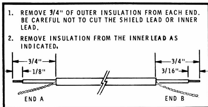
Detail 3-7A
