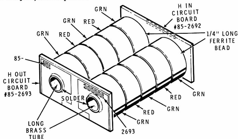
Detail 14-3B
