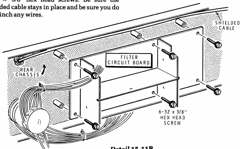
Detail 15-11B
