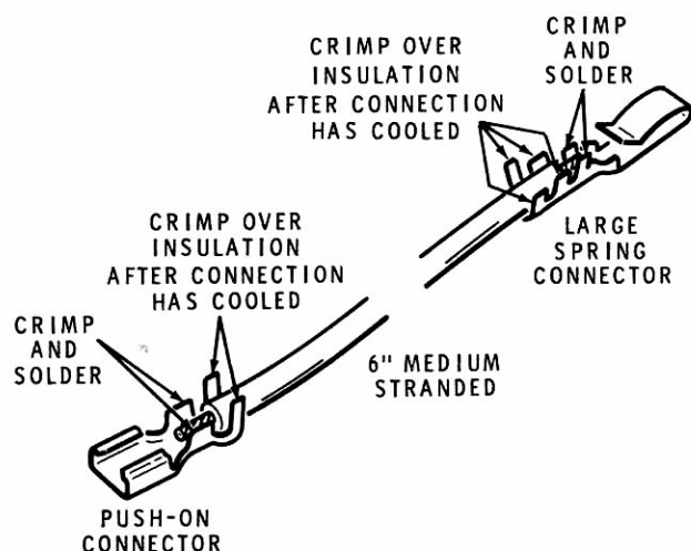
Detail 15-10C
