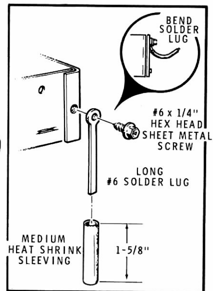
Detail 5-5A
