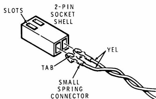
Detail 3-8A
