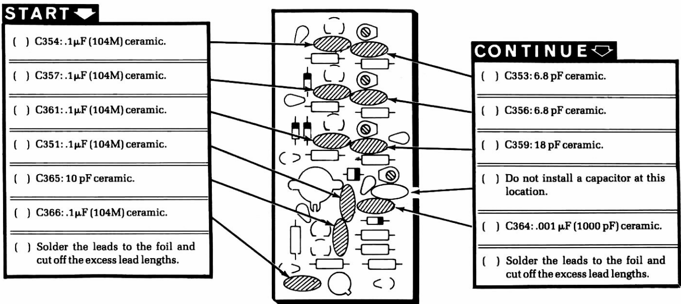
PICTORIAL 5-3
