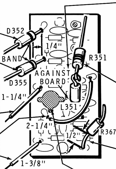
PICTORIAL 5-4
