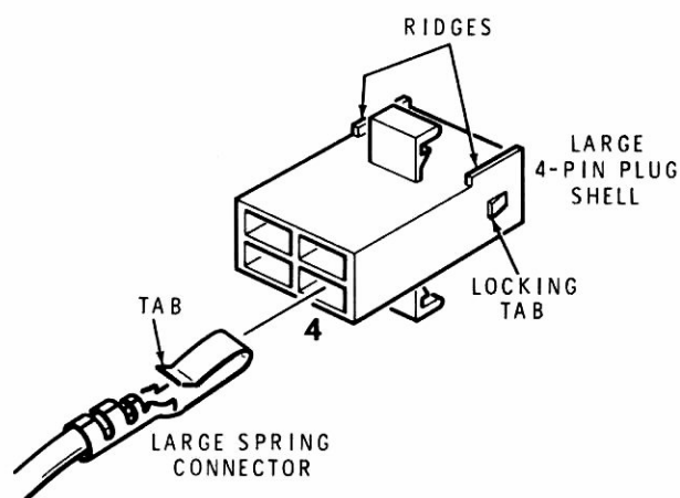
Detail 15-10D
