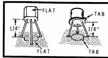
Detail 10-5A
