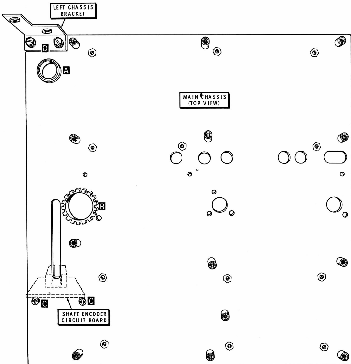
PICTORIAL 15-2
