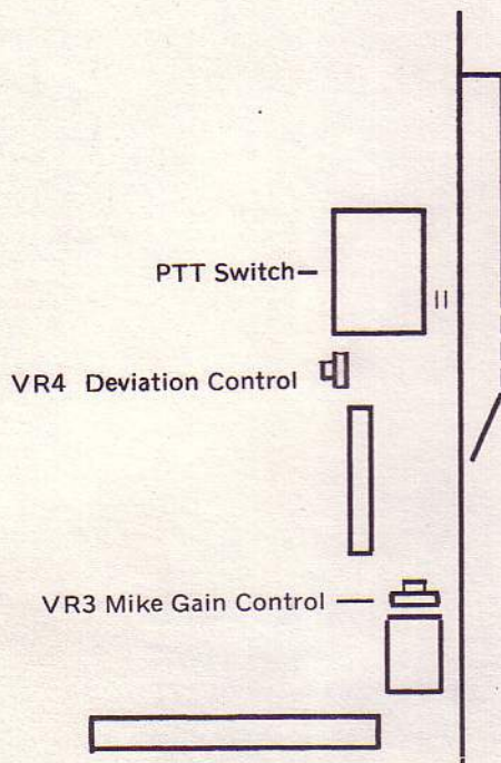
S1 Main Transceiver Board
