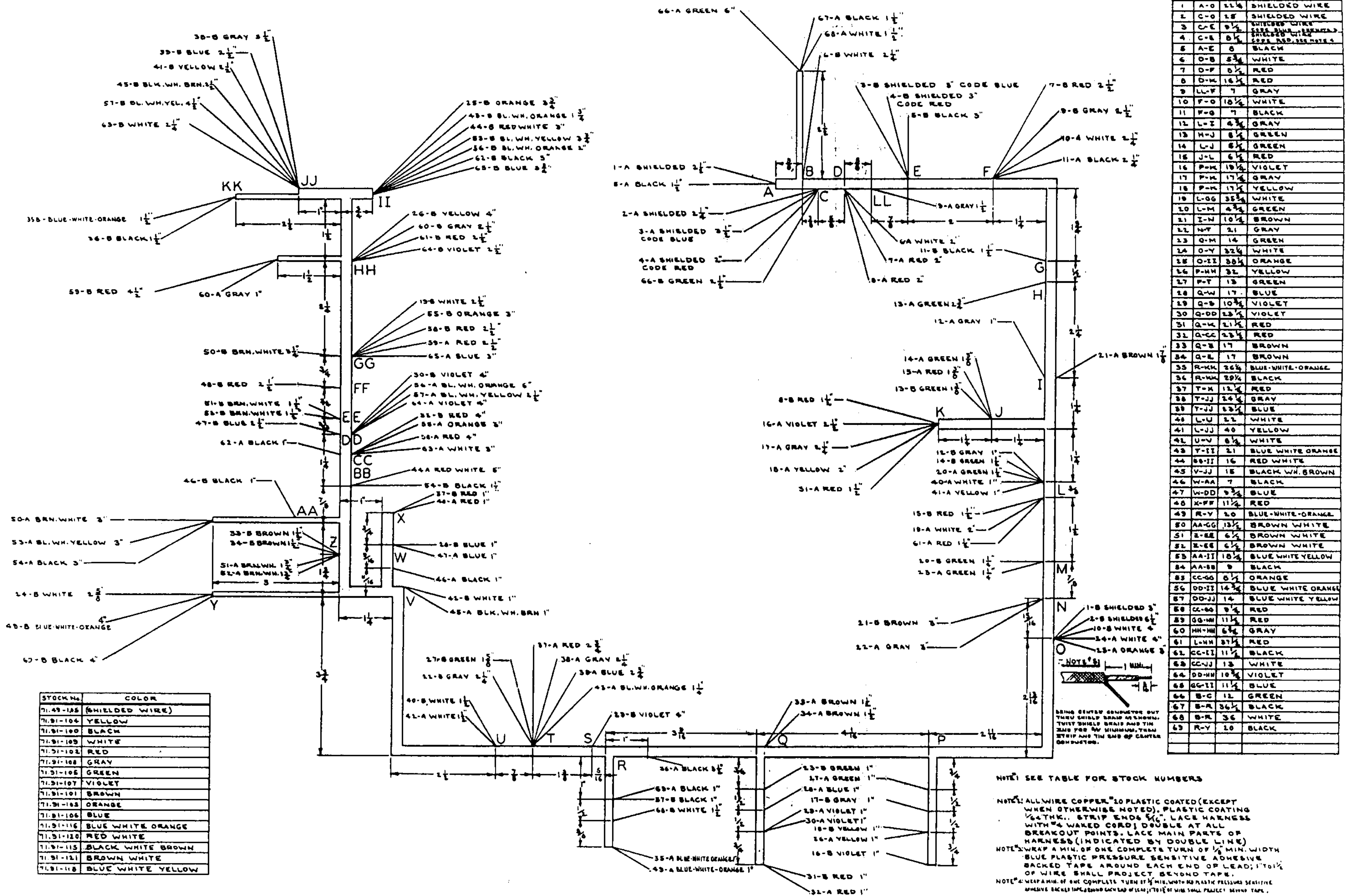
Figure 10, Valiant Wiring Harness
