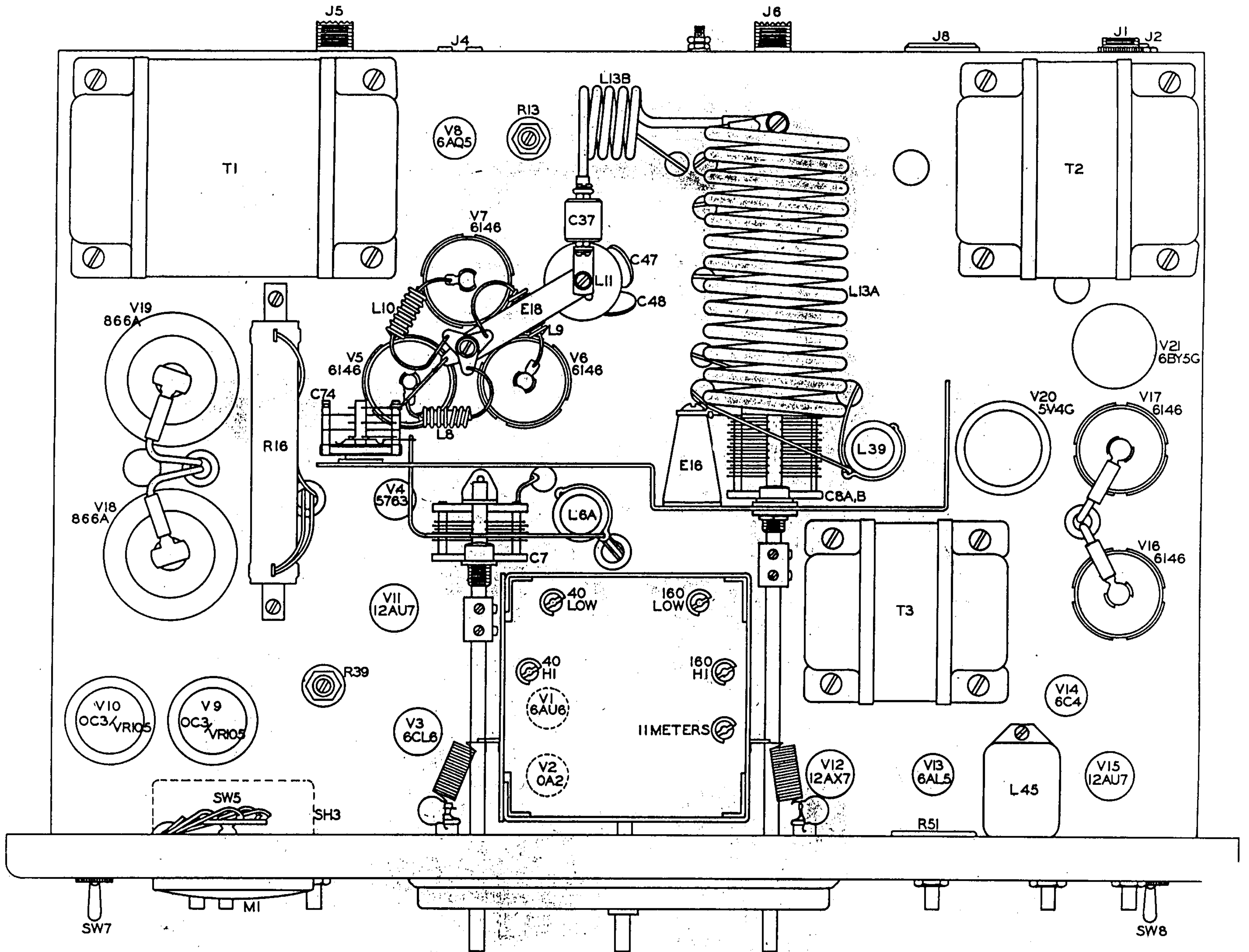
Figure 1, Valiant Tube Layout Guide
