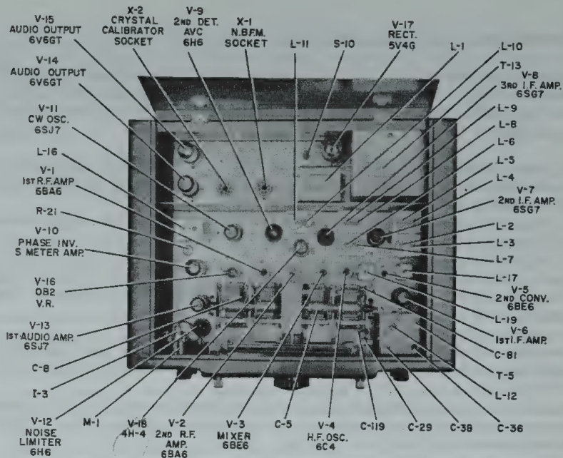
Figure No. 6. Top View of Receiver
