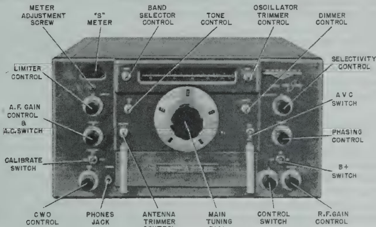
Figure No. 5. Front View of Receiver
