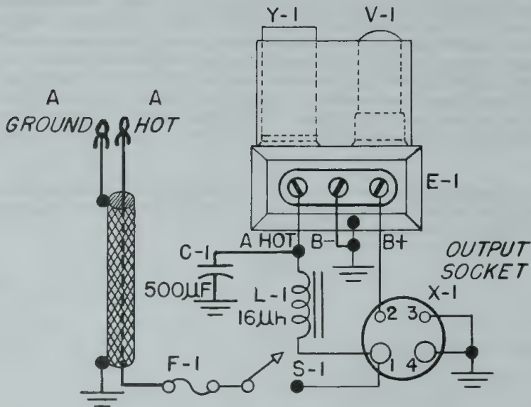
Figure No. 17. Schematic Diagram, 650S Vibrator Power Supply
