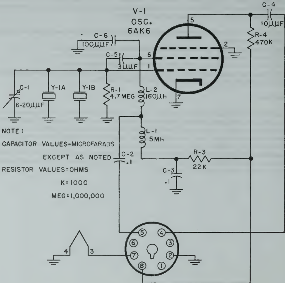
Figure No. 15. Schematic Diagram, XCU-50-2 Calibrator
