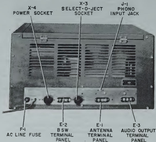
Figure No. 4. Rear View of Receiver
