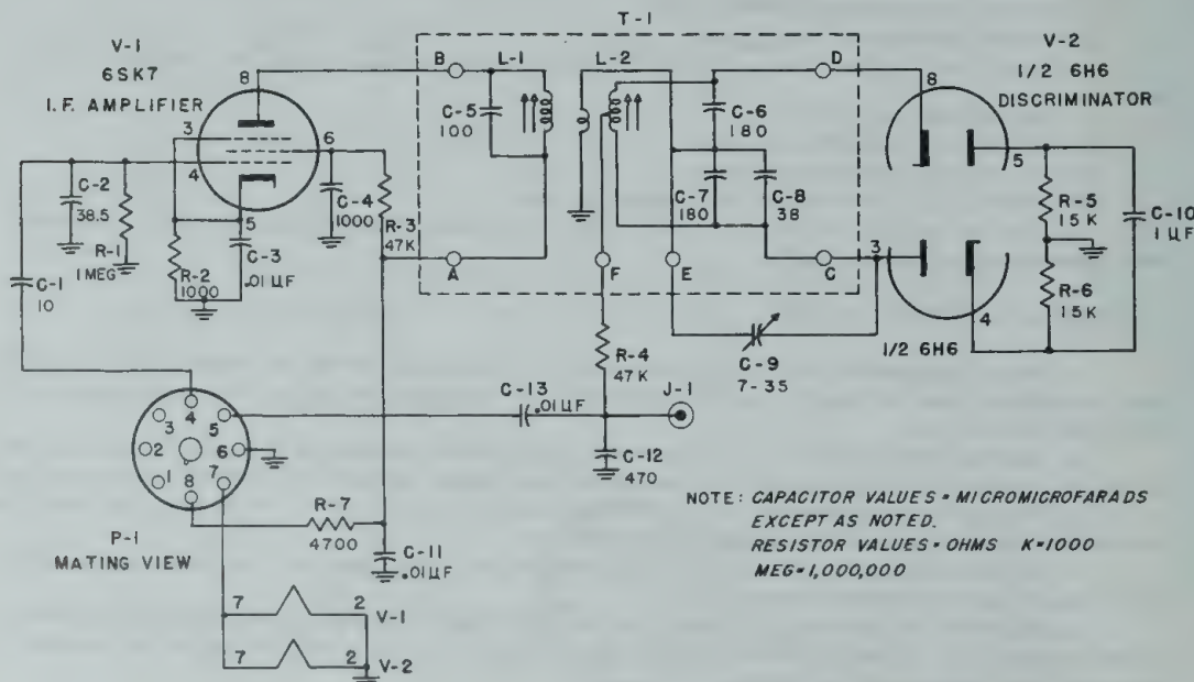
Figure No. 16. Schematic Diagram, NFM-83-50 Adaptor
