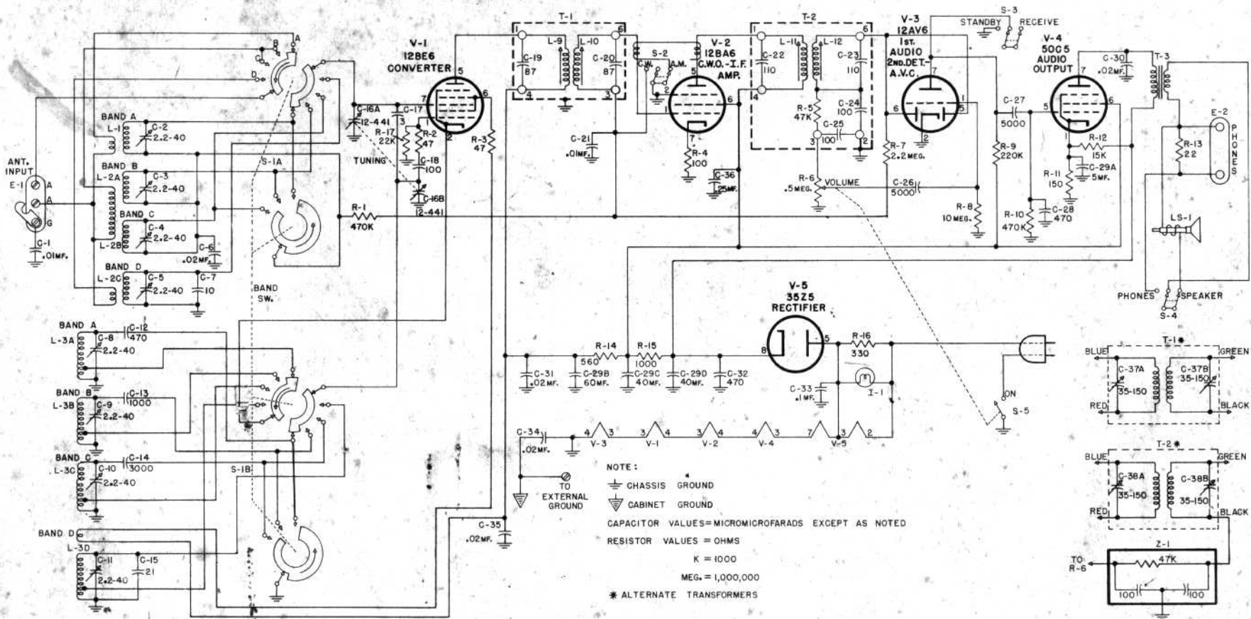
Figure No. 5. Schematic Diagram, SW-54 Receiver
