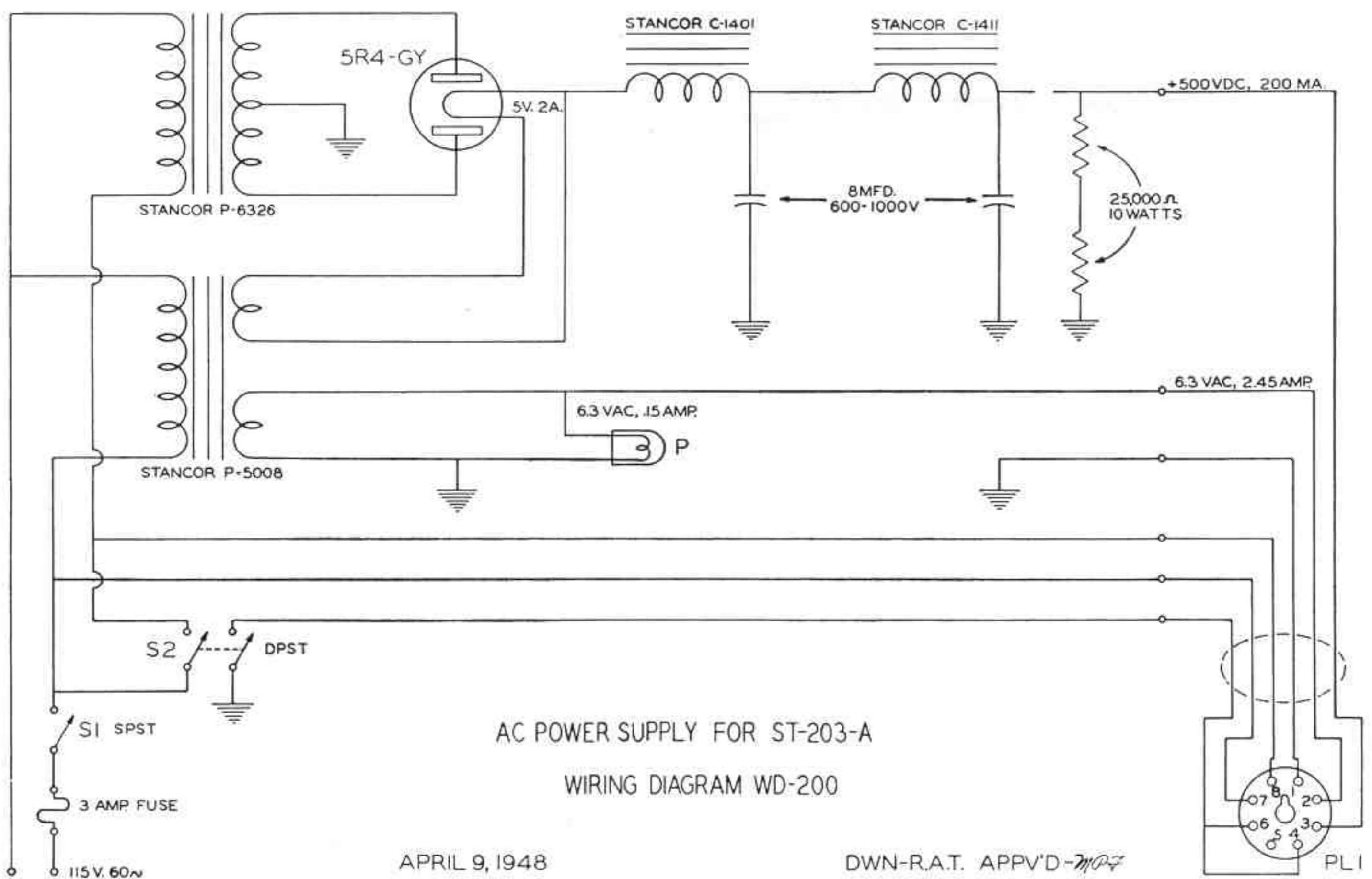
Figure 6. AC Power Supply Schematic Diagram
