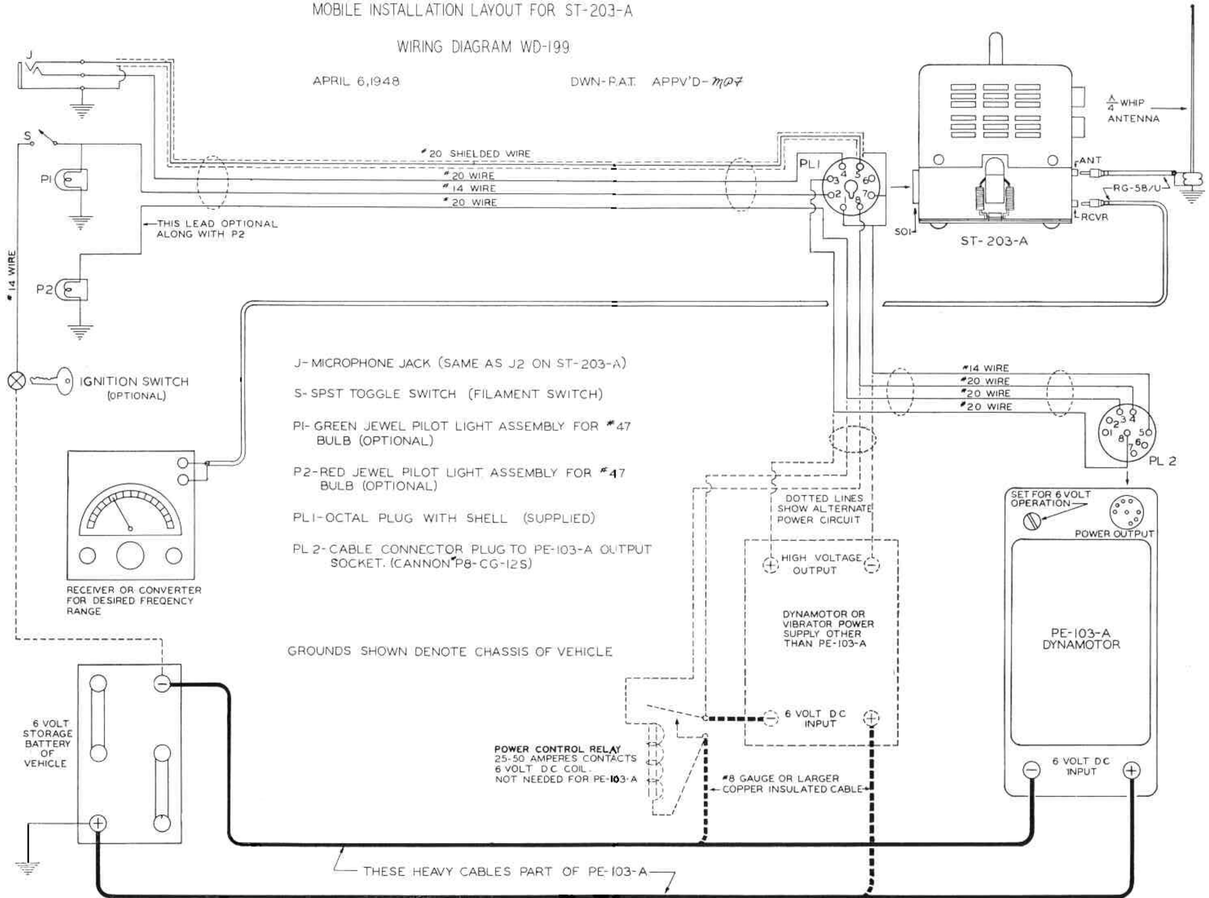
Figure 7. ST-203-A Mobile Installation Diagram
