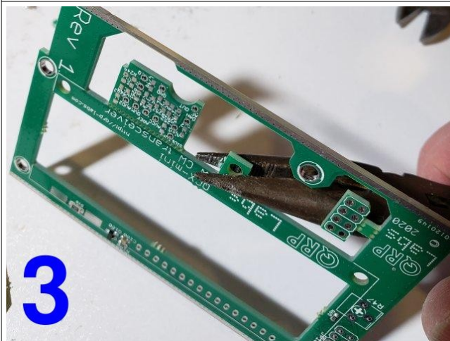
Gently grip and bend to remove – but be careful of the central spar of the panel PCB
