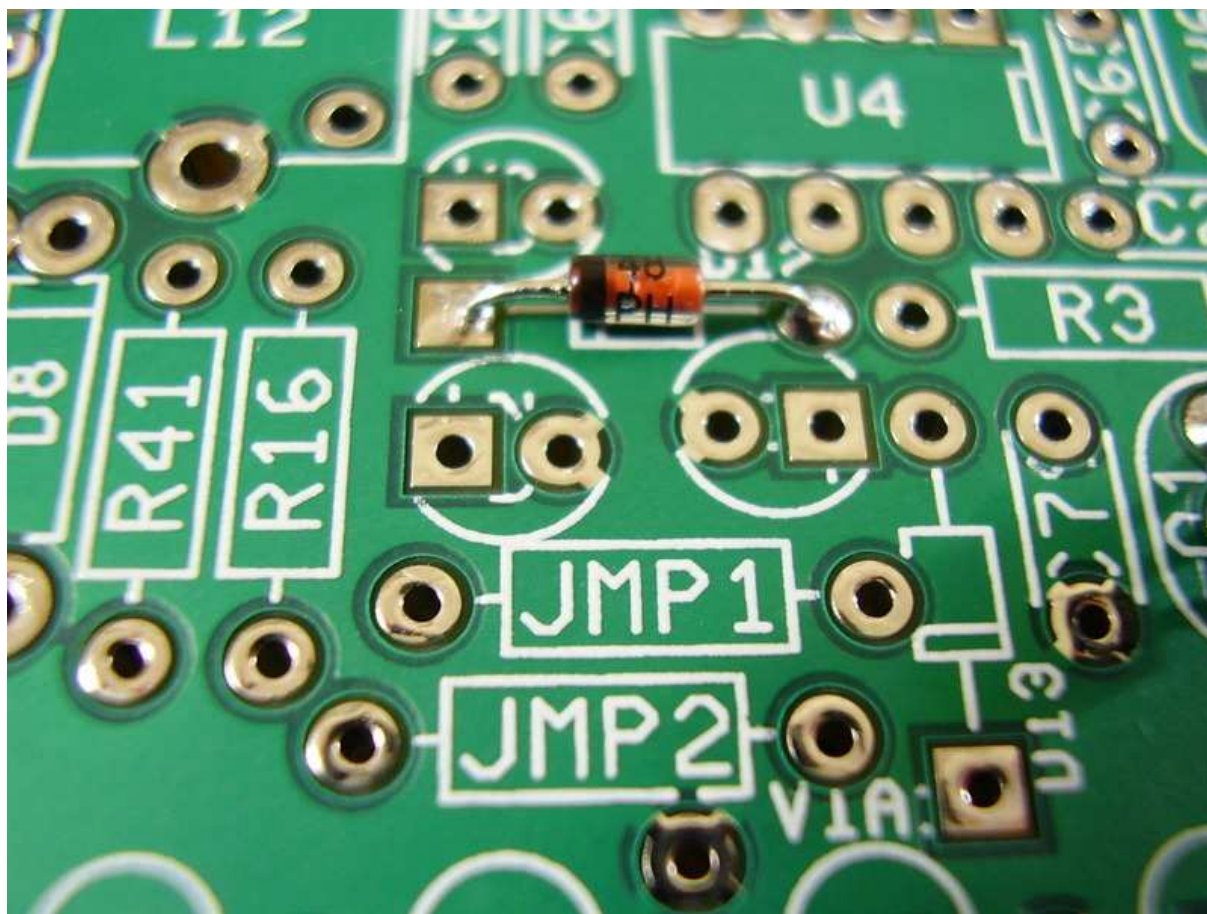
Figure 3.30: C92 Location.
