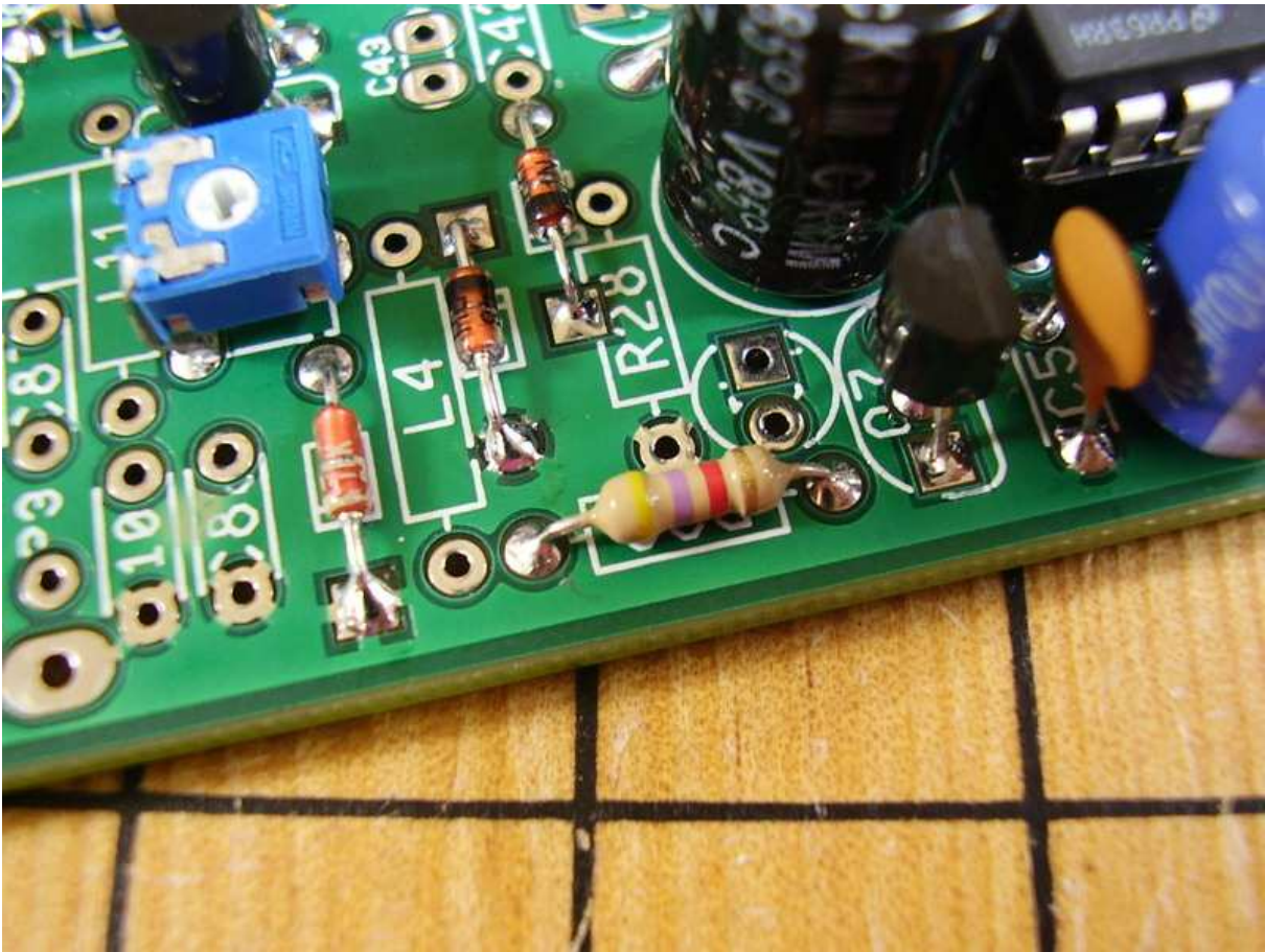
Figure 8.18: [6-15] R29 4.7K.
