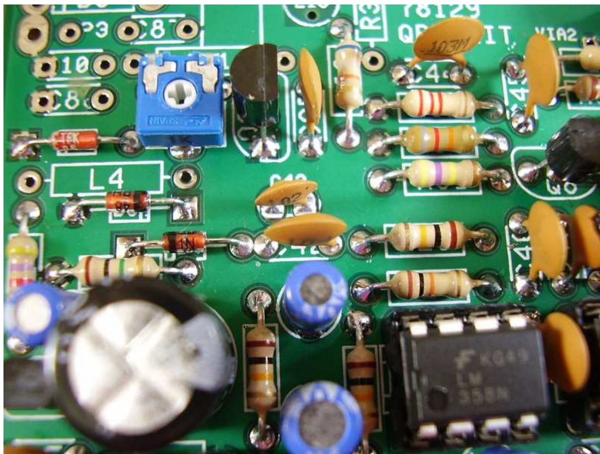
Figure 8.25: [6-22] C42 .01\mu\text{F} (103).
