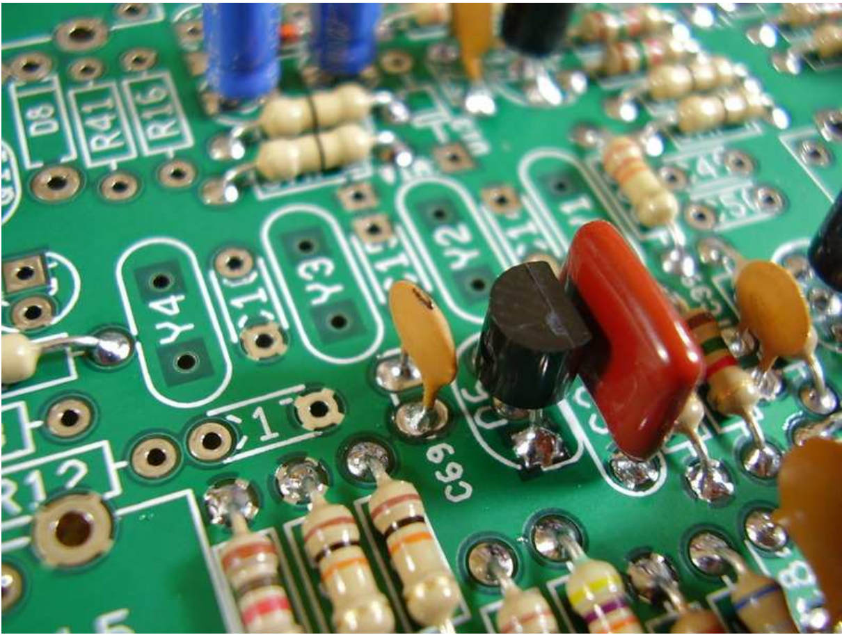
Figure 5.2: [3-2] C69 5pF.
