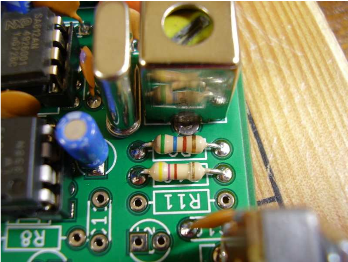
Figure 8.4: [6-4] R9 560 ohms.
