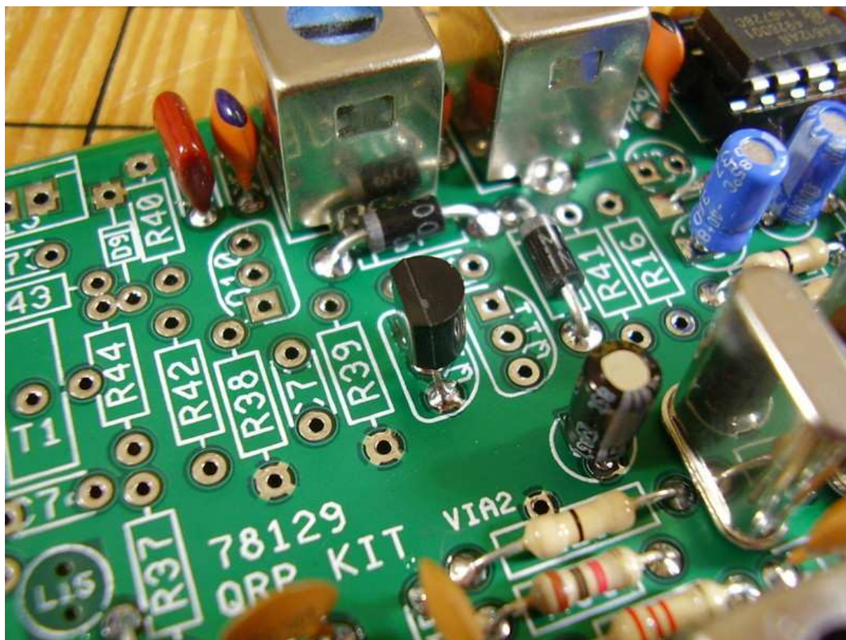
Figure 9.3: [7-3] Q12 2N4126.
