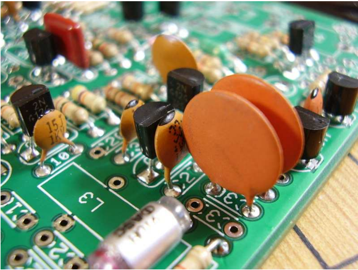
Figure 4.45: [2-42] C27 33pF.
