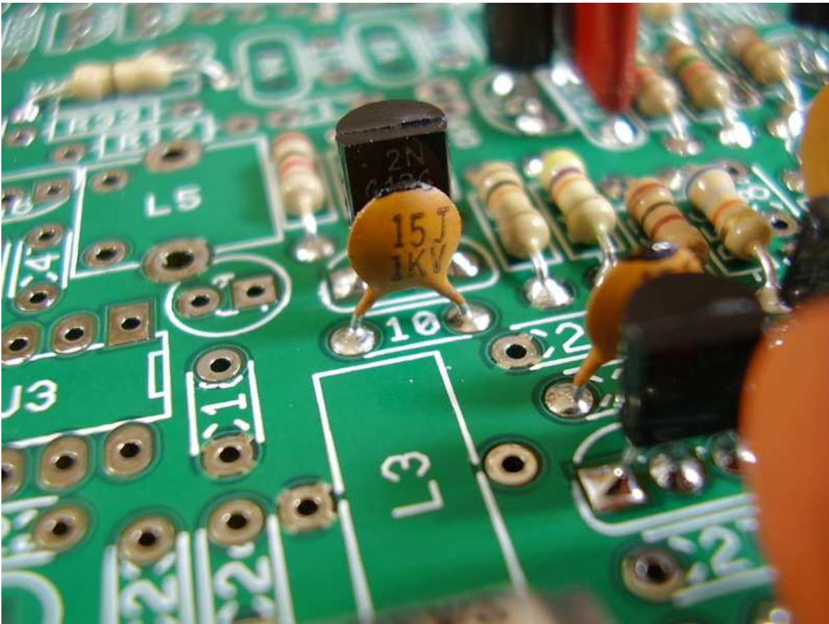
Figure 4.43: [2-40] C101 15pF.
