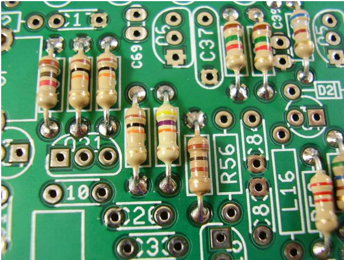
Figure 4.17: [2-19] R14 47K.
