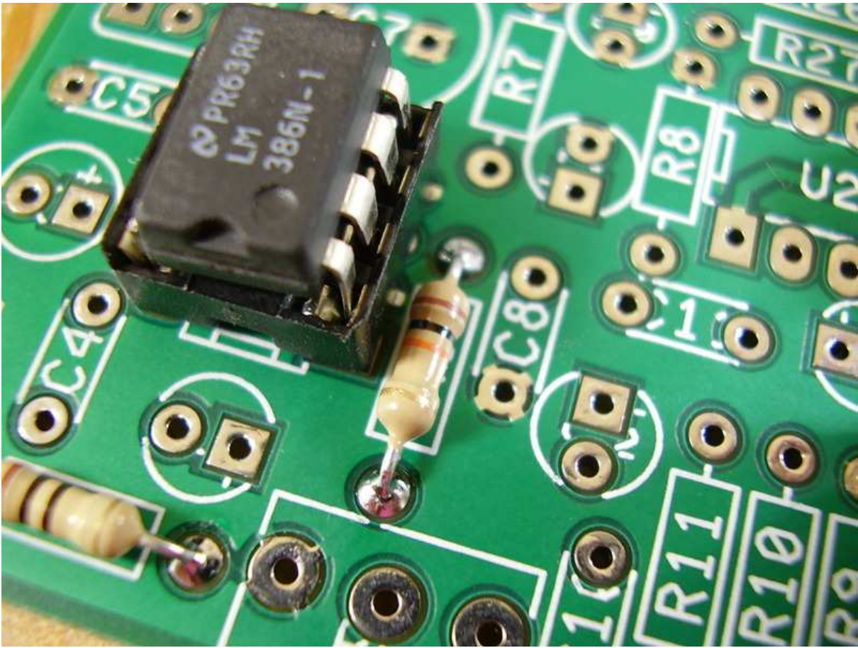
Figure 7.11: [5-13] R5 10K.
