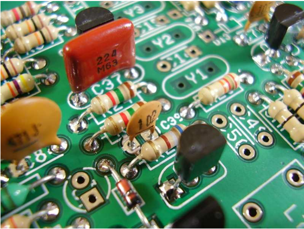
Figure 4.49: [2-46] C39 .001\mu\text{F} .
