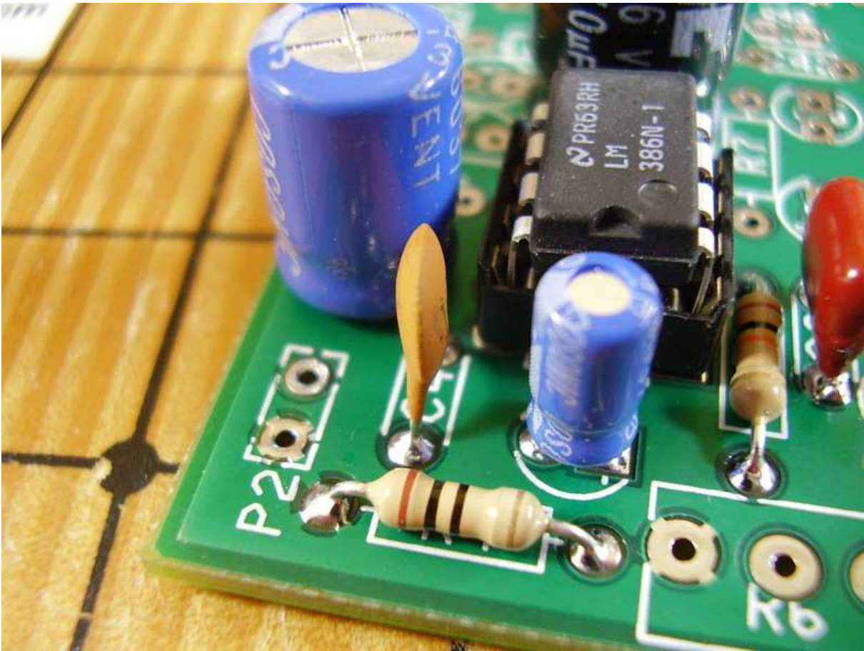
Figure 7.16: [5-18] C4 .1\mu\text{F} (104).
