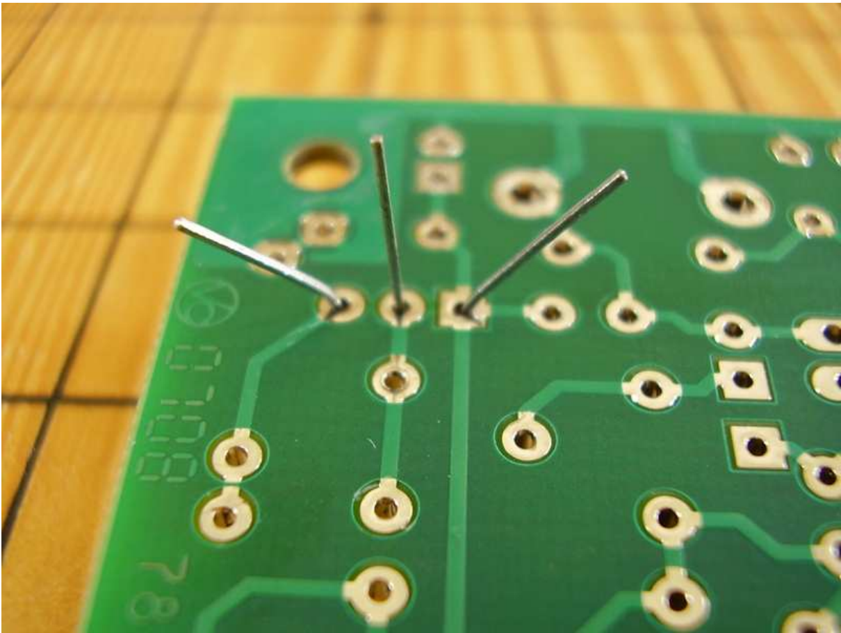
Figure 3.17: 45 Degree Bends.
