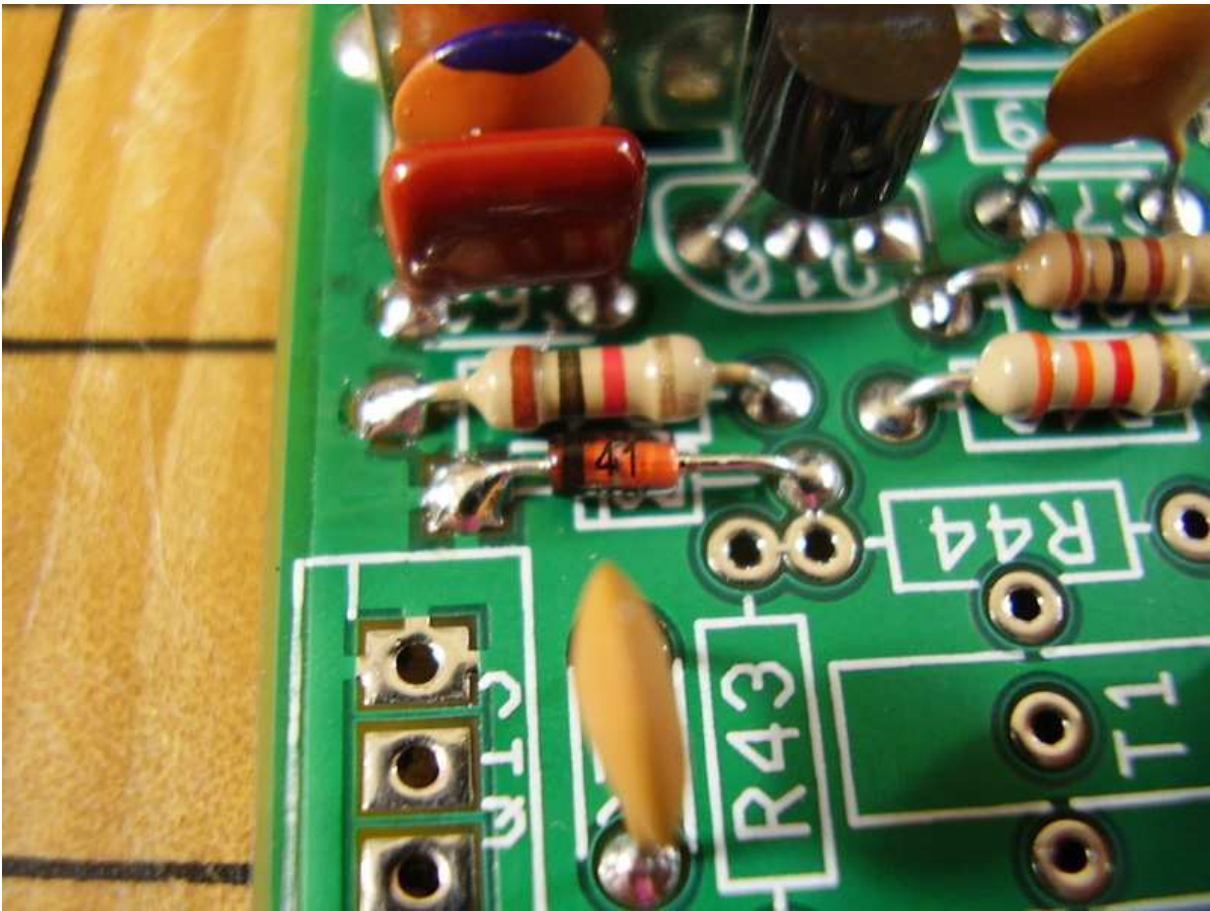
Figure 9.16: [7-17] D9 1N4148.
