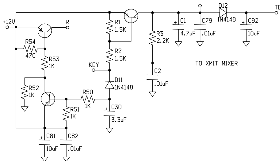
Figure 3.1: Phase 1.0 Schematic.
