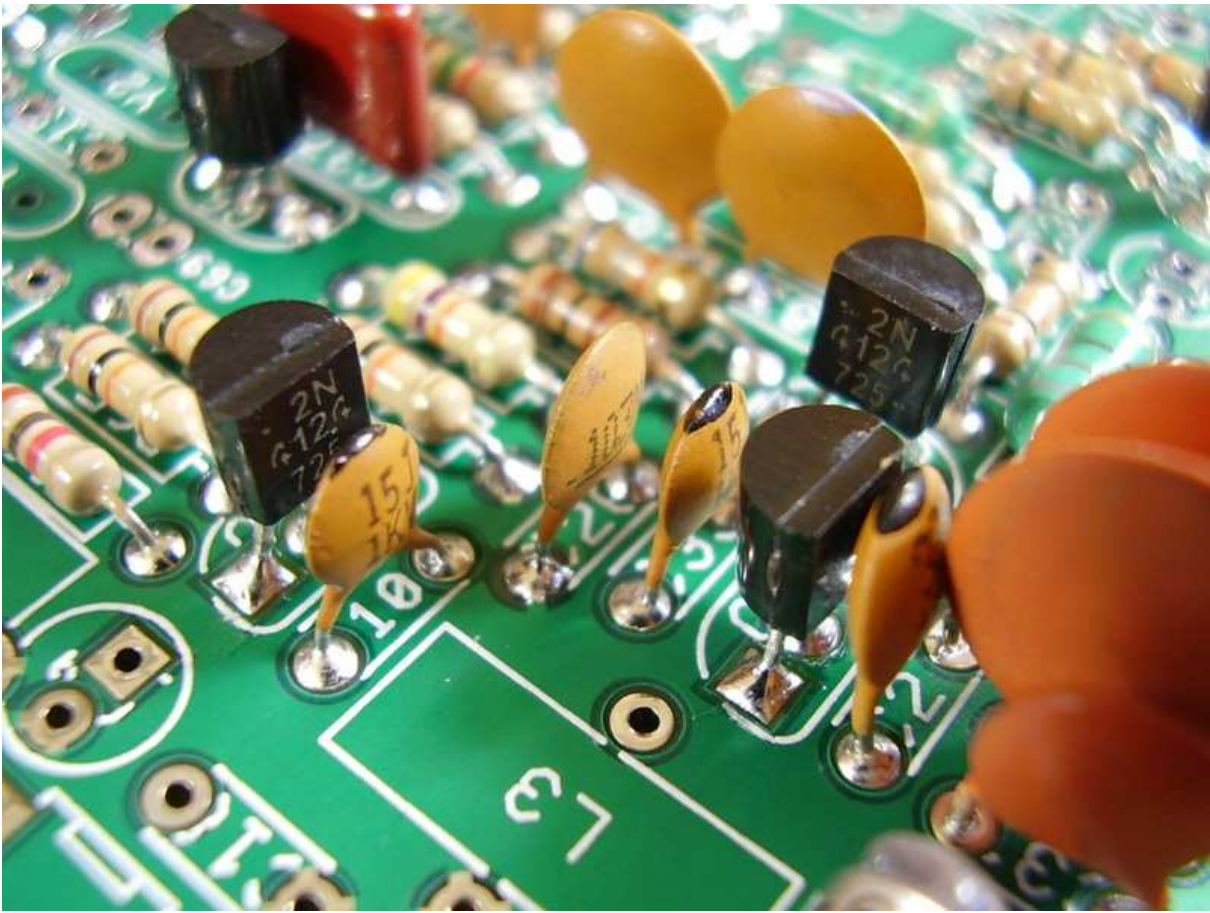
Figure 4.50: [2-47] C26 .01\mu\text{F} .
