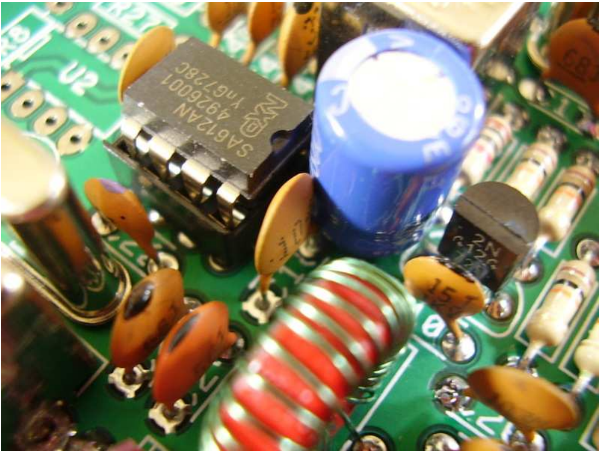
Figure 7.8: [5-10] C18 .1\mu\text{F} (104).
