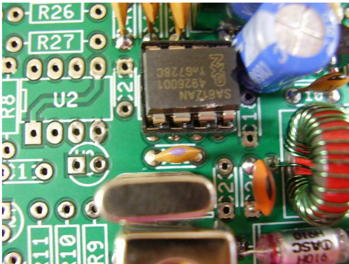
Figure 7.5: [5-6] C24 56pF.
