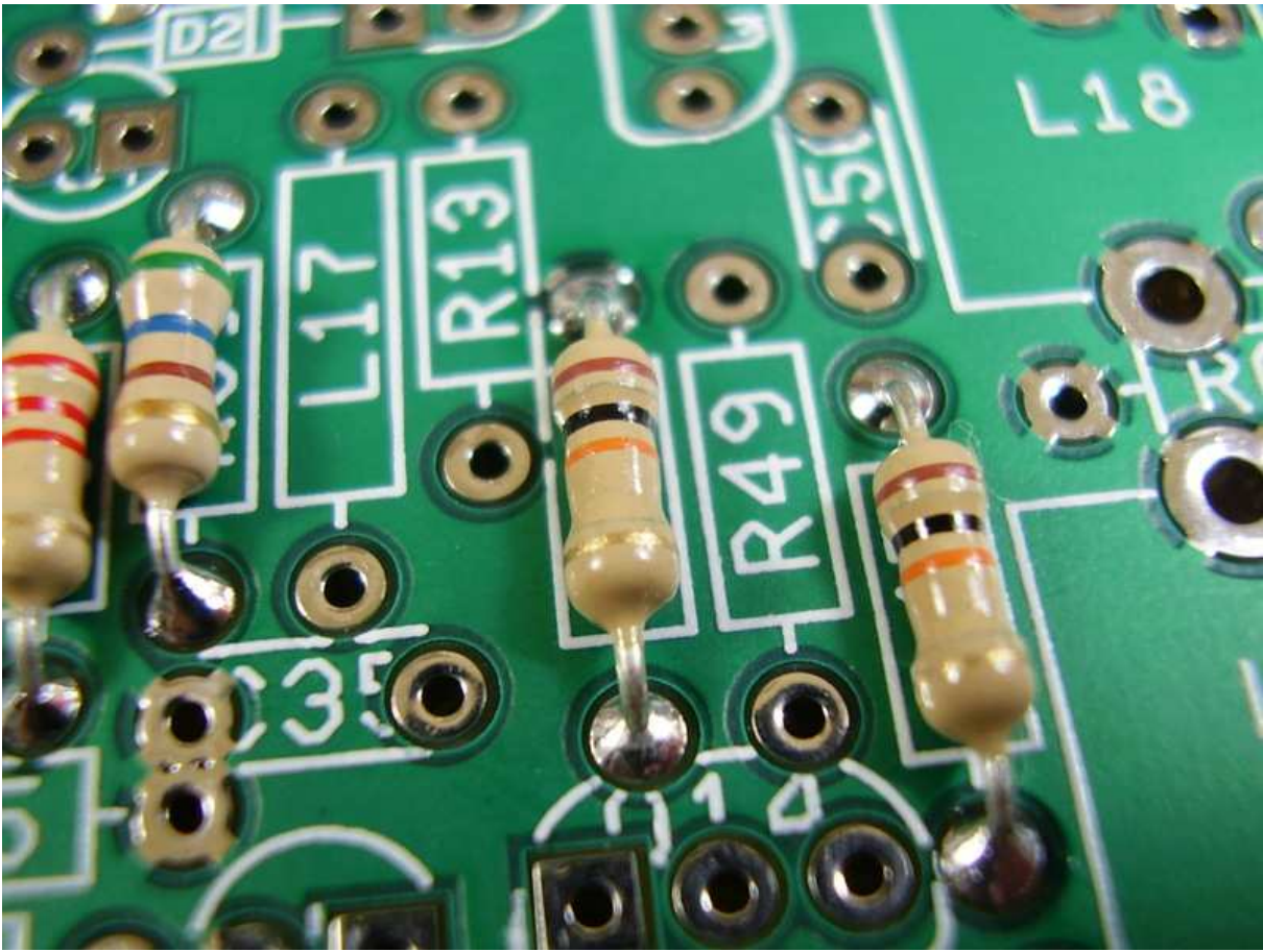
Figure 4.12: [2-14] R48 10K.
