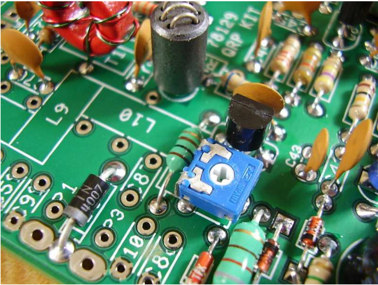
Figure 9.22: [7-24] L11 100\mu\text{H} .
