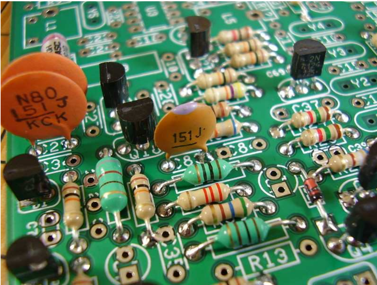
Figure 4.40: [2-37] C83 150pF NP0 Disc Cap.
