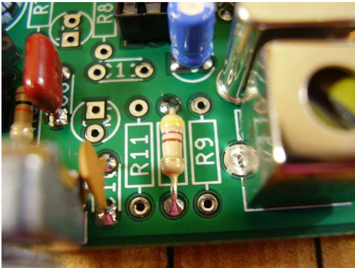
Figure 8.3: [6-3] R10 470 ohms.
