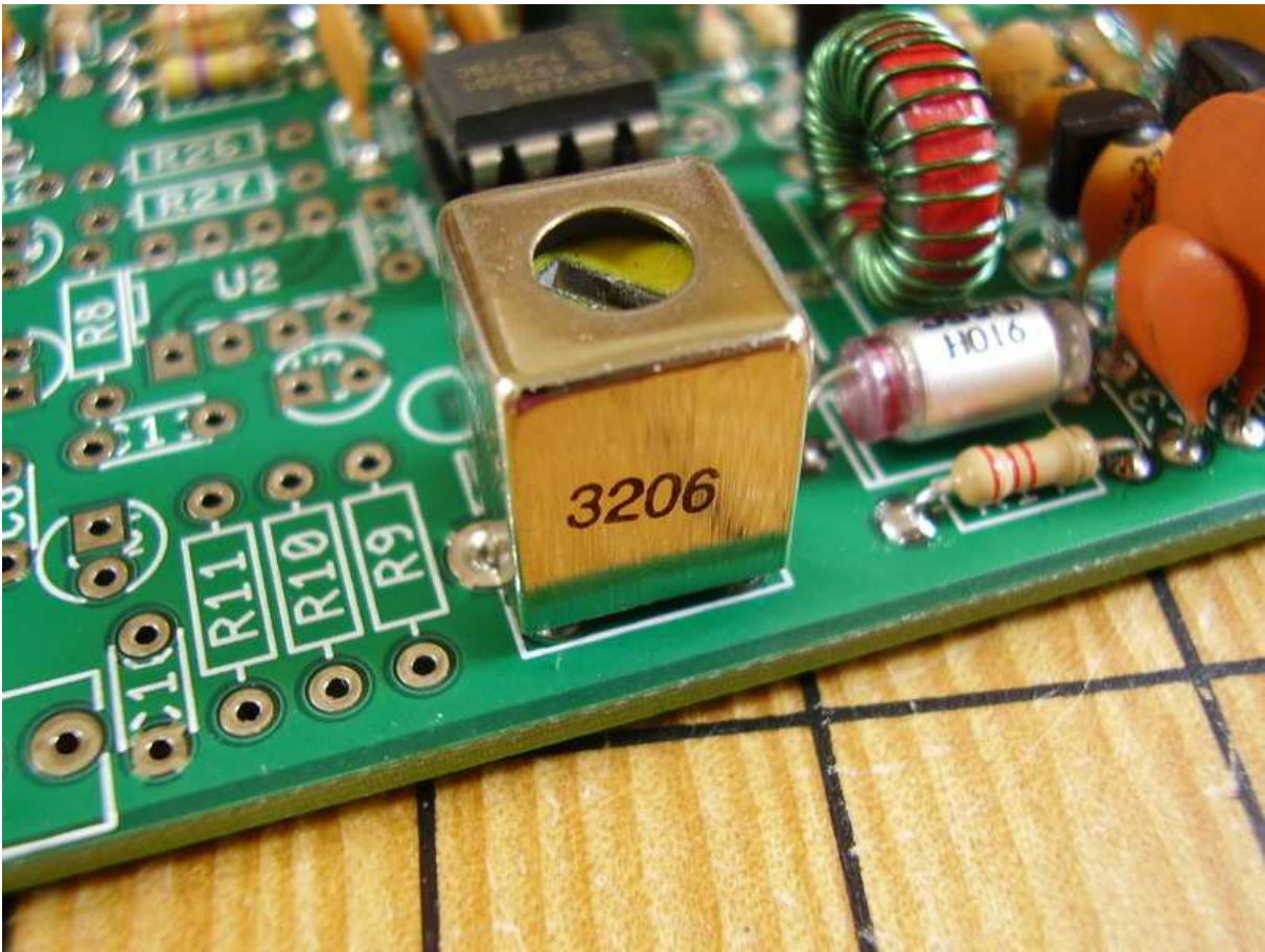
Figure 7.2: [5-3] L1 1.3\mu\text{H} (3206).
