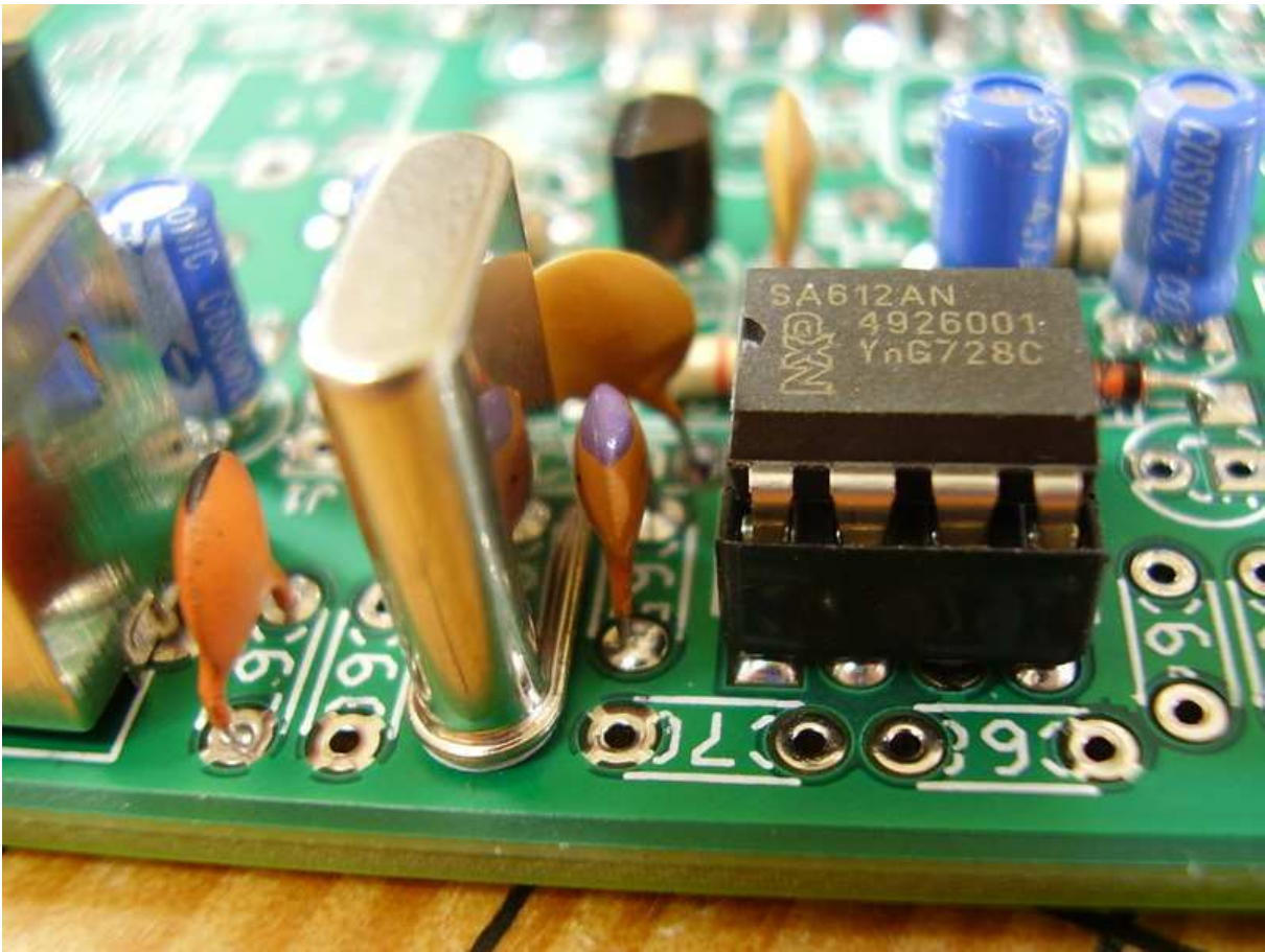
Figure 5.10: [3-7] C65 47pF.
