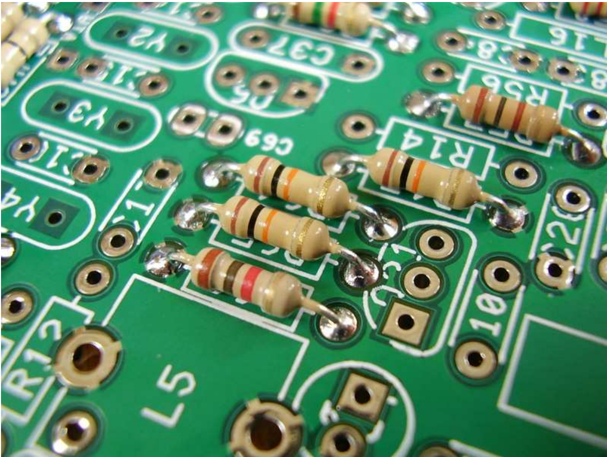
Figure 4.15: [2-17] R65 10K.
