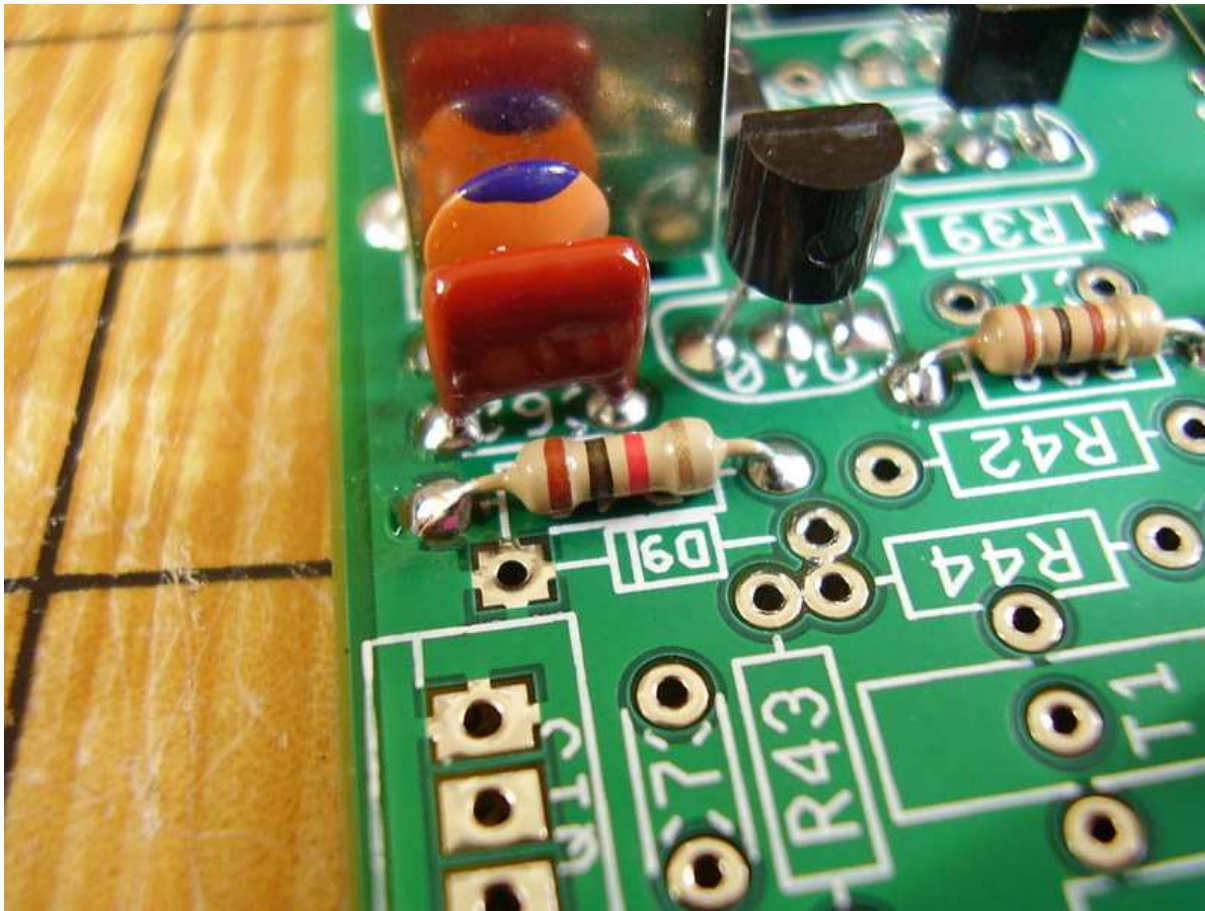
Figure 9.9: [7-9] R40 1K.
