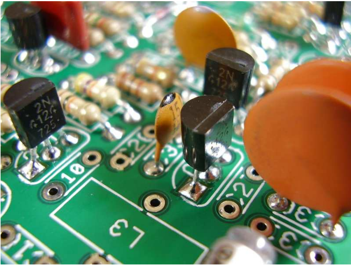
Figure 4.42: [2-39] C33 15pF.
