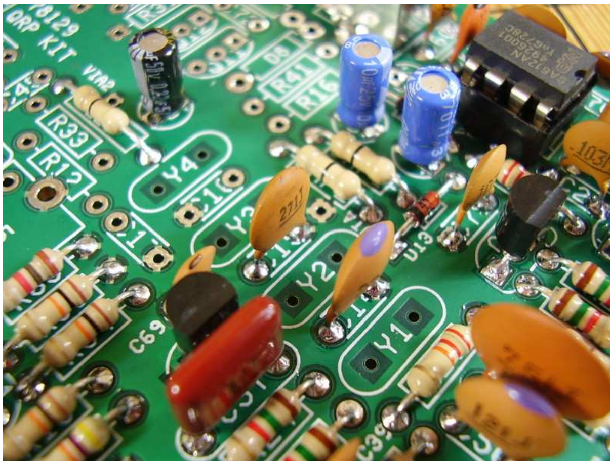
Figure 6.29: [4-31] C15 270pF (271).
