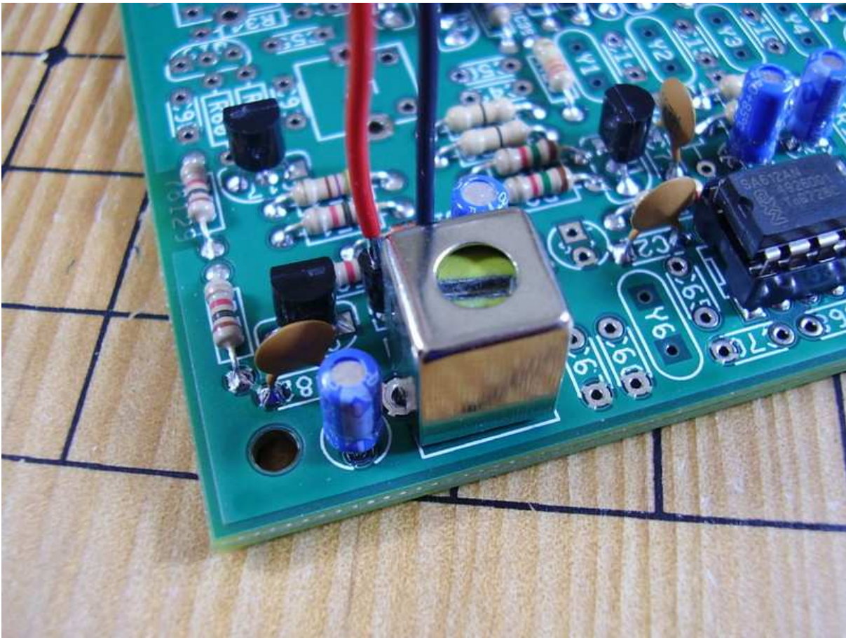
Figure 5.5: [3-3] L14 1.3 \mu H Shielded Coil.
