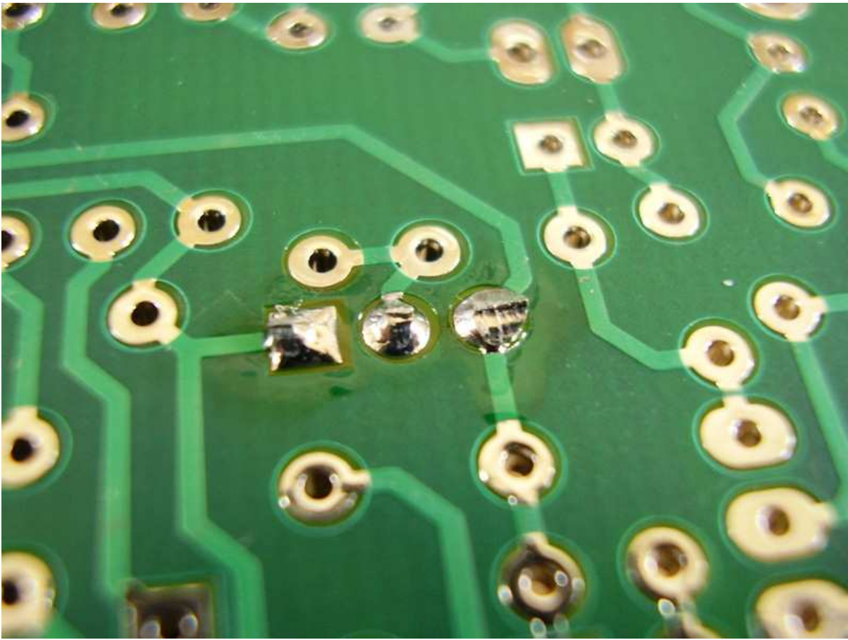
Figure 3.10: Cut Leads .
