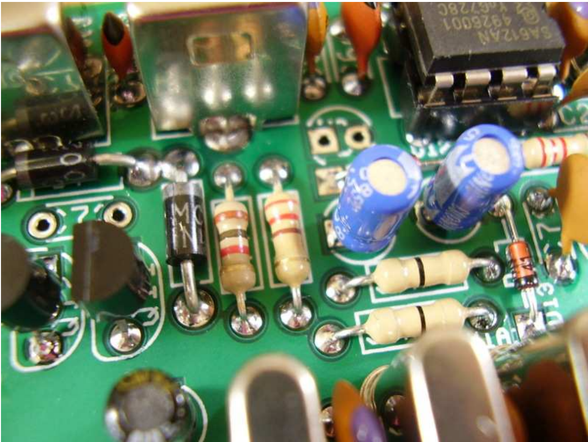
Figure 9.10: [7-10] R41 1K.
