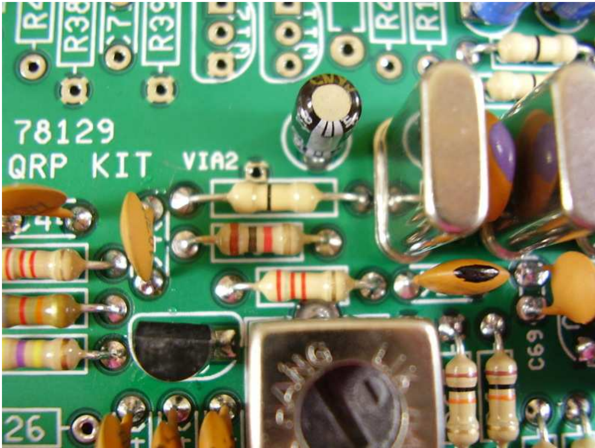
Figure 7.1: [5-2] R12 2.2K.
