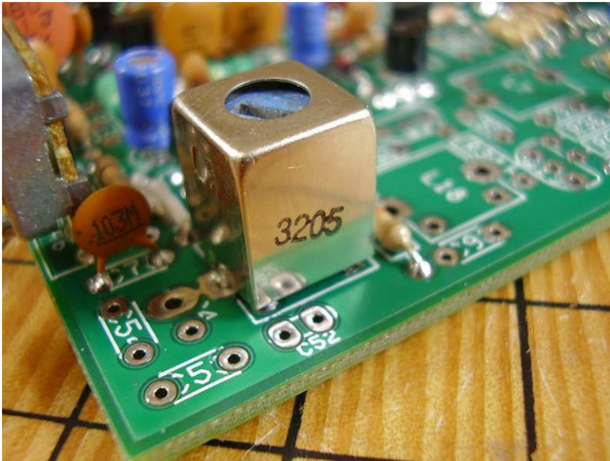
Figure 6.3: [4-1] L6 2.8\mu\text{H} (3205).
