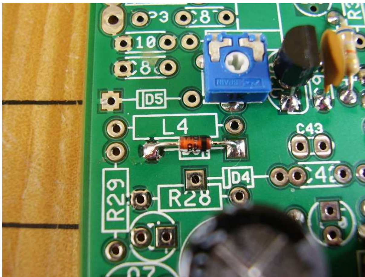
Figure 8.13: [6-11] D3 1N4148.
