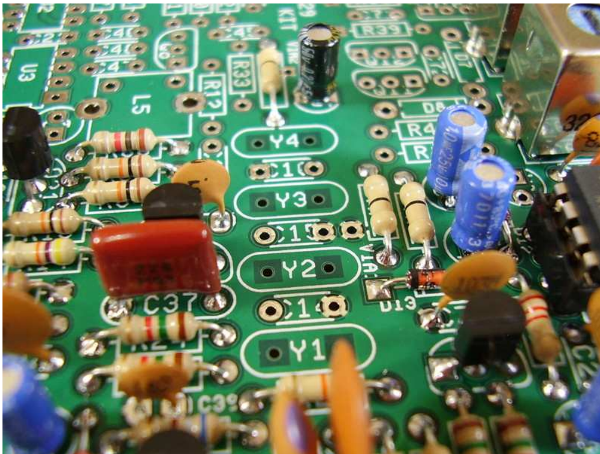
Figure 6.27: Crystal Filter Area of Board.
