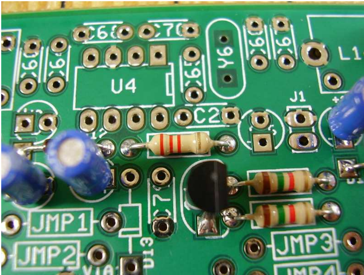
Figure 3.42: [1-13] R3.
