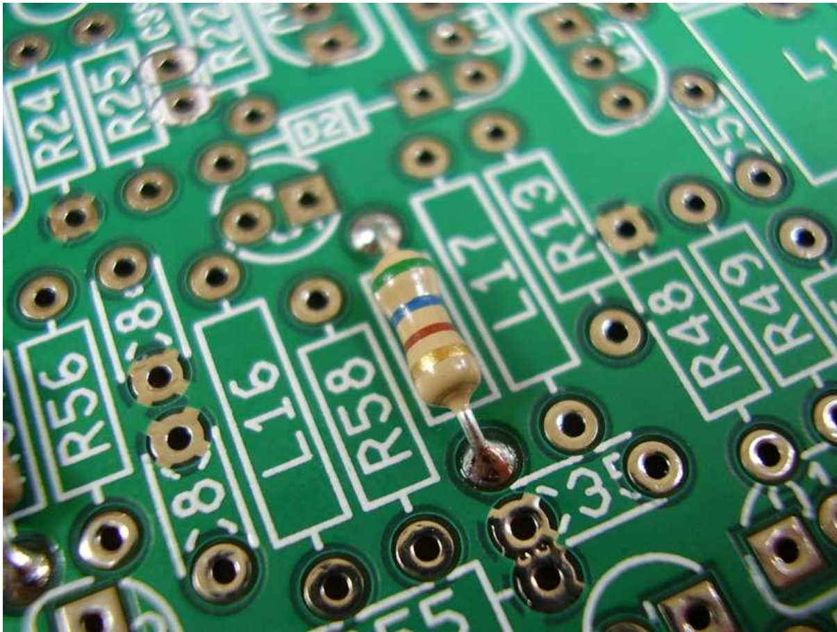
Figure 4.1: [2-3] R59 560 Ohms.
