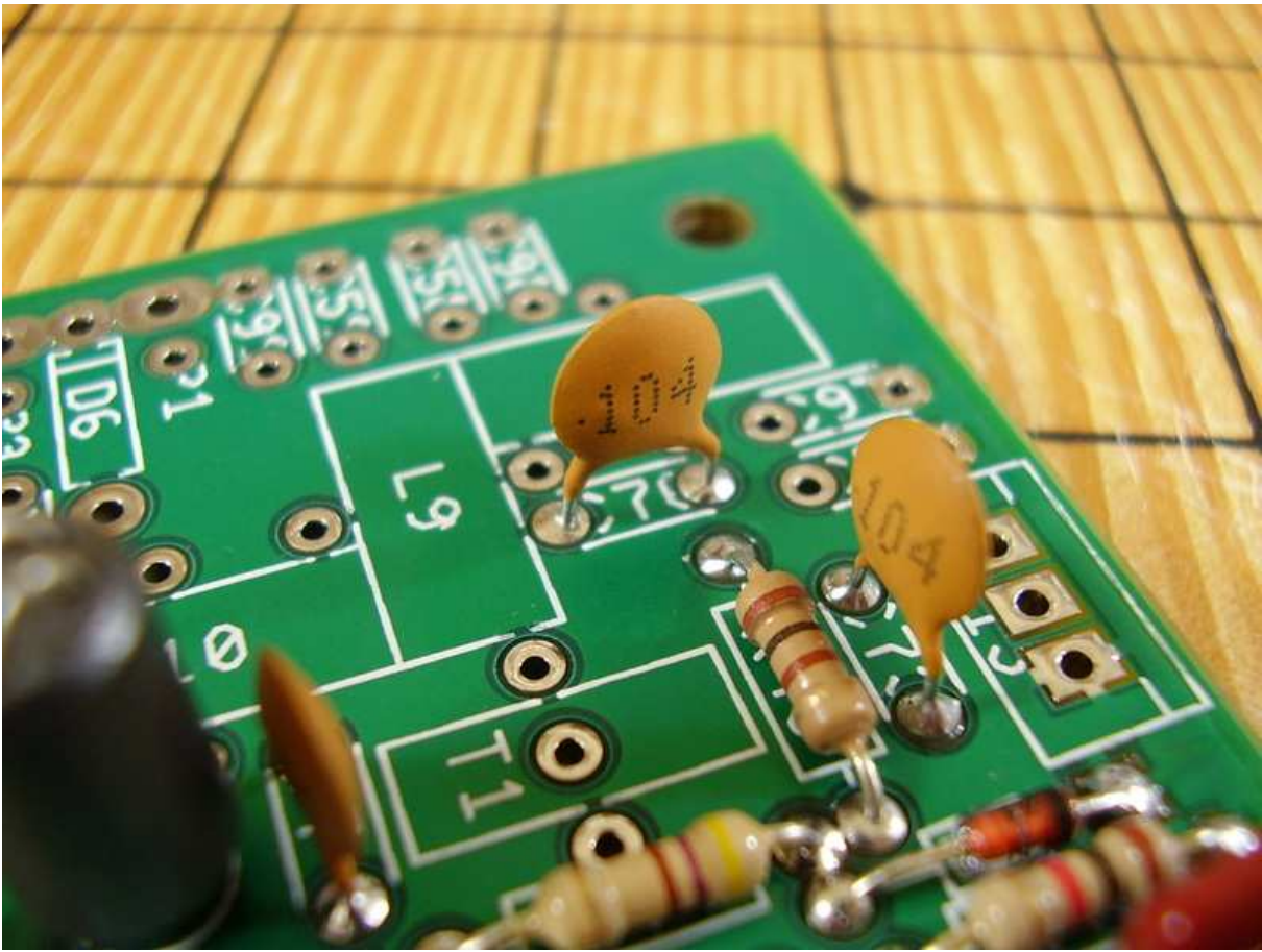
Figure 9.19: [7-20] C76 .1\mu\text{F} .
