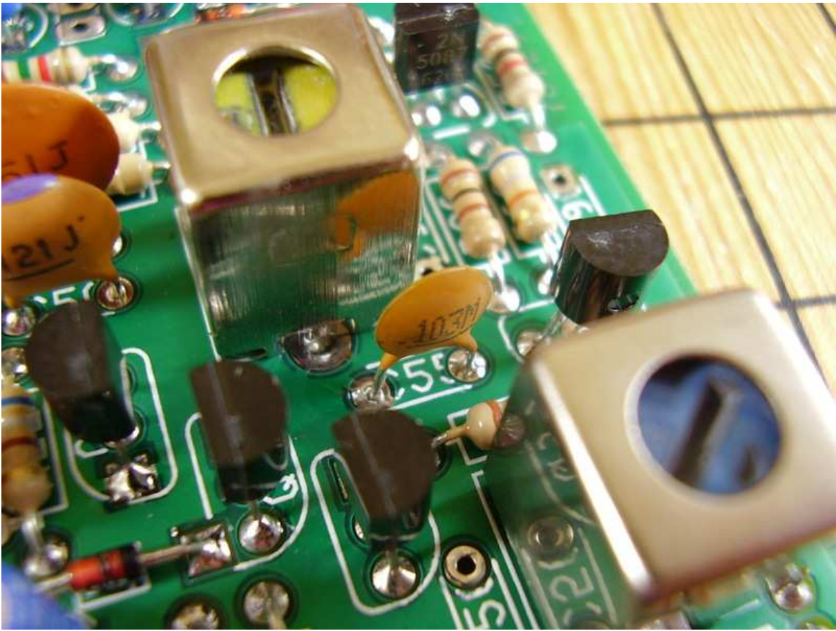
Figure 6.22: [4-20] C55 .01\mu\text{F} (103).
