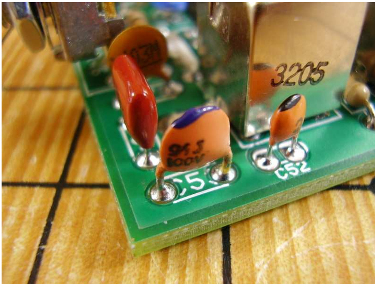
Figure 6.21: [4-19] C53 91pF.
