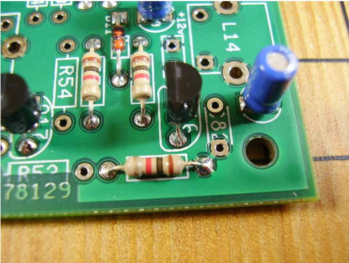
Figure 3.45: [1-16] R52.
