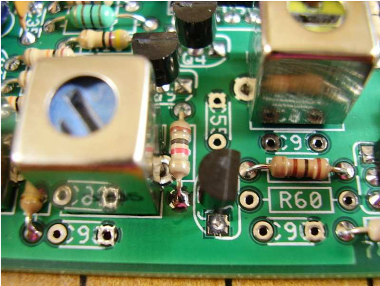
Figure 6.12: [4-9] R34 1K.
