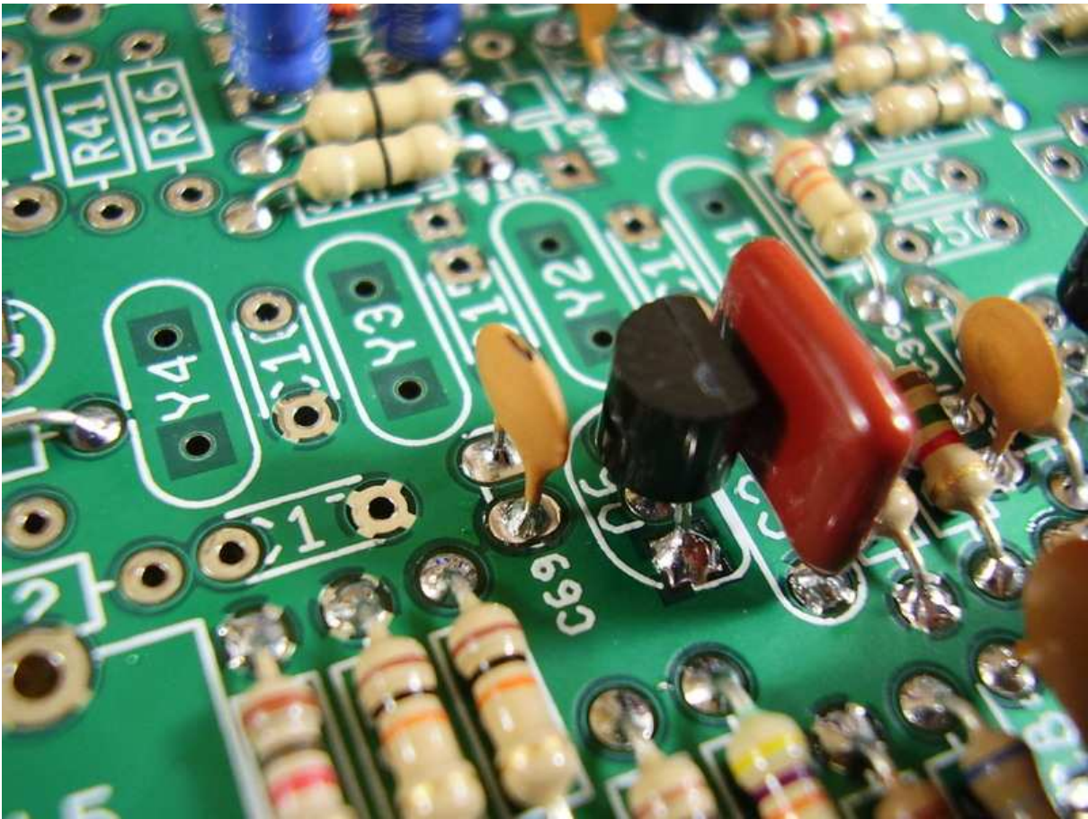
Figure 5.1: [3-2] C69 5pF.
