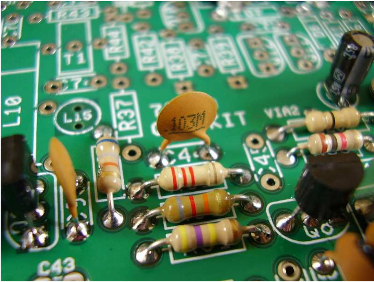
Figure 6.44: [4-43] C44 .01\mu\text{F} .
