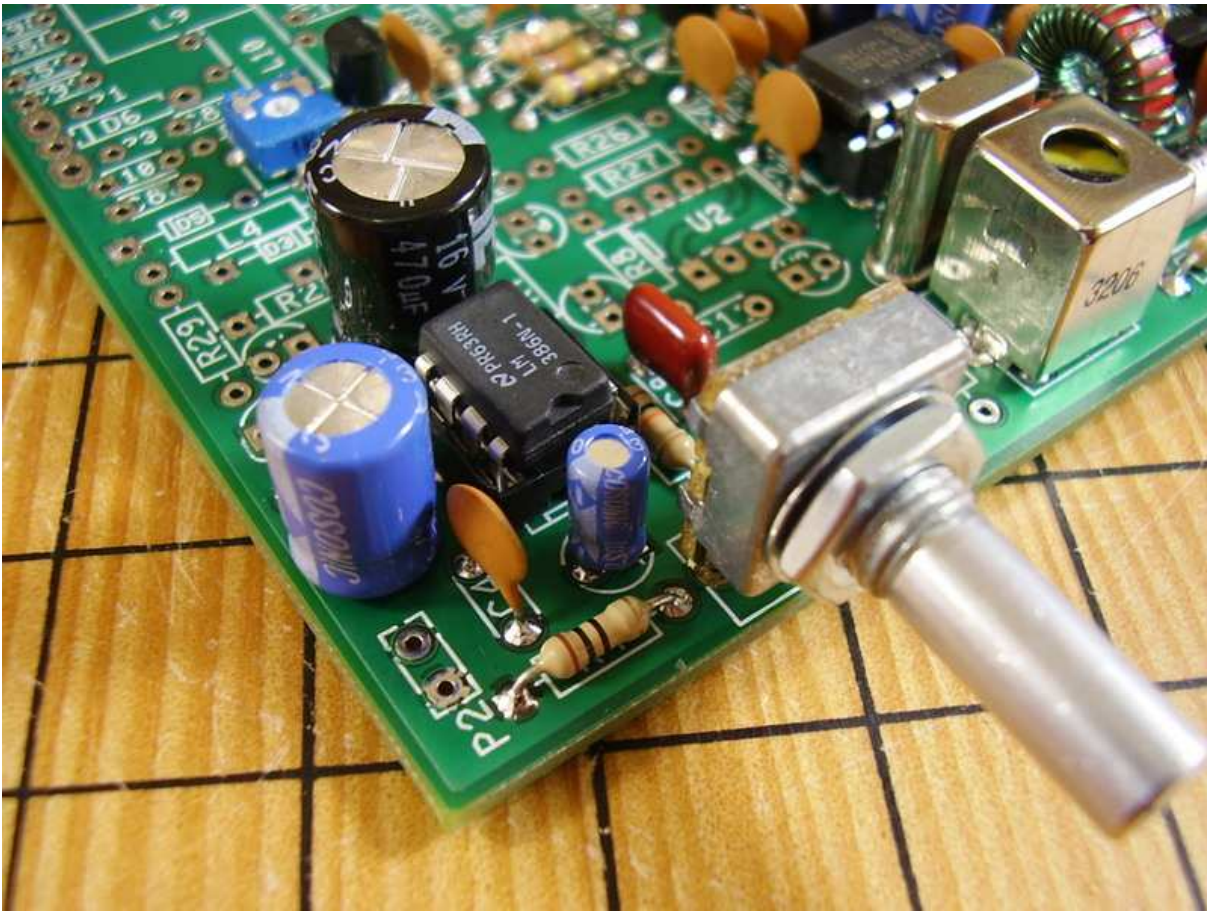
Figure 7.18: [5-20] R6 10K potentiometer.
