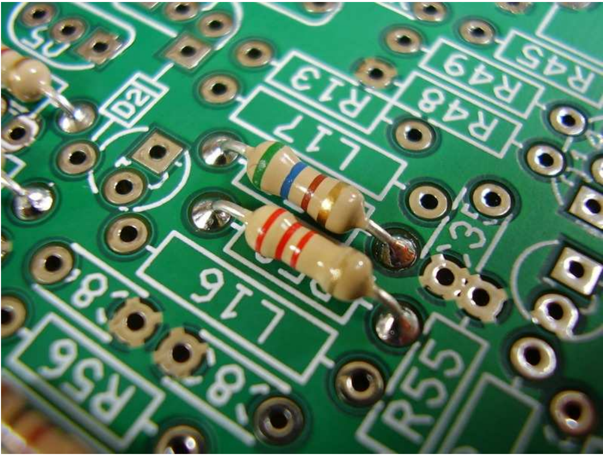
Figure 4.7: [2-9] R58 2.2K.
