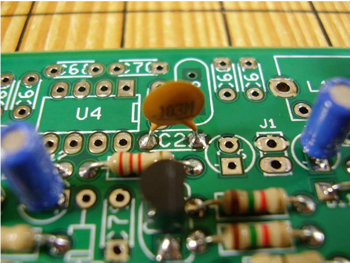
Figure 3.54: [1-23] C2.
