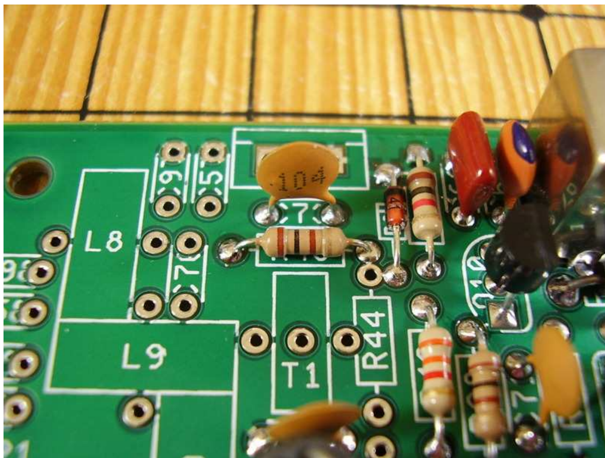
Figure 9.17: [7-18] R43 100 ohms.
