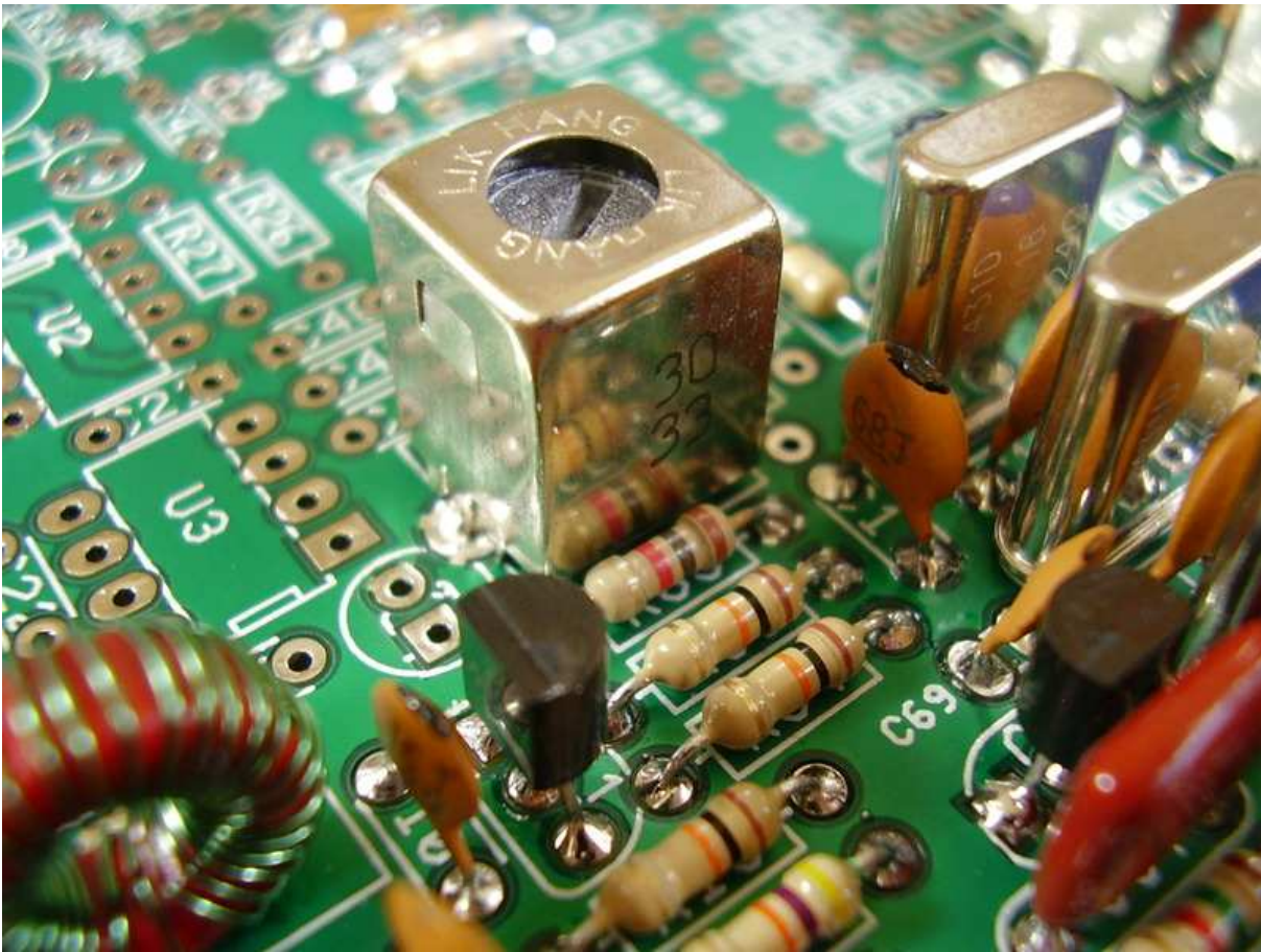
Figure 6.36: [4-35] L5 5.8\mu\text{H} (30-33).
