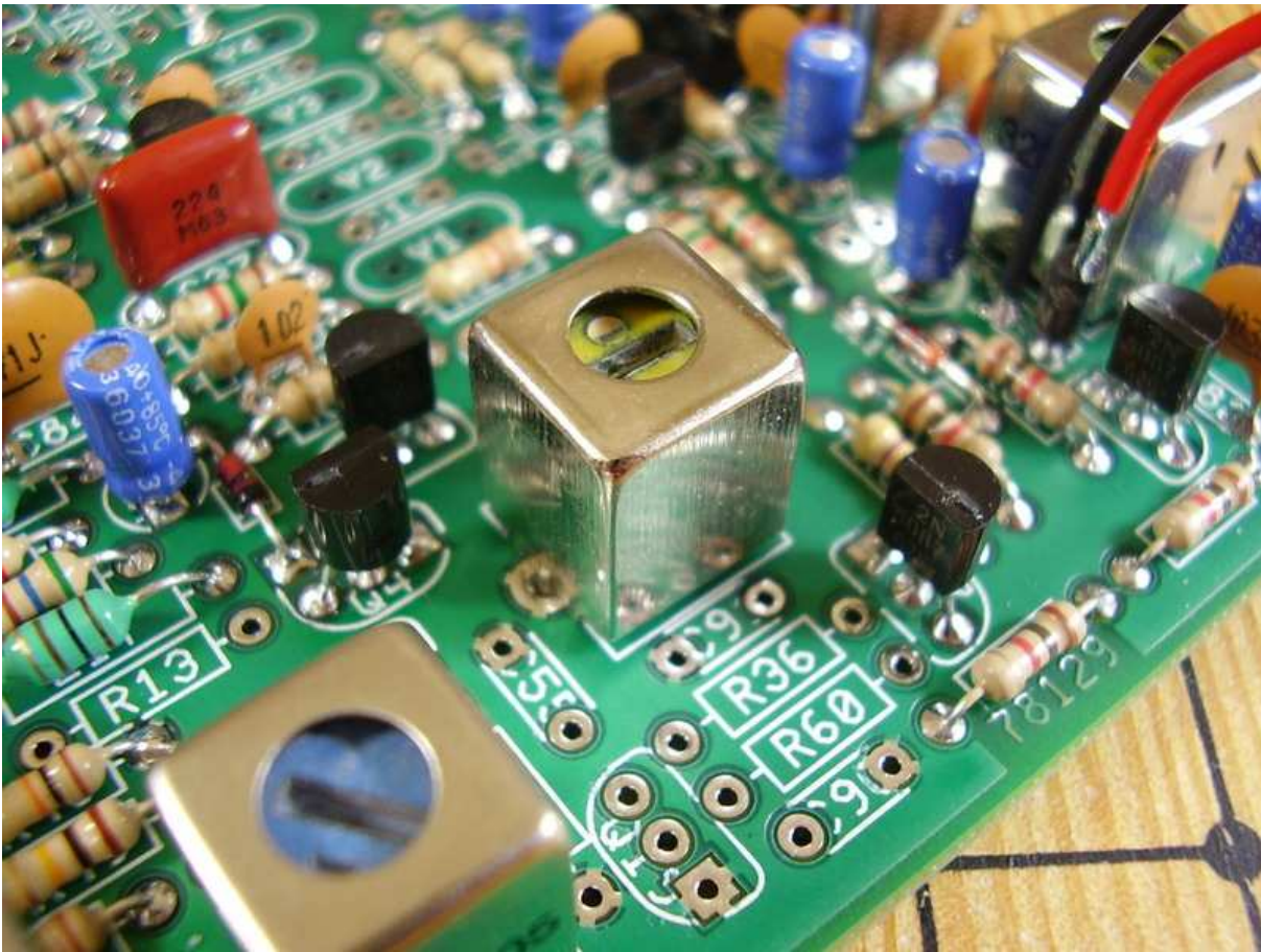
Figure 6.5: [4-3] L7 1.3\mu\text{H} (3206).
