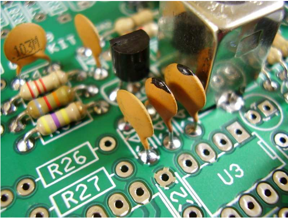
Figure 6.46: [4-45] C46 .01\mu\text{F} .
