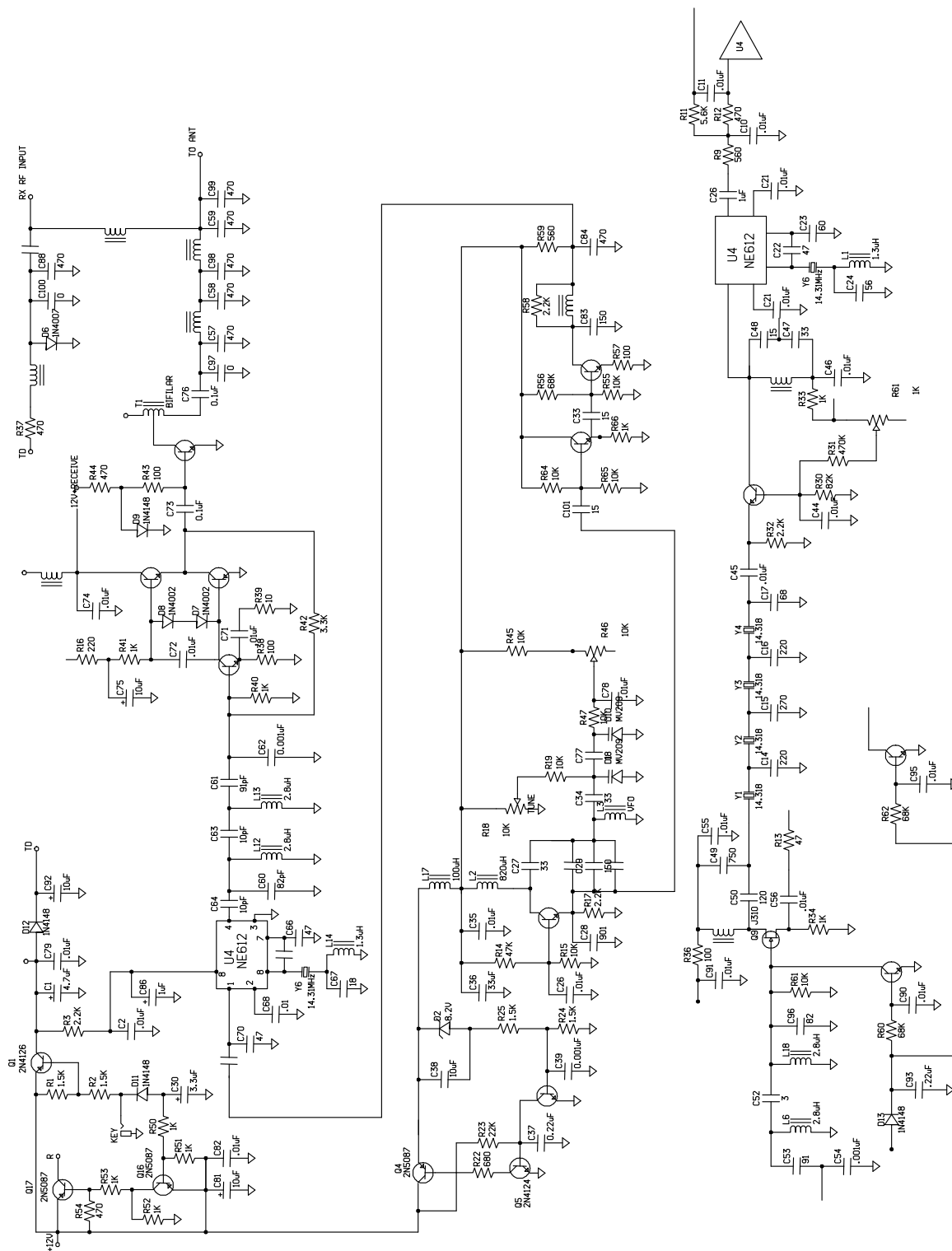
Figure 11.5: TT1340 Schematic.
