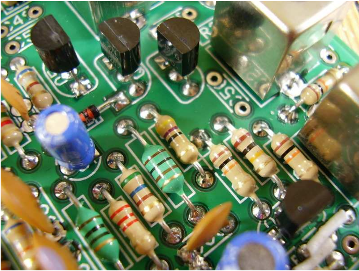
Figure 6.10: [4-7] R13 47 ohms.
