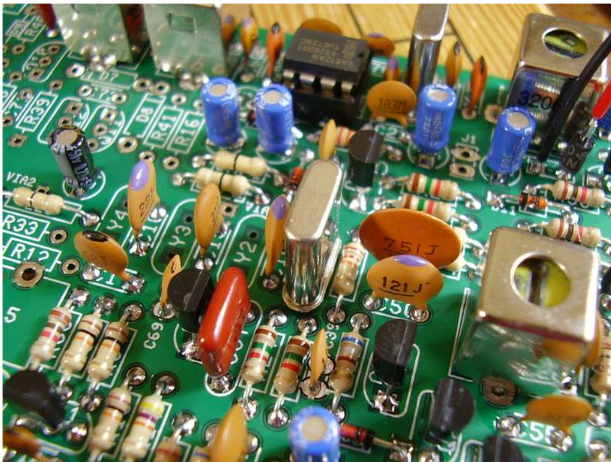
Figure 6.31: [4-33] [4-26] C17 68pF and Y1 14.31818MHz Crystal.
