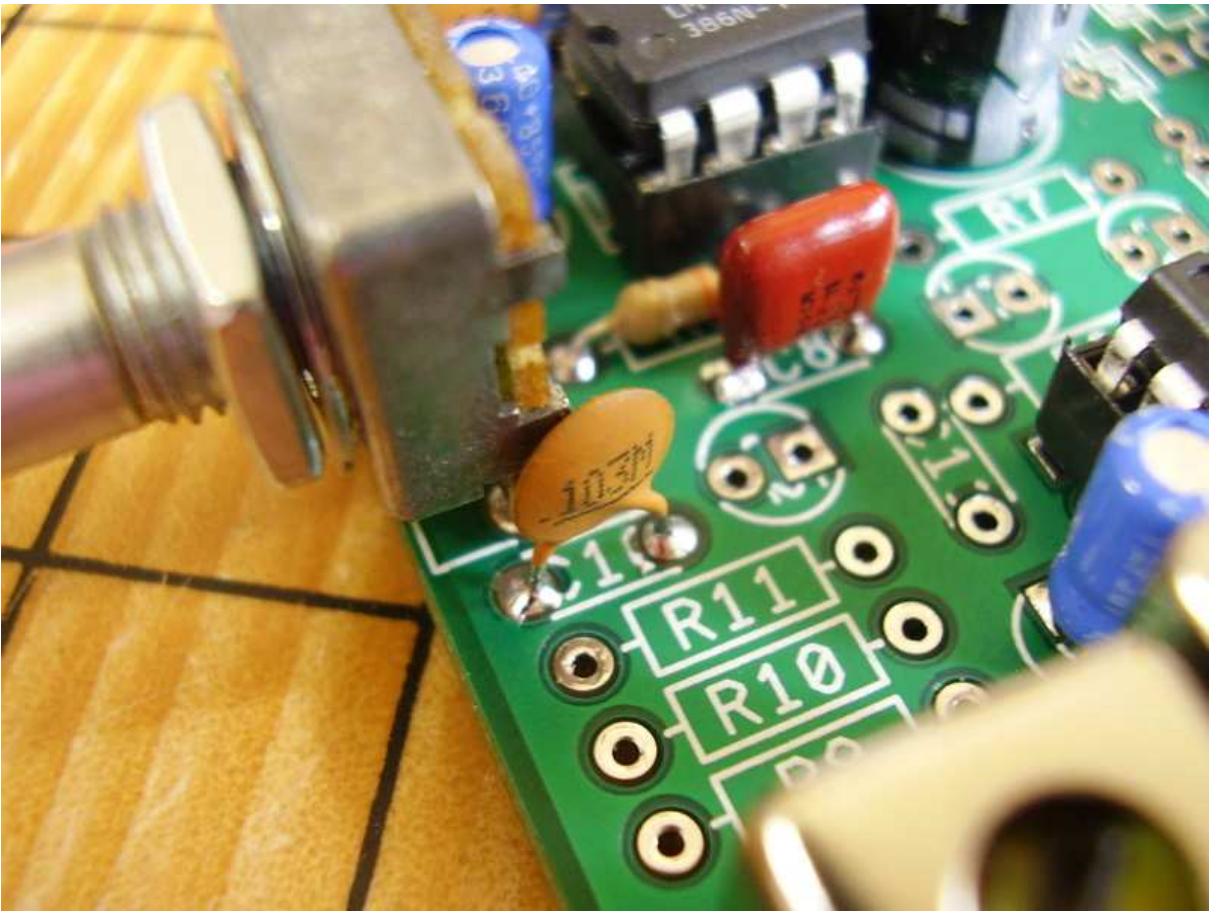
Figure 8.2: [6-2] C10 .01 \mu F.
