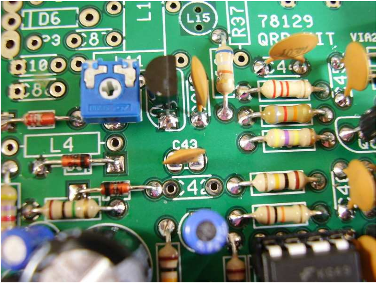
Figure 8.24: [6-21] C43 .001\mu\text{F} (102).
