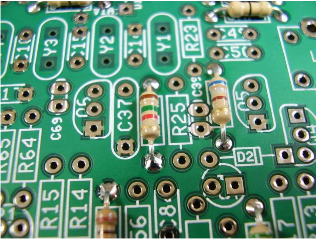
Figure 4.4: [2-6] R24 1.5K.
