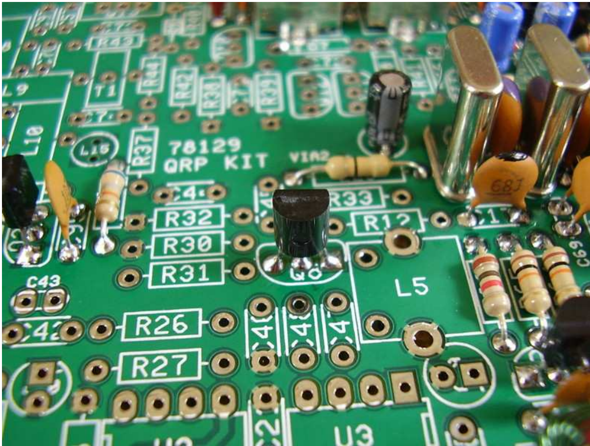
Figure 6.35: [4-34] Q8 2N4124.
