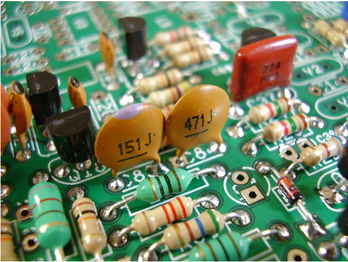
Figure 4.48: [2-45] C84 470pF.
