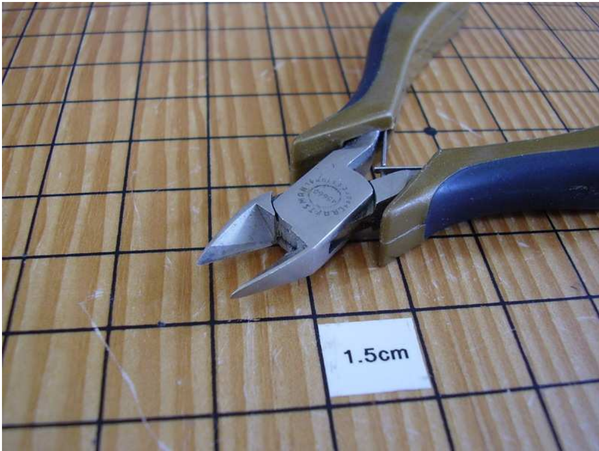
Figure 2.2: Diagonal Cutters.
