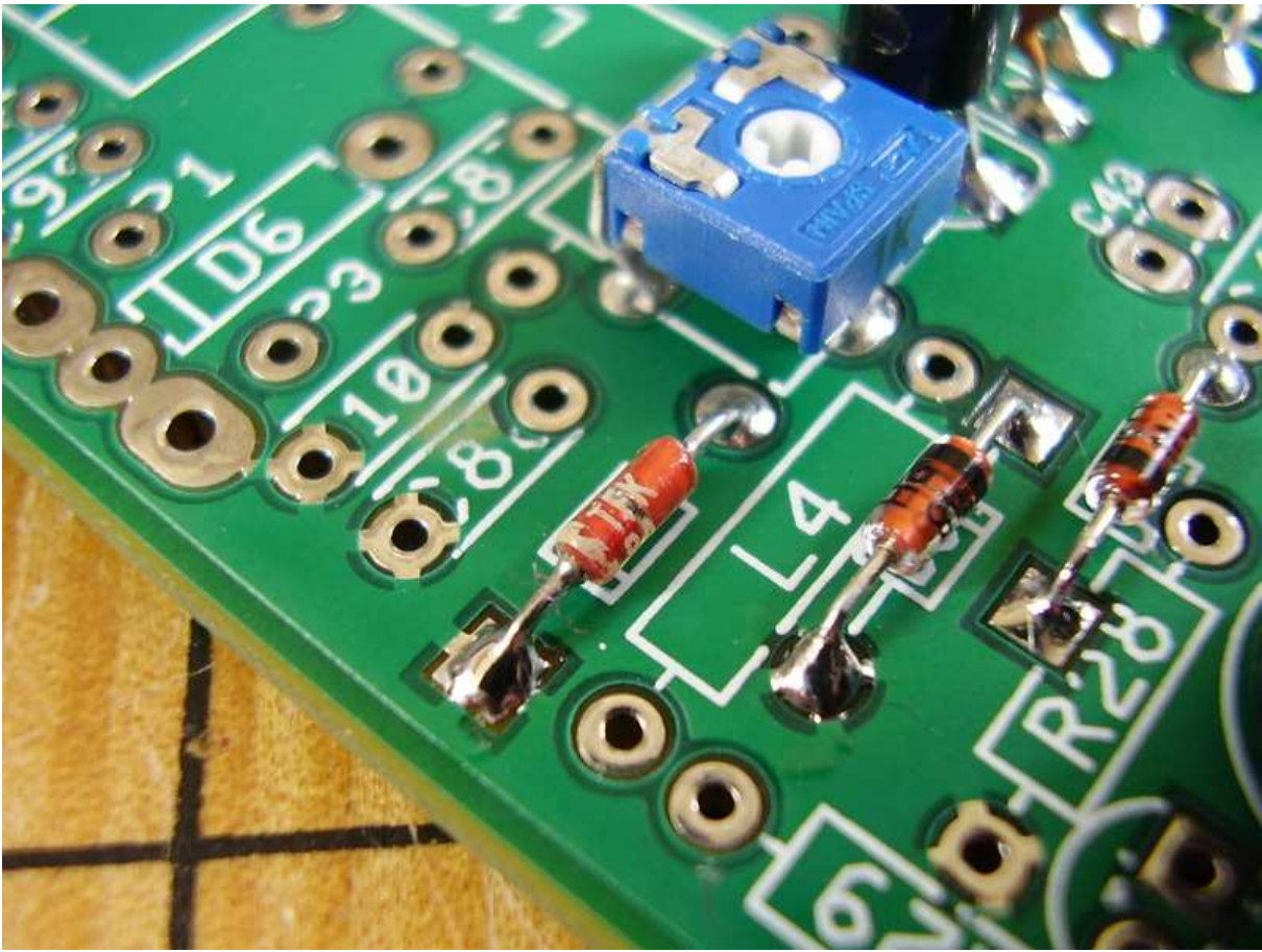
Figure 8.16: [6-13] D5 BA479.
