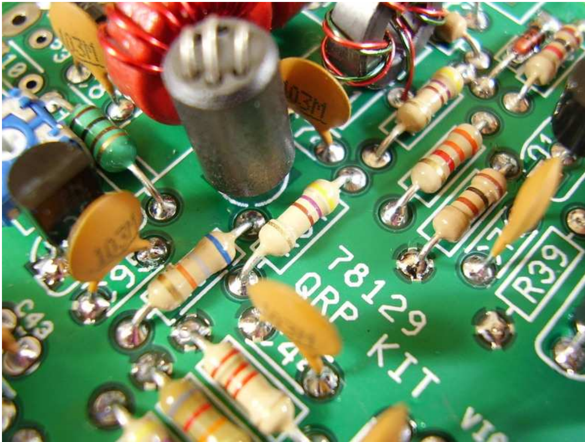
Figure 9.33: [7-37] R37 470 ohms.
