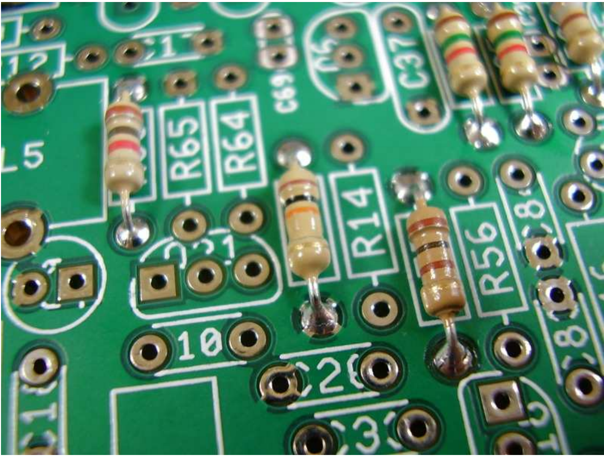
Figure 4.8: [2-10] R15 10K.
