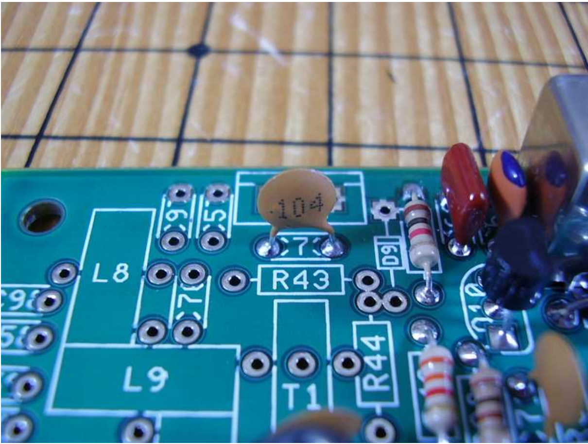
Figure 9.14: [7-15] C73 .1 \mu F (104).
