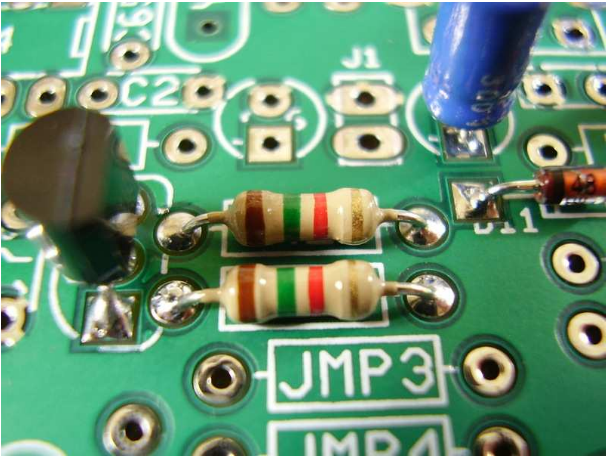
Figure 3.41: [1-12] R2.
