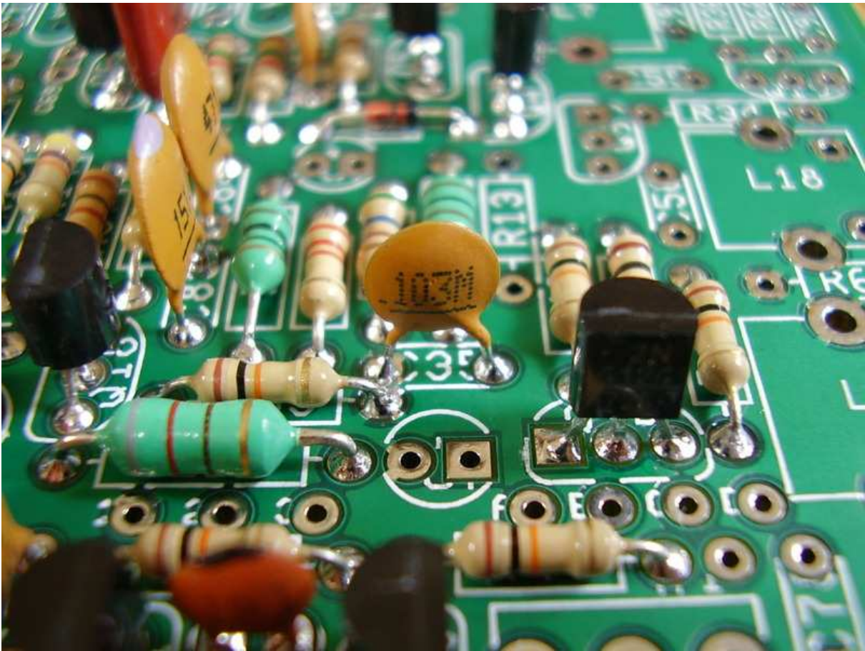
Figure 4.51: [2-48] C35 .04\mu\text{F} .
