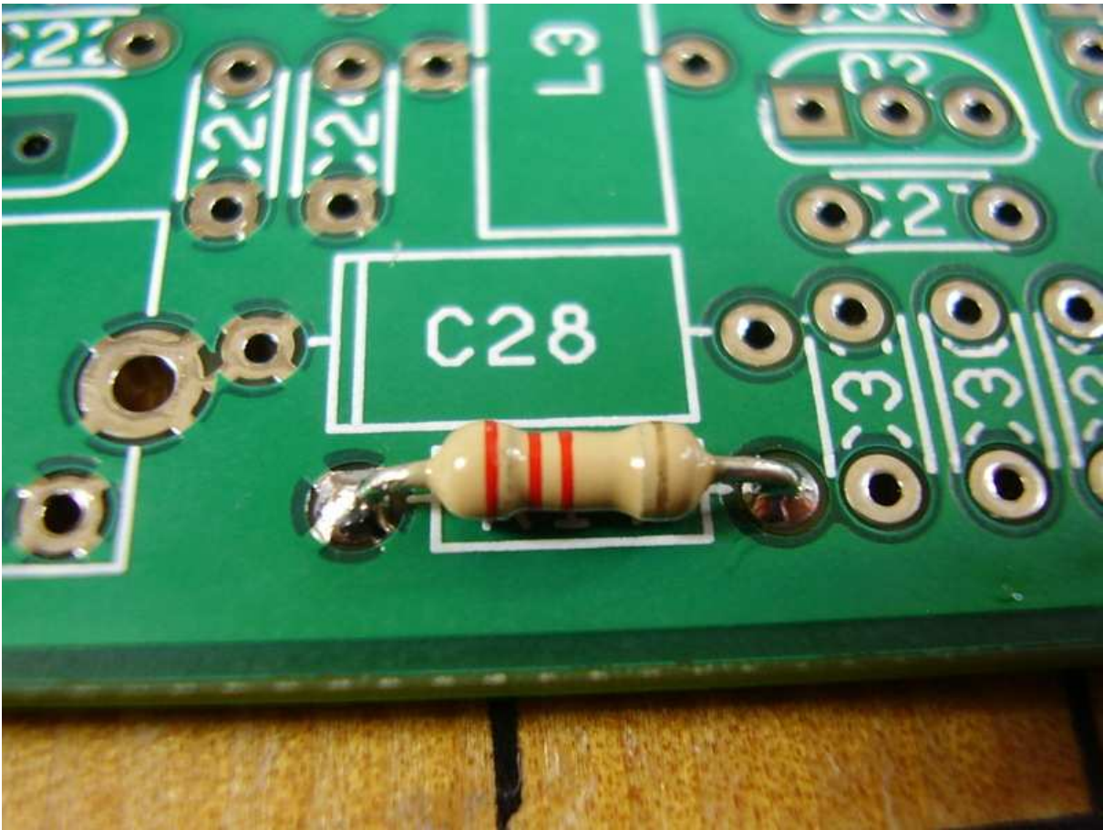
Figure 4.6: [2-8] R17 2.2K.
