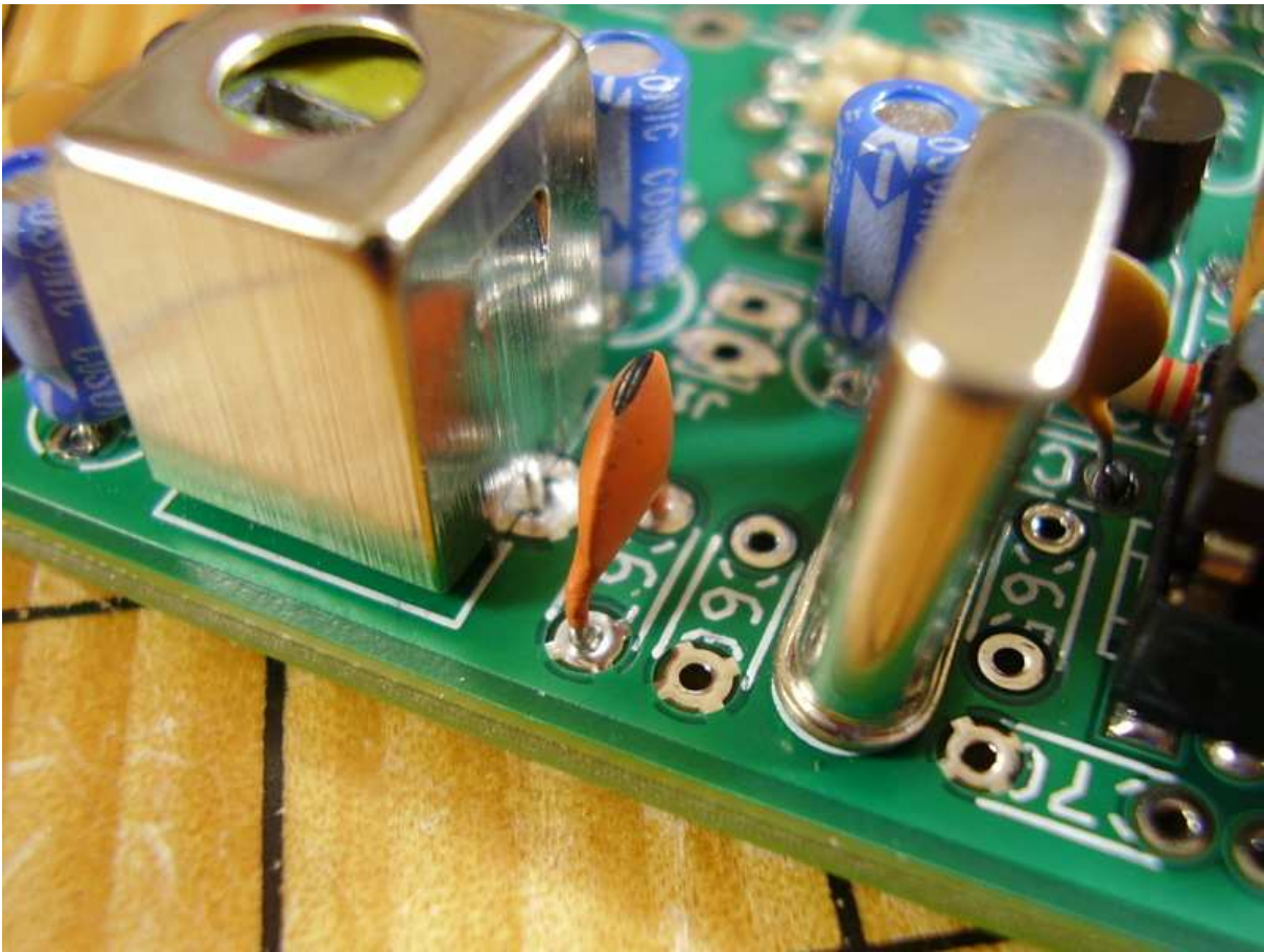
Figure 5.9: [3-6] C67 56pF.
