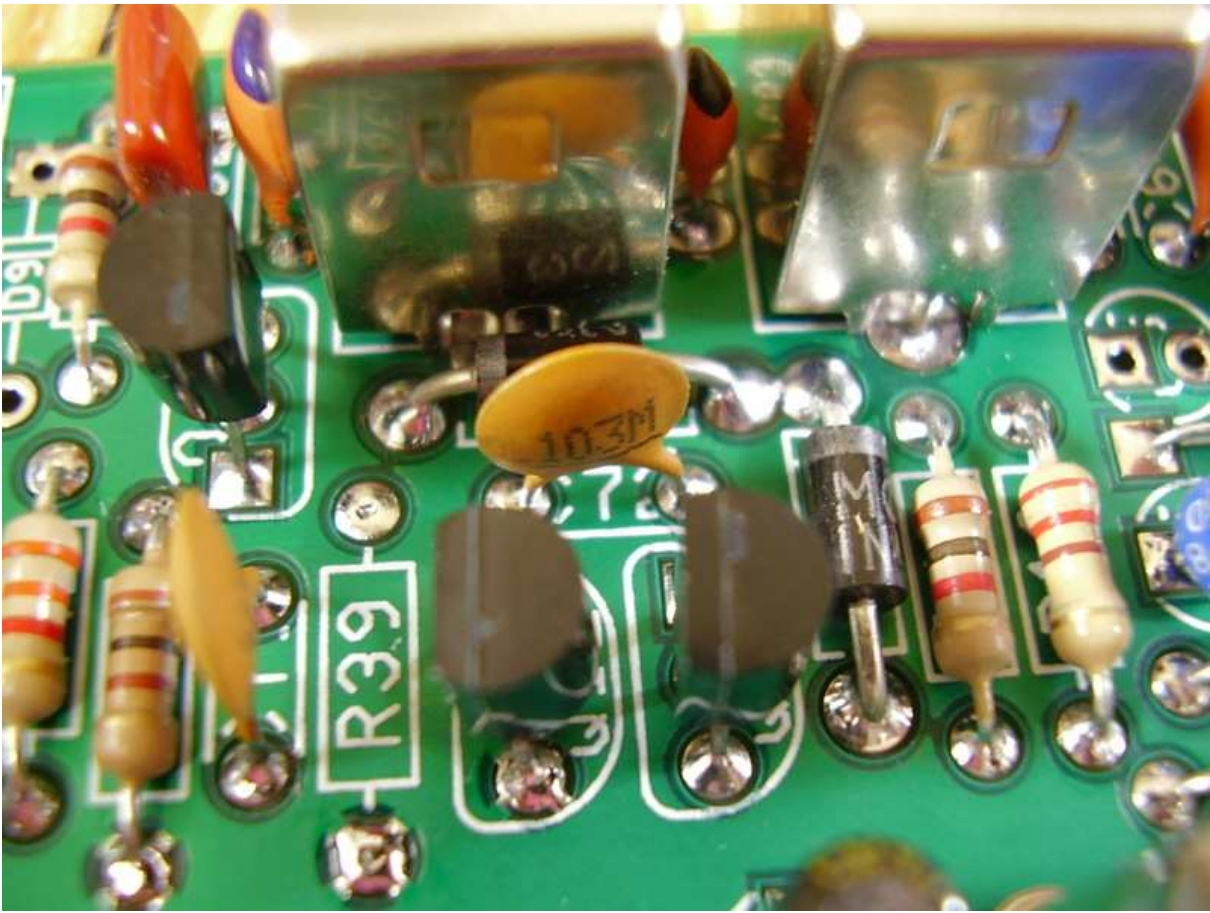
Figure 9.12: [7-12] C71 .01\mu\text{F} (103).
