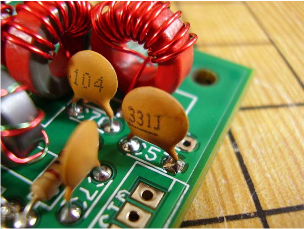
Figure 9.28: [7-30] C57 330pF (331).
