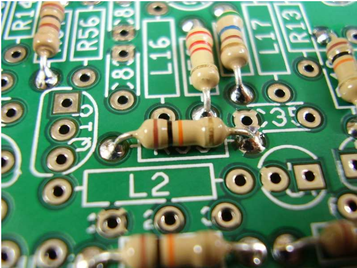
Figure 4.13: [2-15] R55 10K.
