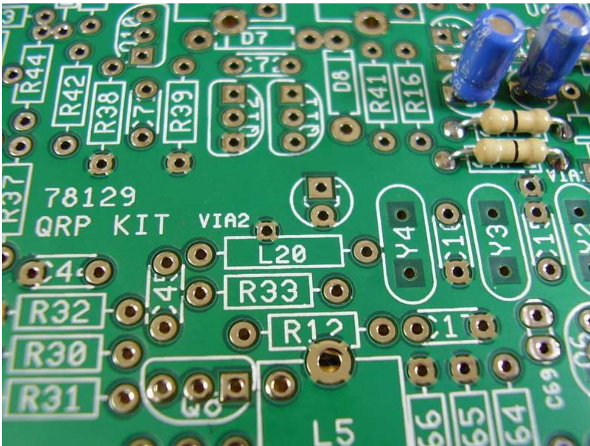
Figure 3.57: L20 Location.
