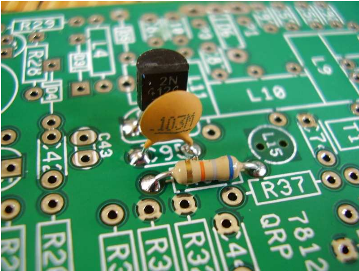
Figure 6.25: [4-23] C56 .01 \mu F.
