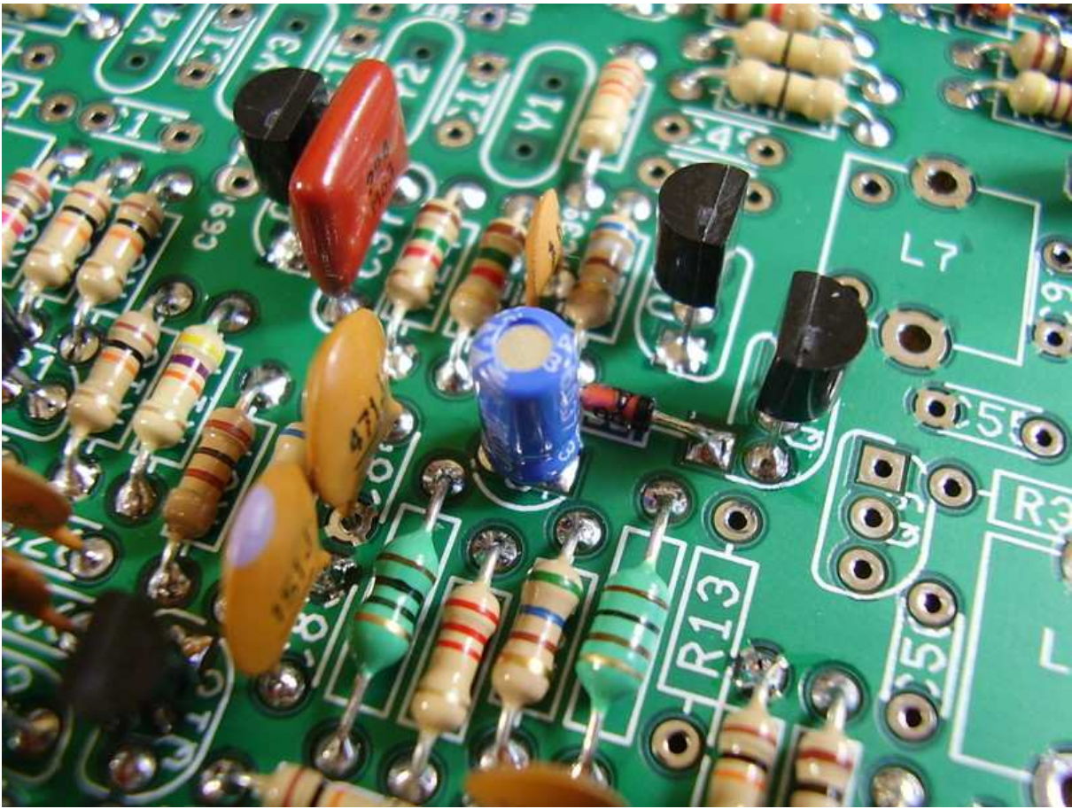
Figure 4.53: [2-50] C38 10\mu\text{F} .
