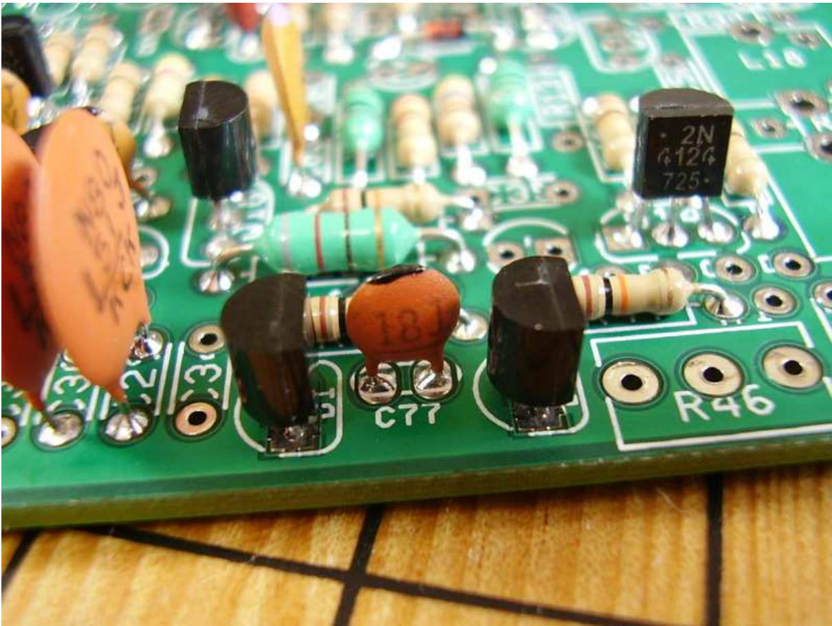
Figure 4.44: [2-41] C77 18pF.
