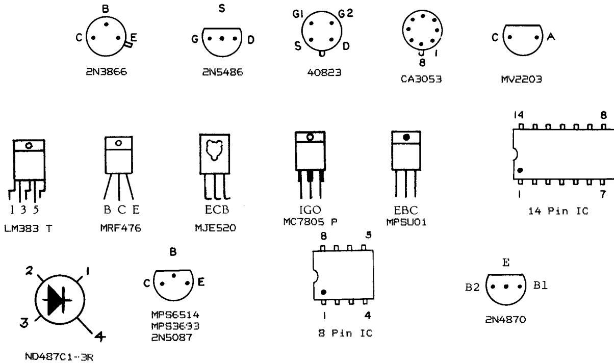
Figure 11 - Semiconductor Terminations
