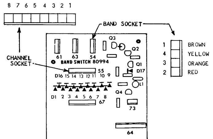
Figure 3 - BAND SWITCH Assembly Printing
