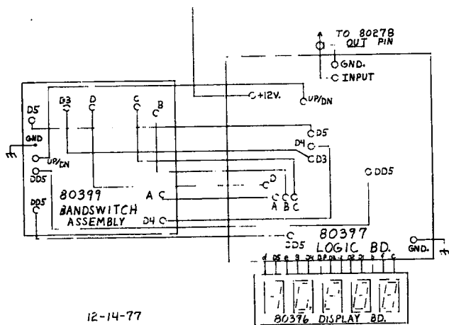
WIRING DIAGRAM
