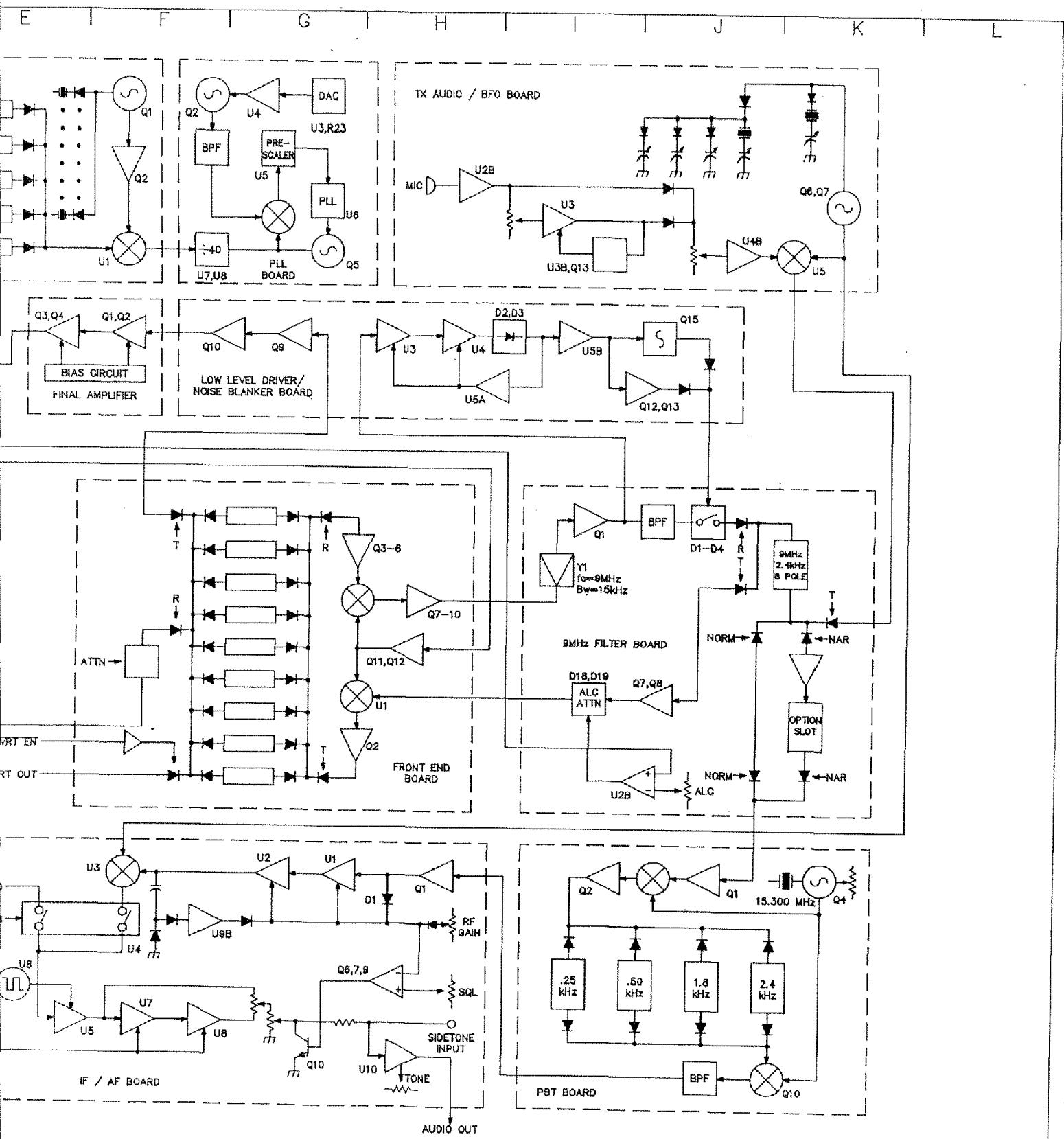
FIGURE 6-1 BLOCK DIAGRAM 562
